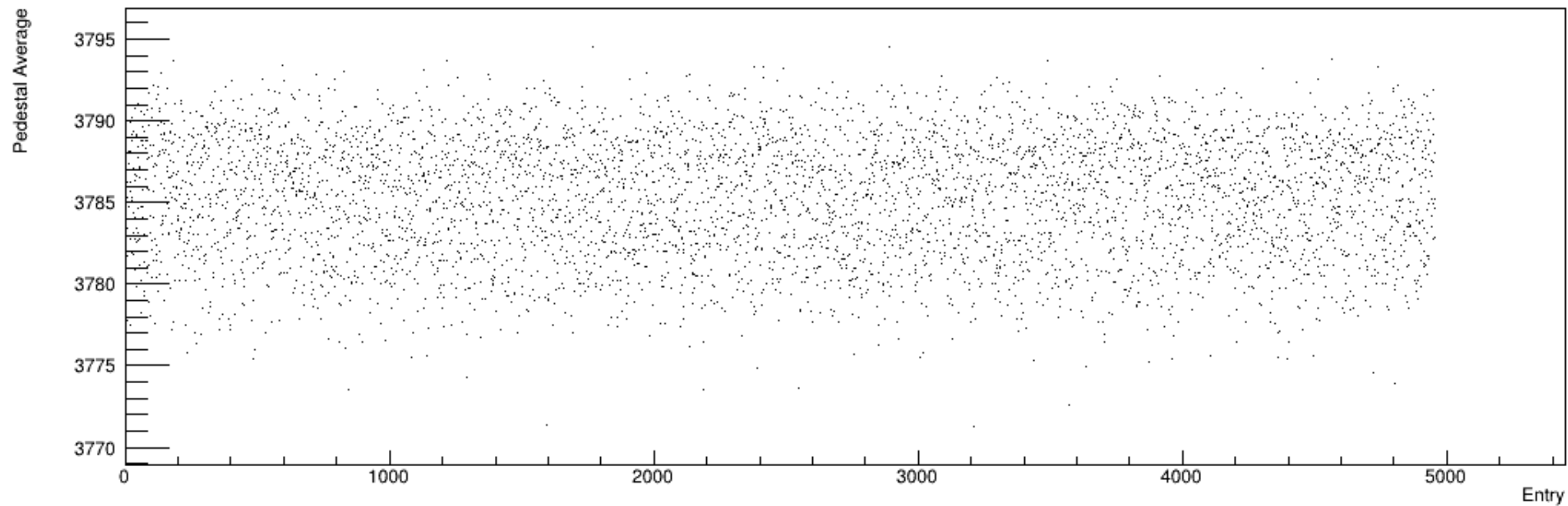
Run 5581, snapshots: Pedestal vs. Time
