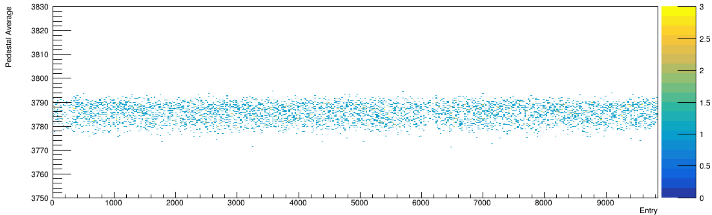
Run 5581, snapshots: Pedestal vs. Time
