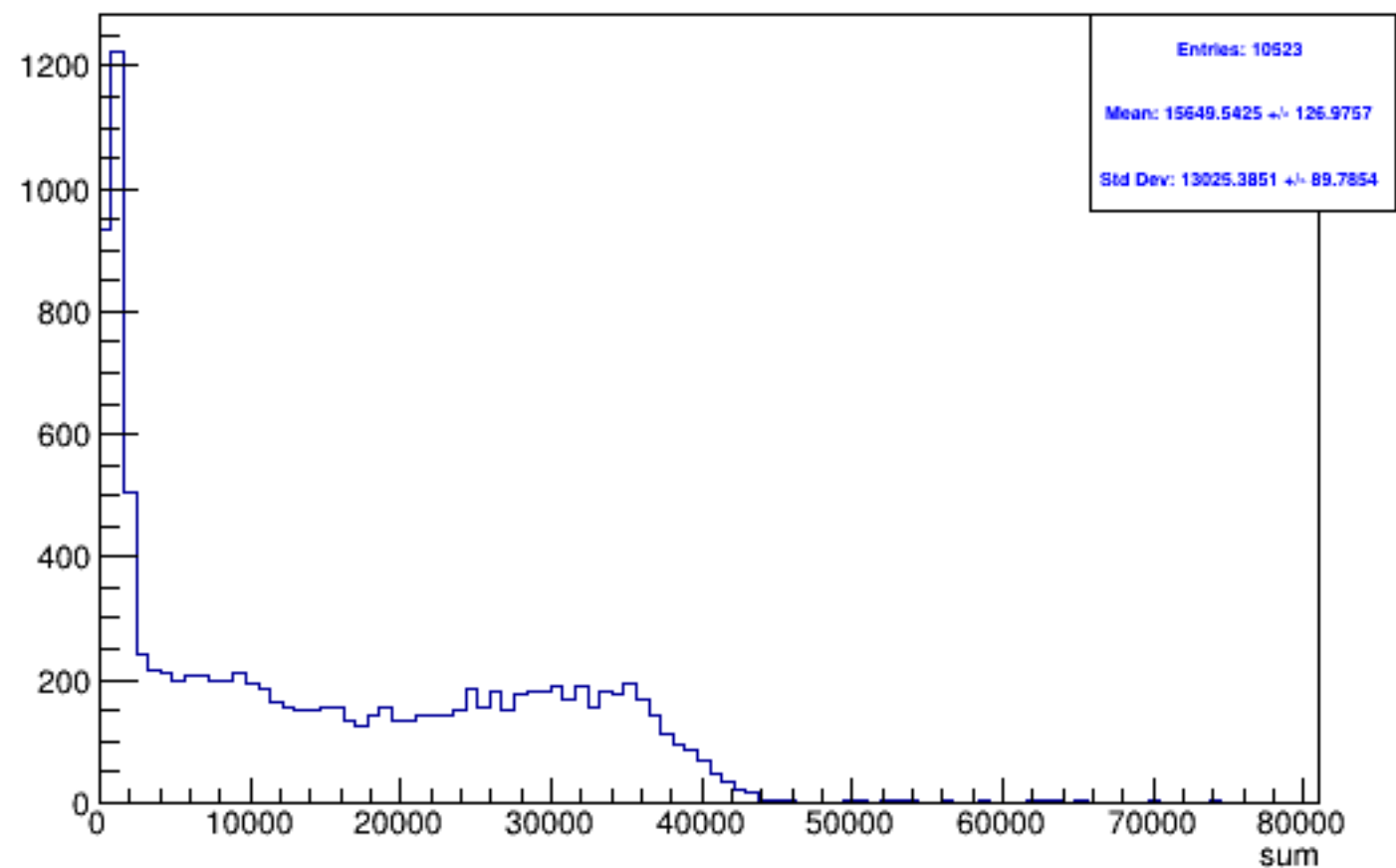
Run 5581 triggerwise, sums: All
