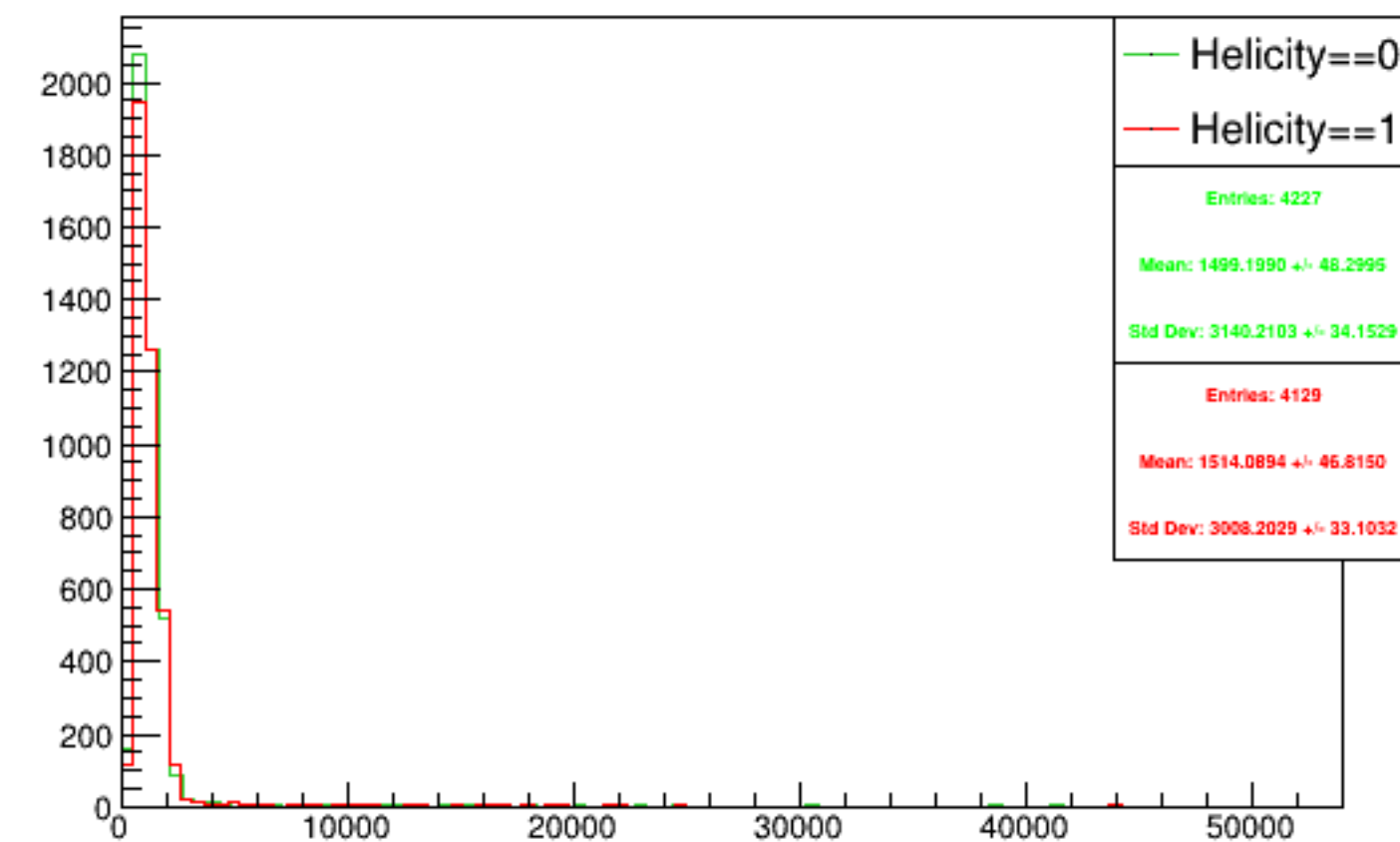
Run 5582 triggerwise, sums: Beam ON, Laser OFF
