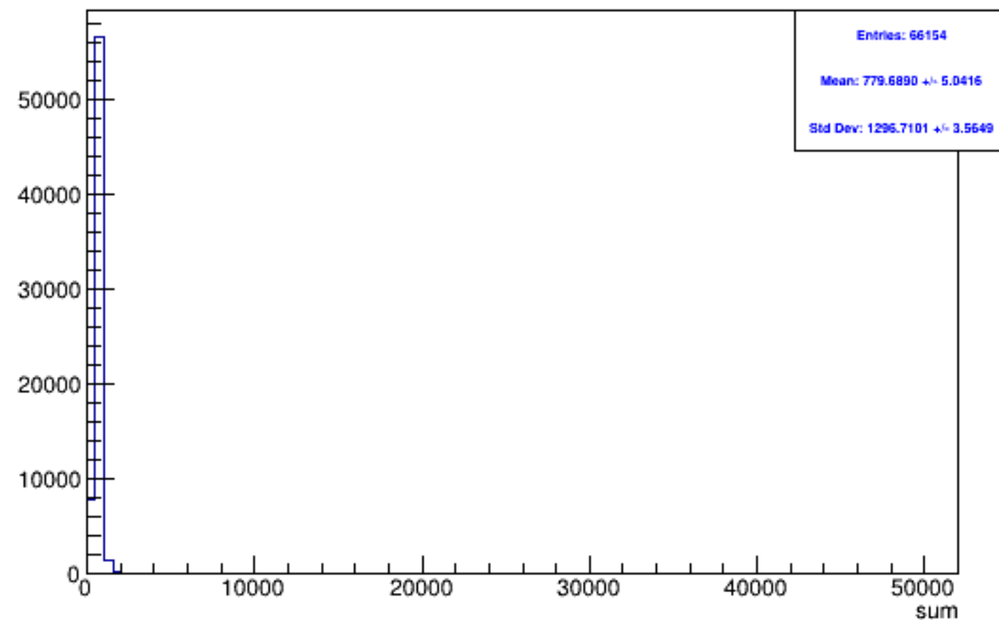
Run 5582 triggerwise, sums: Beam OFF
