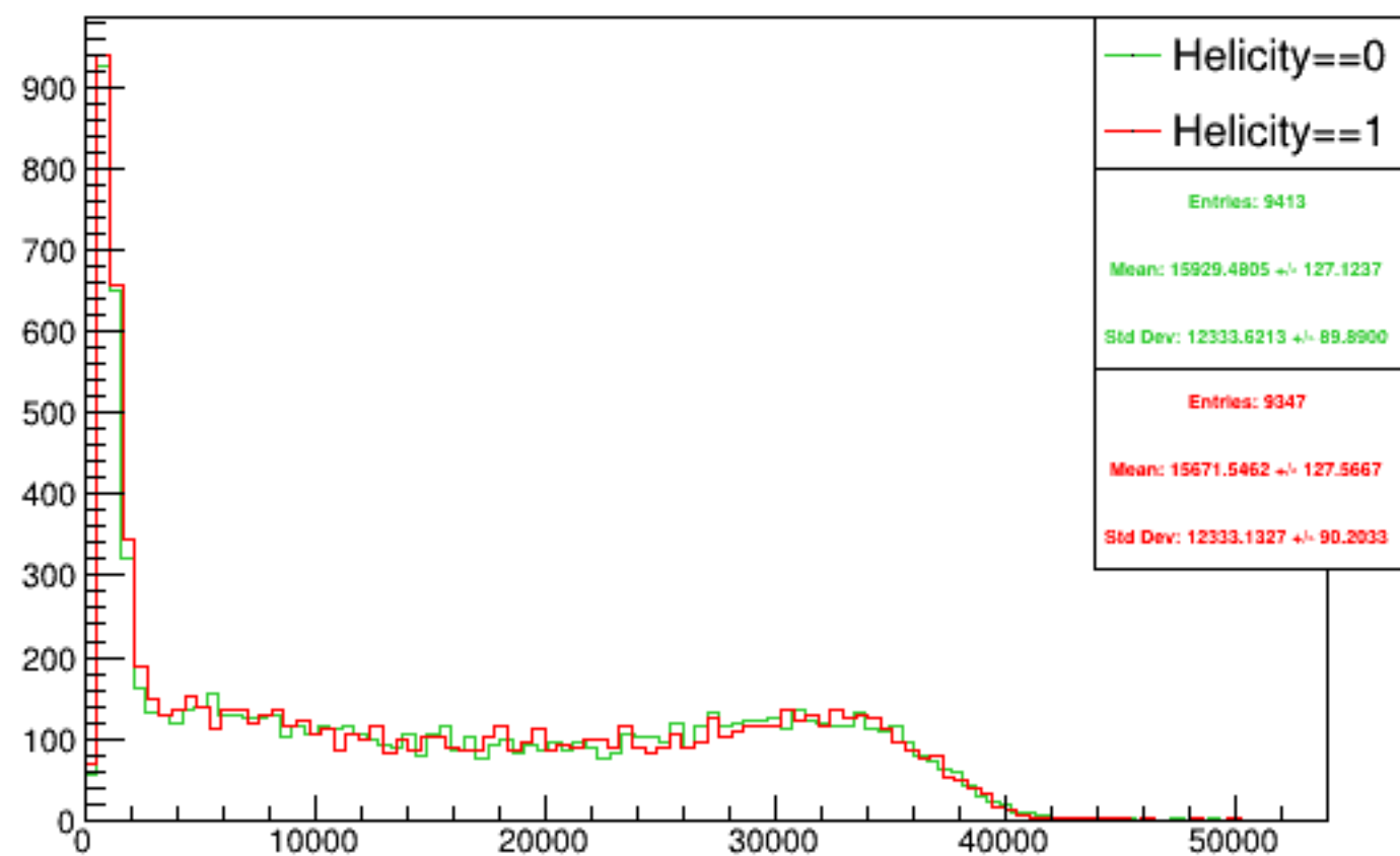
Run 5582 triggerwise, sums: Beam ON, Laser ON
