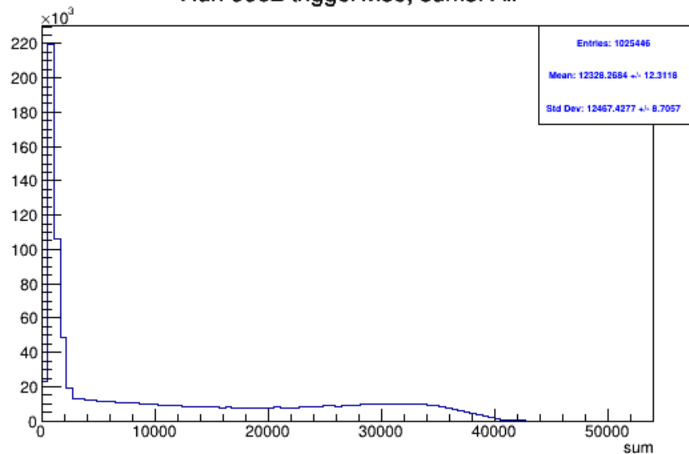
Run 5582 triggerwise, sums: All
