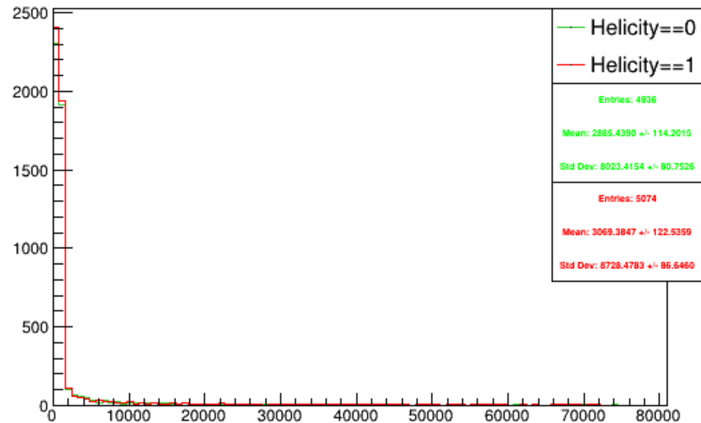
Run 5584 triggerwise, sums: Beam ON, Laser OFF
