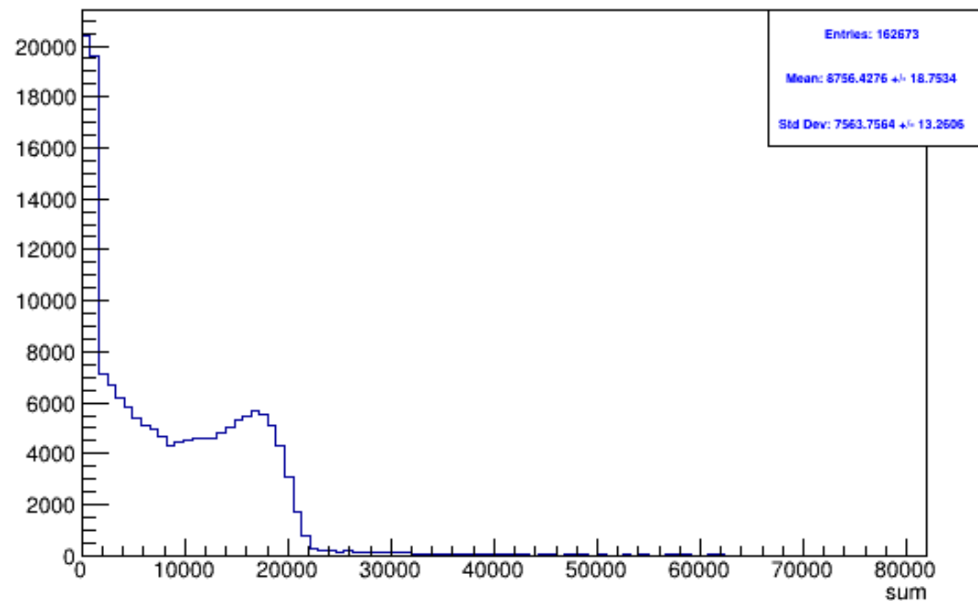
Run 5584 triggerwise, sums: All
