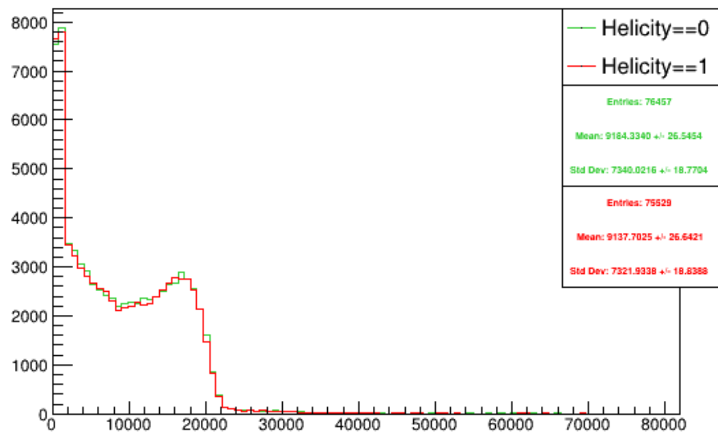
Run 5584 triggerwise, sums: Beam ON, Laser ON
