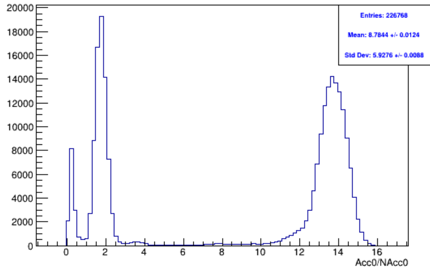
Run 5589 mpwise, acc0: All
