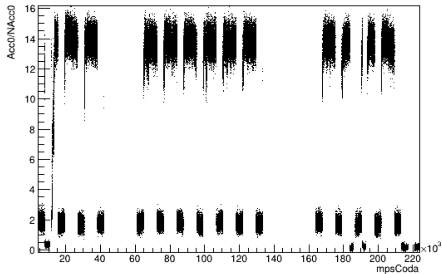
Run 5589 mpwise, Acc0 vs Time: All
