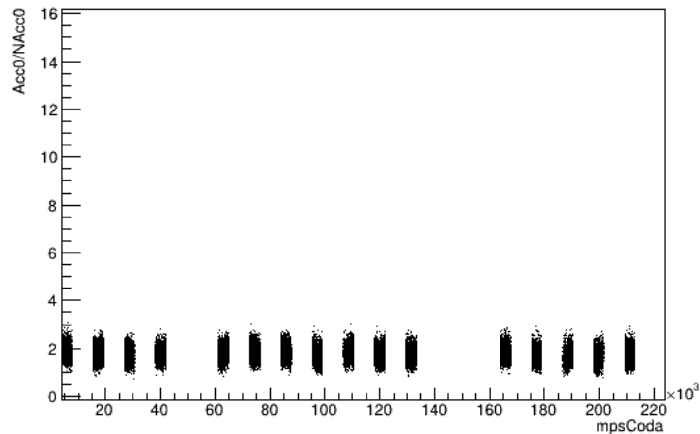
Run 5589 mpwise, Acc0 vs Time: Beam ON, Laser OFF
