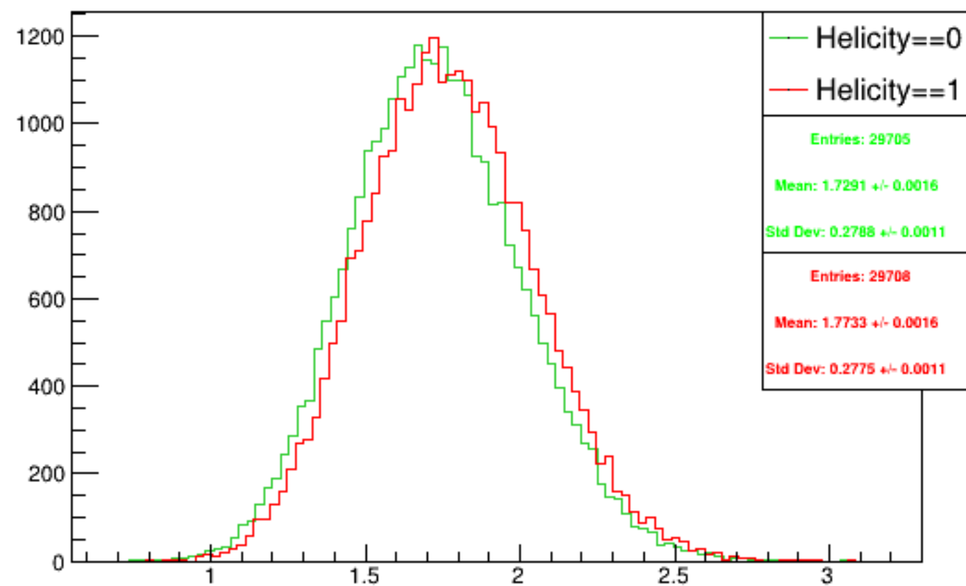
Run 5589 mpwise, acc0: Beam ON, Laser OFF
