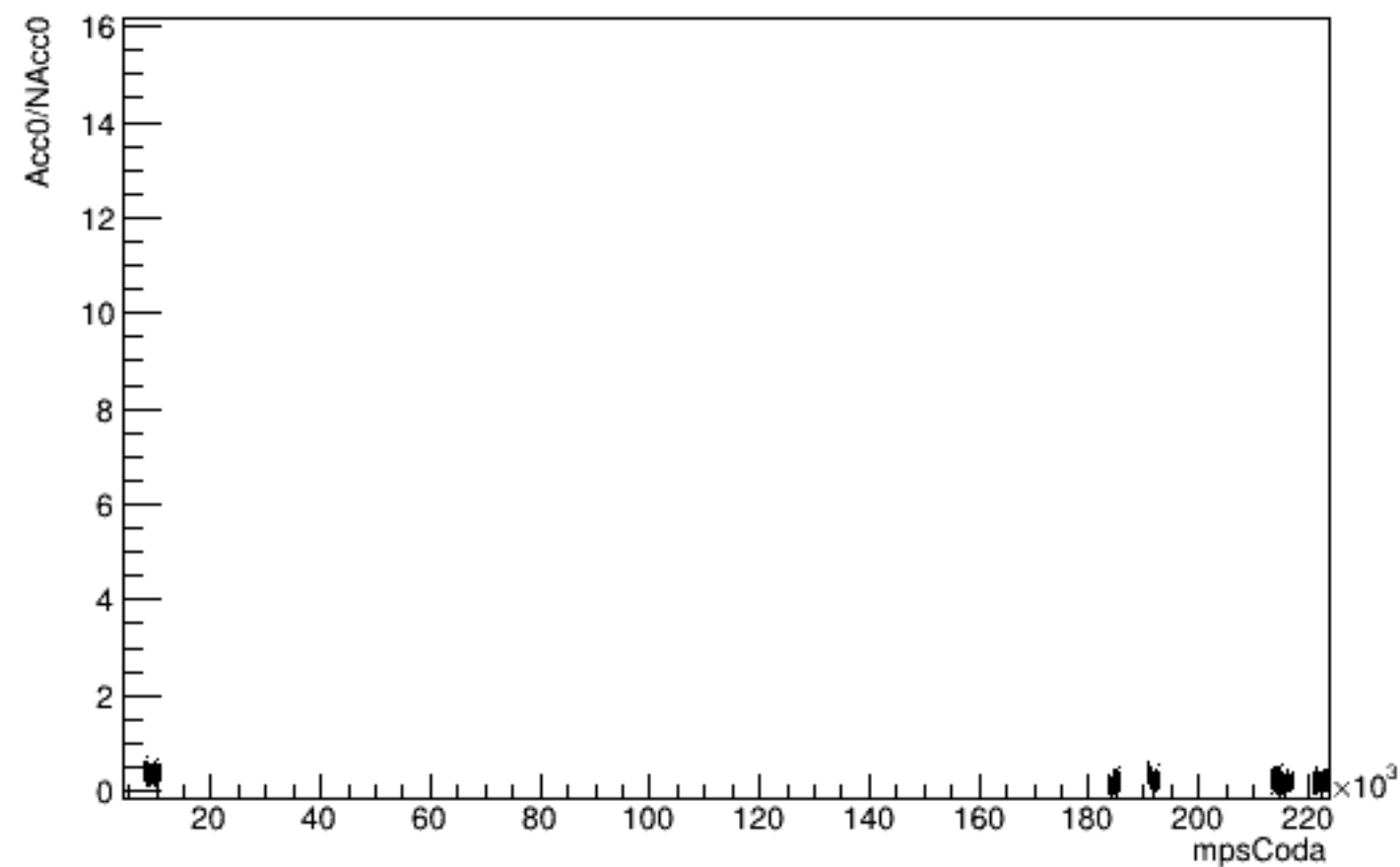
Run 5589 mpwise, Acc0 vs Time: Beam OFF
