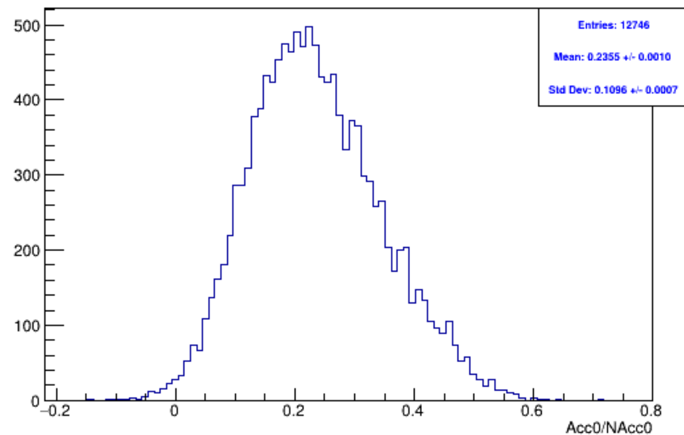
Run 5589 mpwise, acc0: Beam OFF
