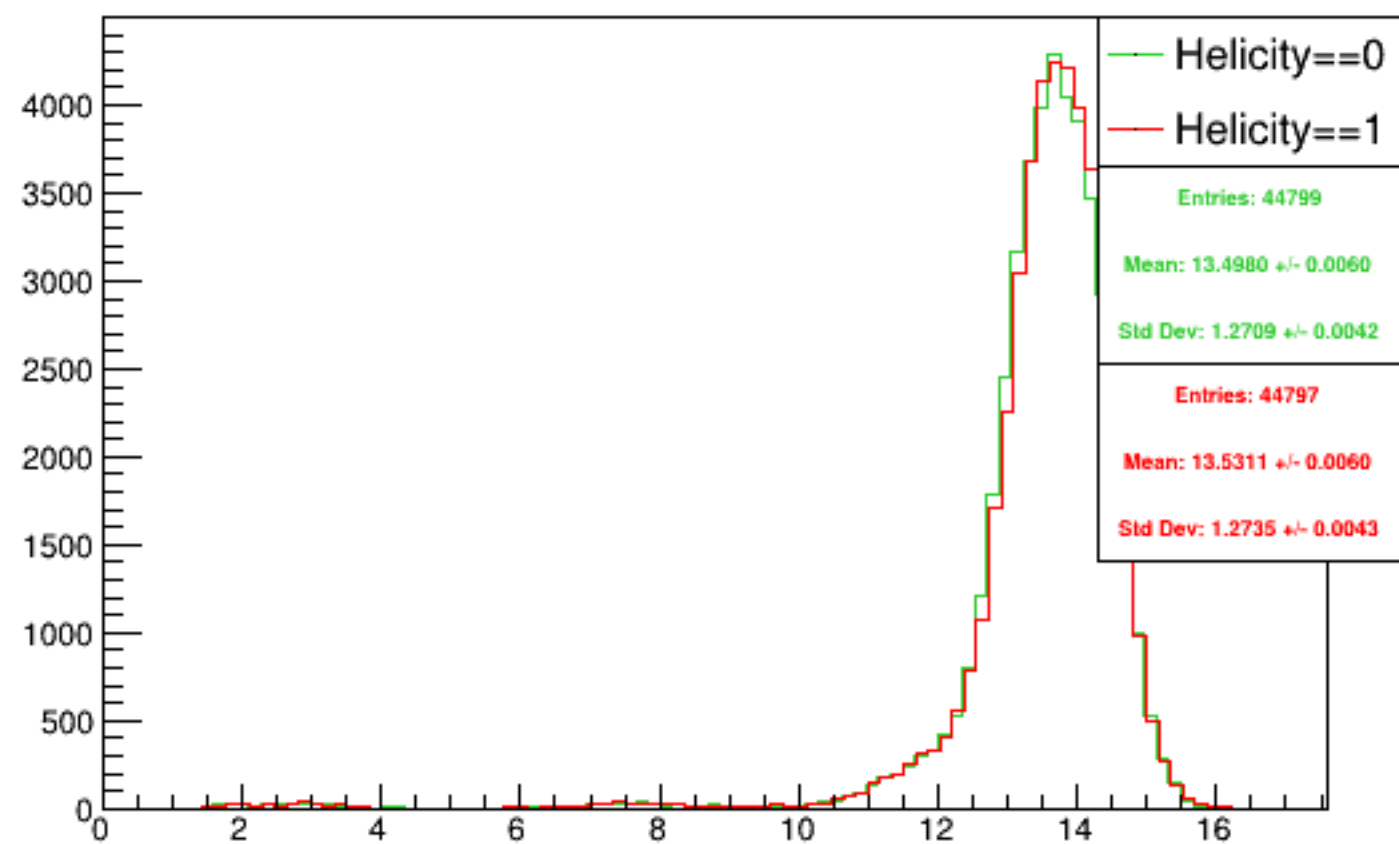
Run 5589 mpwise, acc0: Beam ON, Laser ON
