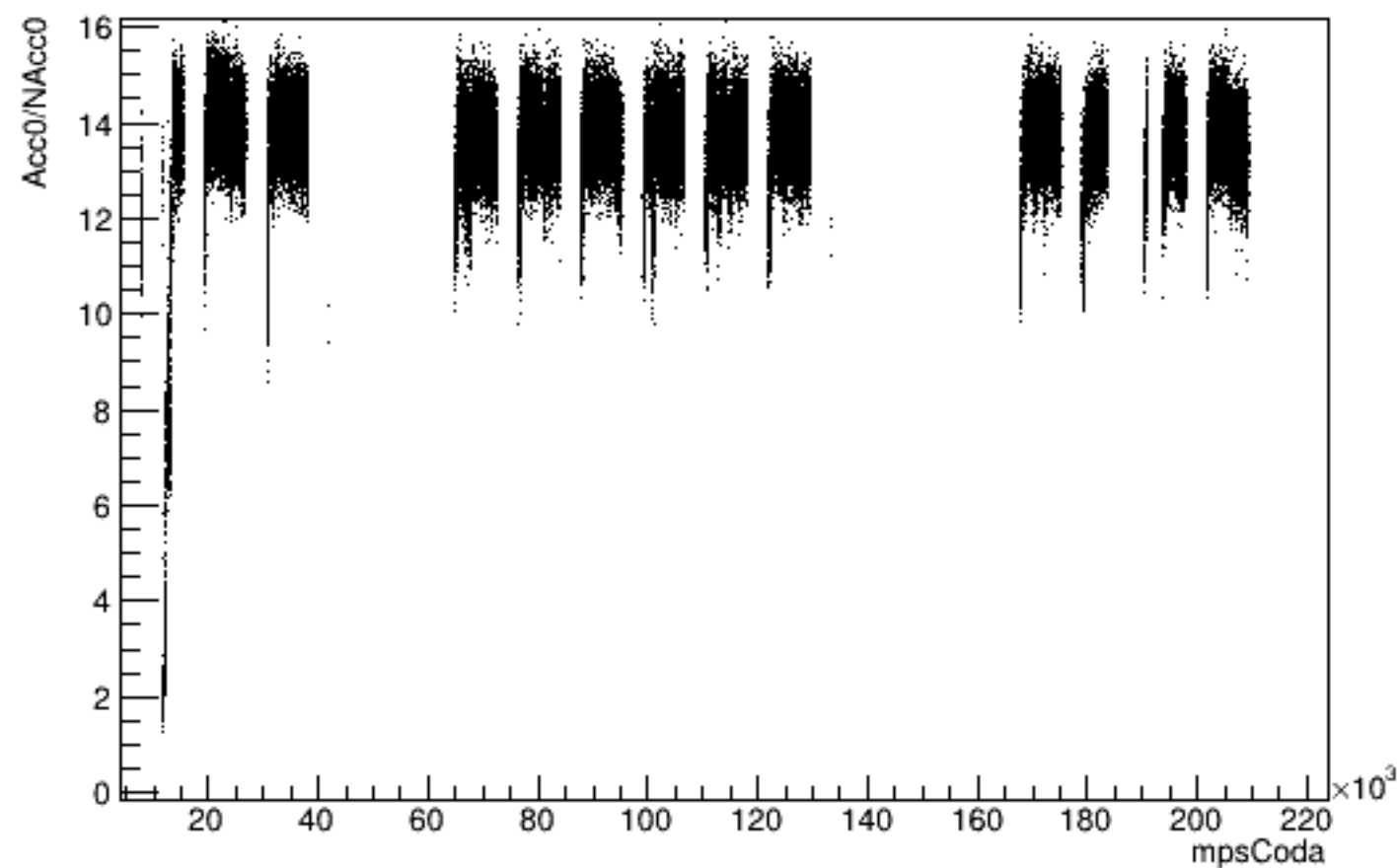
Run 5589 mpwise, Acc0 vs Time: Beam ON, Laser ON
