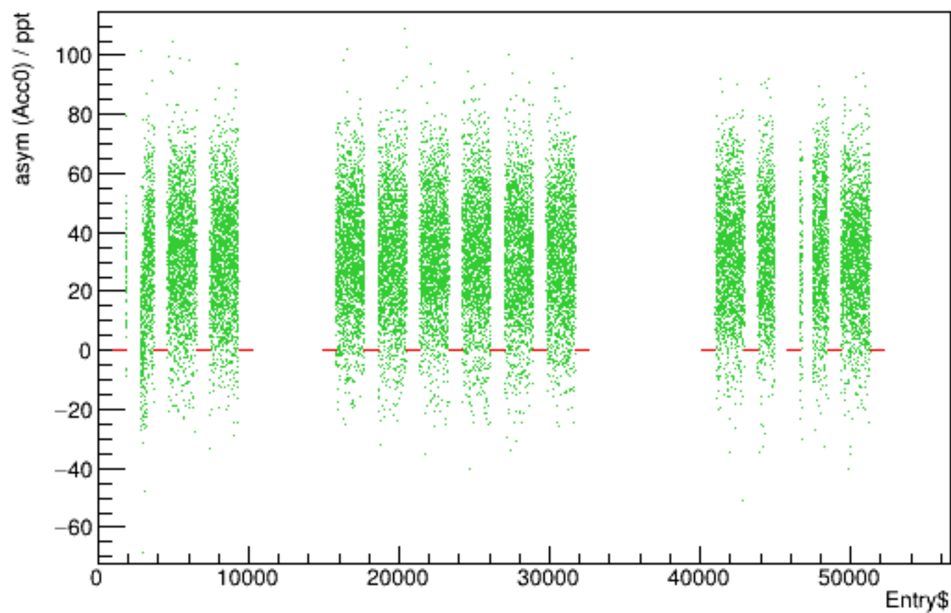
Run 5589 quartetwise, asym0sub vs time
