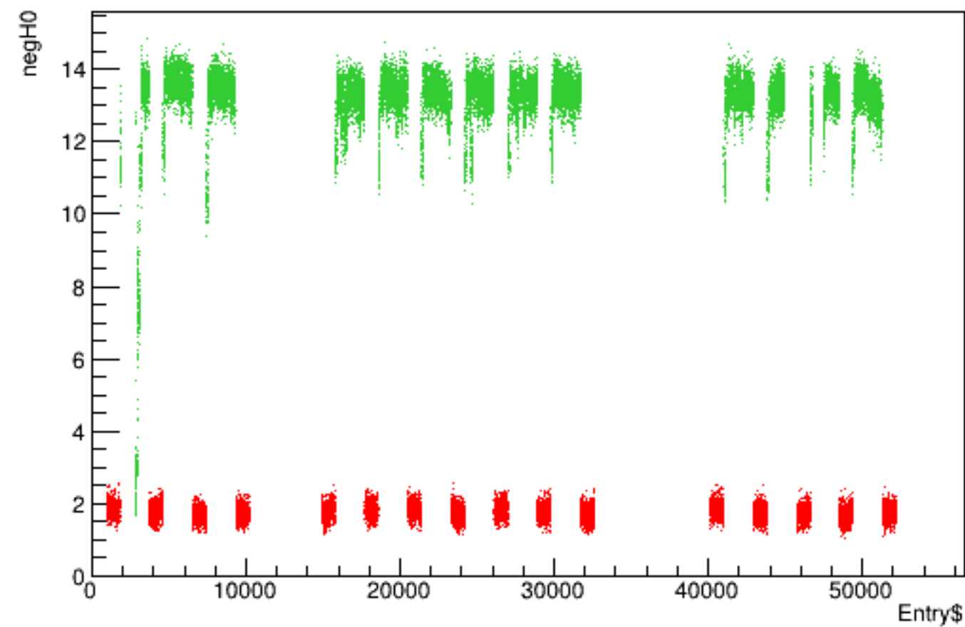
Run 5589 quartetwise, negH0 vs time
