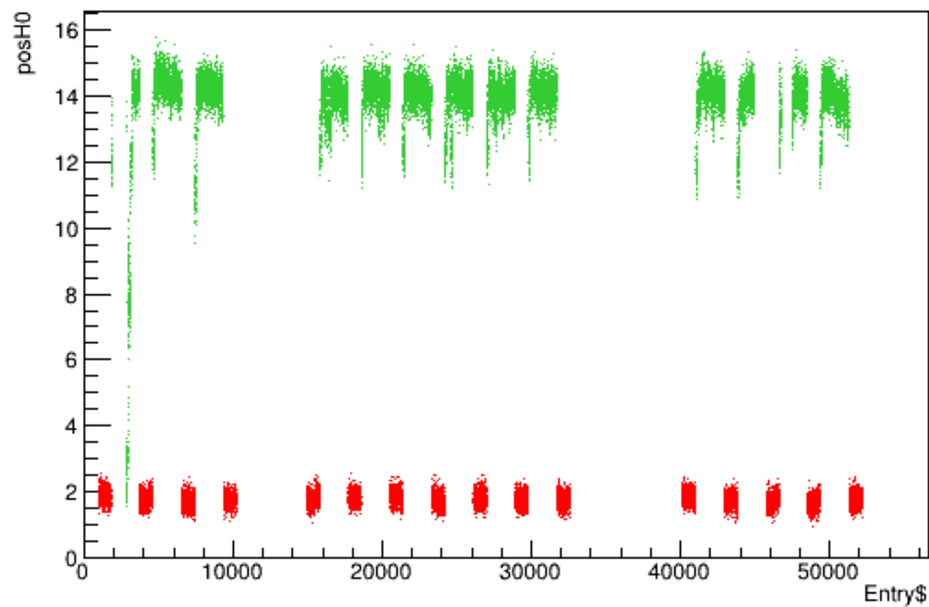
Run 5589 quartetwise, posH0 vs time
