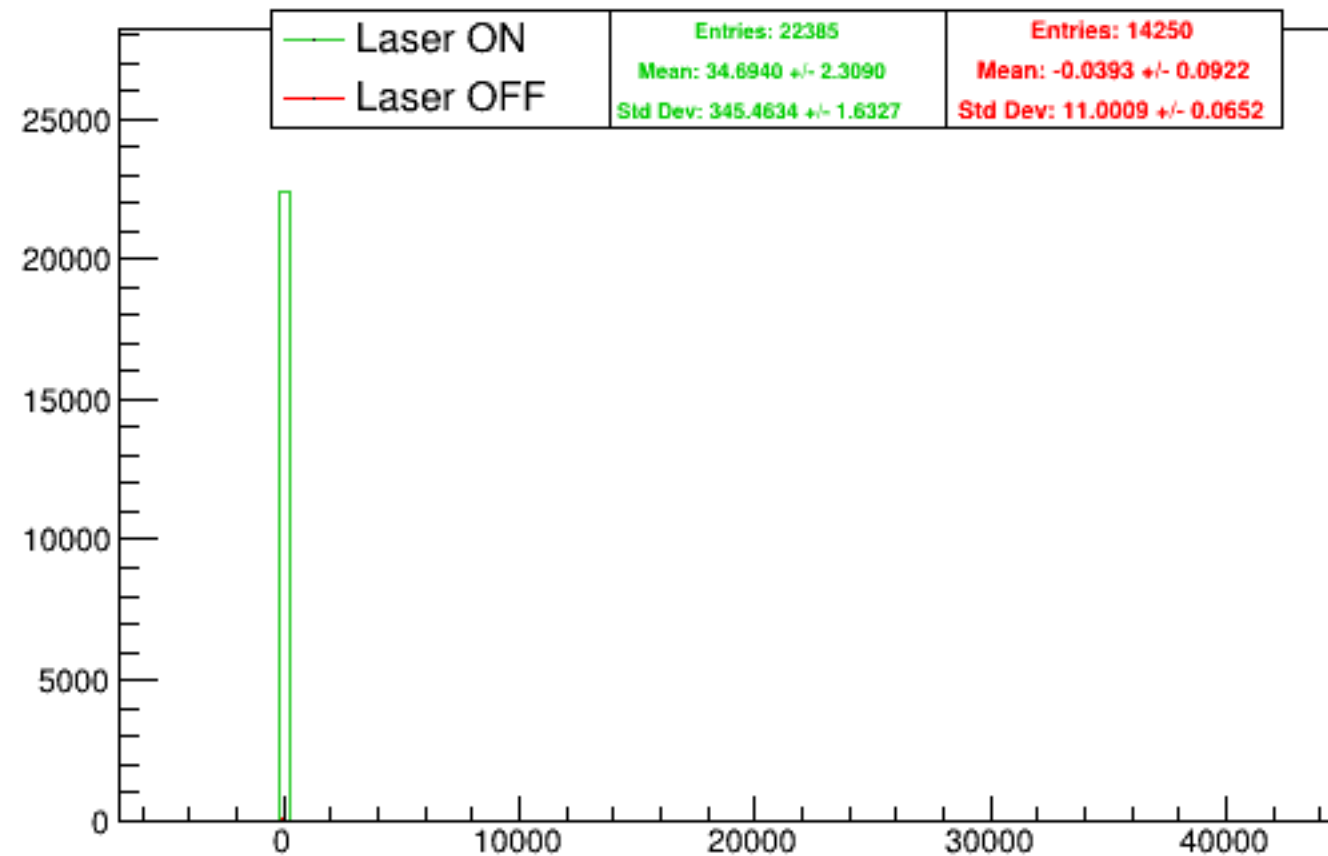
Run 5589 quartetwise, asym0sub: Beam ON
