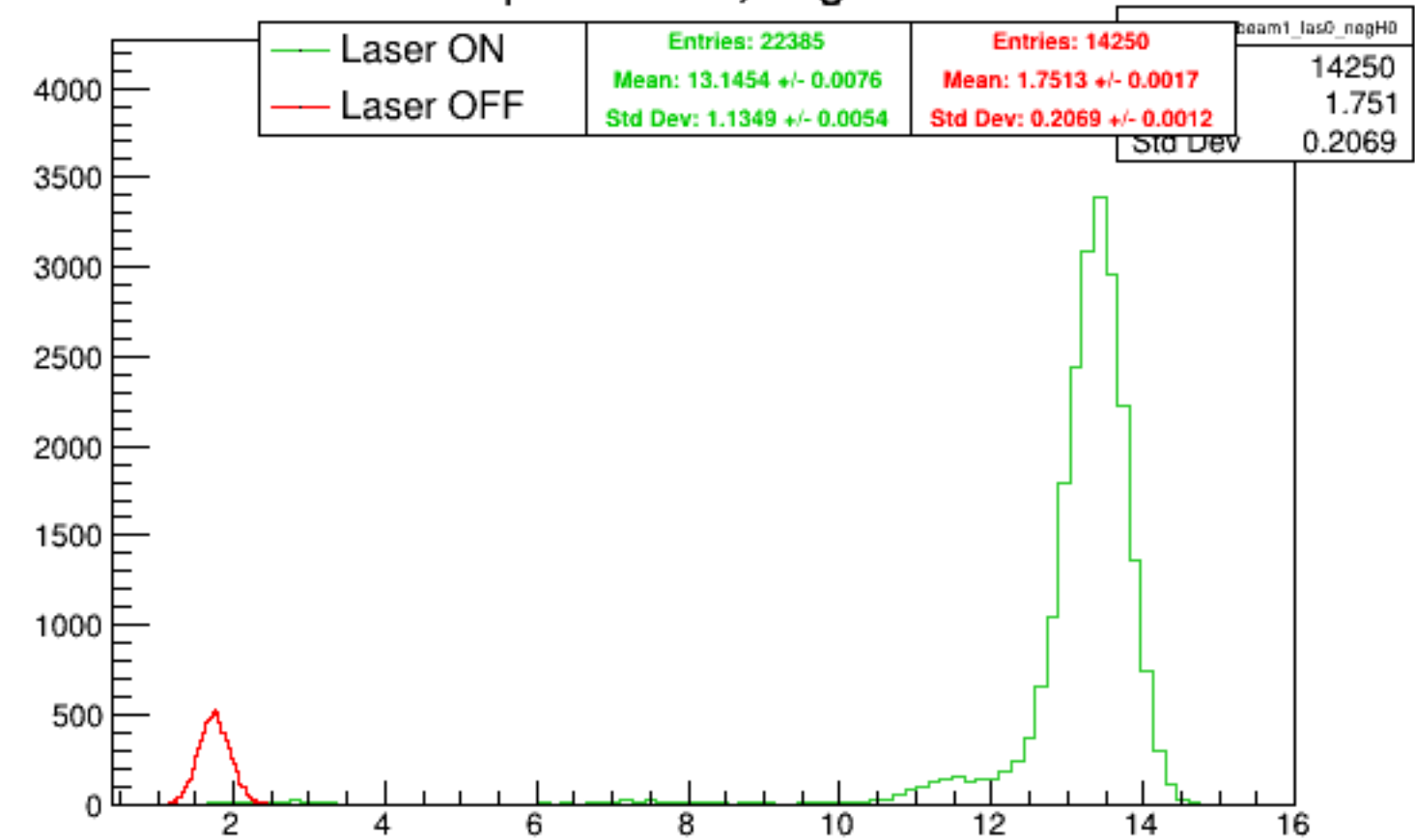
Run 5589 quartetwise, negH0: Beam ON
