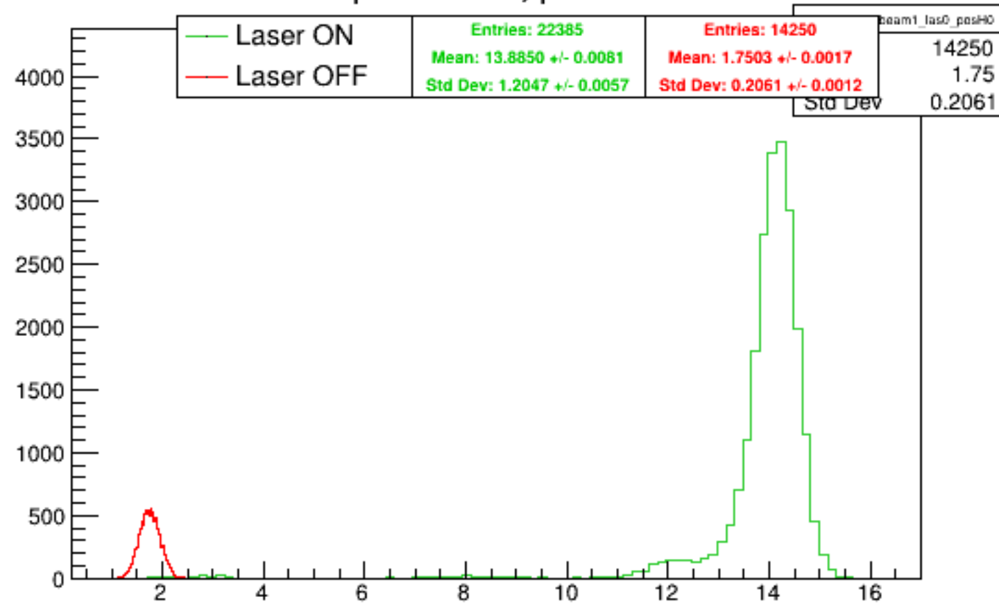
Run 5589 quartetwise, posH0: Beam ON
