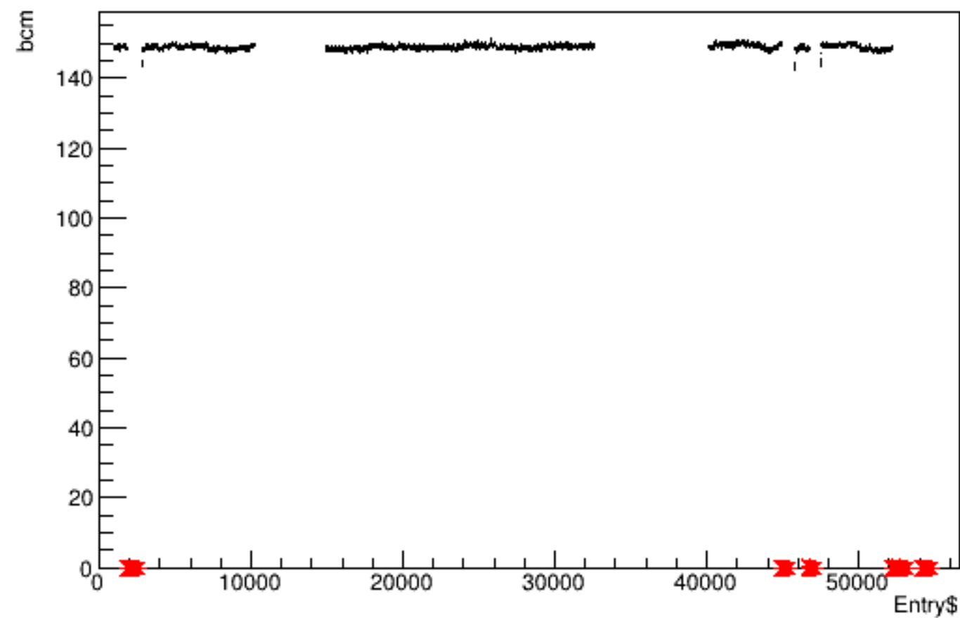
Run 5589 quartetwise, bcm vs time
