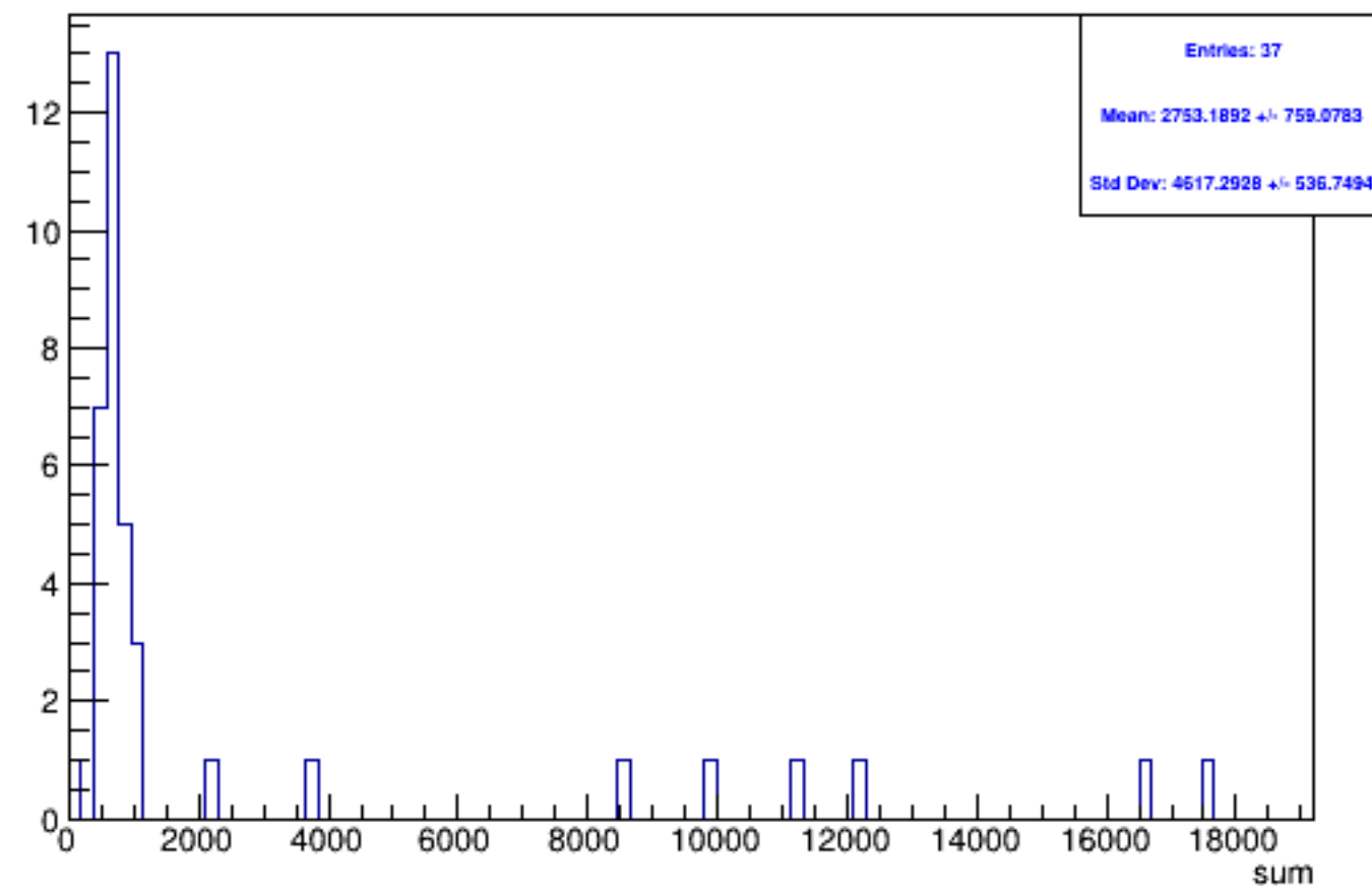
Run 5590 triggerwise, sums: Beam OFF
