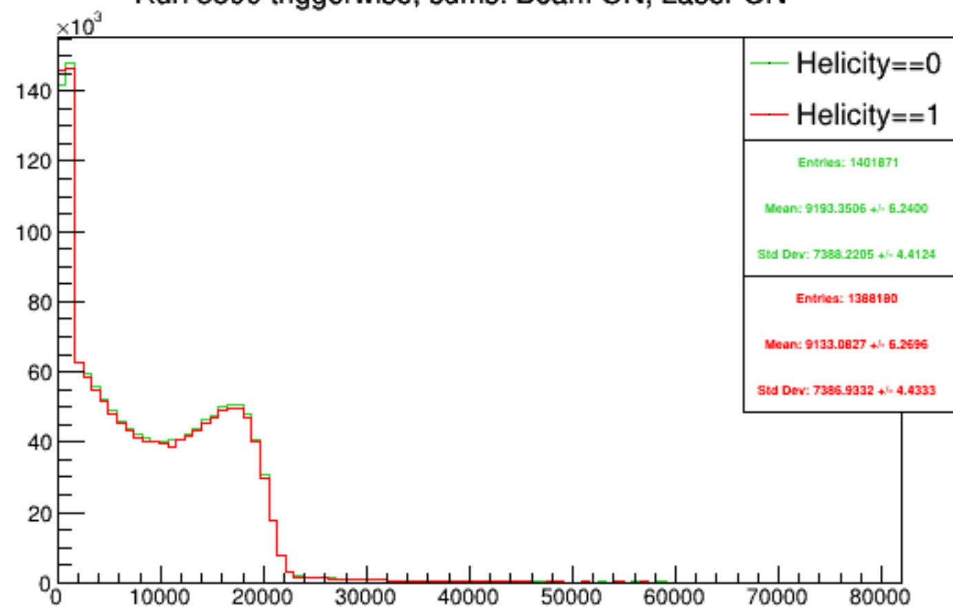
Run 5590 triggerwise, sums: Beam ON, Laser ON
