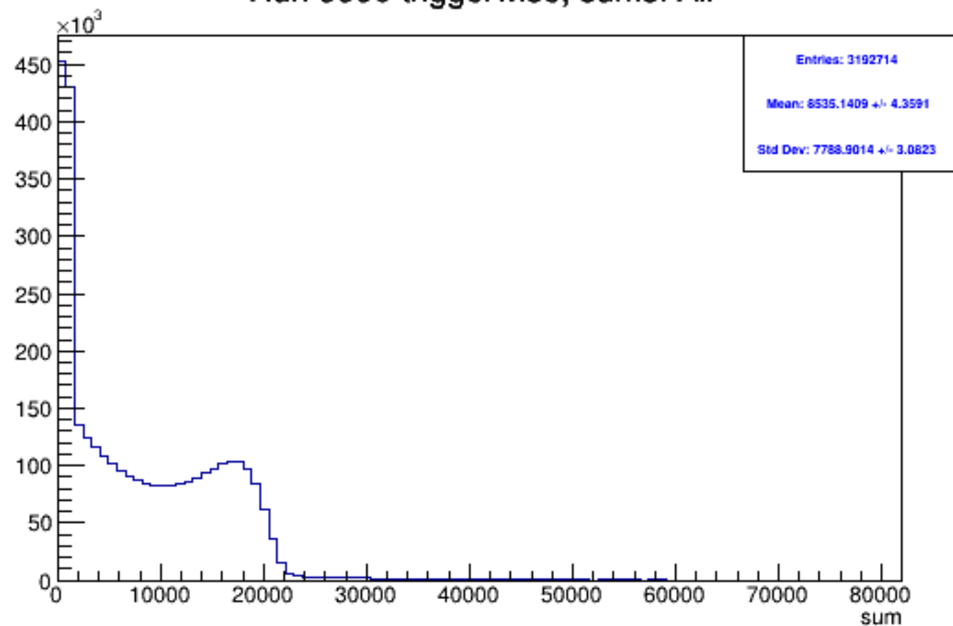
Run 5590 triggerwise, sums: All
