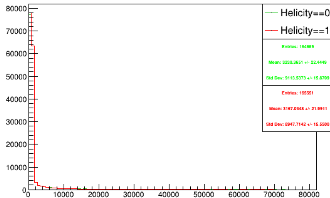
Run 5590 triggerwise, sums: Beam ON, Laser OFF
