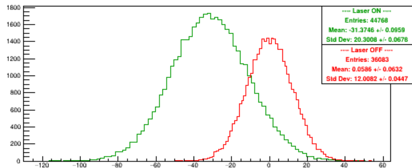
Run 5596 quartetwise, Asyms0
