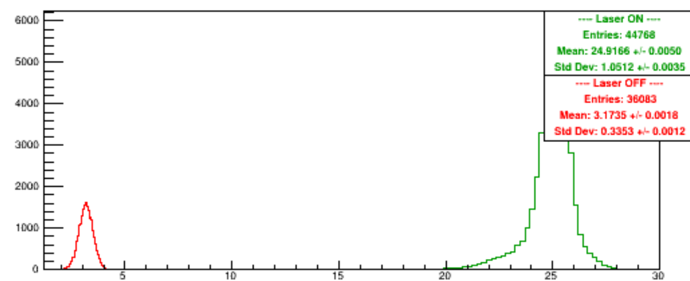
Run 5596 quartetwise, Sums0
