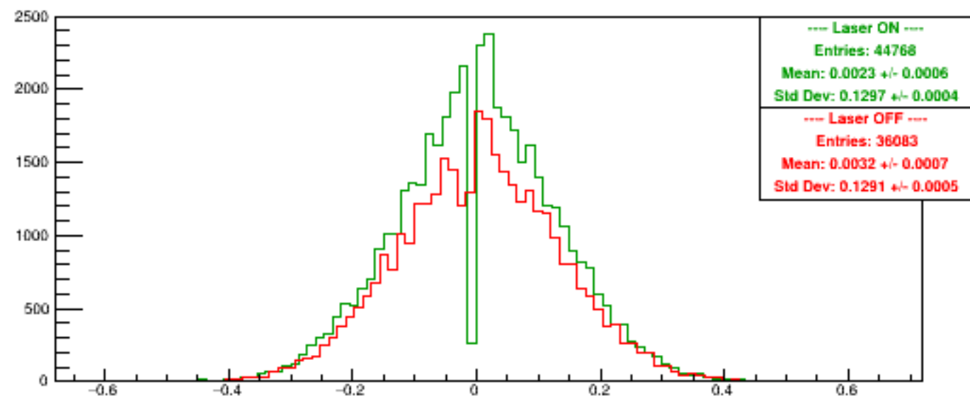
Run 5596 quartetwise, Asyms DSbg1
