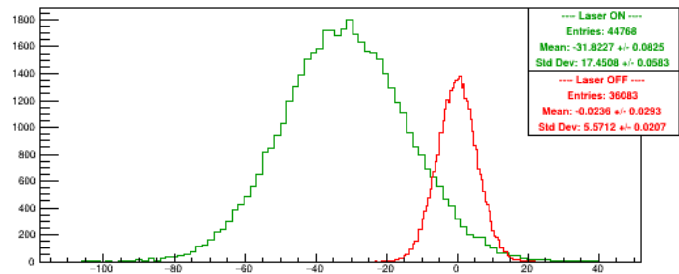
Run 5596 quartetwise, Asyms4
