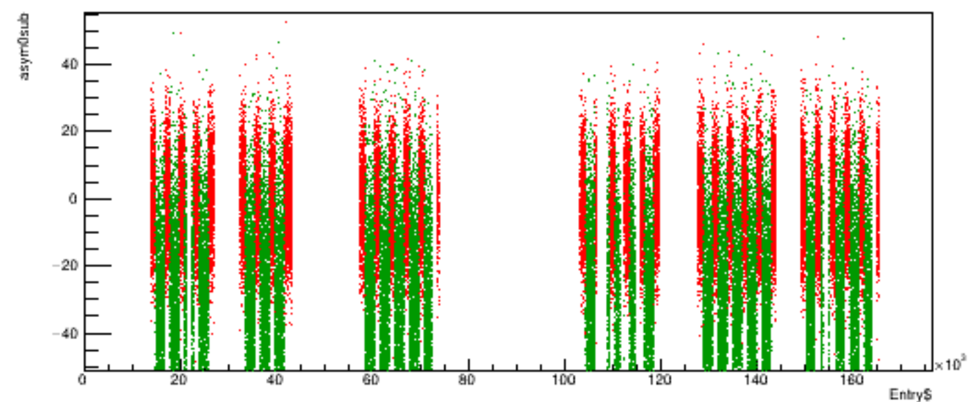
Run 5596 quartetwise, asym0sub vs time
