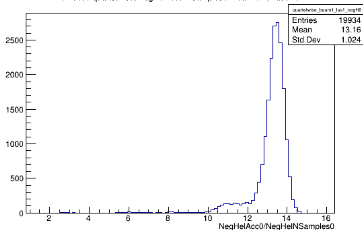
Run 5598 quartetwise, NegHelAcc0/NSamples0: Beam ON, Laser ON
