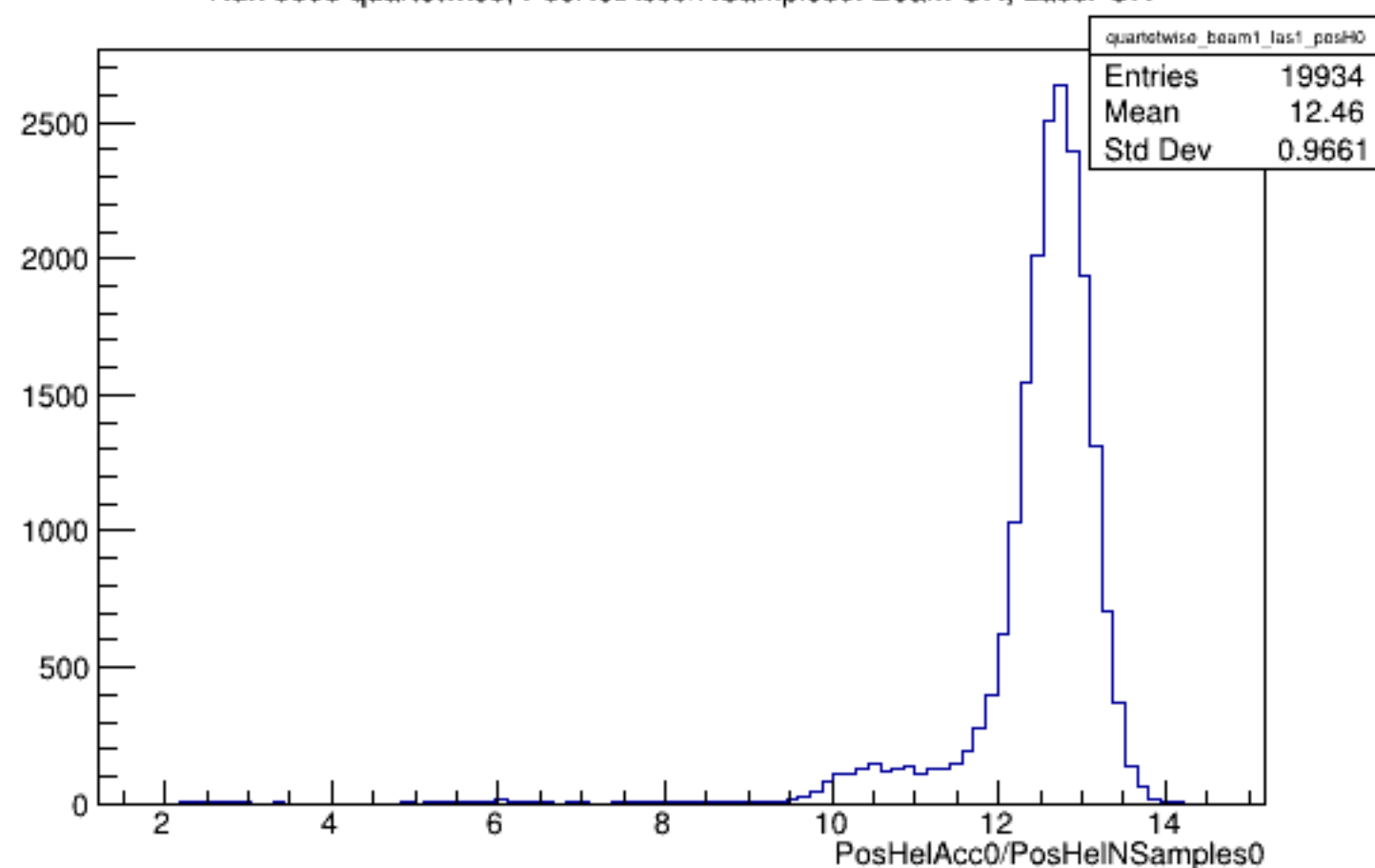
Run 5598 quartetwise, PosHelAcc0/NSamples0: Beam ON, Laser ON
