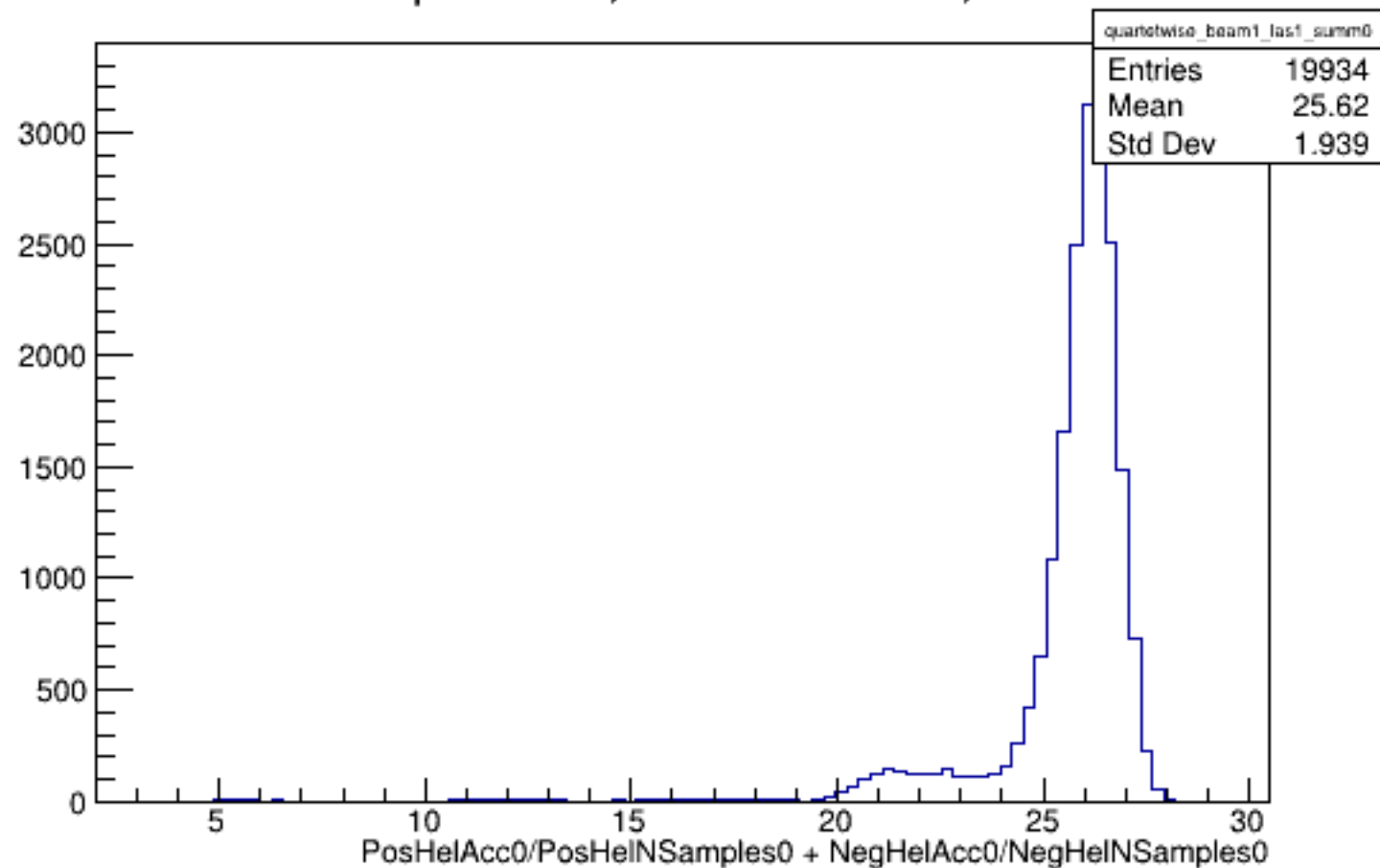
Run 5598 quartetwise, Sums0: Beam ON, Laser ON
