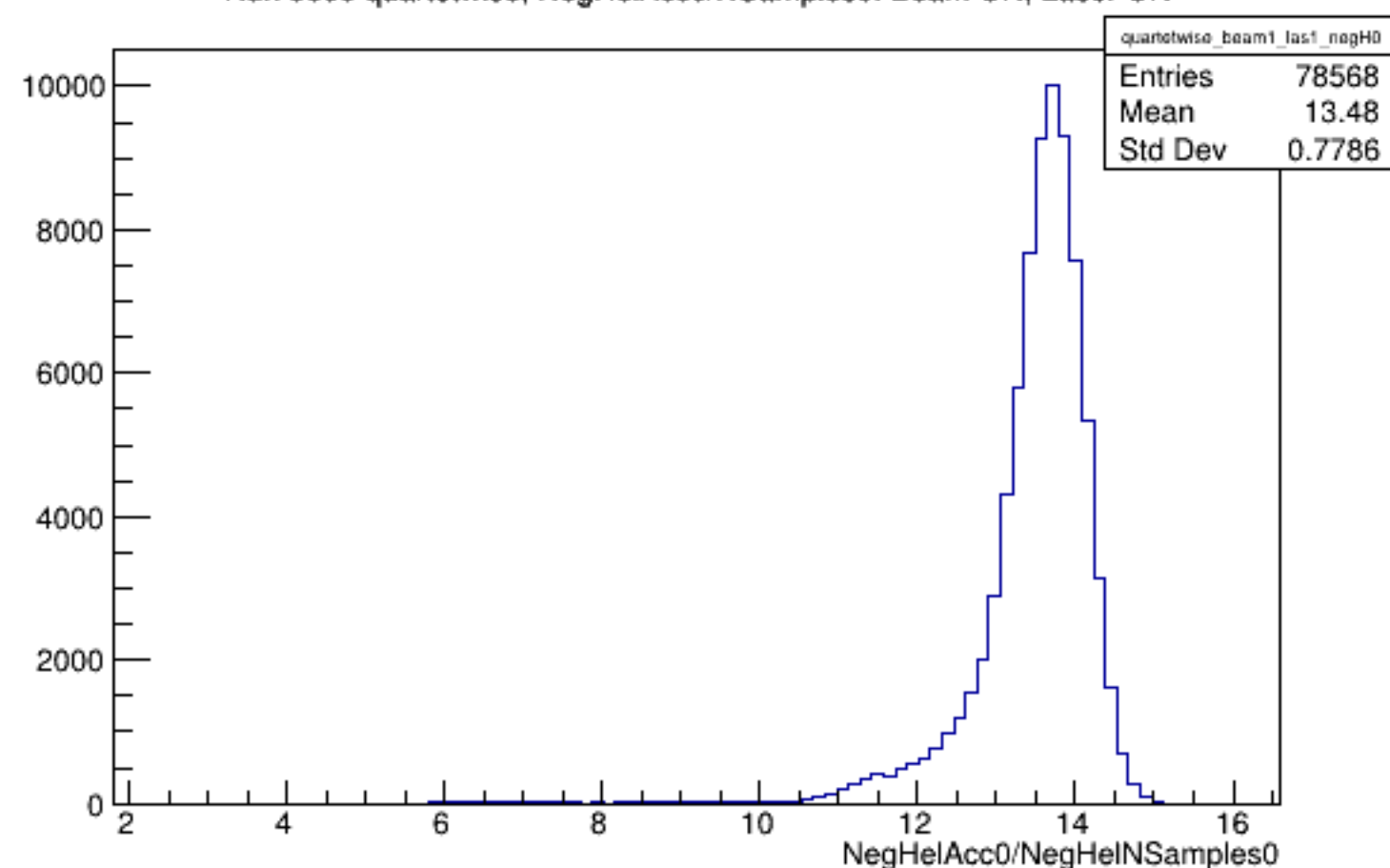
Run 5609 quartetwise, NegHelAcc0/NSamples0: Beam ON, Laser ON
