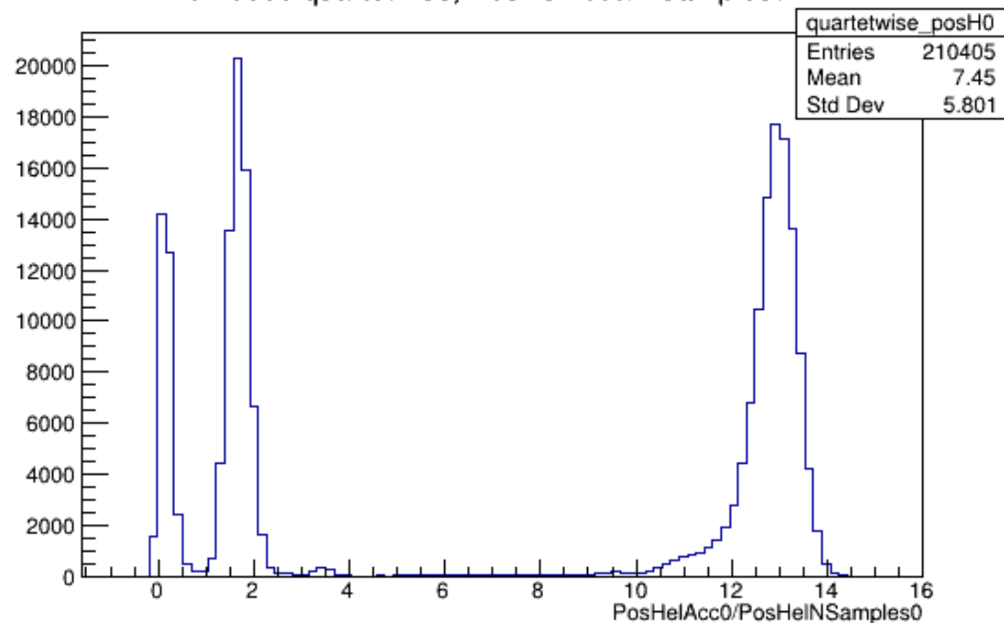
Run 5609 quartetwise, PosHelAcc0/NSamples0: All
