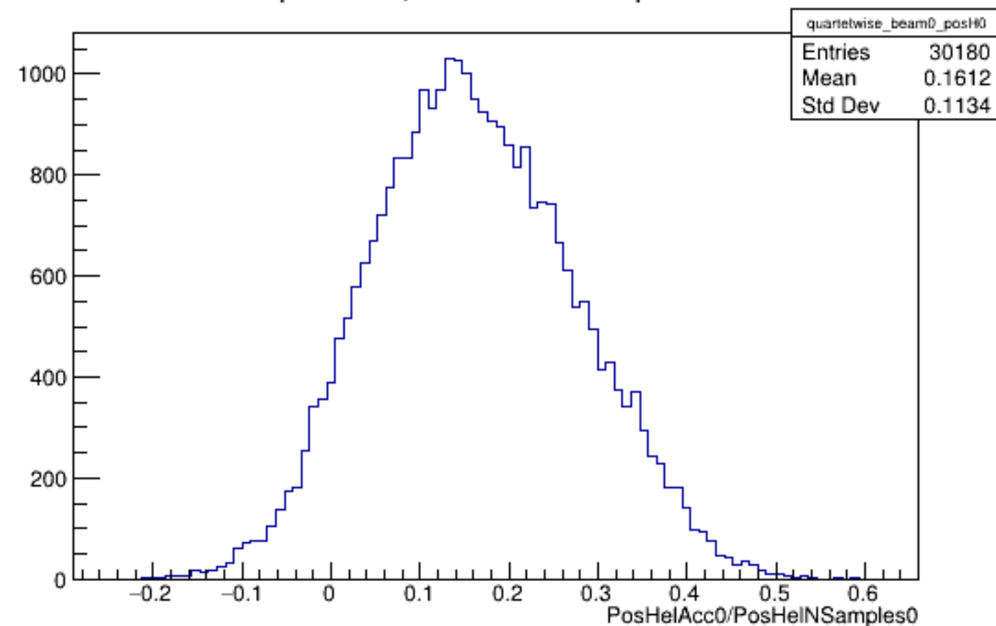
Run 5609 quartetwise, PosHelAcc0/NSamples0: Beam OFF
