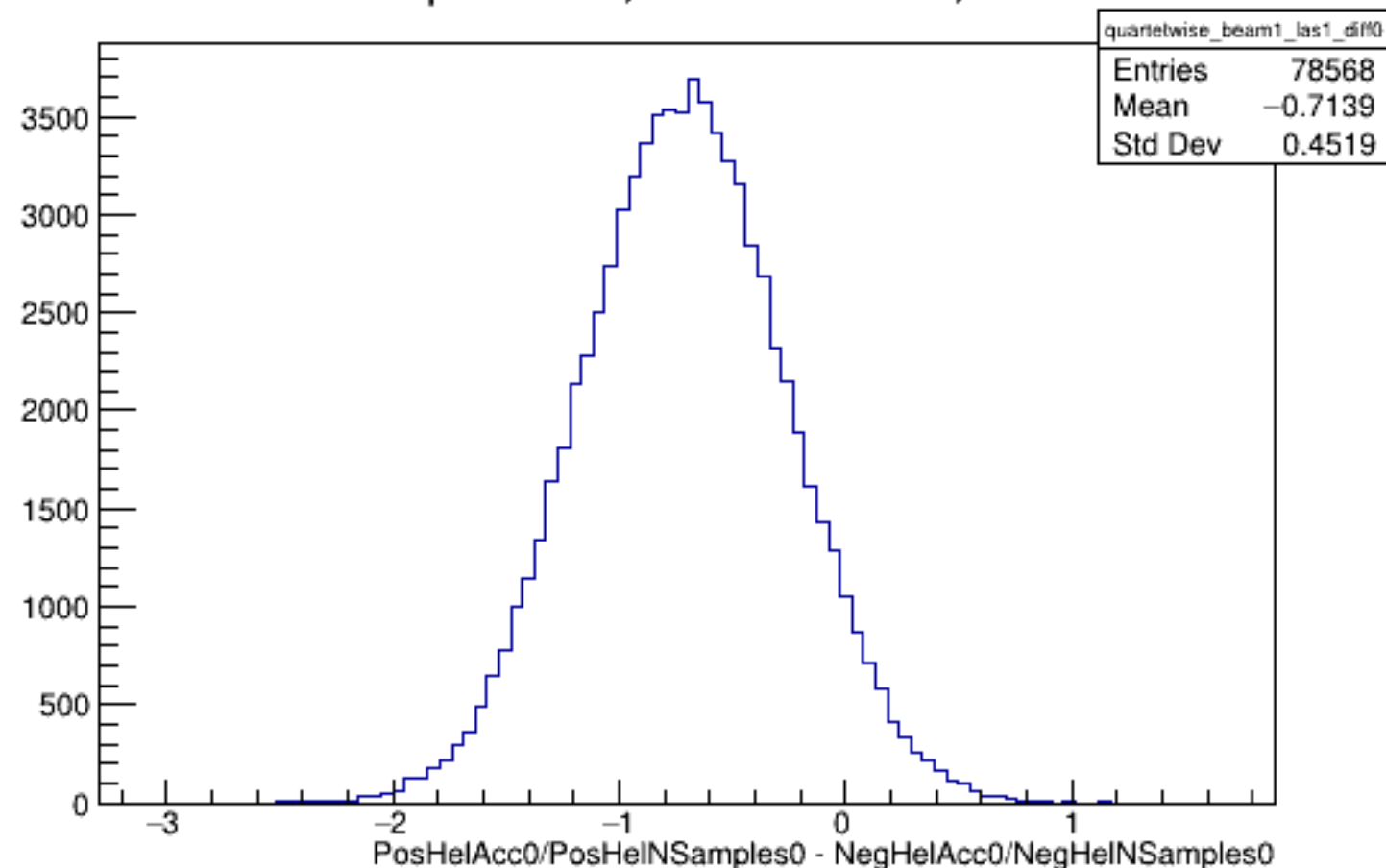
Run 5609 quartetwise, Diffs0: Beam ON, Laser ON
