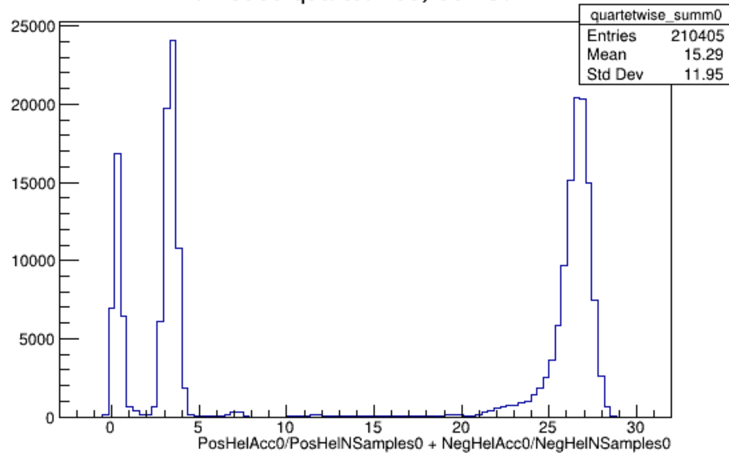
Run 5609 quartetwise, Sums0: All
