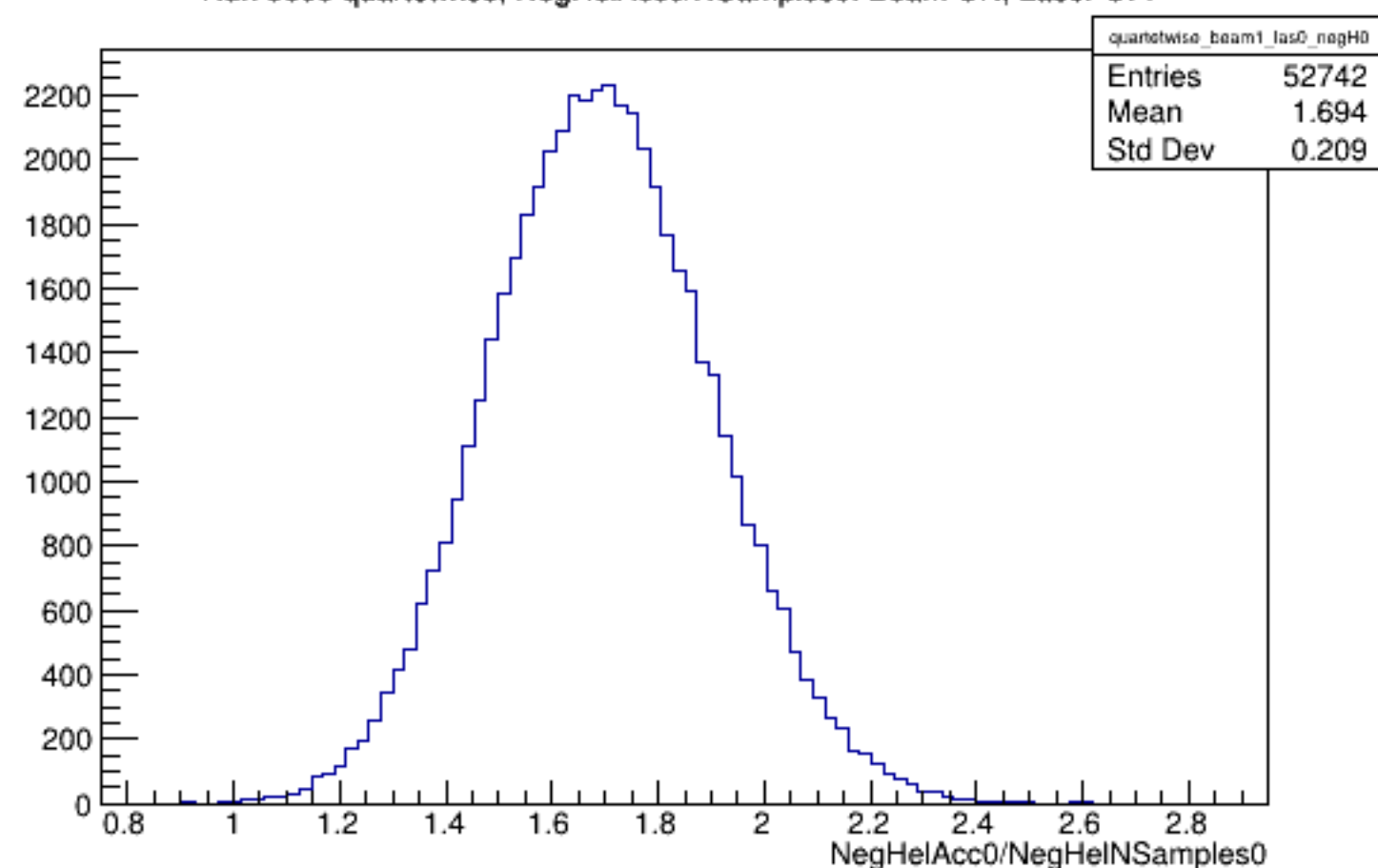
Run 5609 quartetwise, NegHelAcc0/NSamples0: Beam ON, Laser OFF
