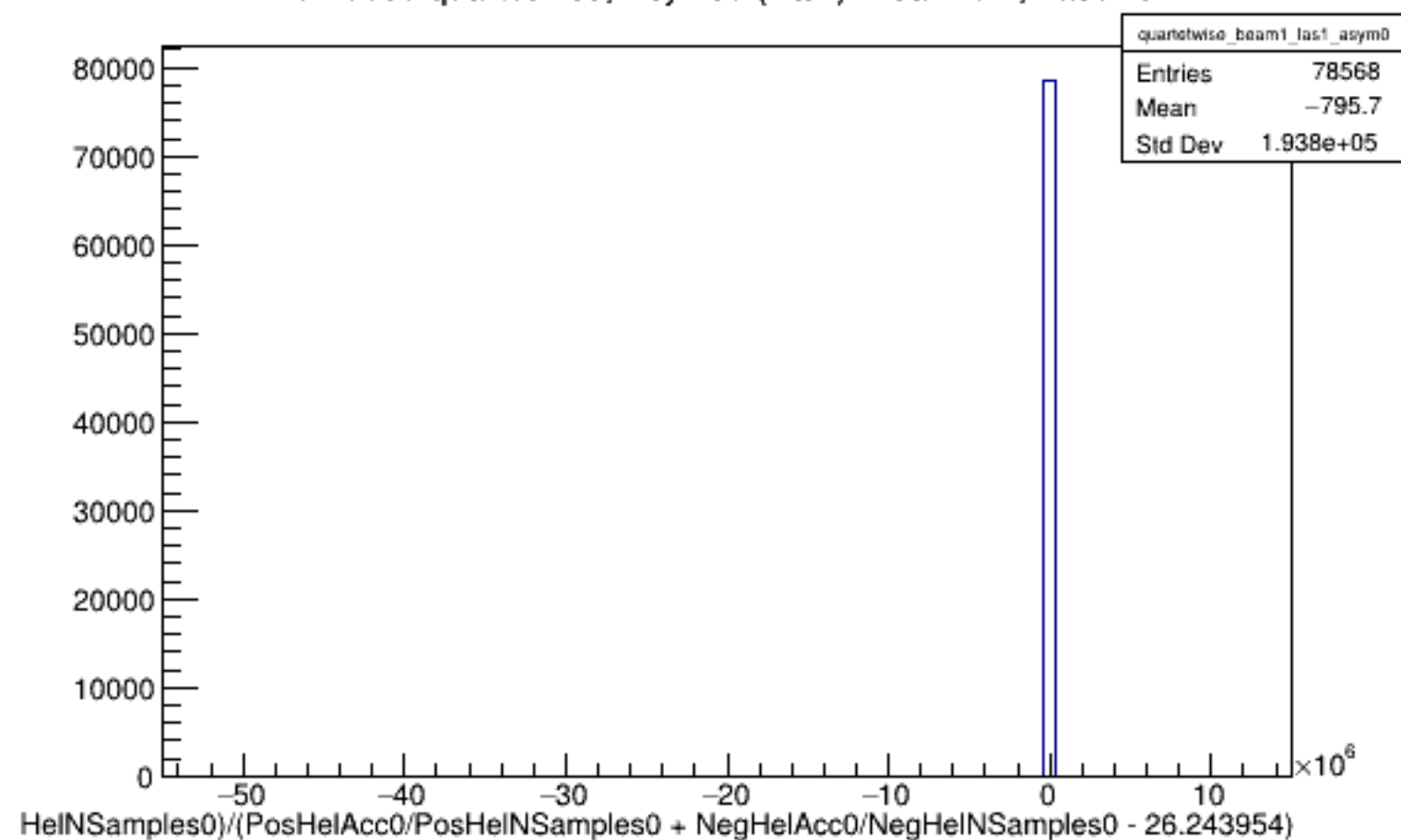
Run 5609 quartetwise, Asyms0 (Raw): Beam ON, Laser ON
