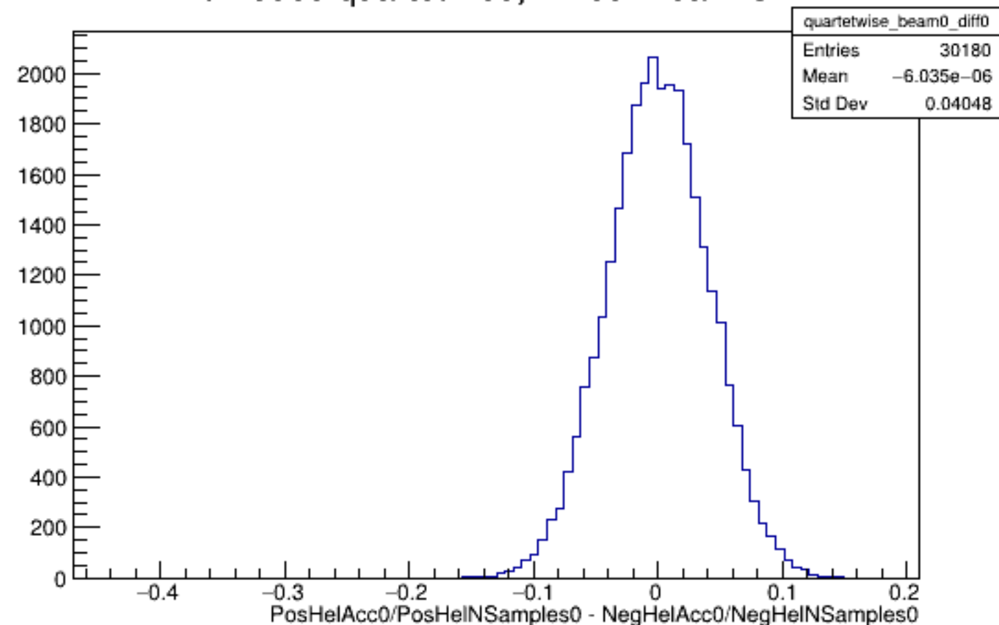
Run 5609 quartetwise, Diffs0: Beam OFF
