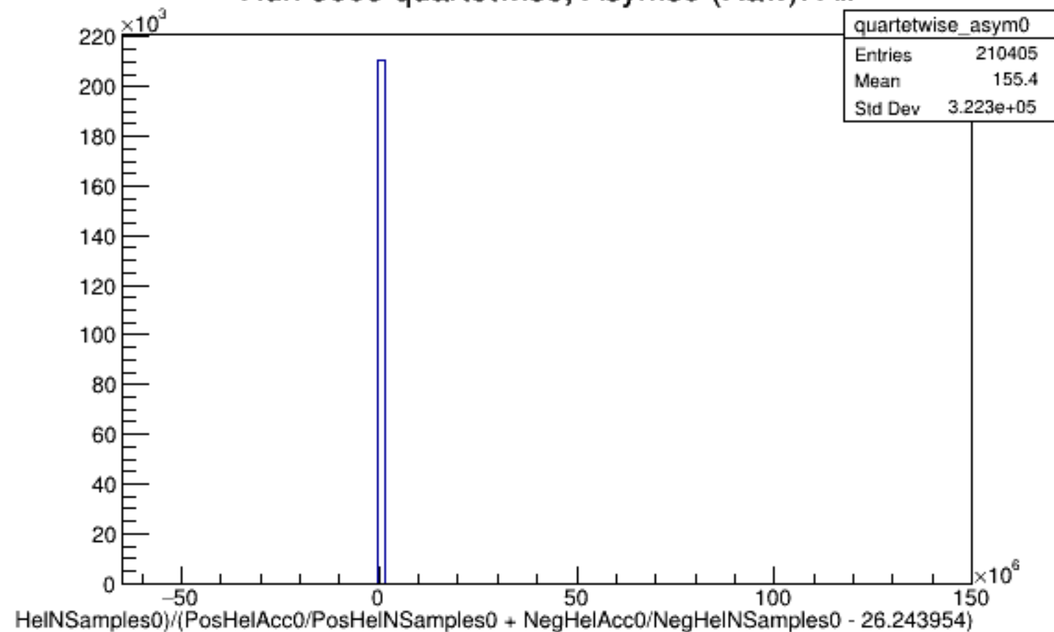
Run 5609 quartetwise, Asyms0 (Raw): All
