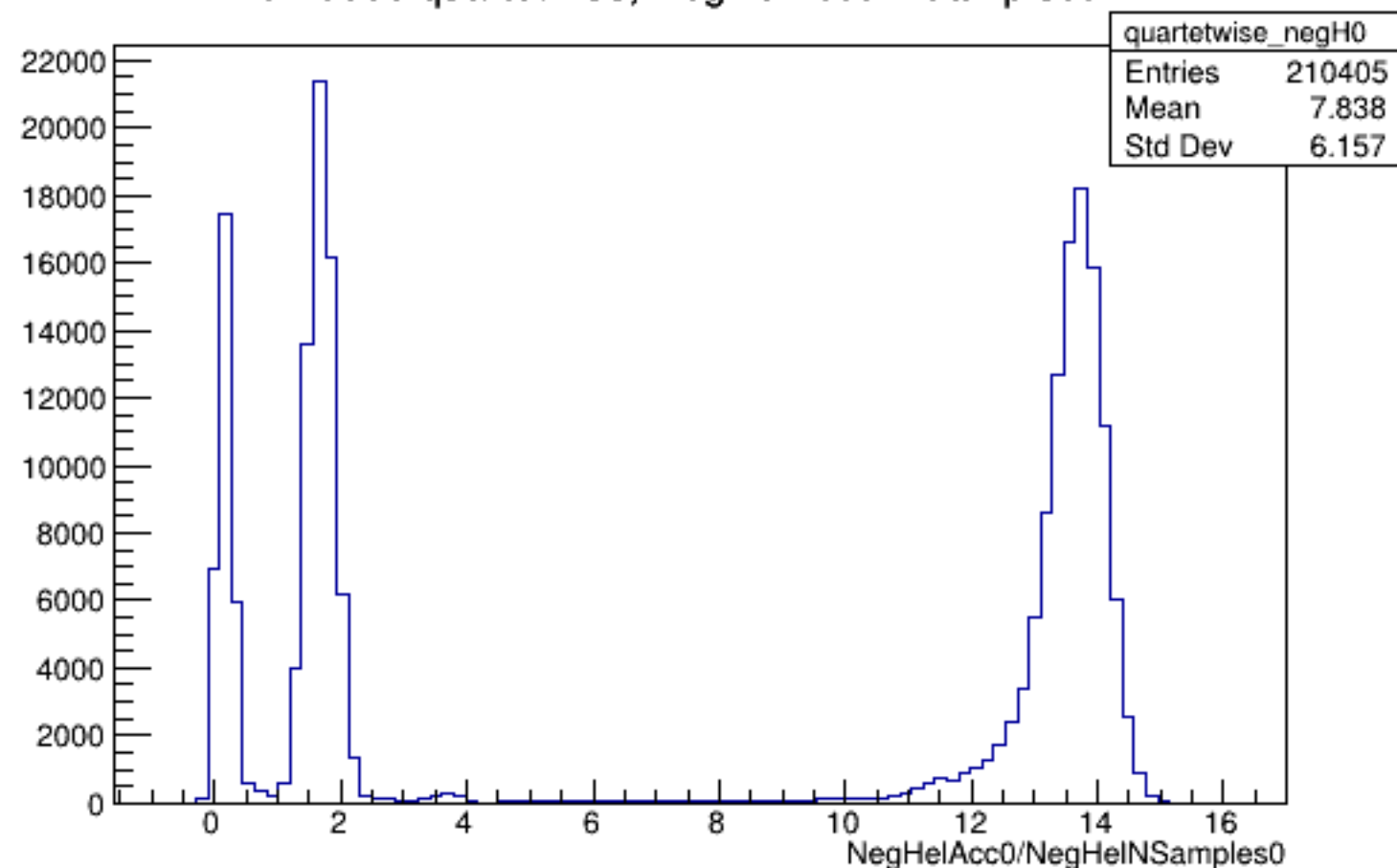
Run 5609 quartetwise, NegHelAcc0/NSamples0: All
