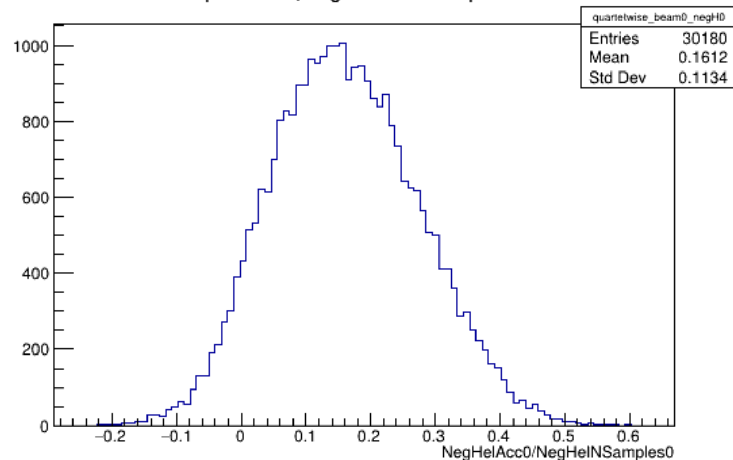
Run 5609 quartetwise, NegHelAcc0/NSamples0: Beam OFF
