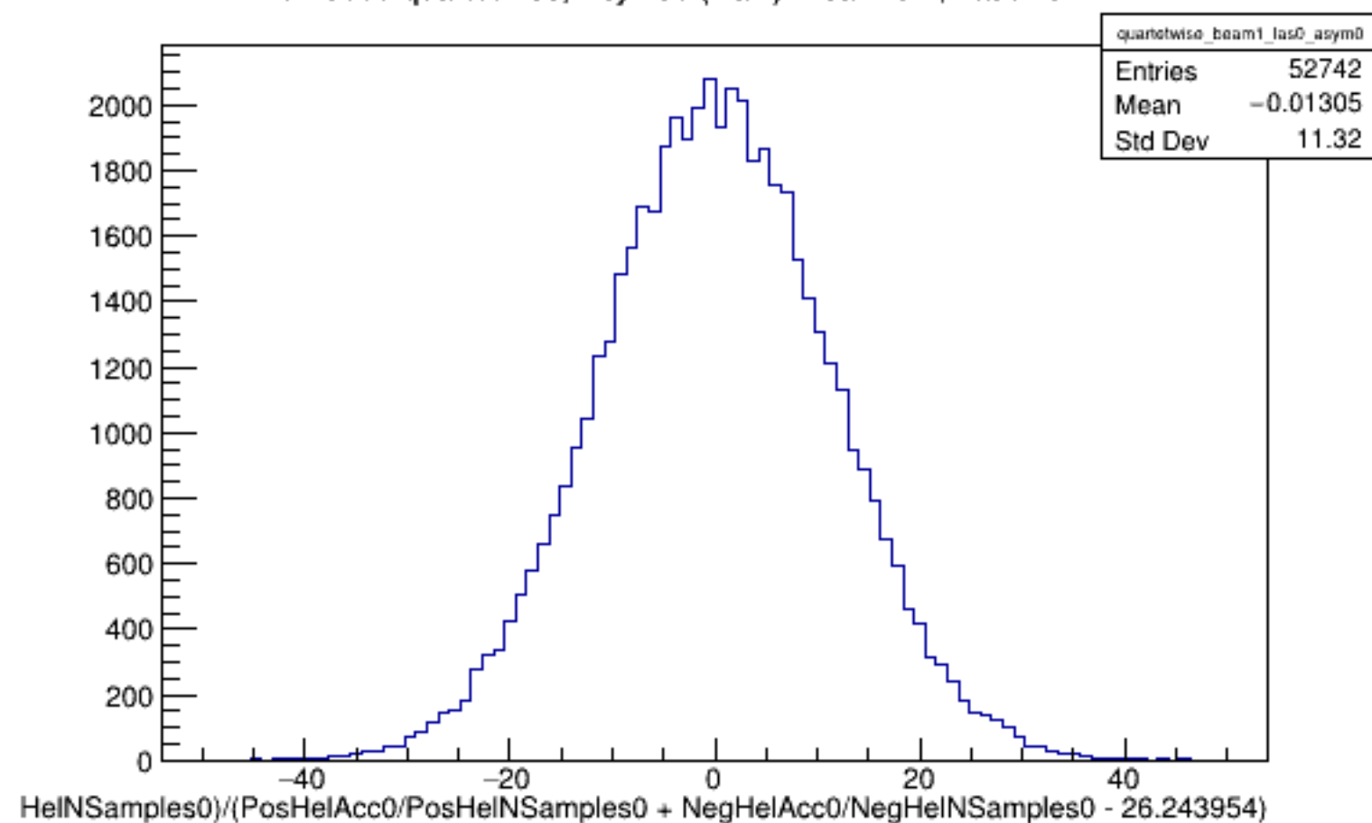
Run 5609 quartetwise, Asyms0 (Raw): Beam ON, Laser OFF
