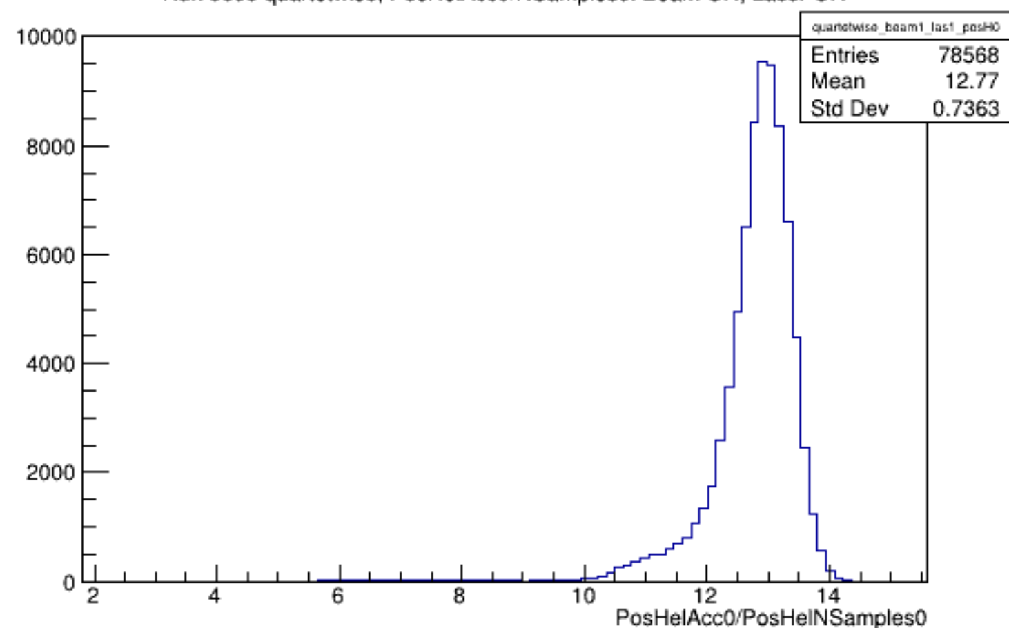
Run 5609 quartetwise, PosHelAcc0/NSamples0: Beam ON, Laser ON
