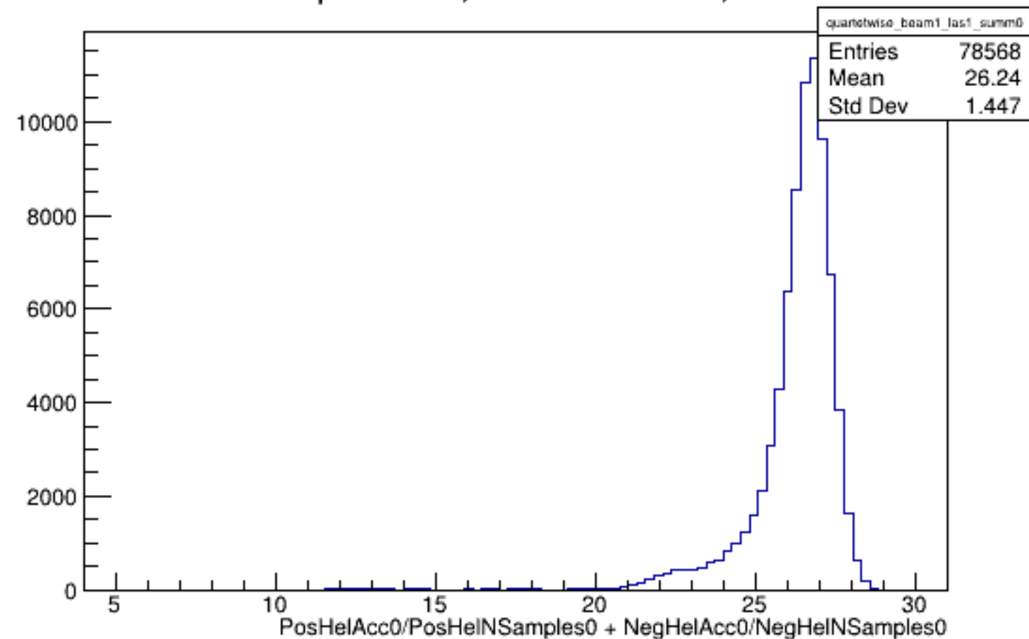
Run 5609 quartetwise, Sums0: Beam ON, Laser ON
