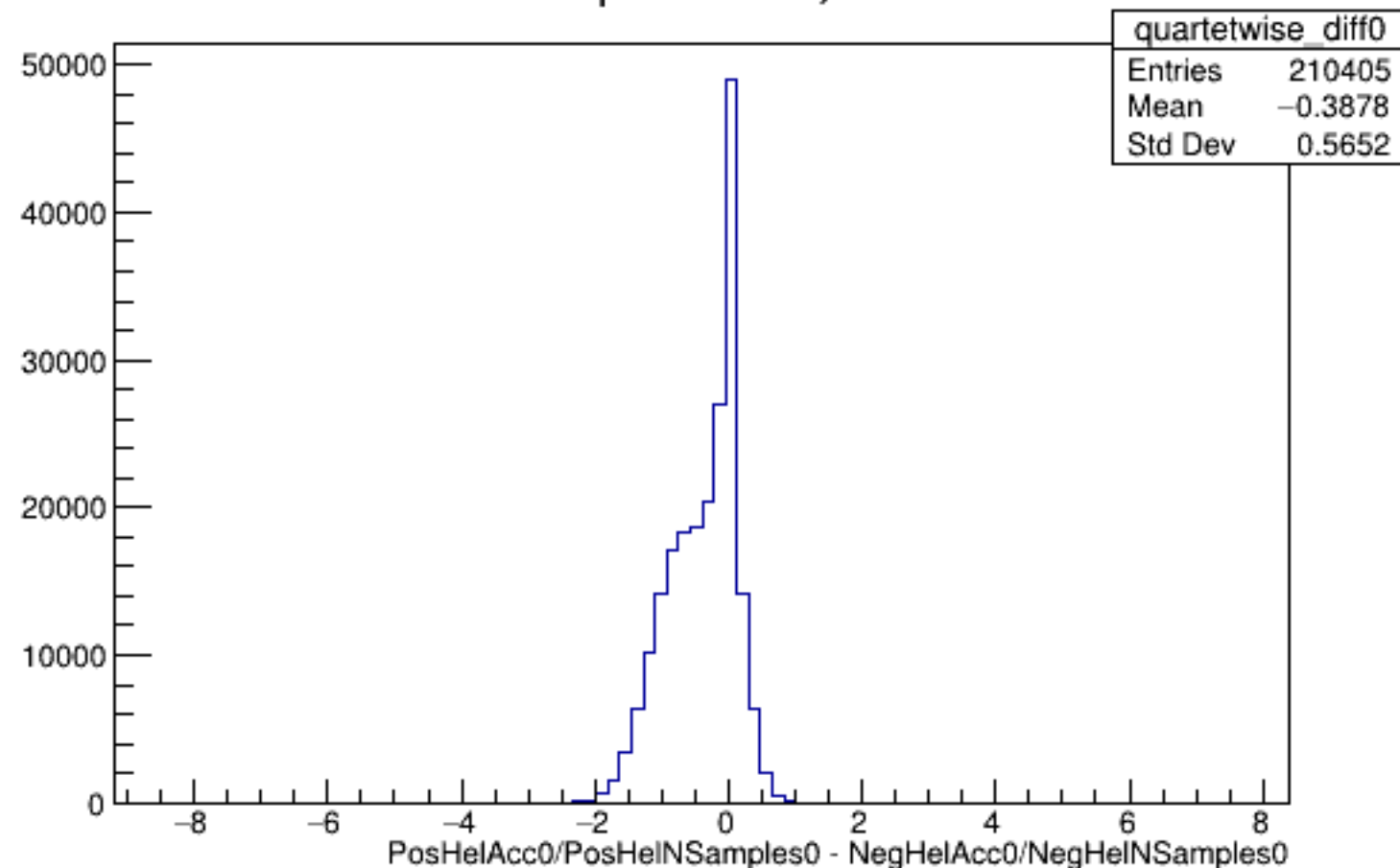
Run 5609 quartetwise, Diffs0: All
