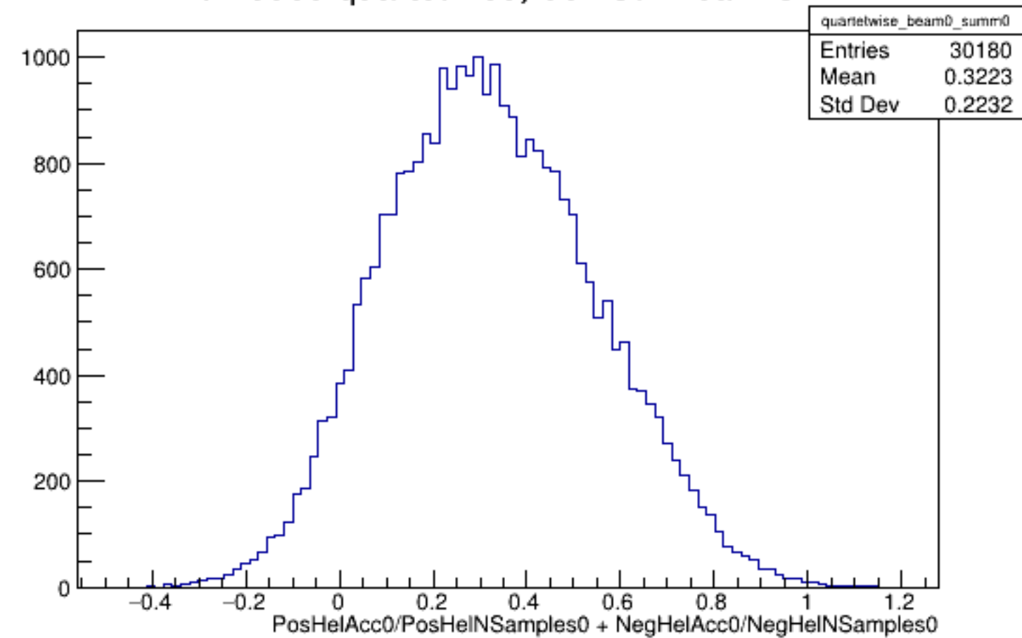
Run 5609 quartetwise, Sums0: Beam OFF
