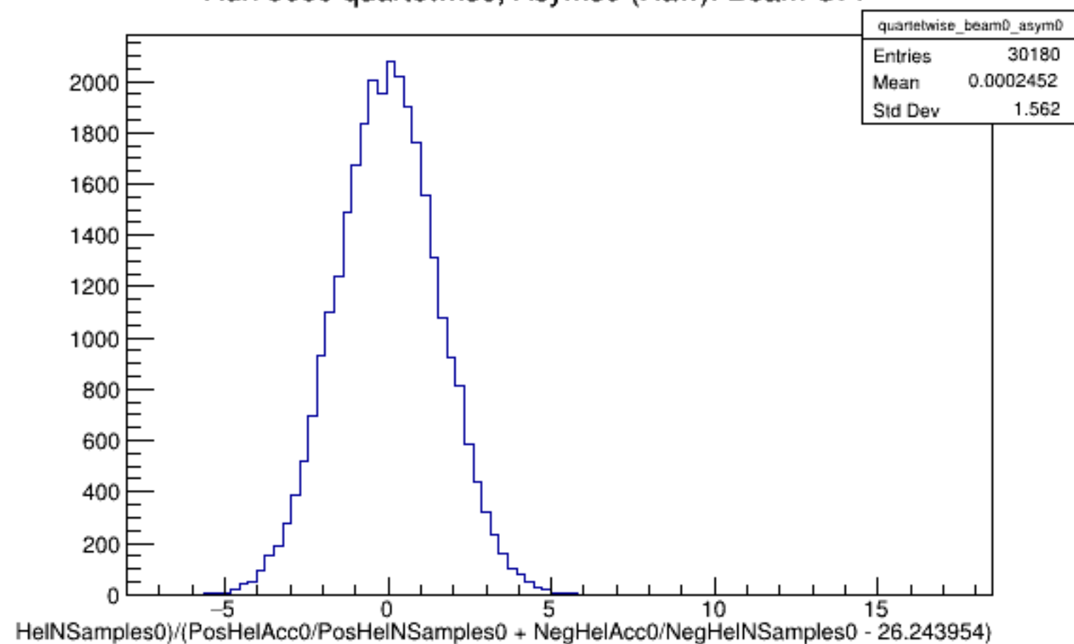
Run 5609 quartetwise, Asyms0 (Raw): Beam OFF
