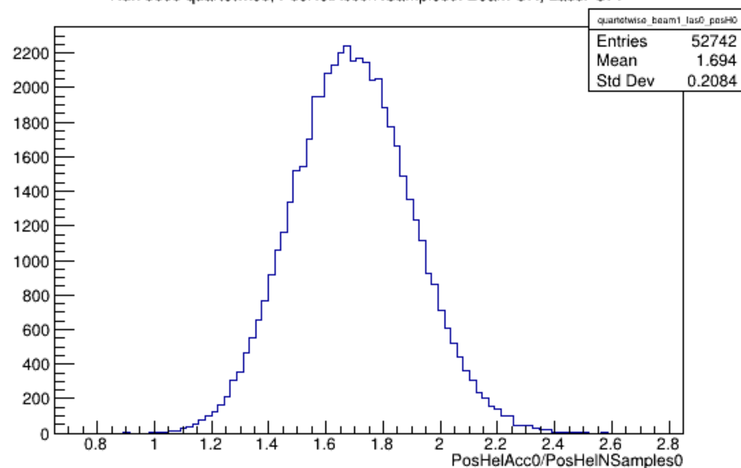
Run 5609 quartetwise, PosHelAcc0/NSamples0: Beam ON, Laser OFF
