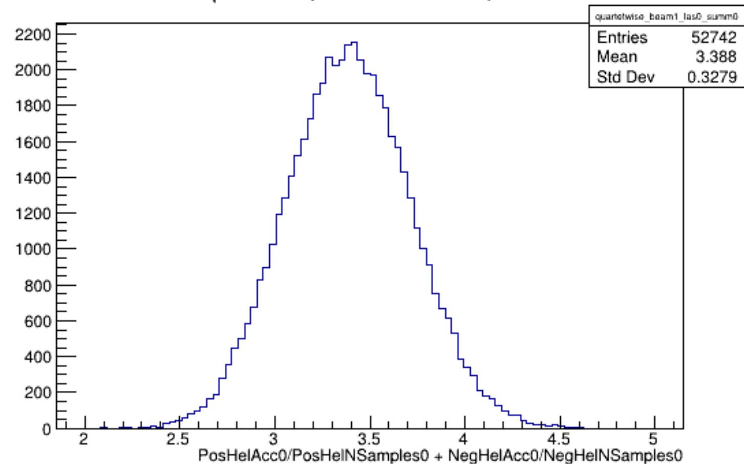
Run 5609 quartetwise, Sums0: Beam ON, Laser OFF
