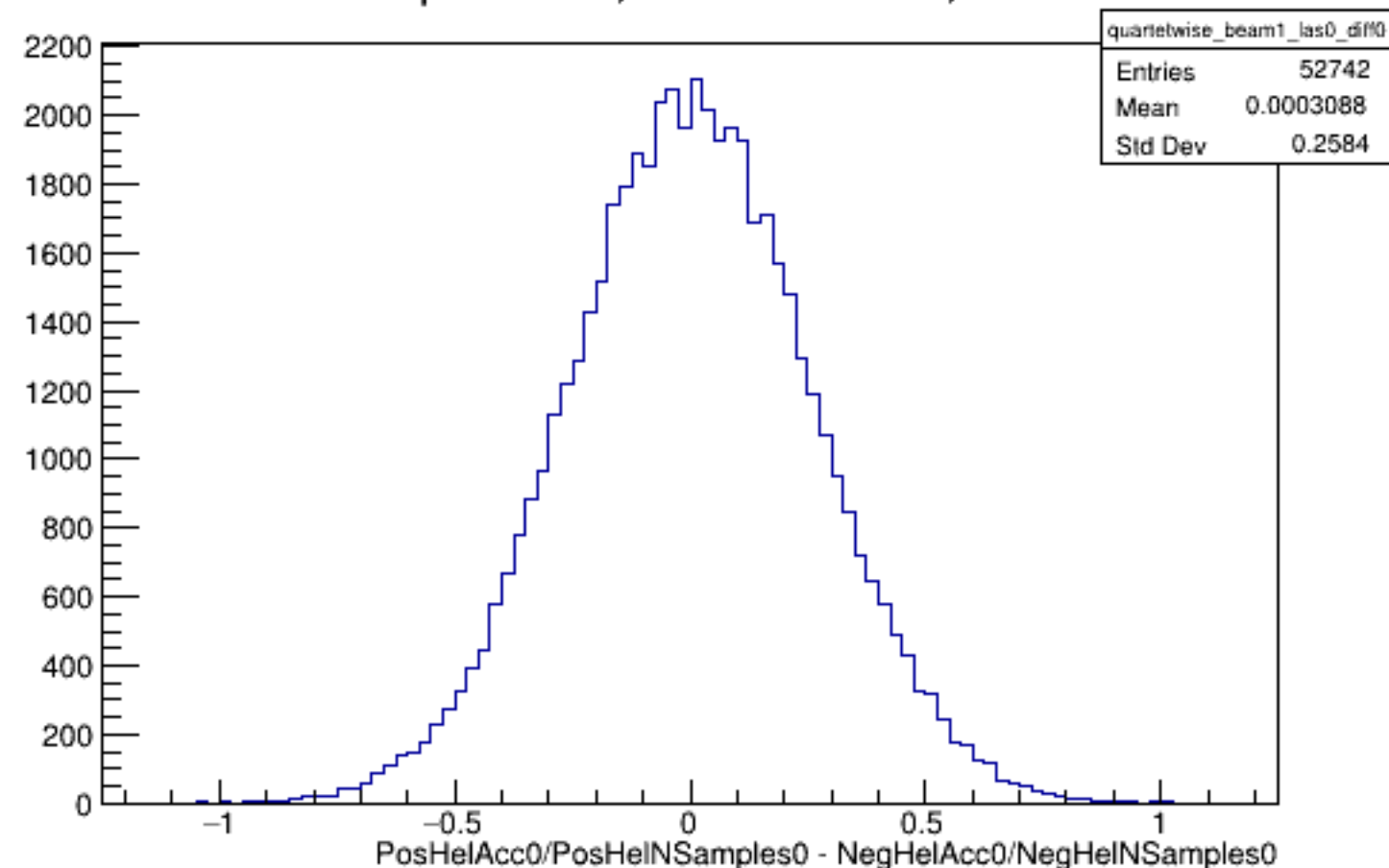
Run 5609 quartetwise, Diffs0: Beam ON, Laser OFF
