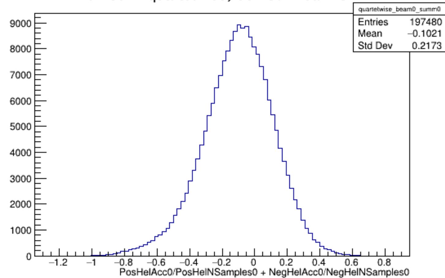
Run 5614 quartetwise, Sums0: Beam OFF
