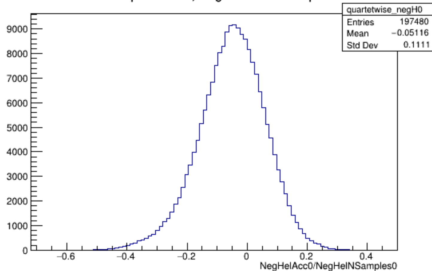
Run 5614 quartetwise, NegHelAcc0/NSamples0: All
