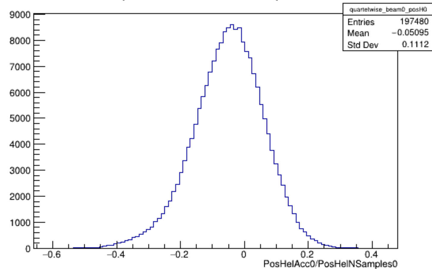
Run 5614 quartetwise, PosHelAcc0/NSamples0: Beam OFF
