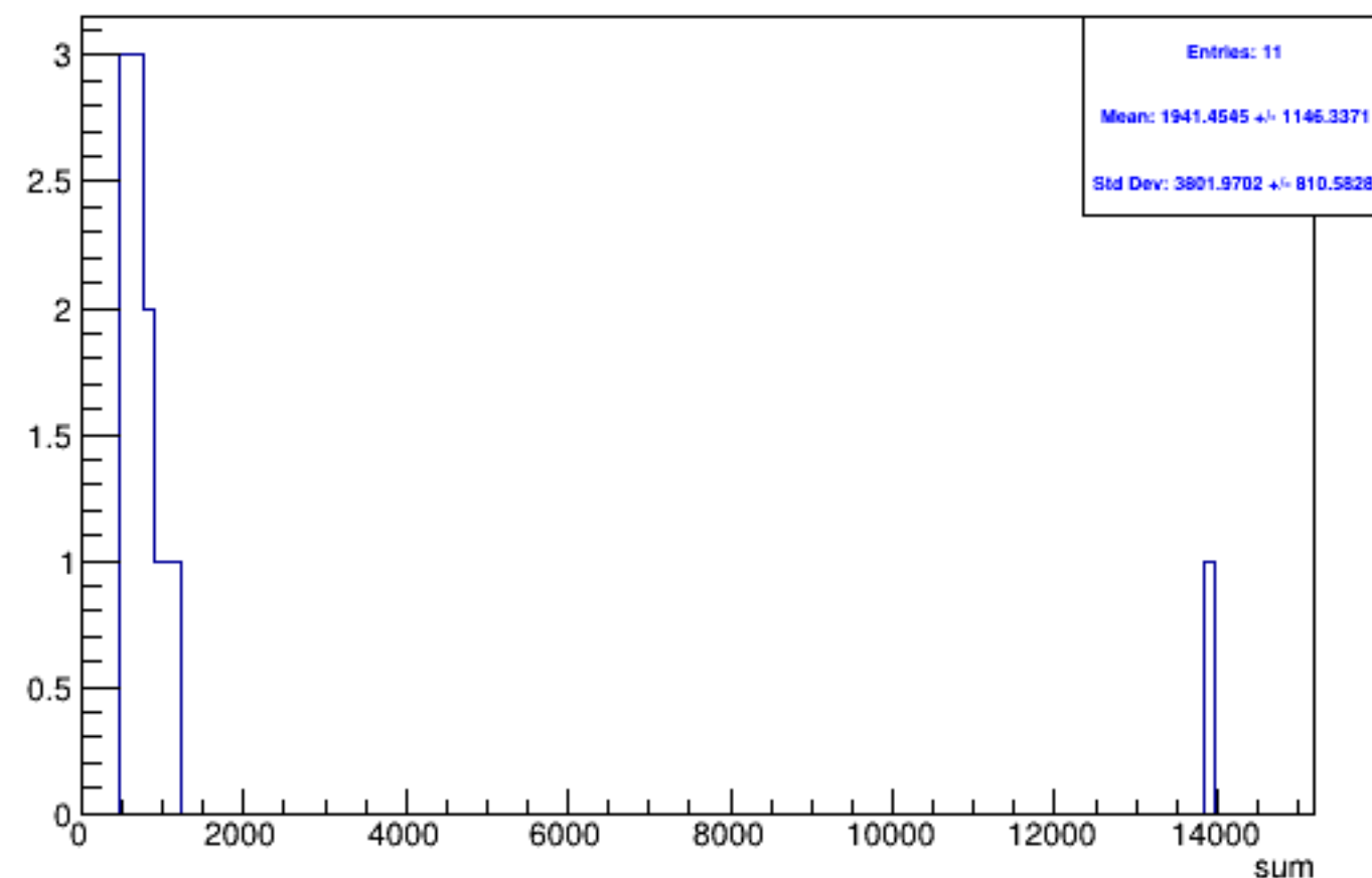
Run 5617 triggerwise, sums: Beam OFF
