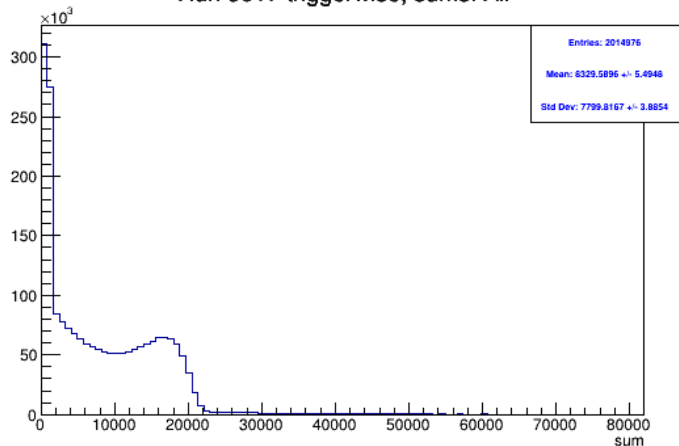
Run 5617 triggerwise, sums: All
