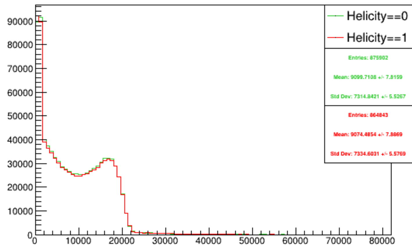
Run 5617 triggerwise, sums: Beam ON, Laser ON
