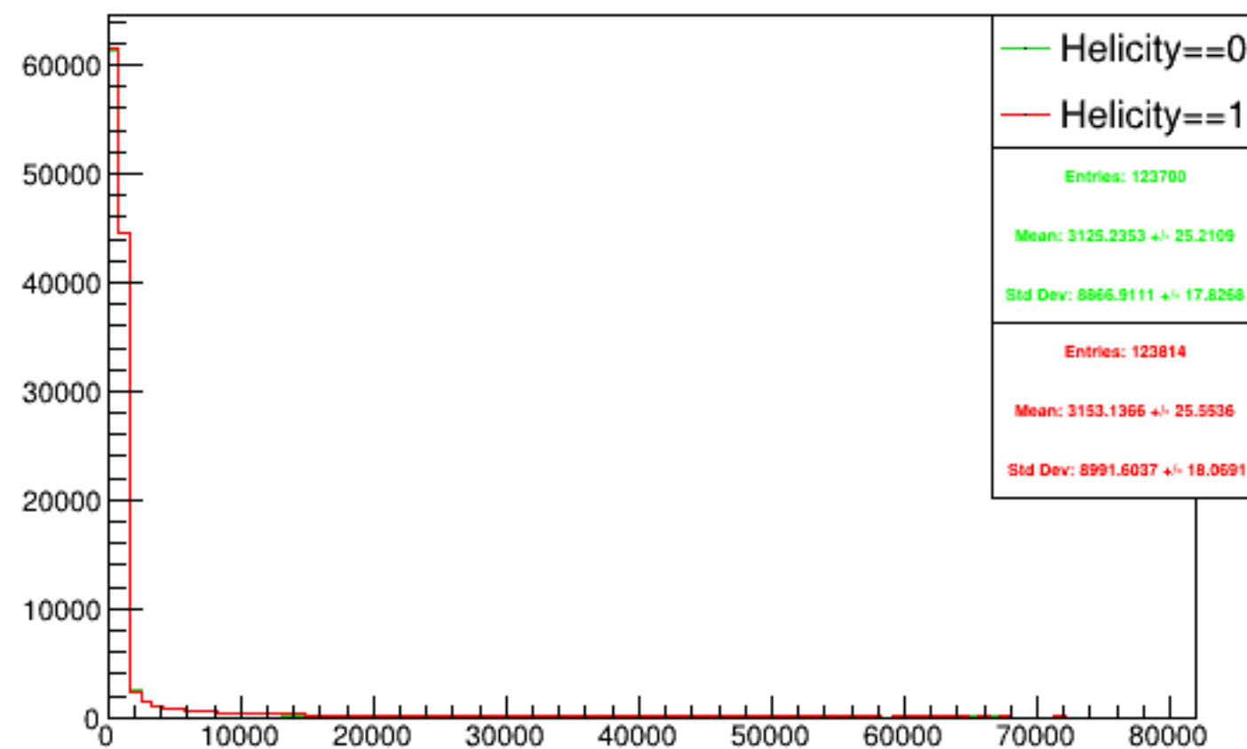
Run 5617 triggerwise, sums: Beam ON, Laser OFF
