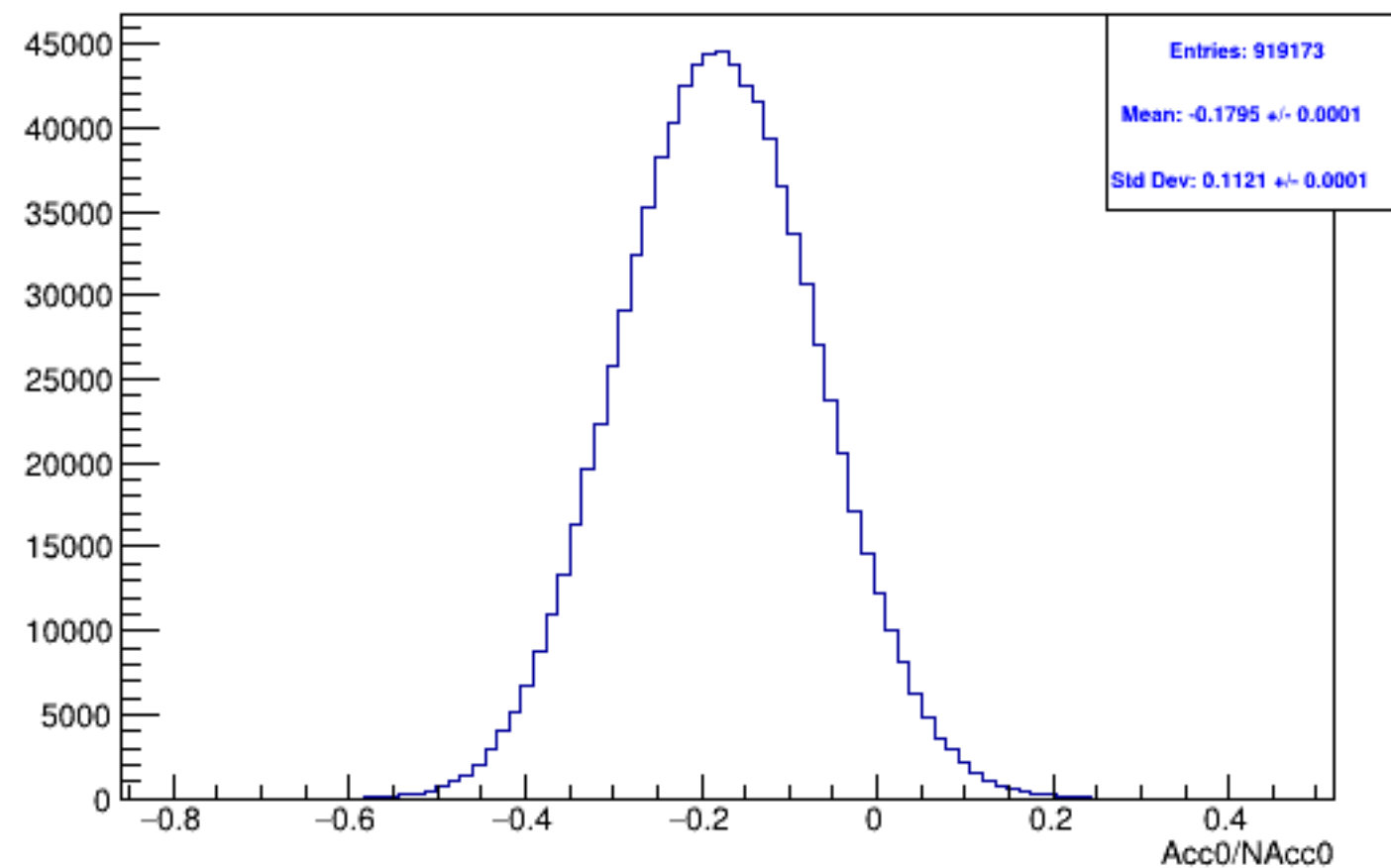
Run 5627 mpwise, acc0: Beam OFF
