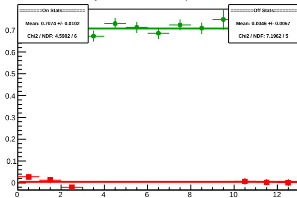
Cycle 5628.1: Multiplet Diffs
