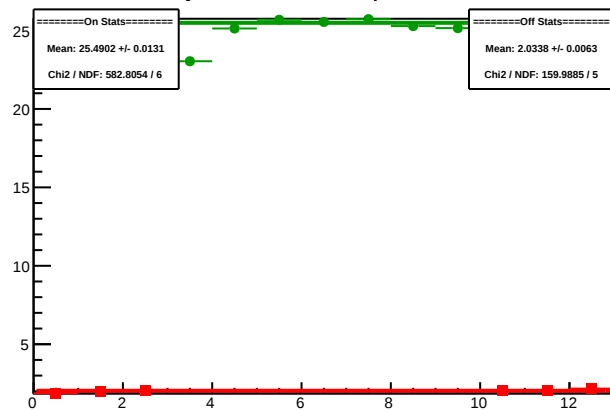
Cycle 5628.1: Multiplet Sums
