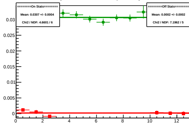
Cycle 5628.1: Multiplet Asyms
