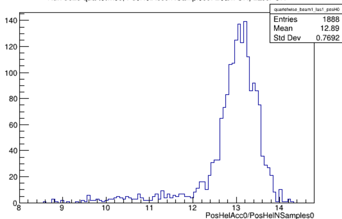
Run 5628 quartetwise, PosHelAcc0/NSamples0: Beam ON, Laser ON
