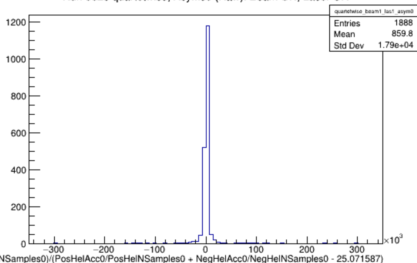
Run 5628 quartetwise, Asyms0 (Raw): Beam ON, Laser ON
