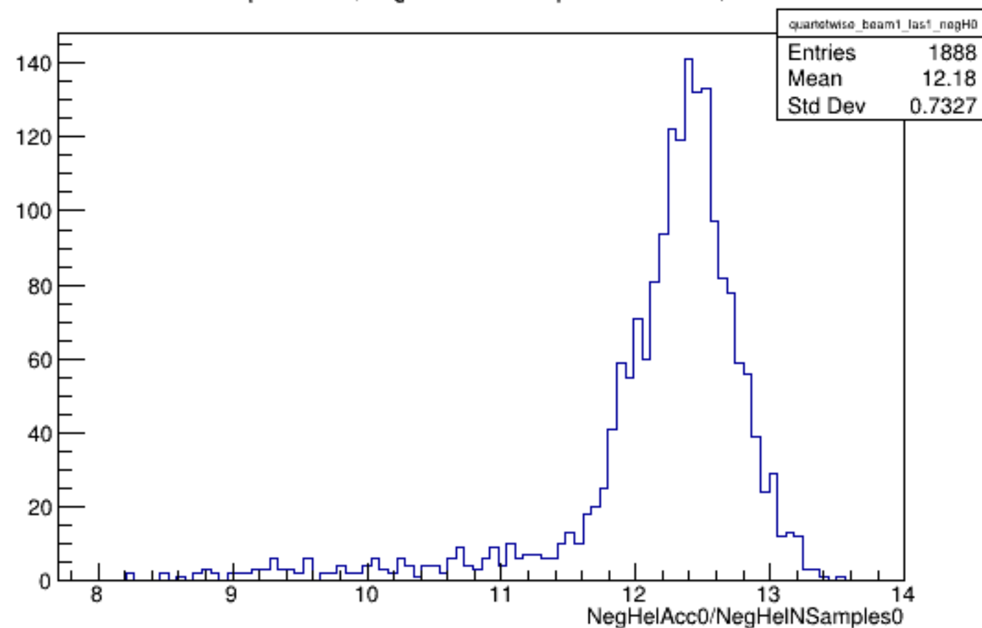
Run 5628 quartetwise, NegHelAcc0/NSamples0: Beam ON, Laser ON
