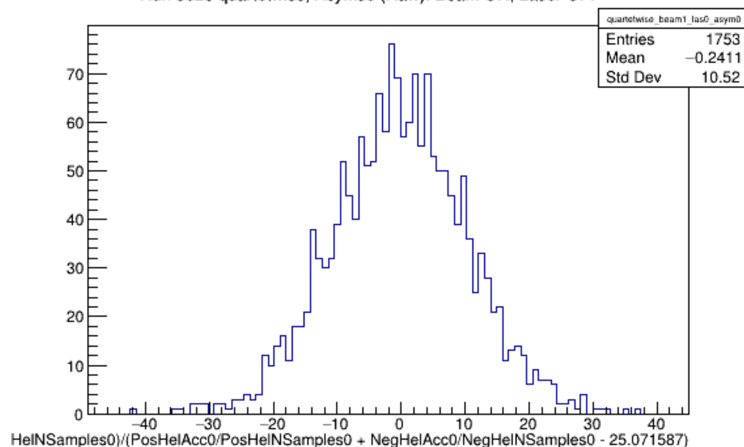
Run 5628 quartetwise, Asyms0 (Raw): Beam ON, Laser OFF
