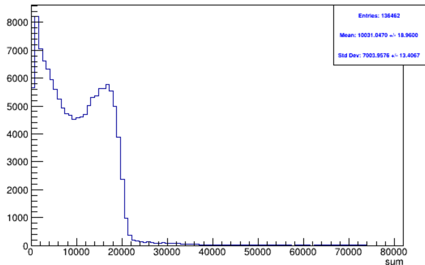
Run 5628 triggerwise, sums: All
