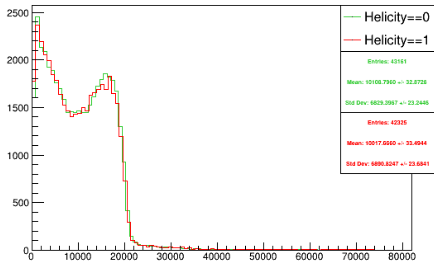
Run 5628 triggerwise, sums: Beam ON, Laser ON
