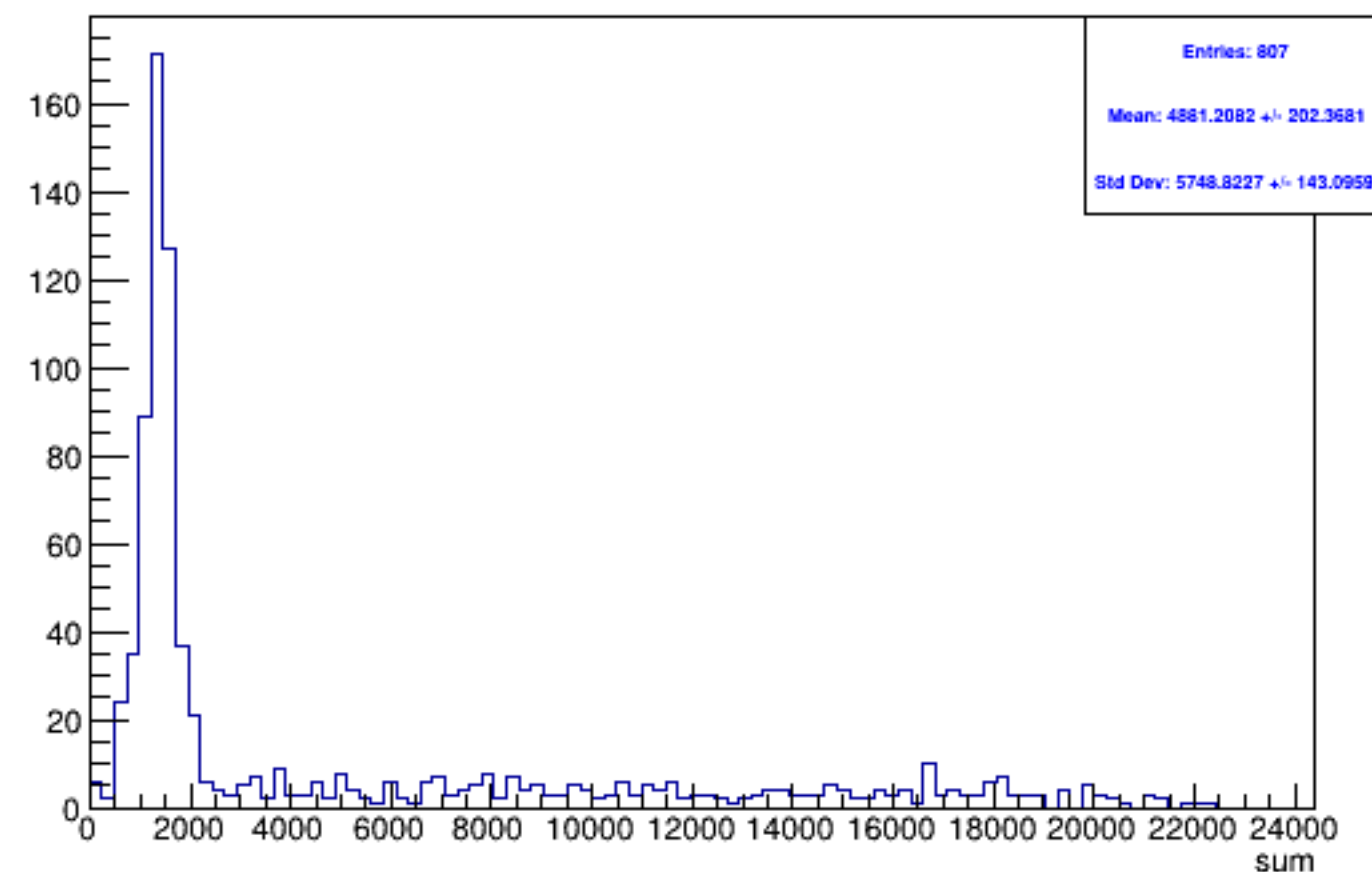
Run 5628 triggerwise, sums: Beam OFF
