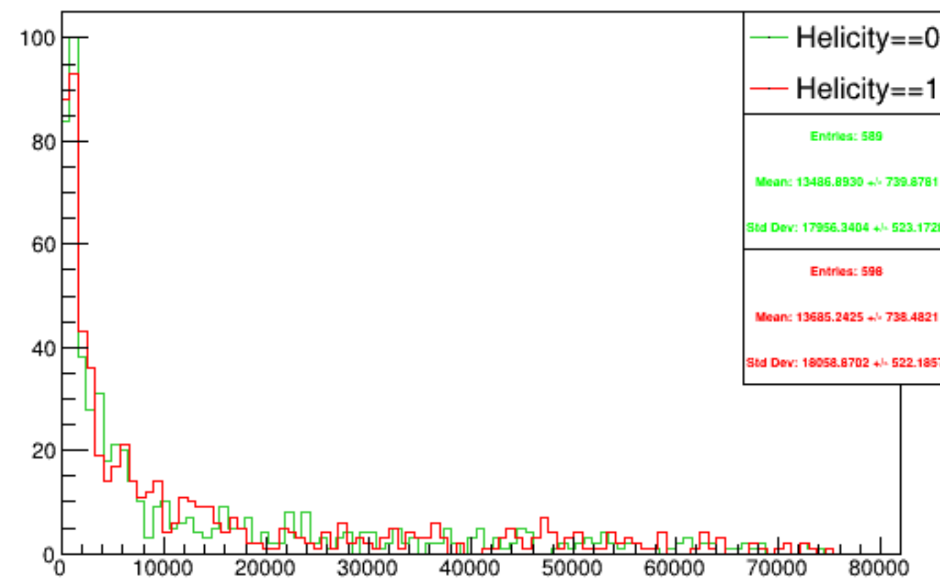
Run 5628 triggerwise, sums: Beam ON, Laser OFF
