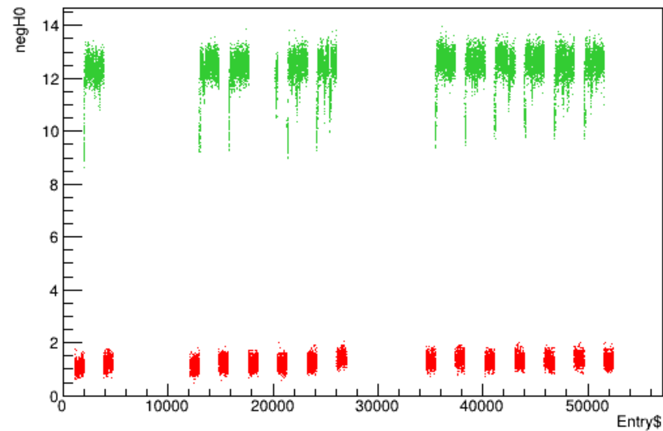
Run 5629 quartetwise, negH0 vs time
