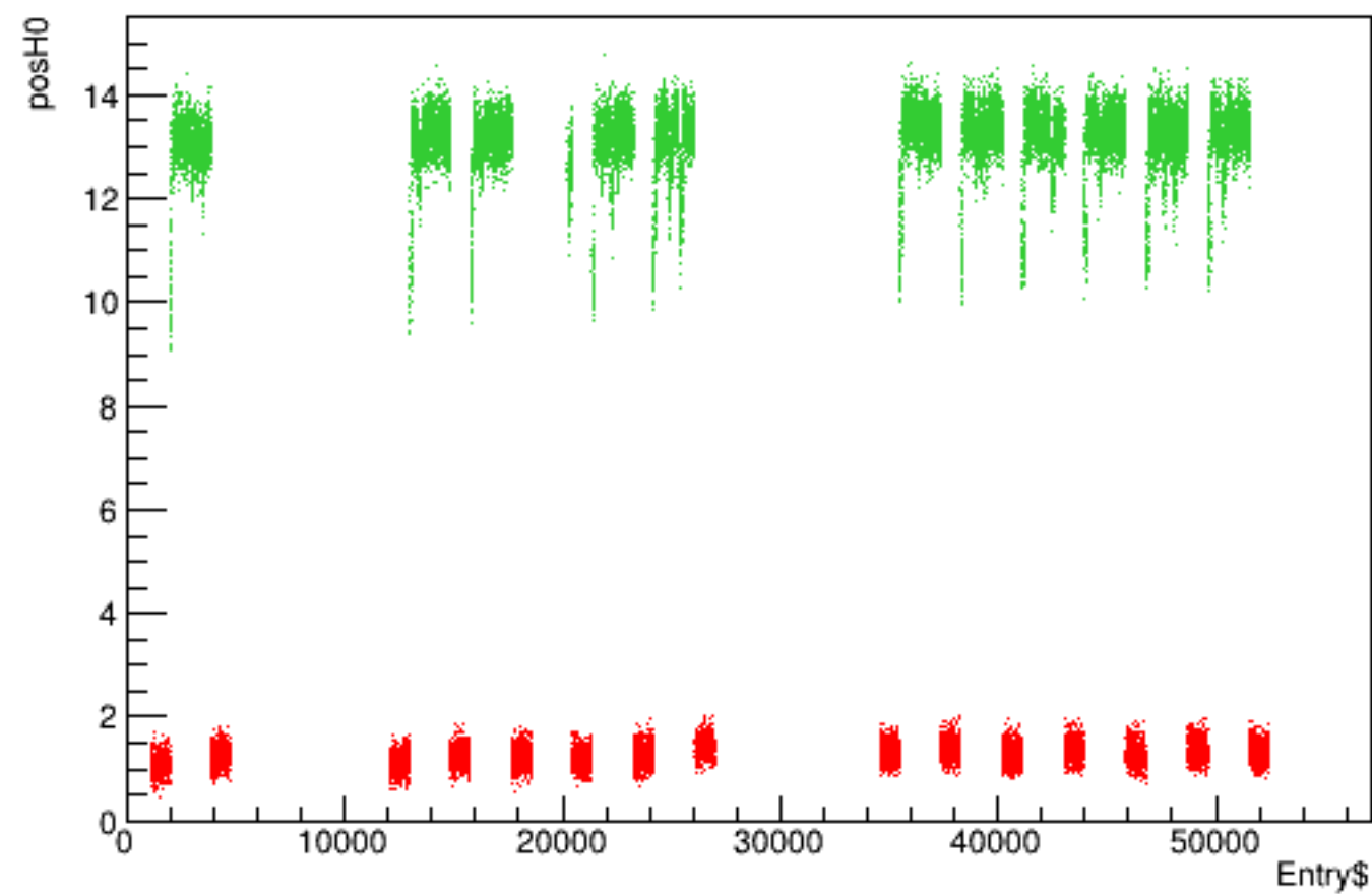
Run 5629 quartetwise, posH0 vs time
