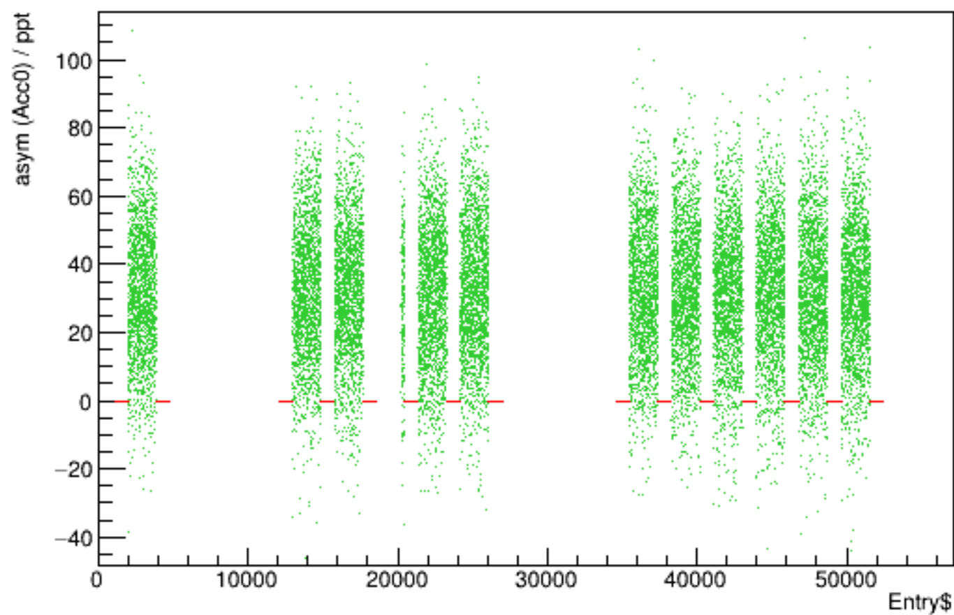
Run 5629 quartetwise, asym0sub vs time
