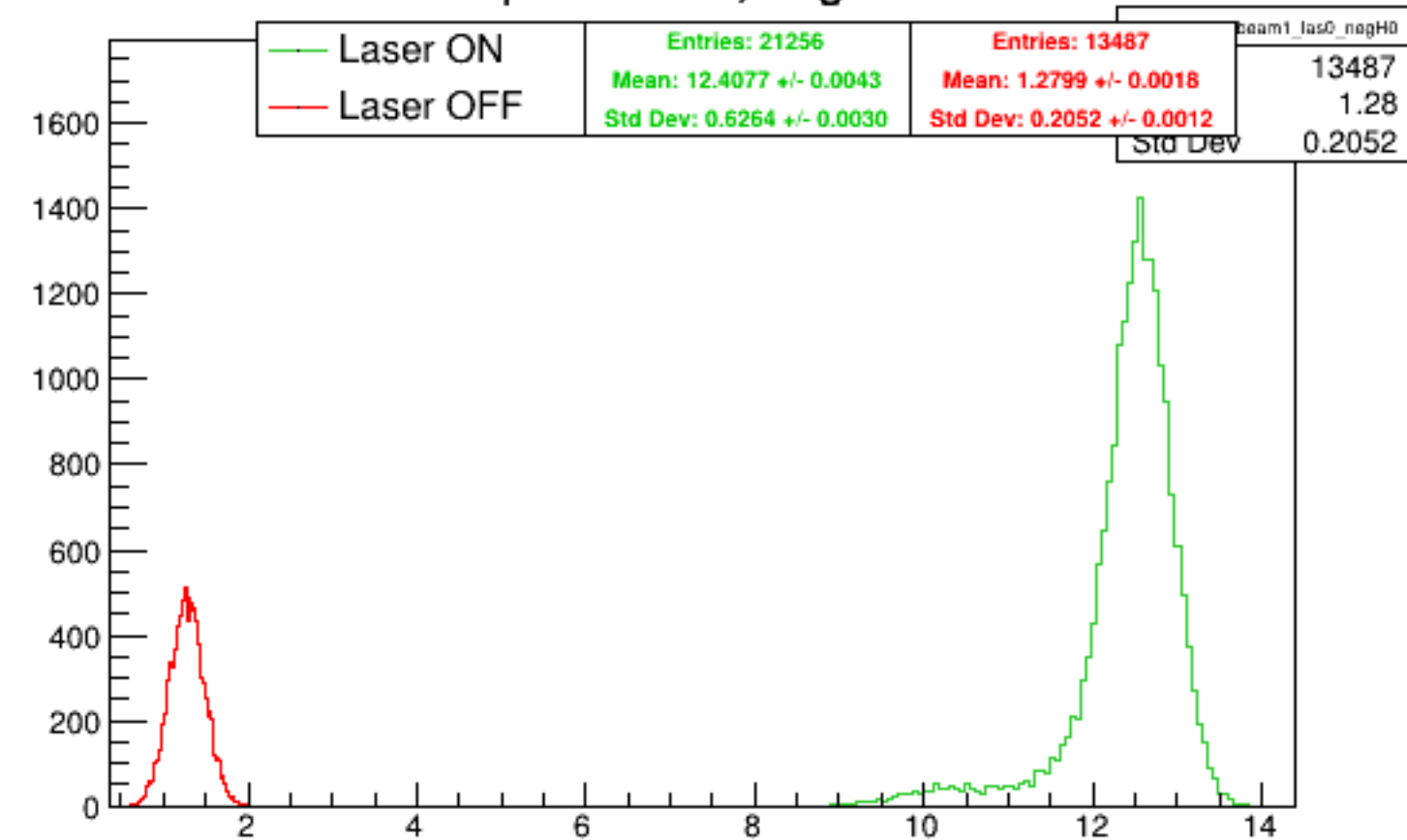
Run 5629 quartetwise, negH0: Beam ON
