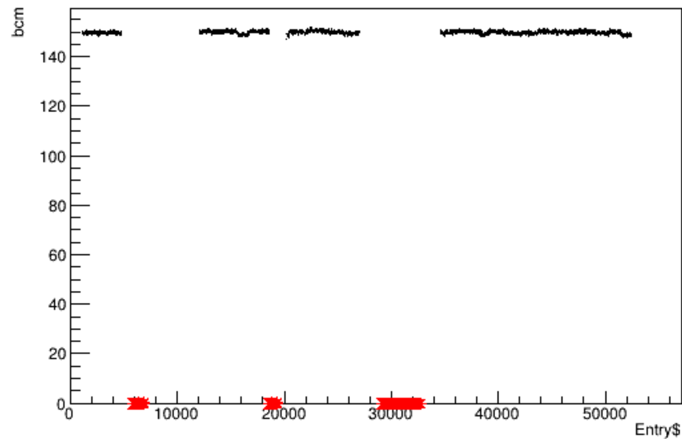
Run 5629 quartetwise, bcm vs time
