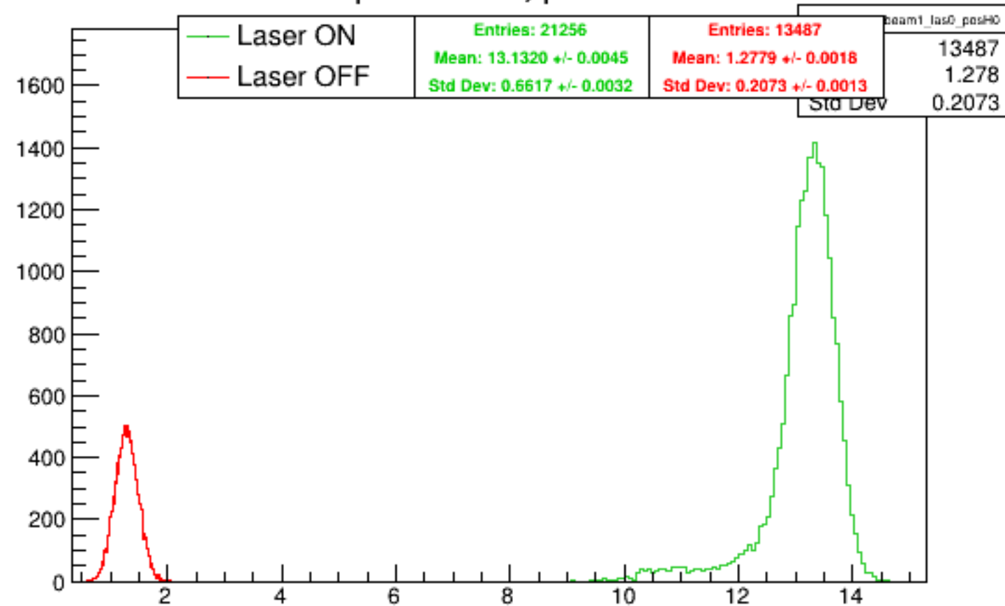
Run 5629 quartetwise, posH0: Beam ON
