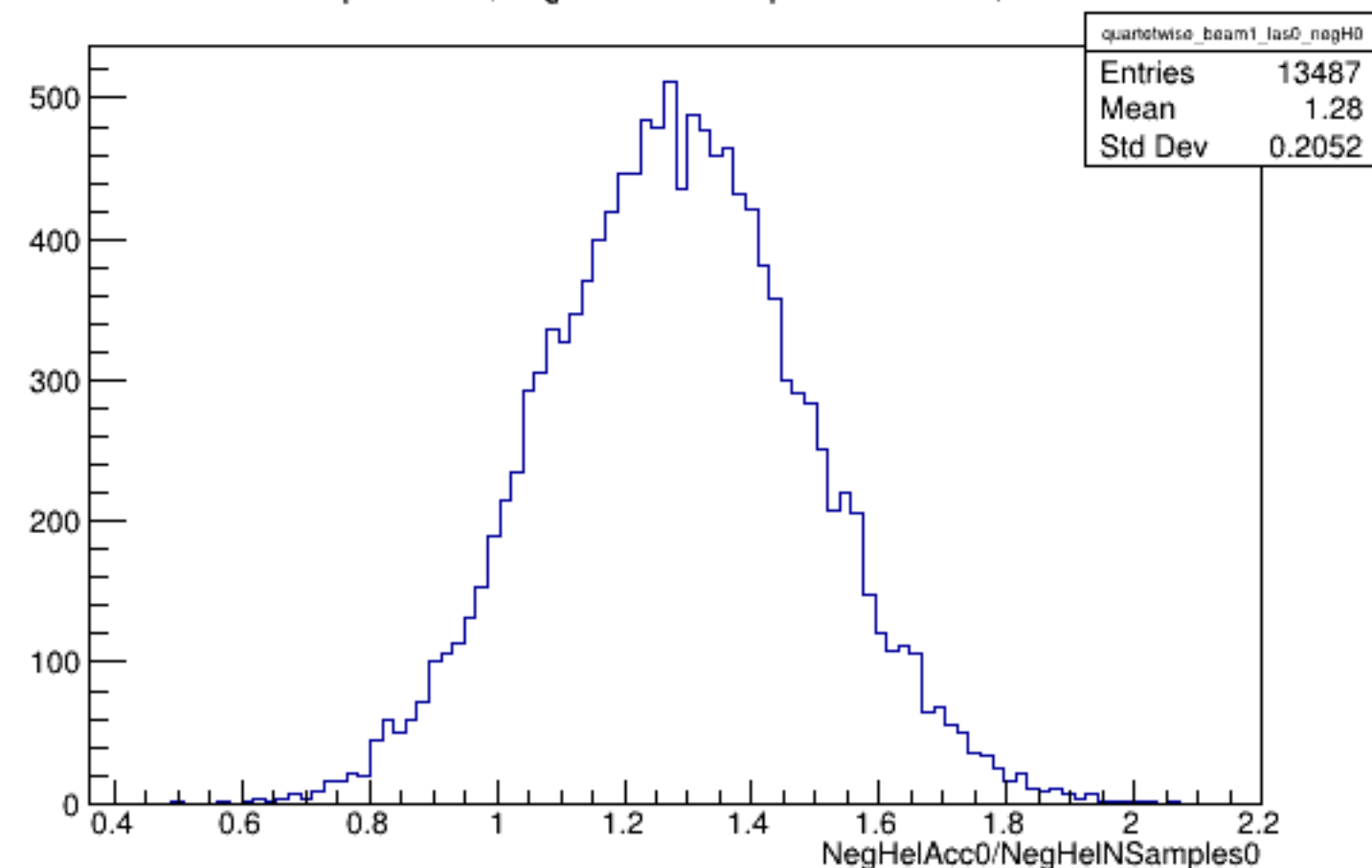
Run 5629 quartetwise, NegHelAcc0/NSamples0: Beam ON, Laser OFF
