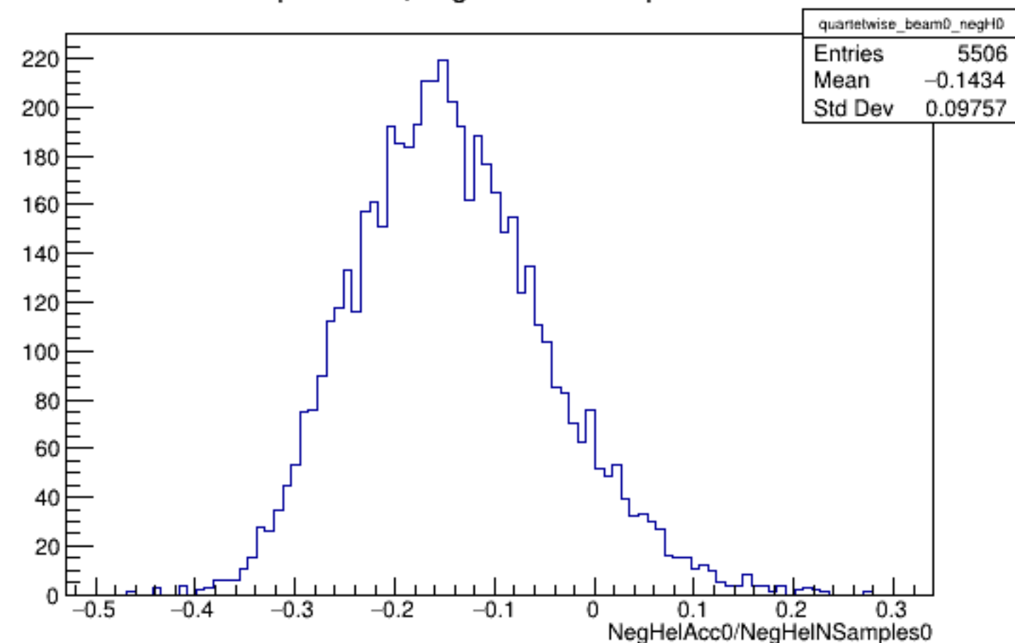
Run 5629 quartetwise, NegHelAcc0/NSamples0: Beam OFF
