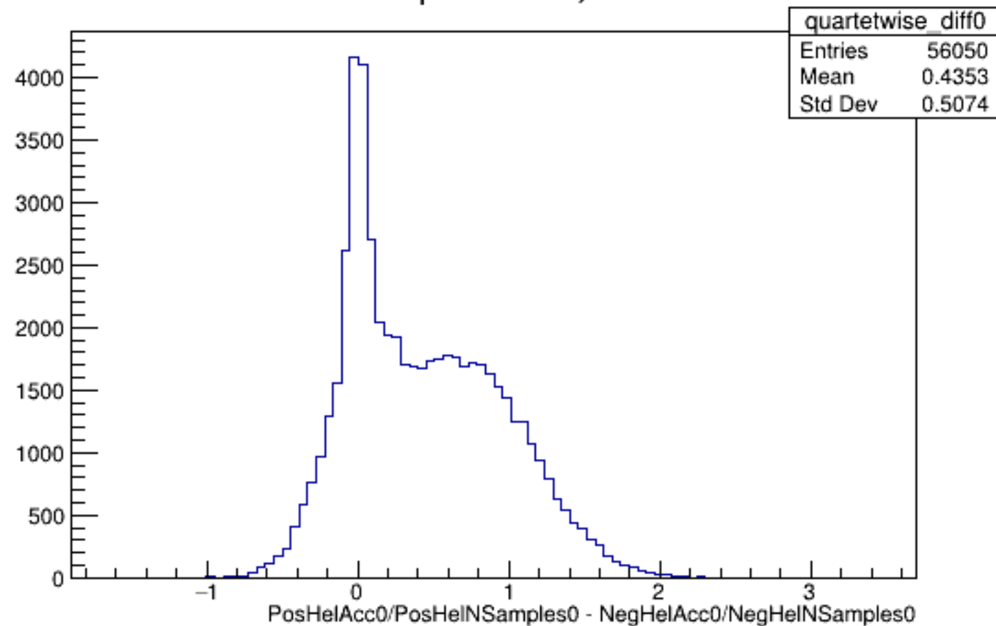
Run 5629 quartetwise, Diffs0: All
