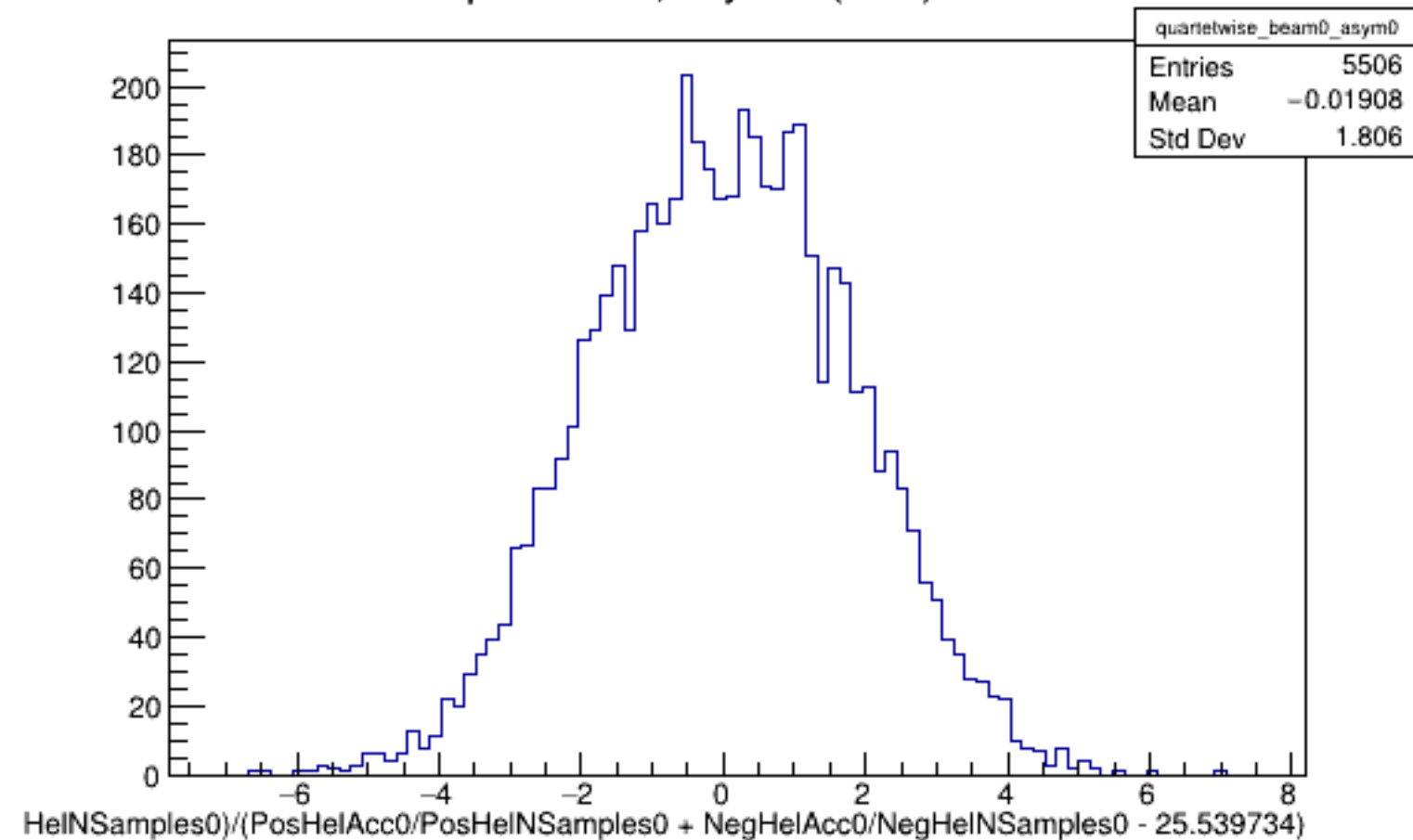
Run 5629 quartetwise, Asyms0 (Raw): Beam OFF
