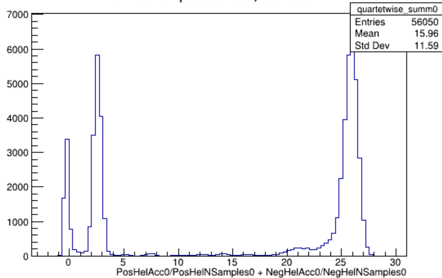
Run 5629 quartetwise, Sums0: All
