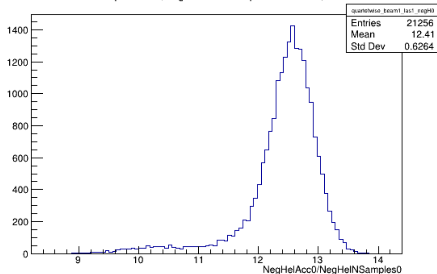
Run 5629 quartetwise, NegHelAcc0/NSamples0: Beam ON, Laser ON
