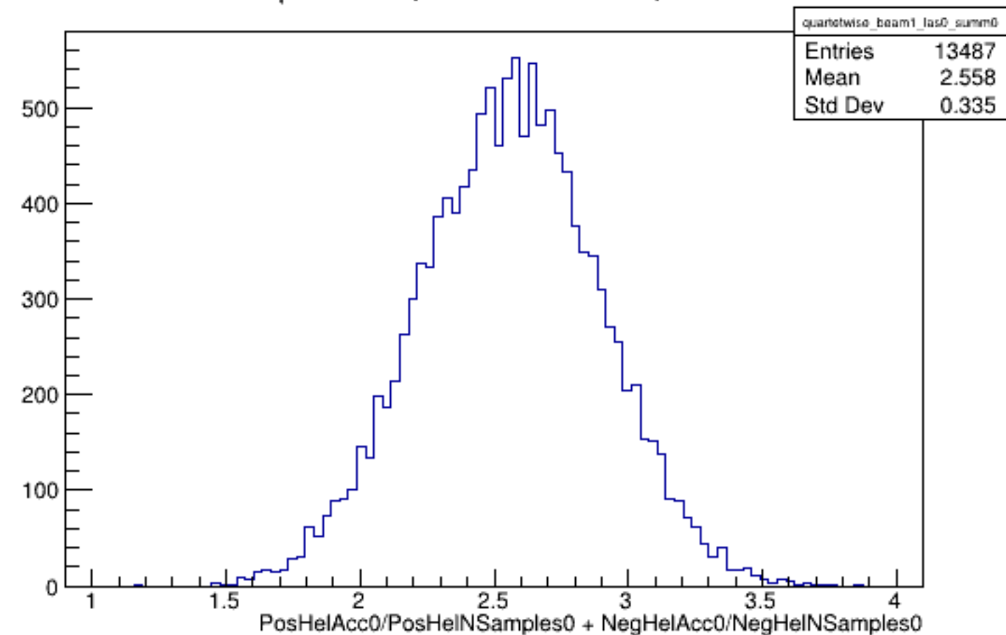
Run 5629 quartetwise, Sums0: Beam ON, Laser OFF
