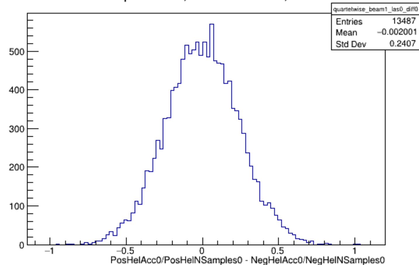
Run 5629 quartetwise, Diffs0: Beam ON, Laser OFF
