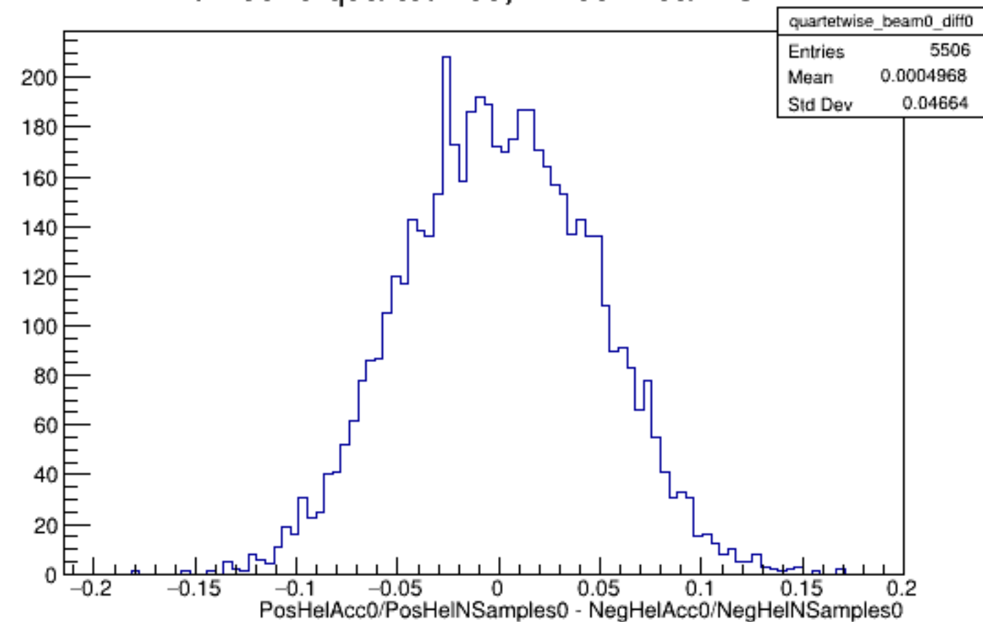
Run 5629 quartetwise, Diffs0: Beam OFF
