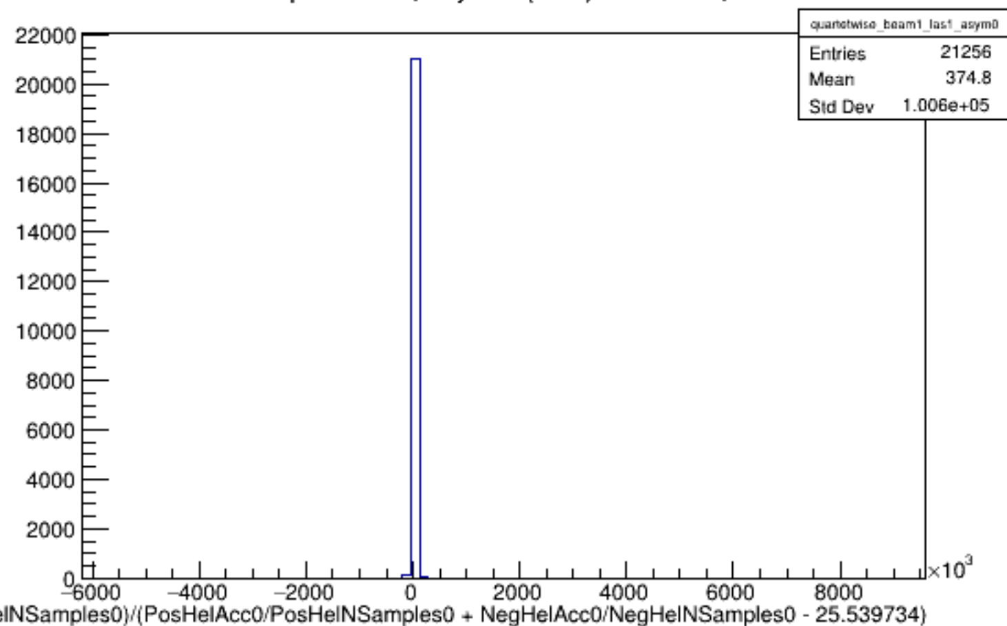
Run 5629 quartetwise, Asyms0 (Raw): Beam ON, Laser ON
