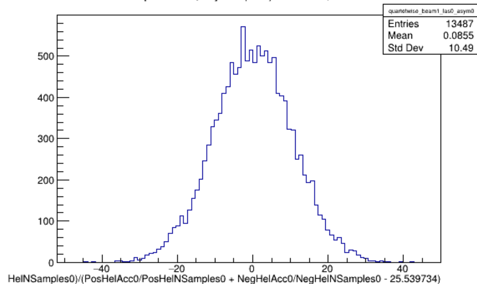
Run 5629 quartetwise, Asyms0 (Raw): Beam ON, Laser OFF
