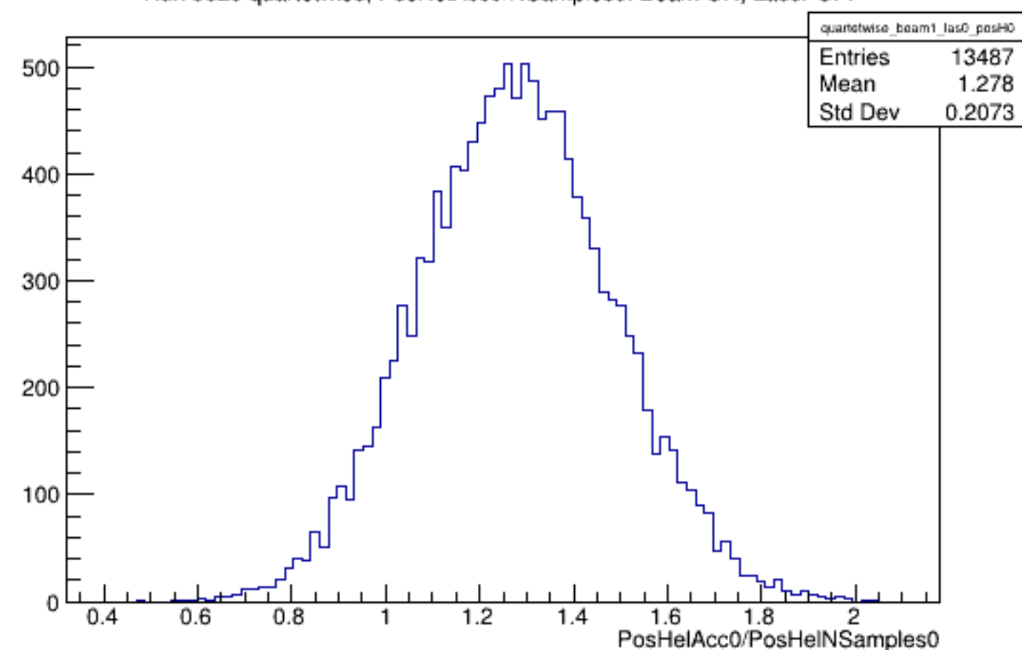
Run 5629 quartetwise, PosHelAcc0/NSamples0: Beam ON, Laser OFF
