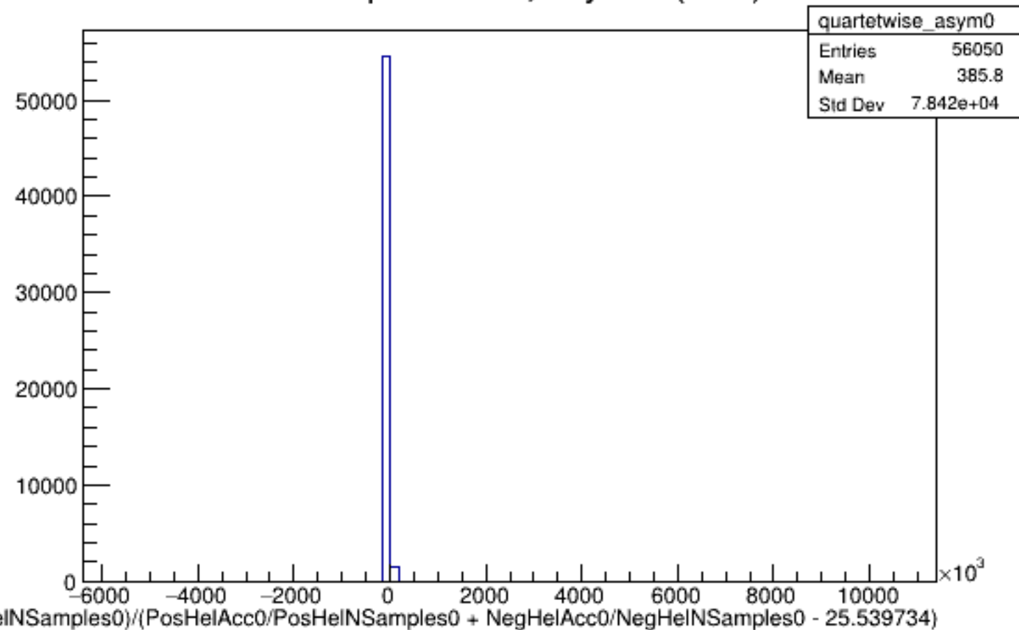
Run 5629 quartetwise, Asyms0 (Raw): All
