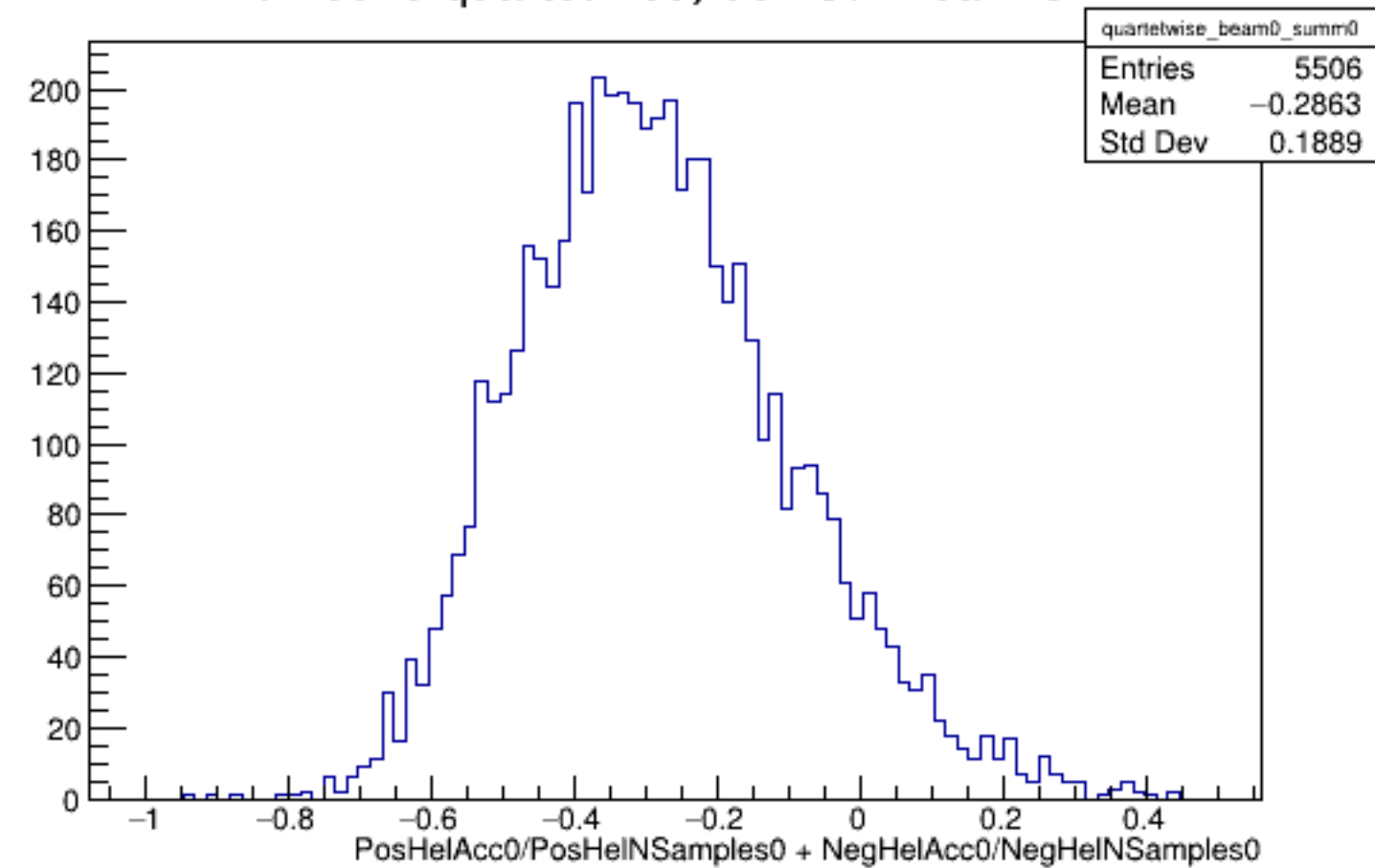
Run 5629 quartetwise, Sums0: Beam OFF
