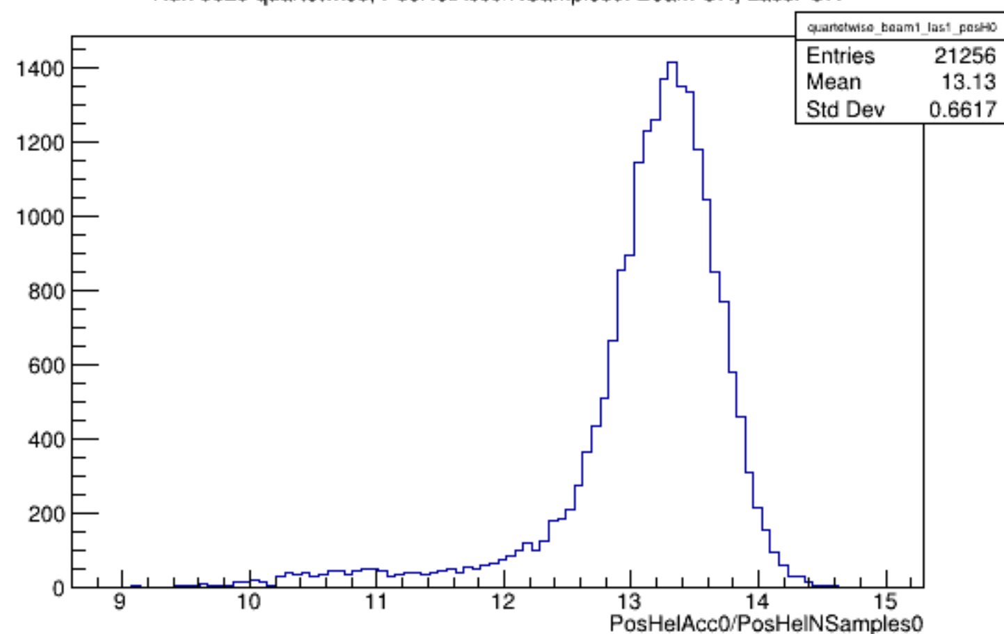
Run 5629 quartetwise, PosHelAcc0/NSamples0: Beam ON, Laser ON
