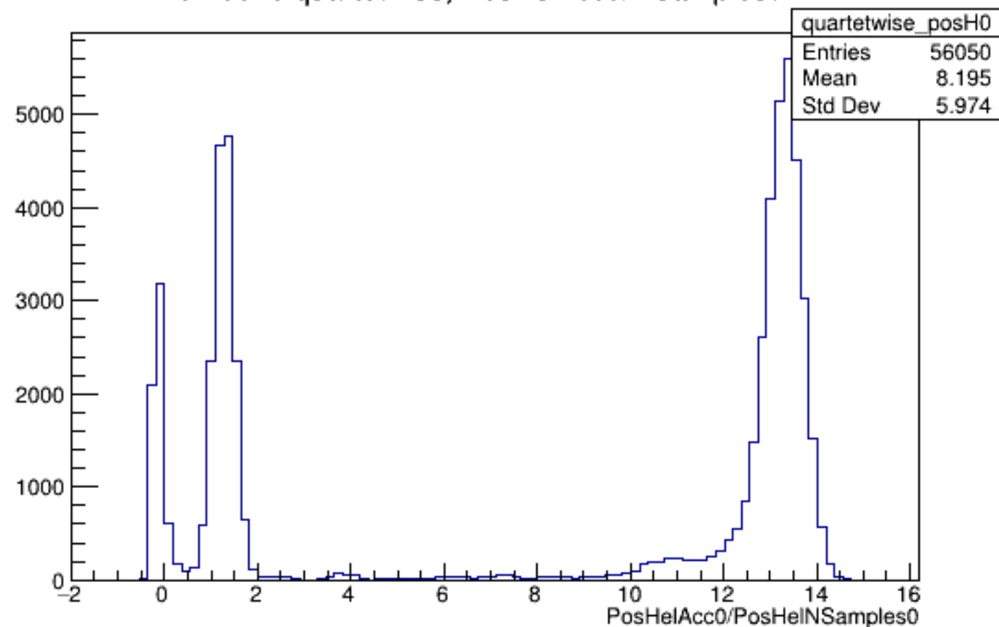
Run 5629 quartetwise, PosHelAcc0/NSamples0: All
