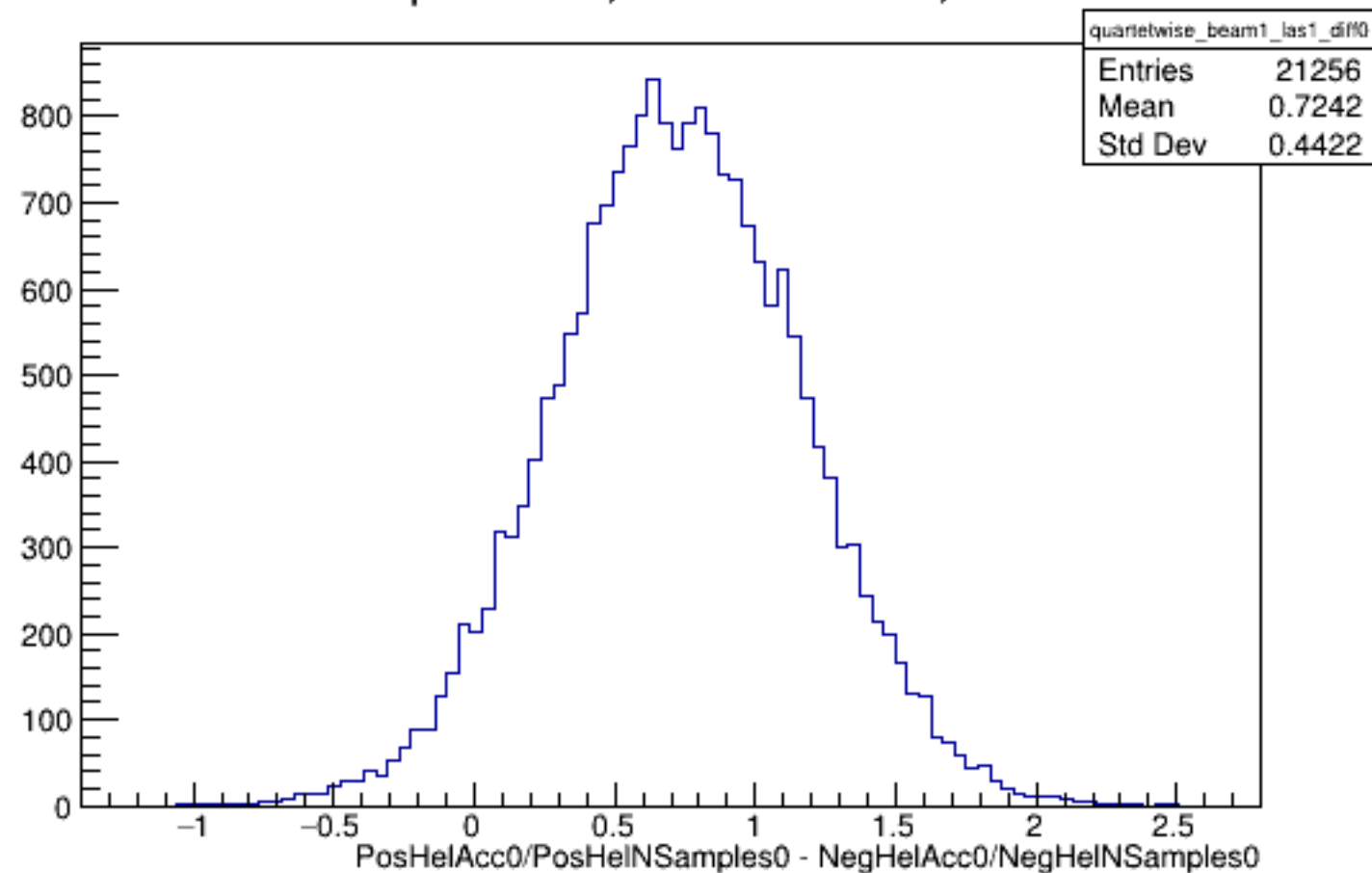
Run 5629 quartetwise, Diffs0: Beam ON, Laser ON
