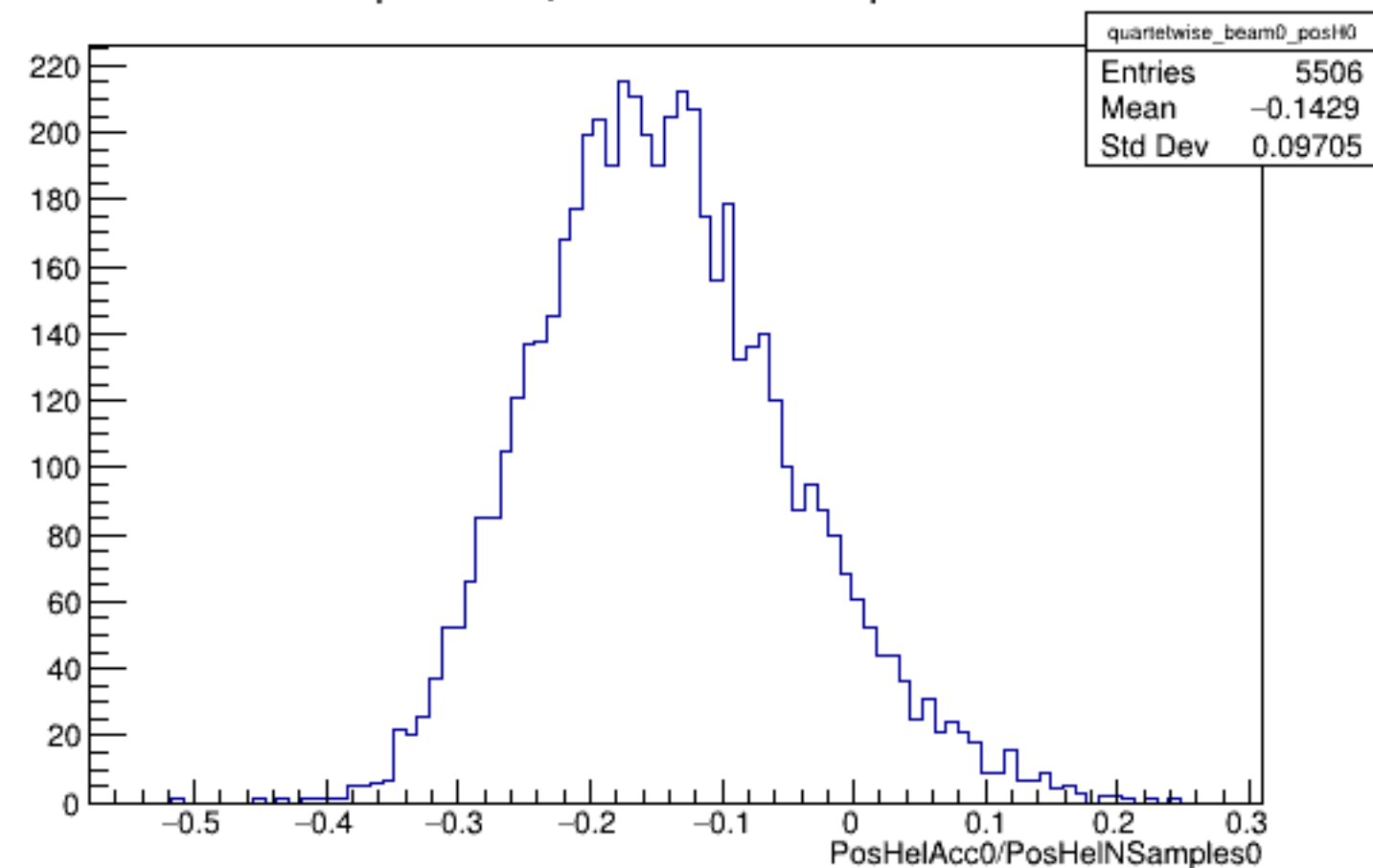
Run 5629 quartetwise, PosHelAcc0/NSamples0: Beam OFF
