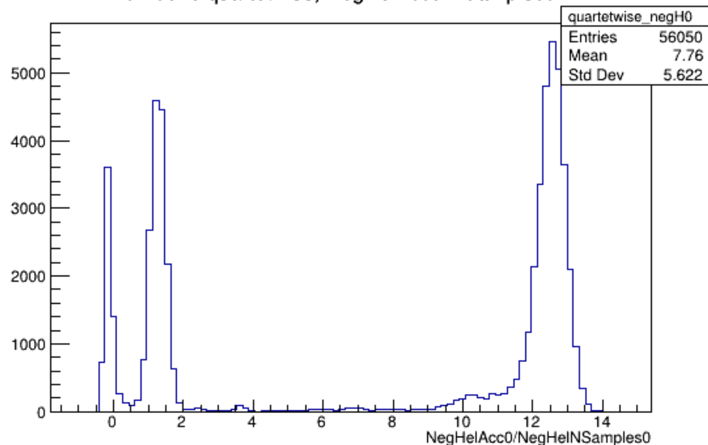
Run 5629 quartetwise, NegHelAcc0/NSamples0: All
