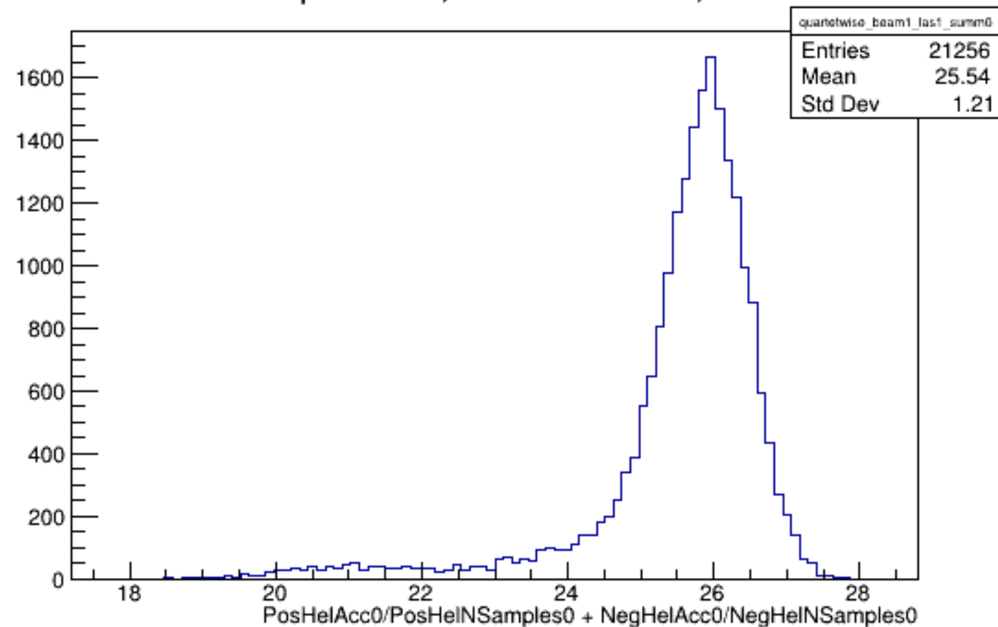
Run 5629 quartetwise, Sums0: Beam ON, Laser ON
