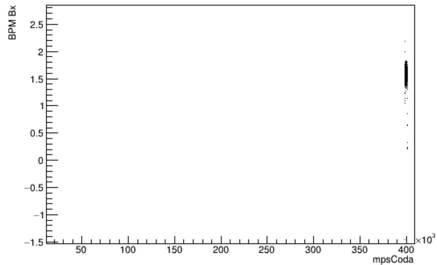
Run 5631 mpwise, beam OFF, laser OFF
