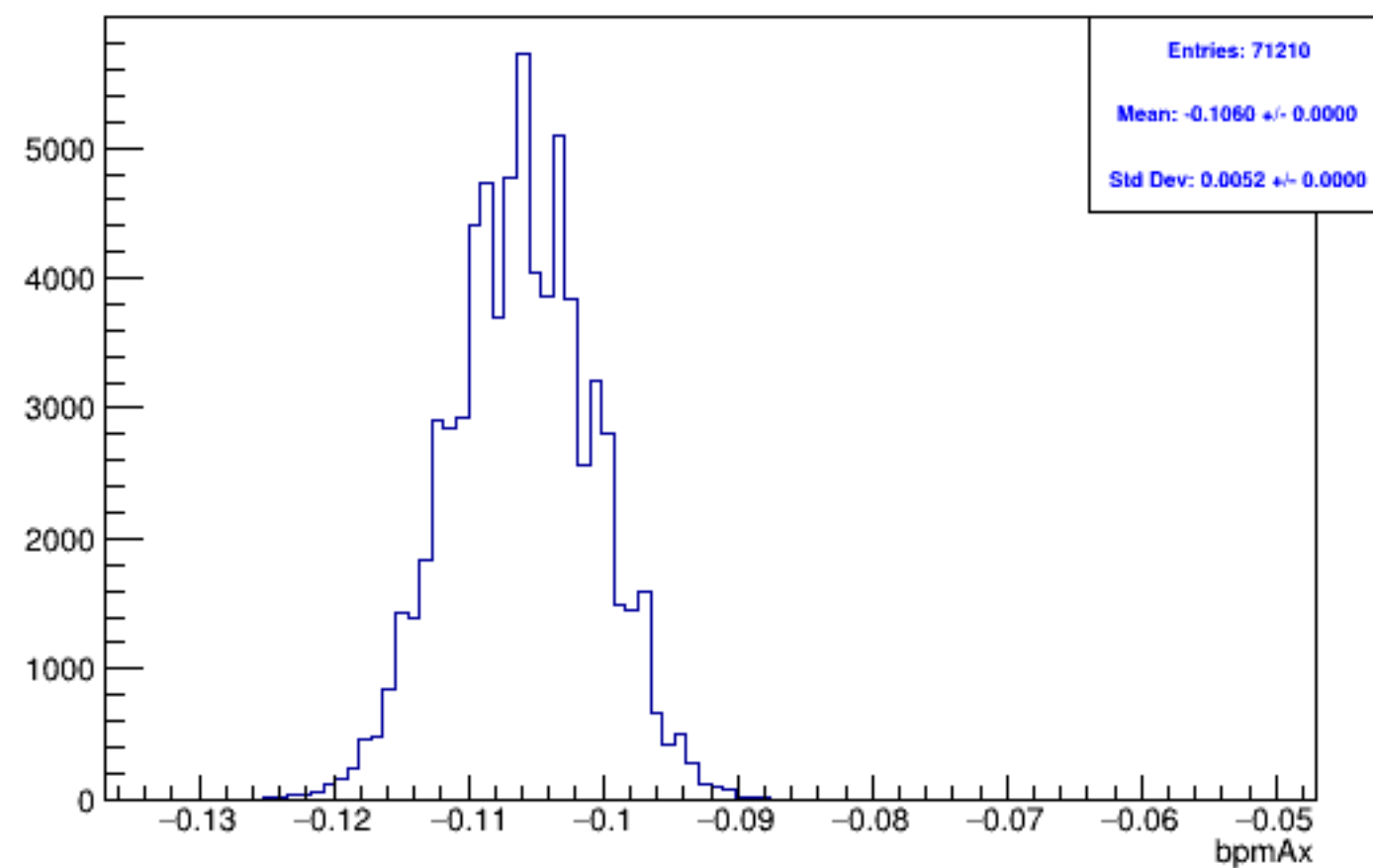
Run 5631, mpswise, bpmAx: Beam ON, Laser OFF
