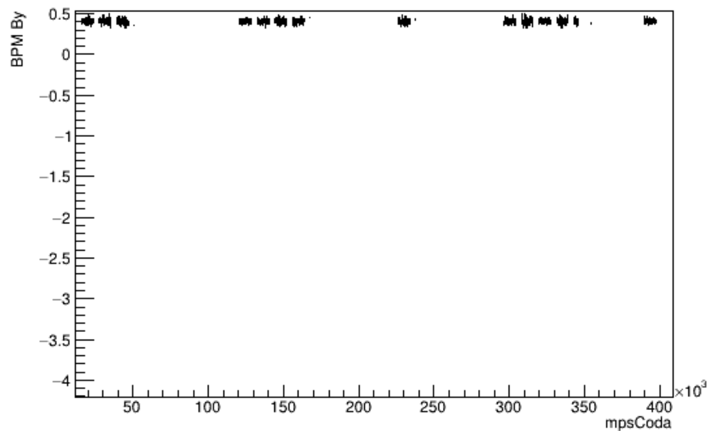
Run 5631 mpwise, beam ON, laser ON
