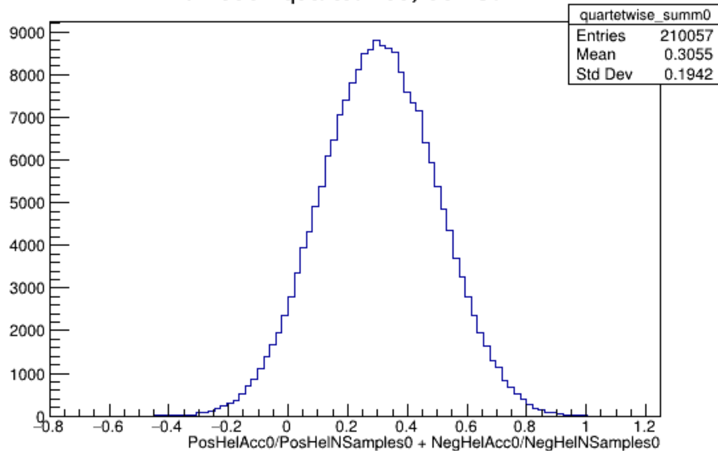
Run 5634 quartetwise, Sums0: All
