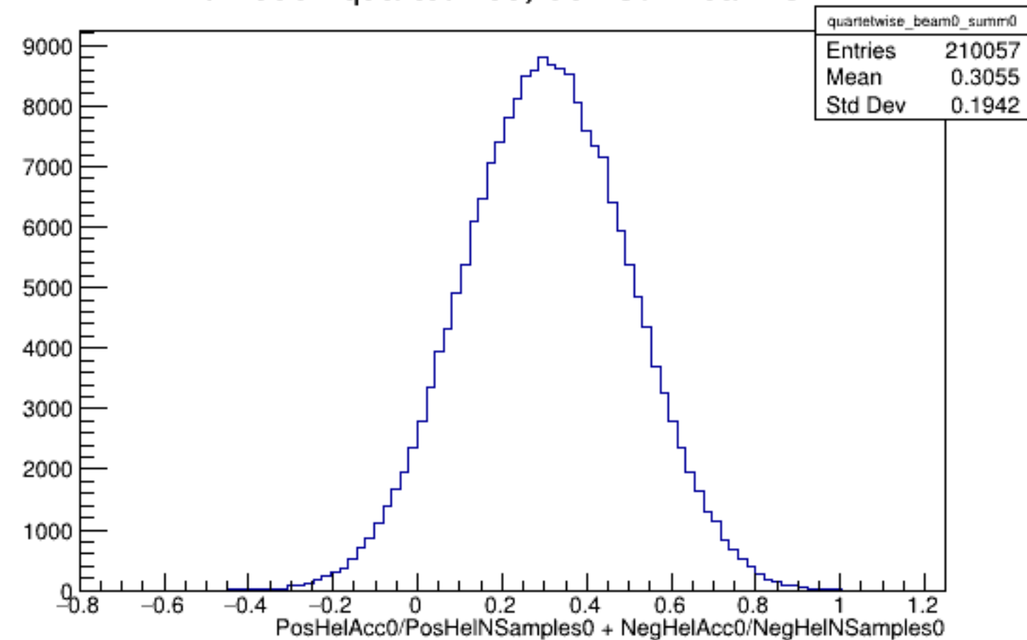
Run 5634 quartetwise, Sums0: Beam OFF
