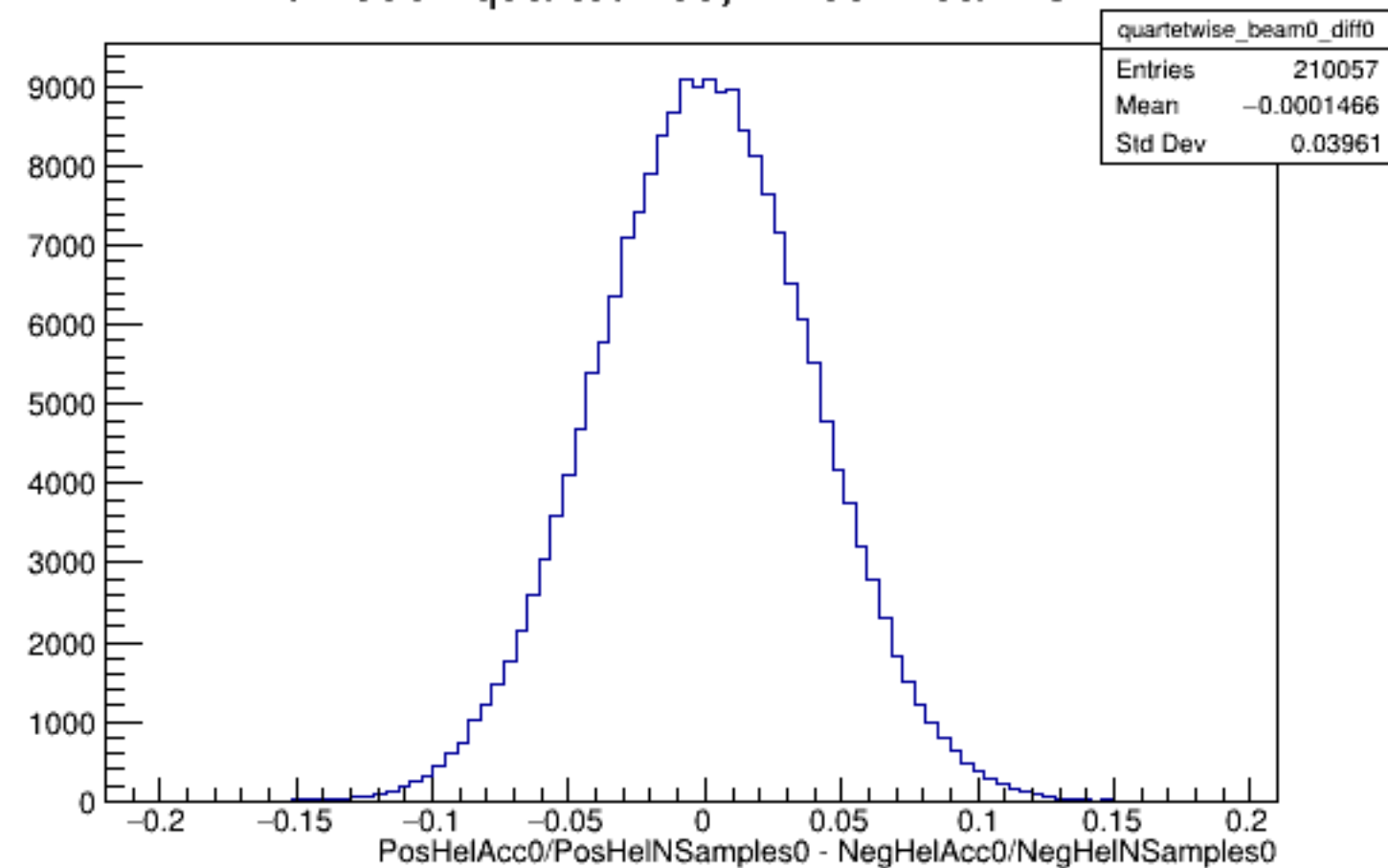
Run 5634 quartetwise, Diffs0: Beam OFF
