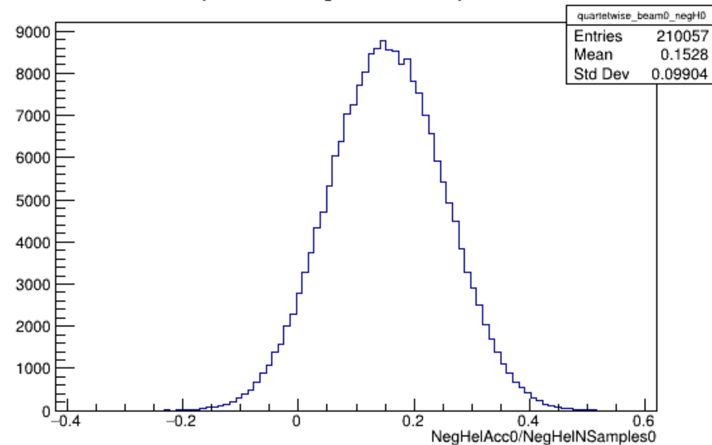
Run 5634 quartetwise, NegHelAcc0/NSamples0: Beam OFF
