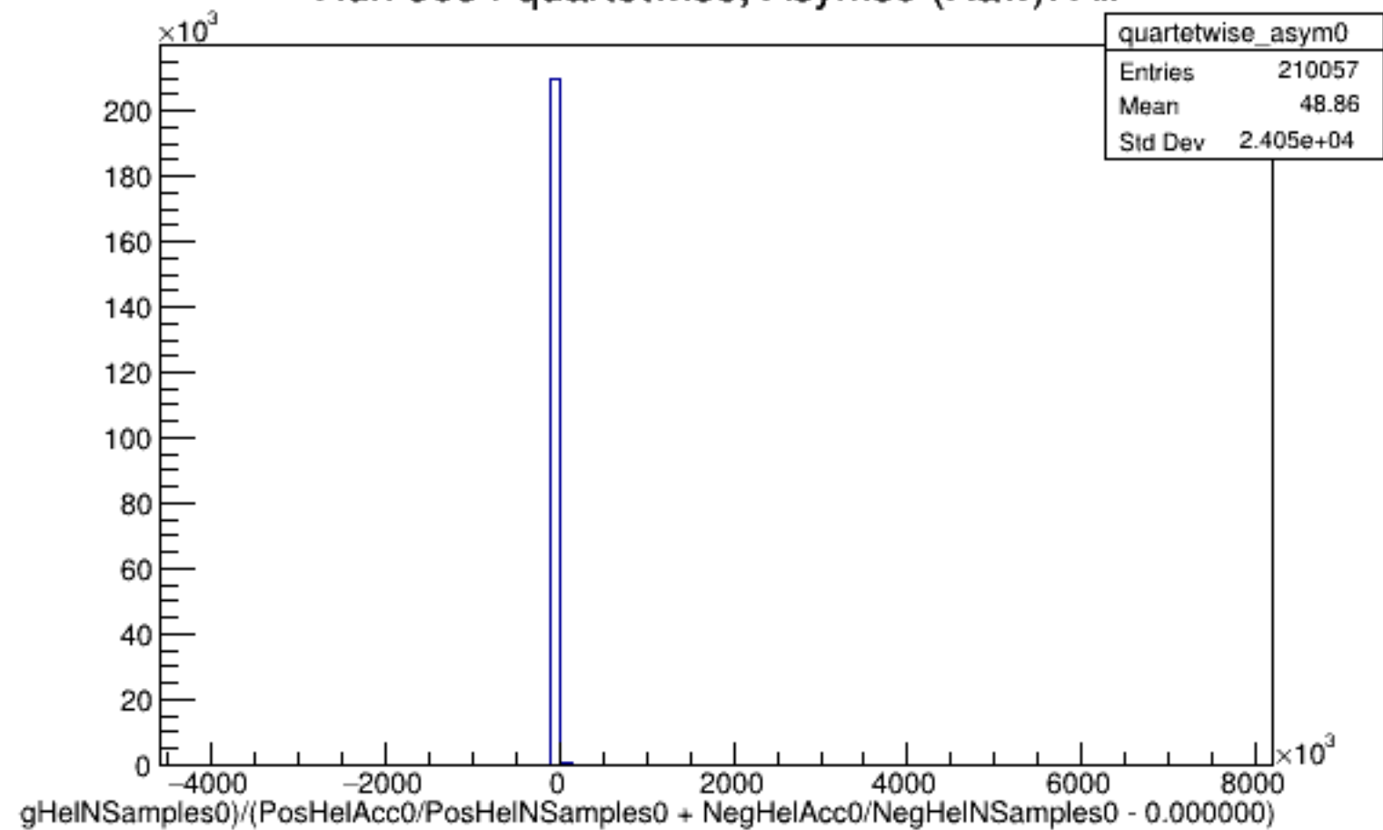
Run 5634 quartetwise, Asyms0 (Raw): All
