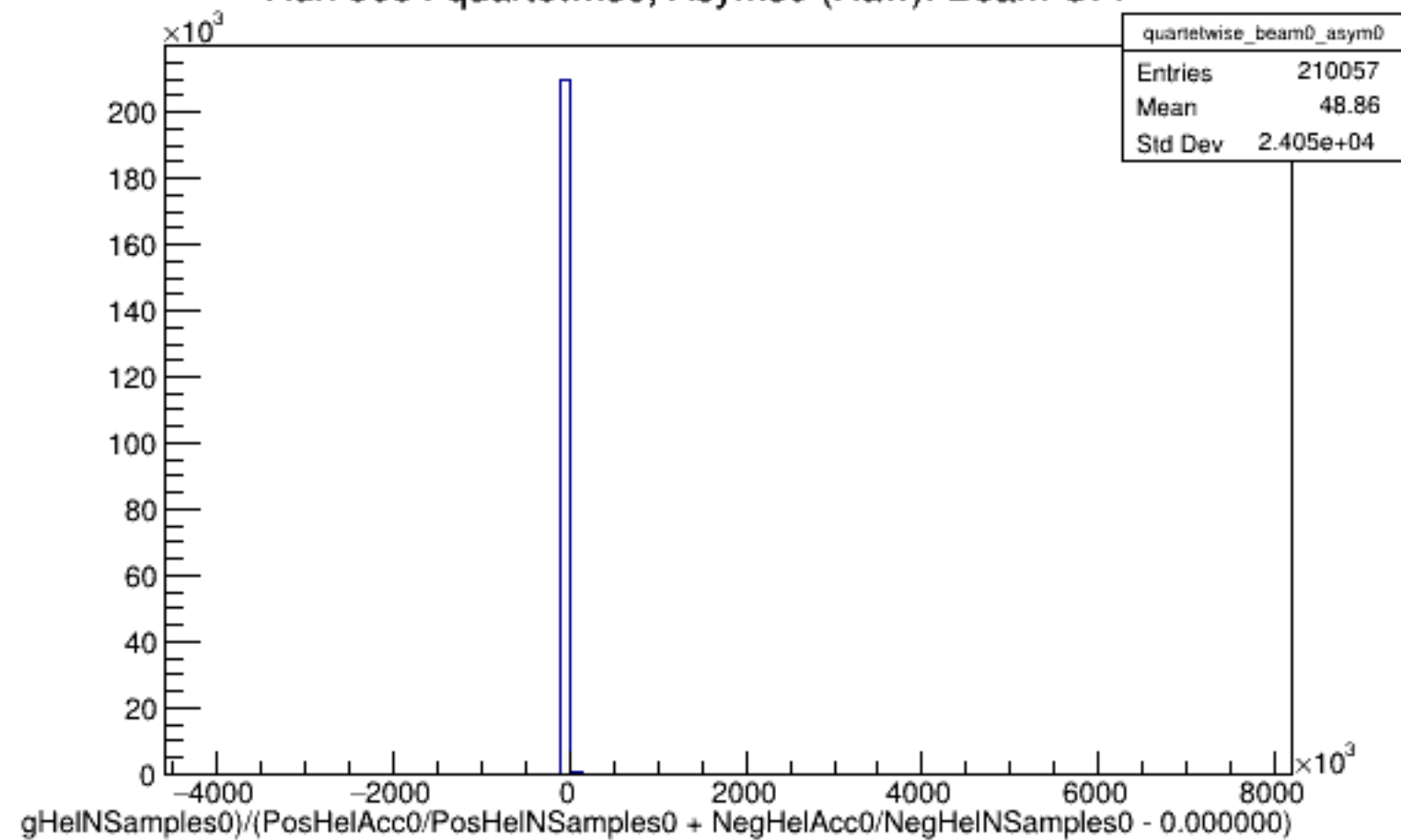
Run 5634 quartetwise, Asyms0 (Raw): Beam OFF
