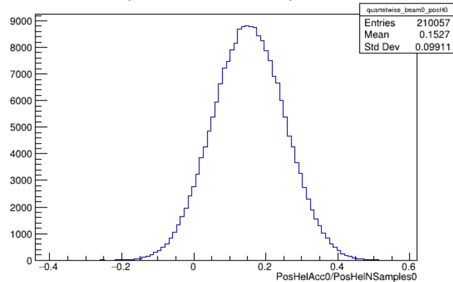
Run 5634 quartetwise, PosHelAcc0/NSamples0: Beam OFF
