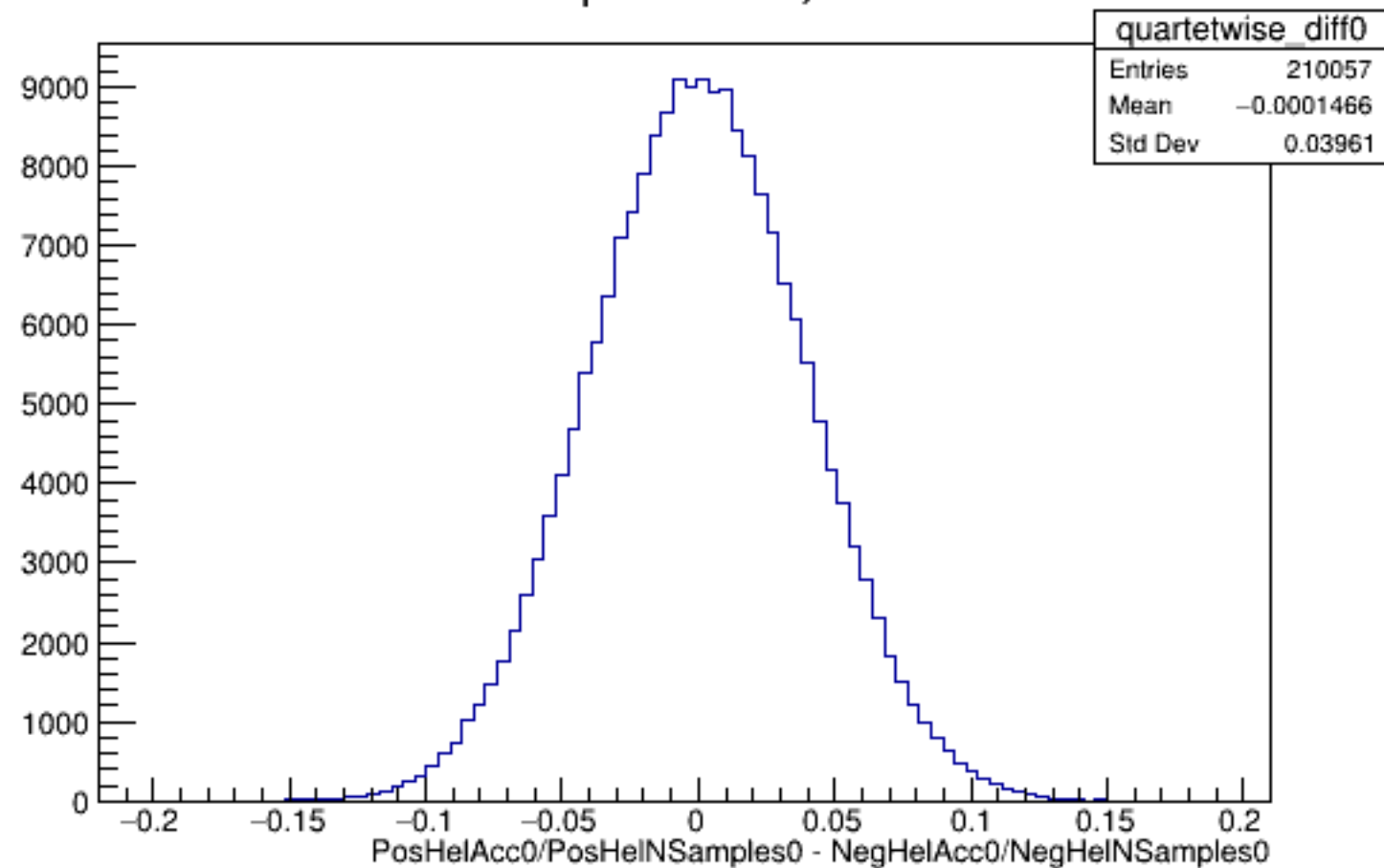
Run 5634 quartetwise, Diffs0: All
