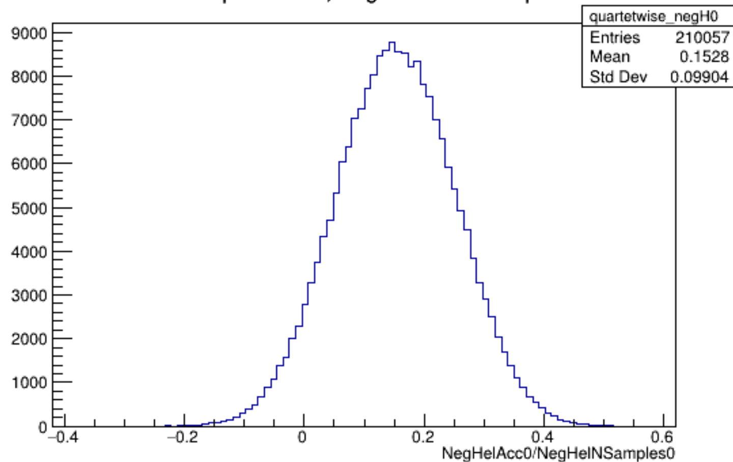
Run 5634 quartetwise, NegHelAcc0/NSamples0: All
