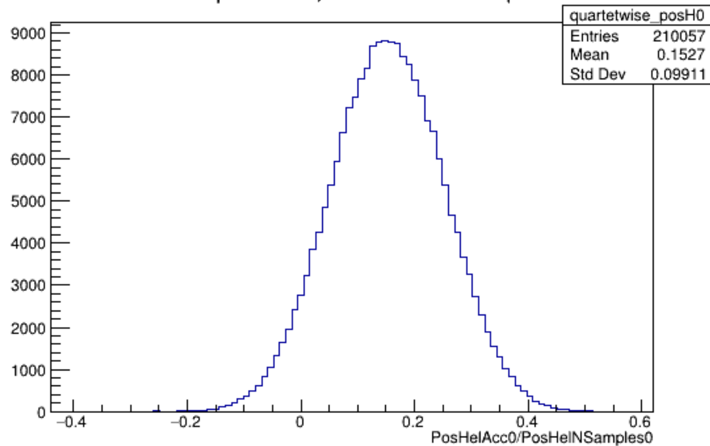
Run 5634 quartetwise, PosHelAcc0/NSamples0: All
