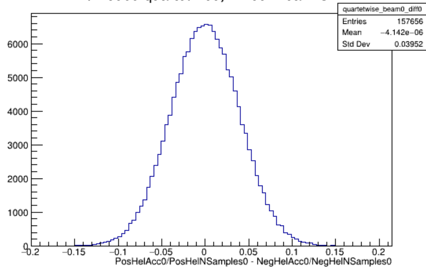
Run 5635 quartetwise, Diffs0: Beam OFF
