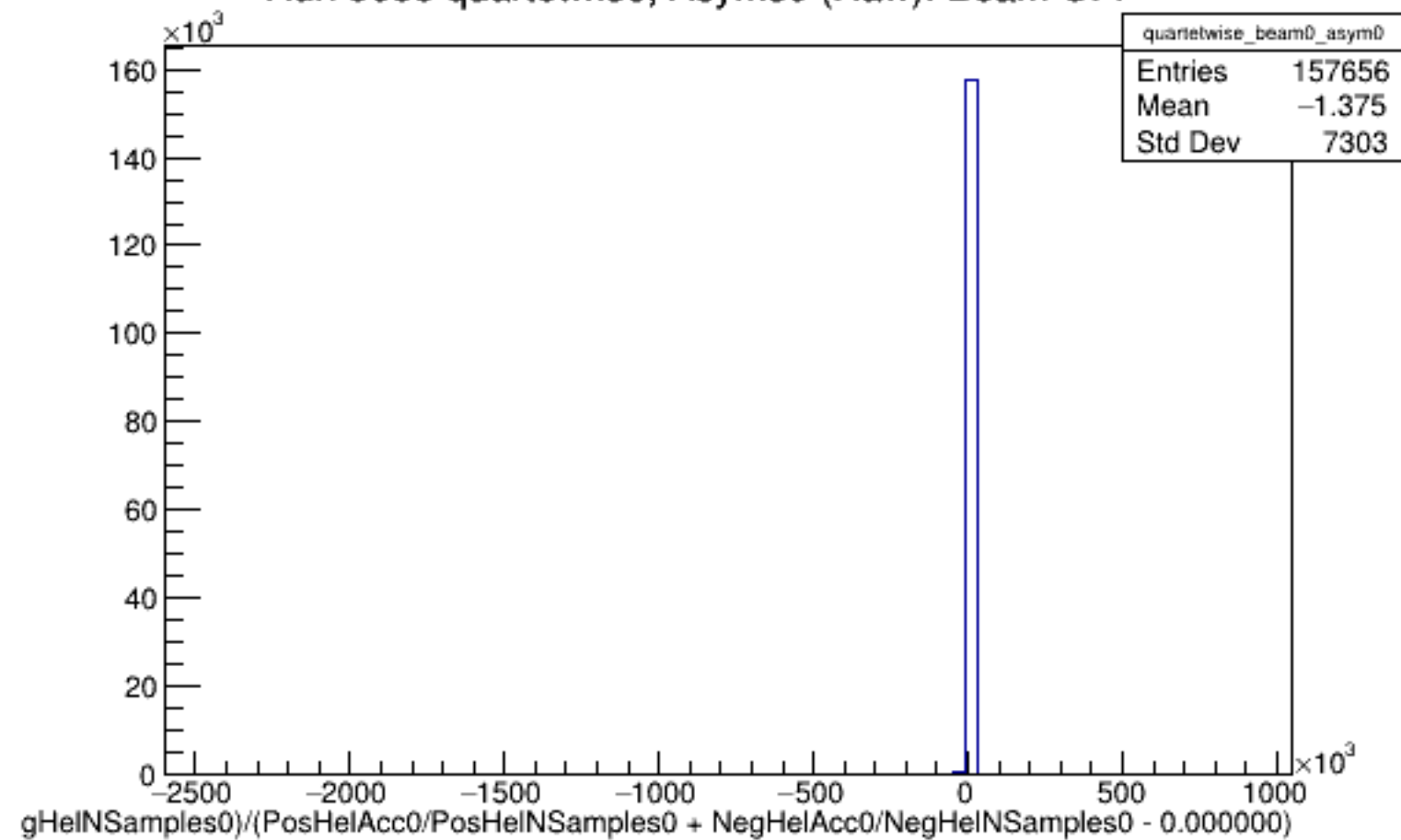
Run 5635 quartetwise, Asyms0 (Raw): Beam OFF
