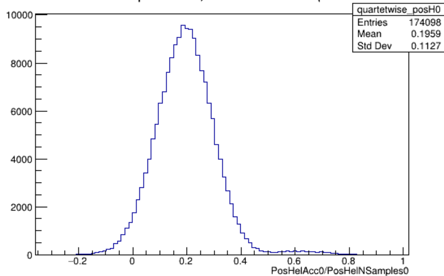
Run 5635 quartetwise, PosHelAcc0/NSamples0: All
