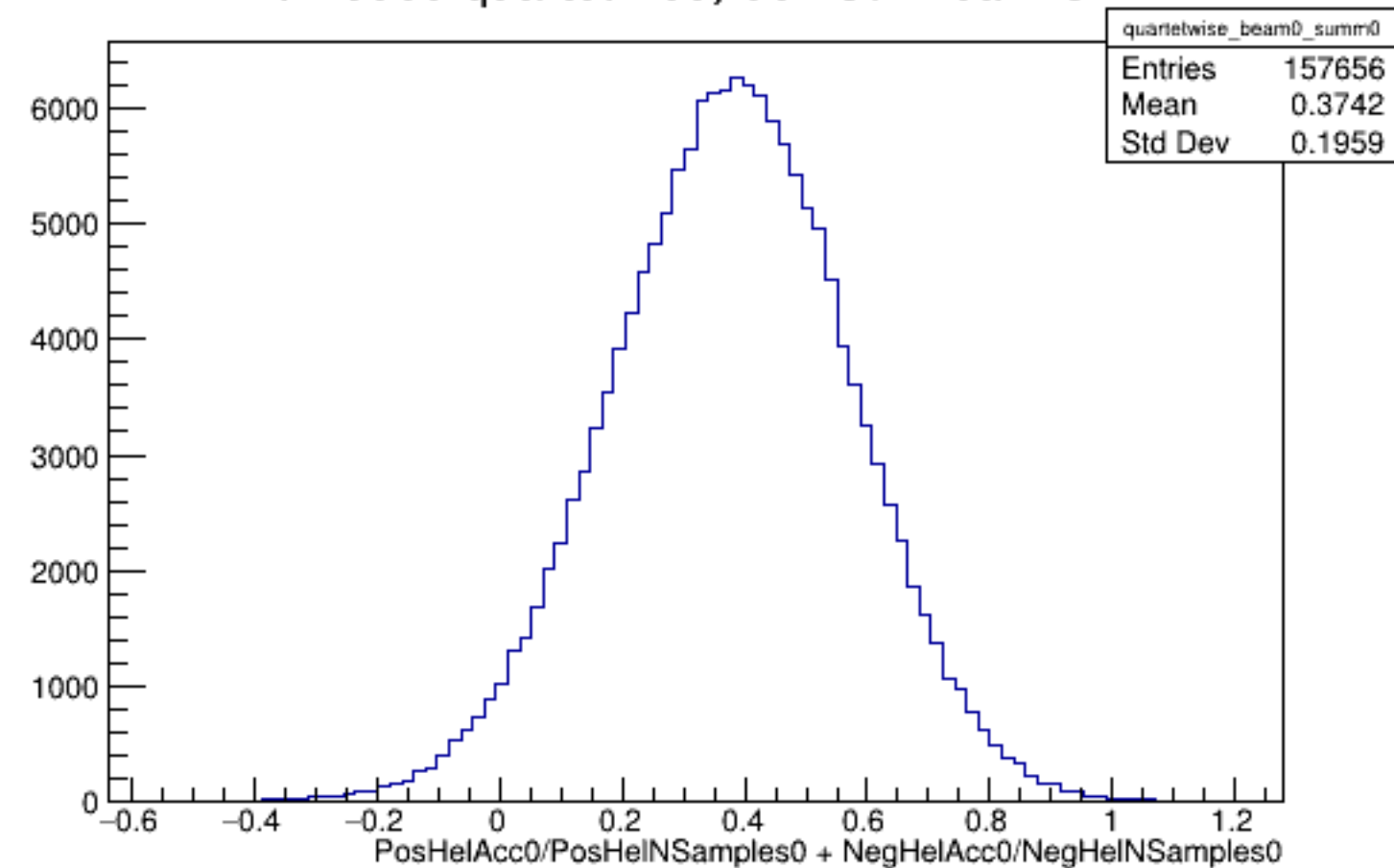
Run 5635 quartetwise, Sums0: Beam OFF
