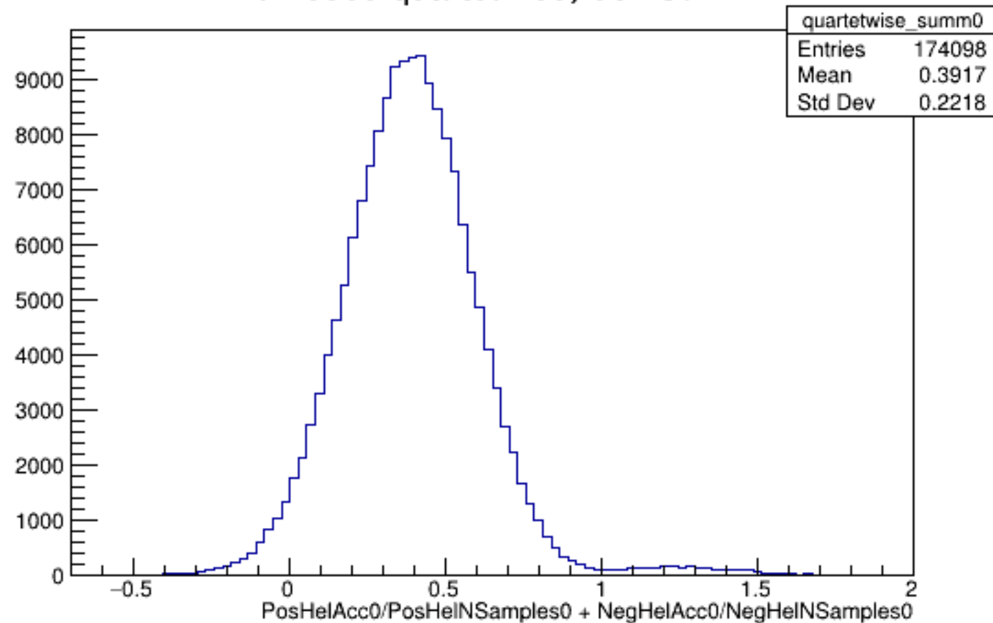
Run 5635 quartetwise, Sums0: All
