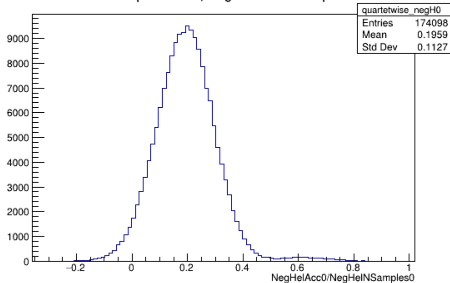
Run 5635 quartetwise, NegHelAcc0/NSamples0: All
