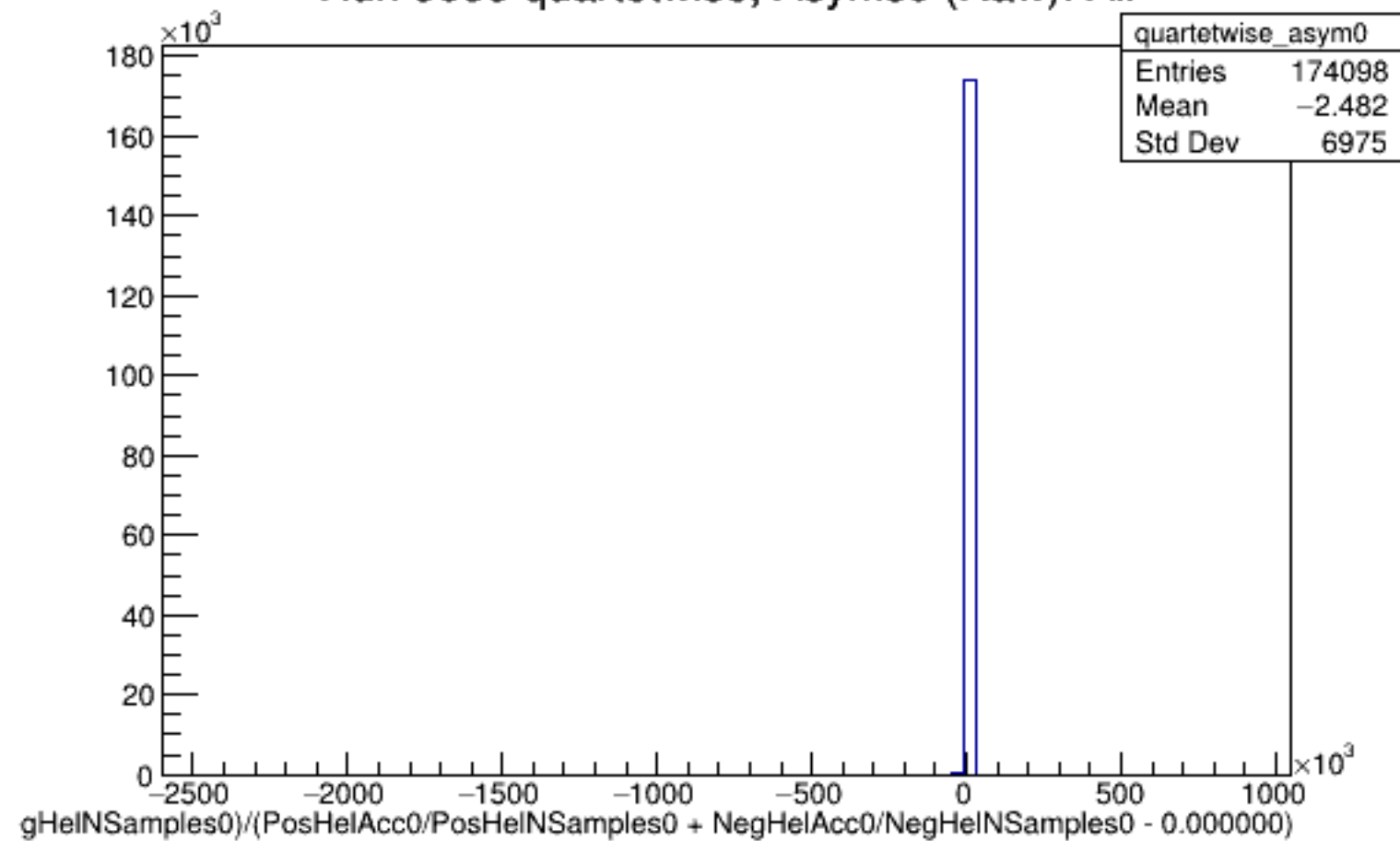
Run 5635 quartetwise, Asyms0 (Raw): All
