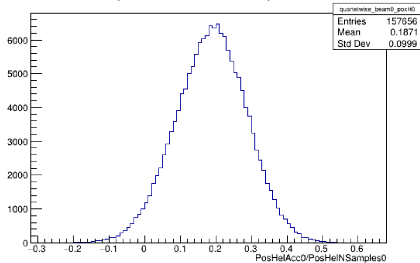
Run 5635 quartetwise, PosHelAcc0/NSamples0: Beam OFF
