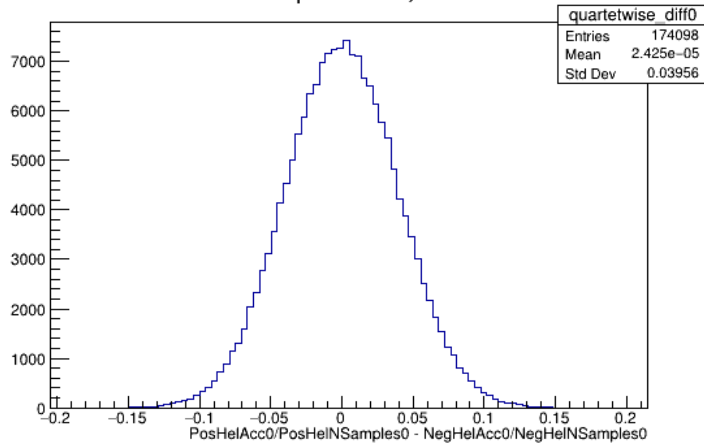
Run 5635 quartetwise, Diffs0: All
