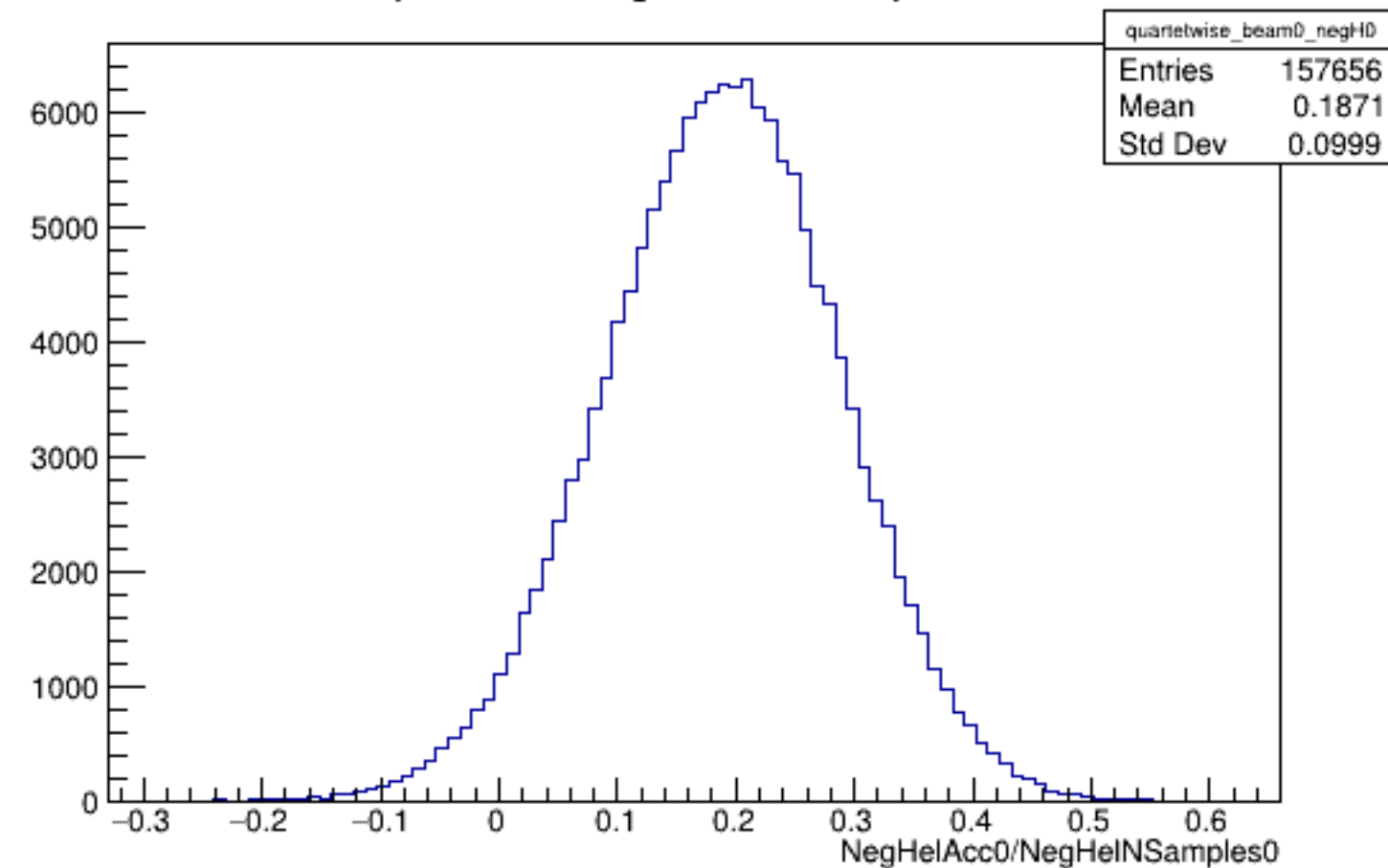
Run 5635 quartetwise, NegHelAcc0/NSamples0: Beam OFF
