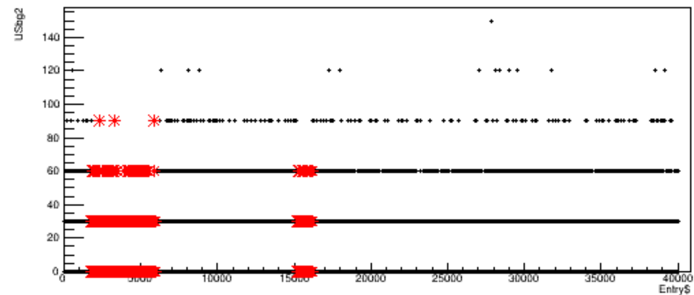
Run 5637, quartetwise: USbg2 vs time
