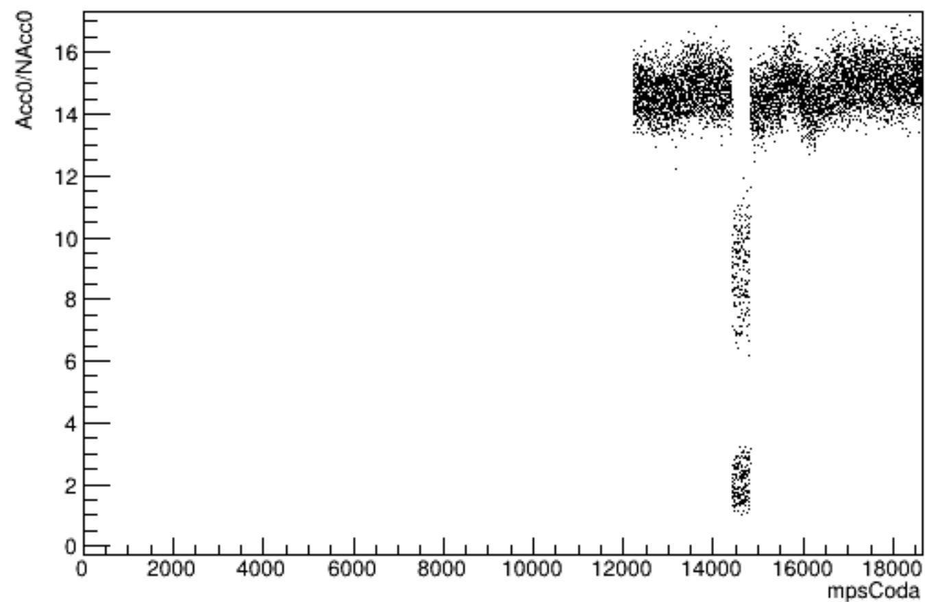
Run 5638 mpwise, Acc0 vs Time: Beam ON, Laser ON
