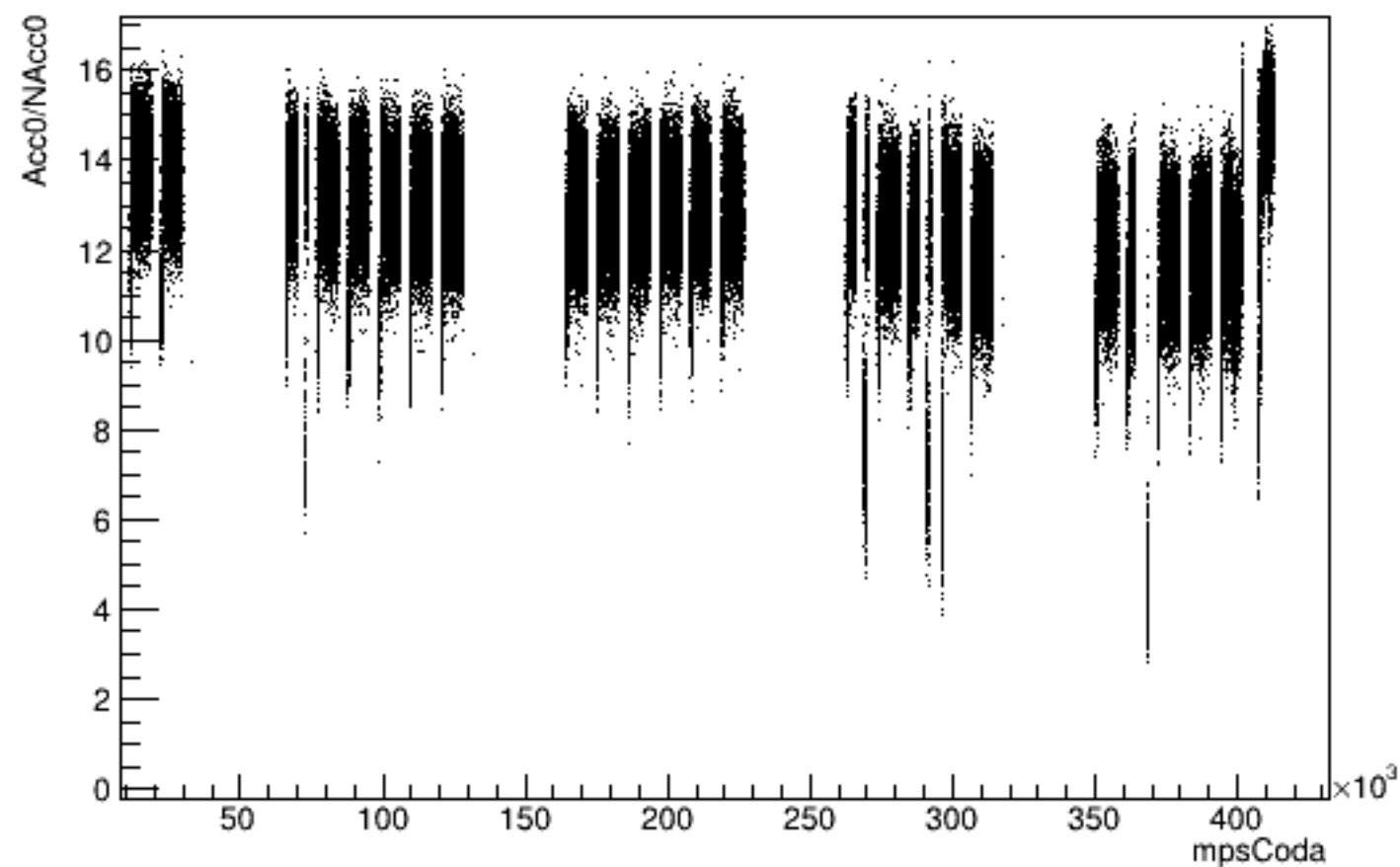
Run 5644 mpwise, Acc0 vs Time: Beam ON, Laser ON
