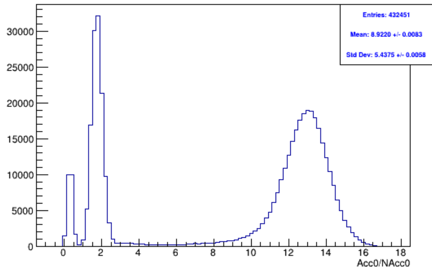
Run 5644 mpwise, acc0: All
