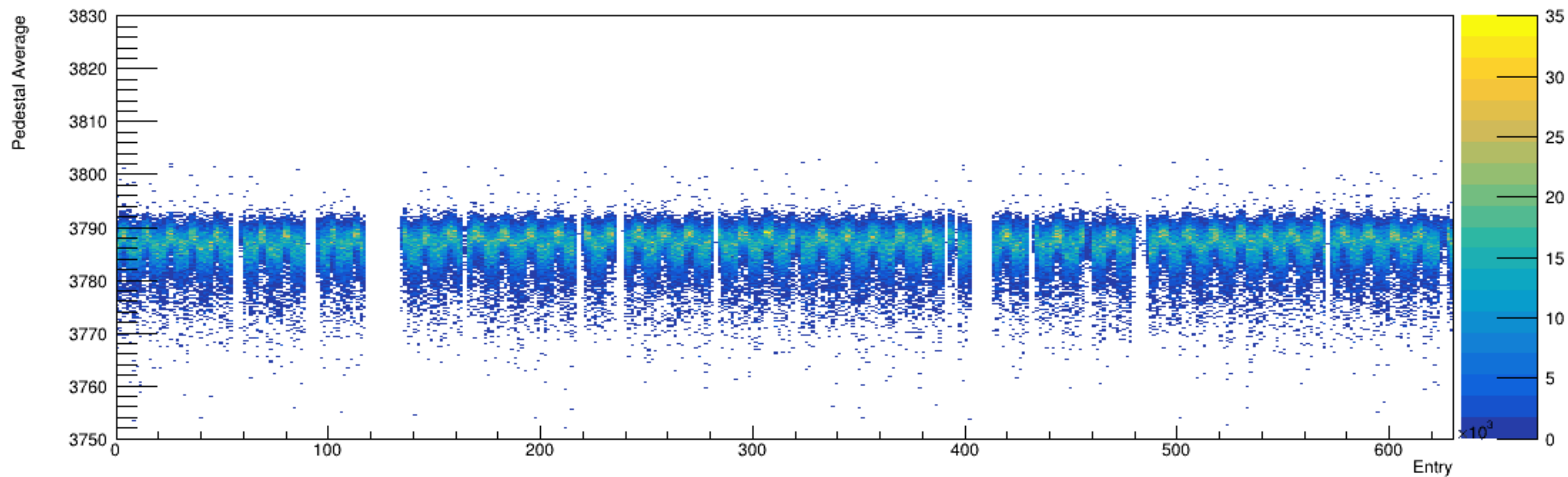
Run 5645, snapshots: Pedestal vs. Time
