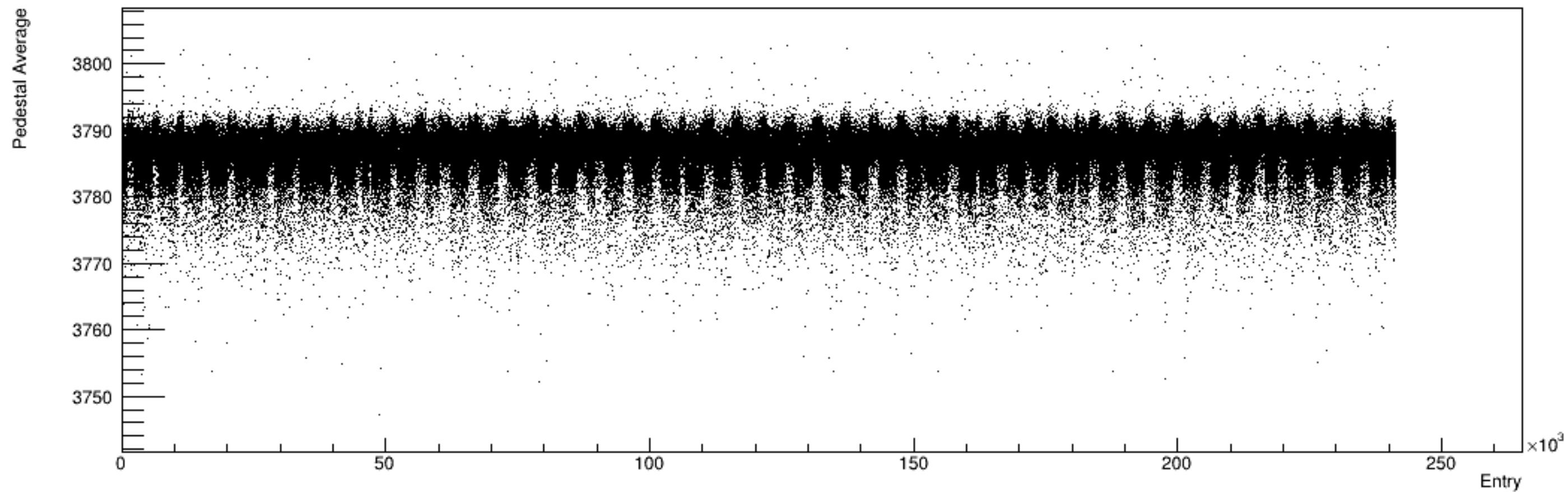
Run 5645, snapshots: Pedestal vs. Time
