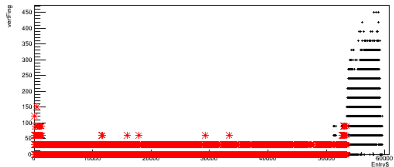
Run 5656, quartetwise: vertFing vs time
