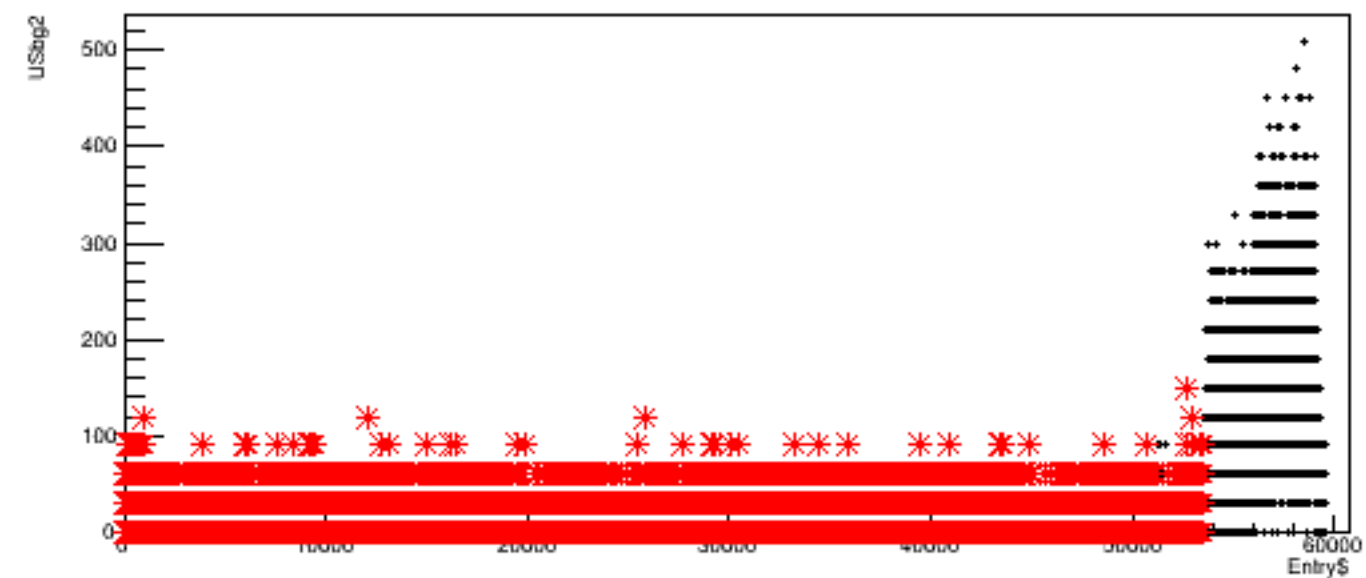
Run 5656, quartetwise: USbg2 vs time
