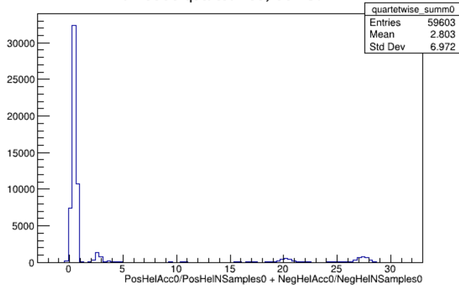
Run 5656 quartetwise, Sums0: All
