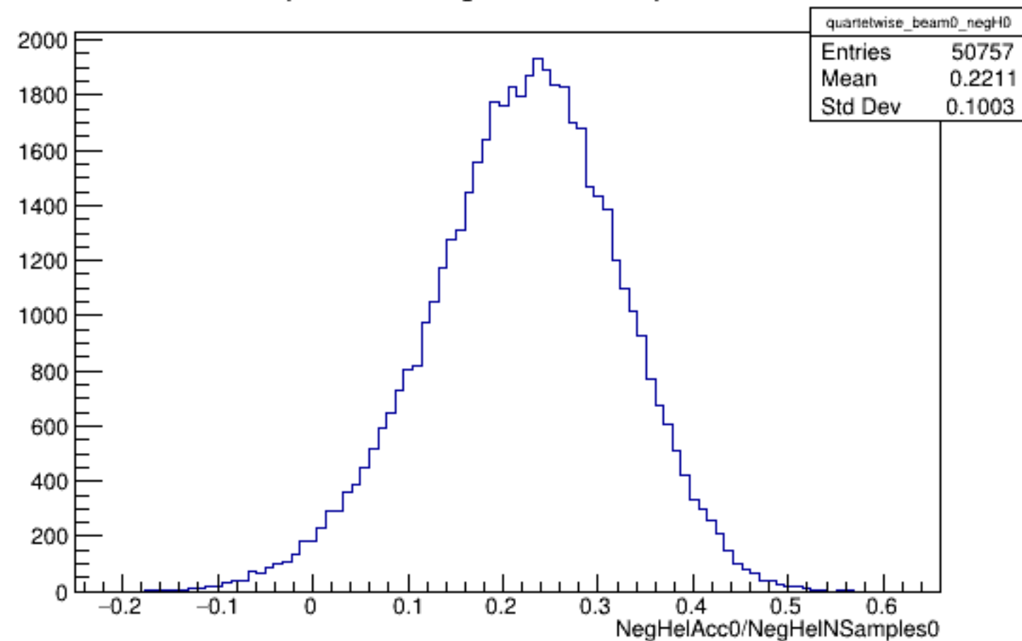
Run 5656 quartetwise, NegHelAcc0/NSamples0: Beam OFF
