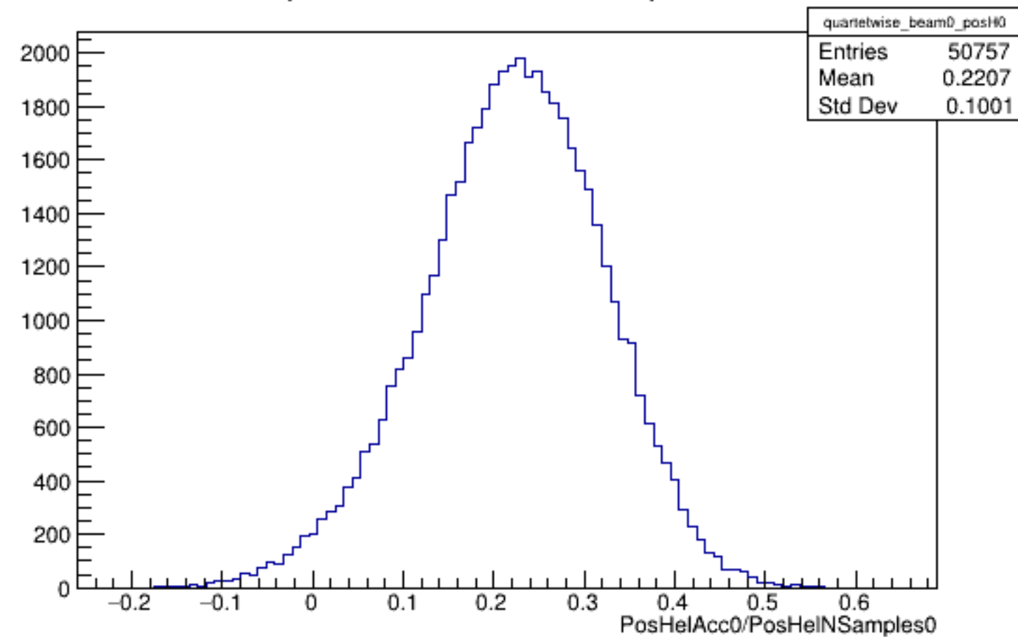
Run 5656 quartetwise, PosHelAcc0/NSamples0: Beam OFF
