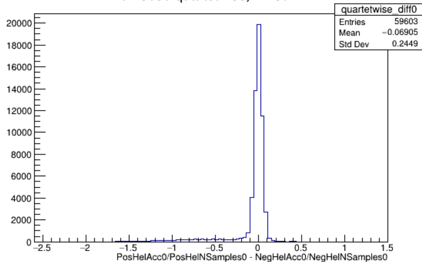
Run 5656 quartetwise, Diffs0: All
