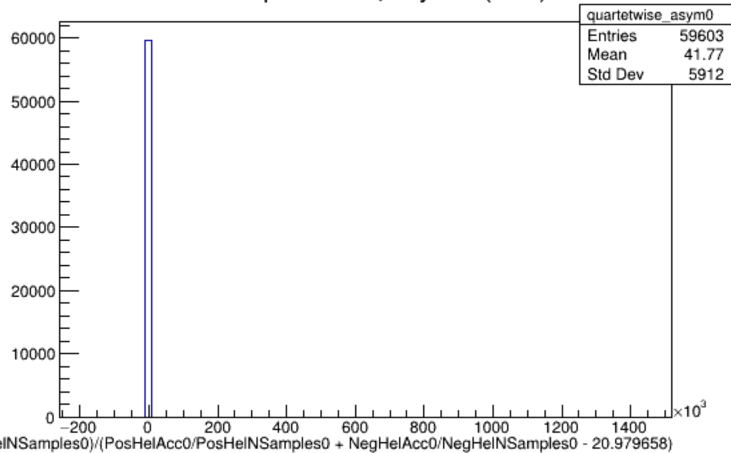
Run 5656 quartetwise, Asyms0 (Raw): All
