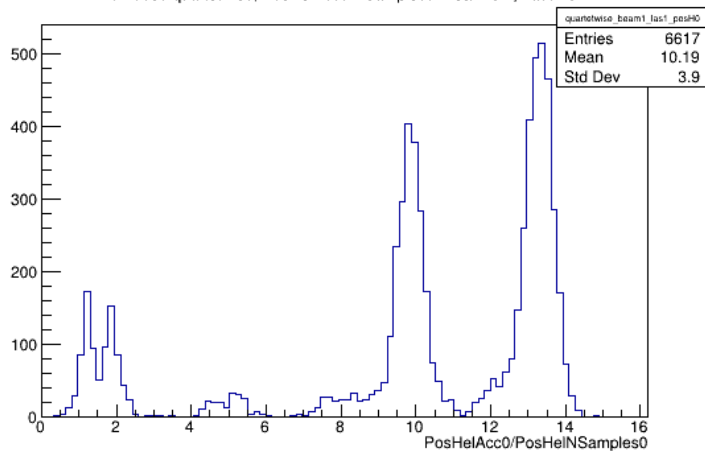
Run 5656 quartetwise, PosHelAcc0/NSamples0: Beam ON, Laser ON
