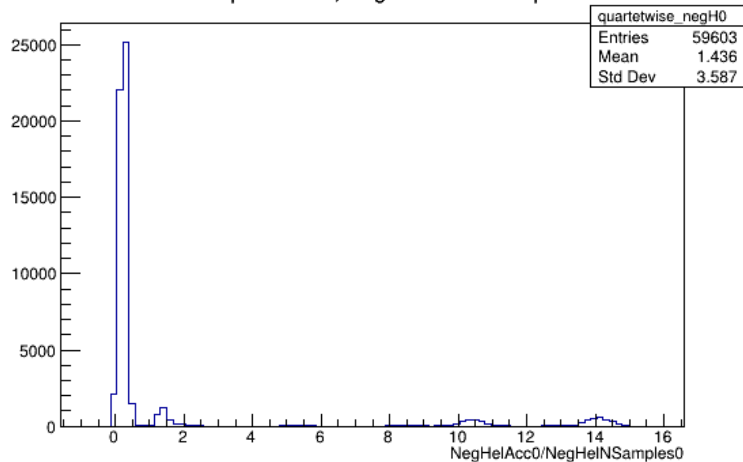
Run 5656 quartetwise, NegHelAcc0/NSamples0: All
