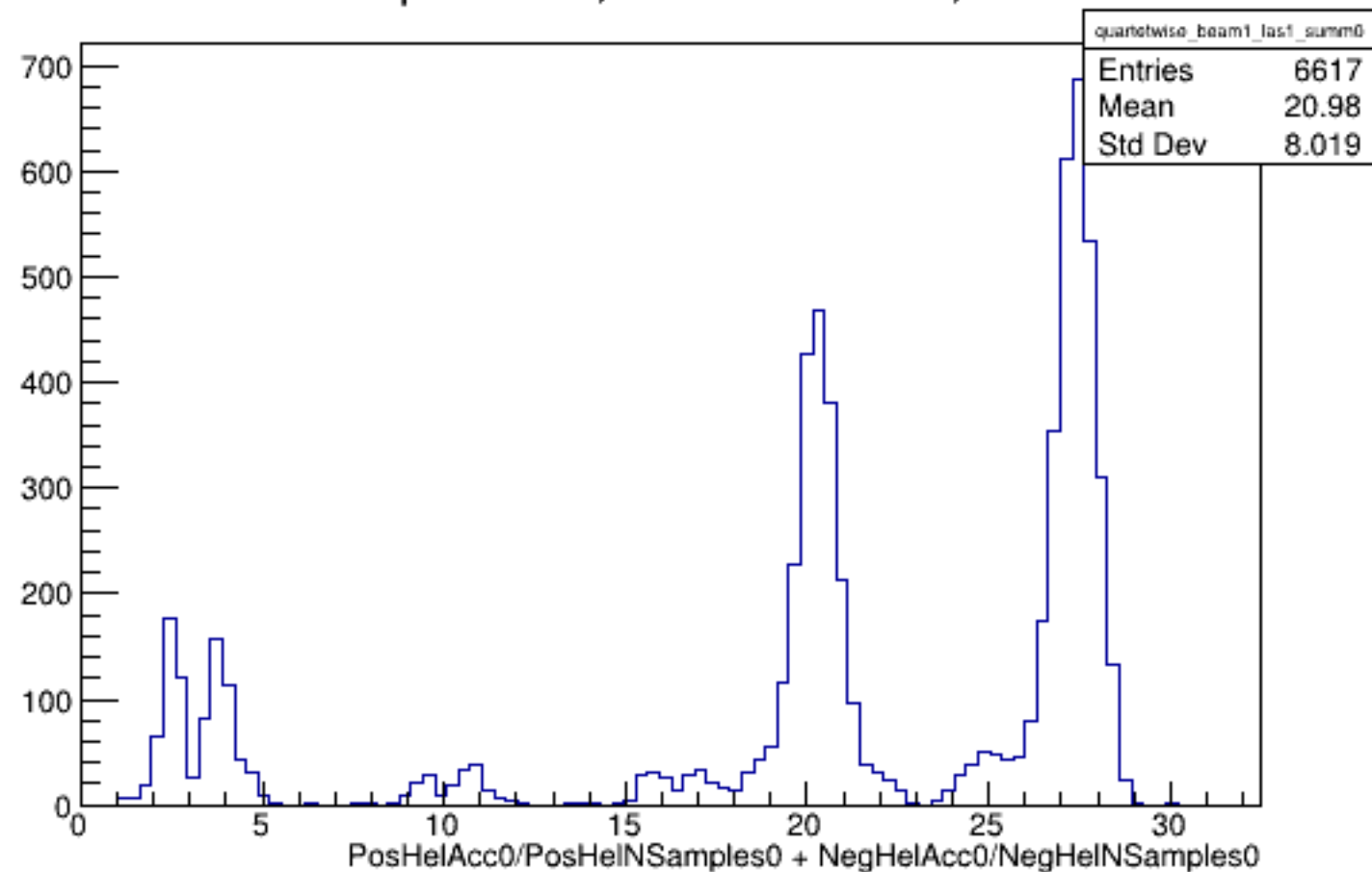
Run 5656 quartetwise, Sums0: Beam ON, Laser ON
