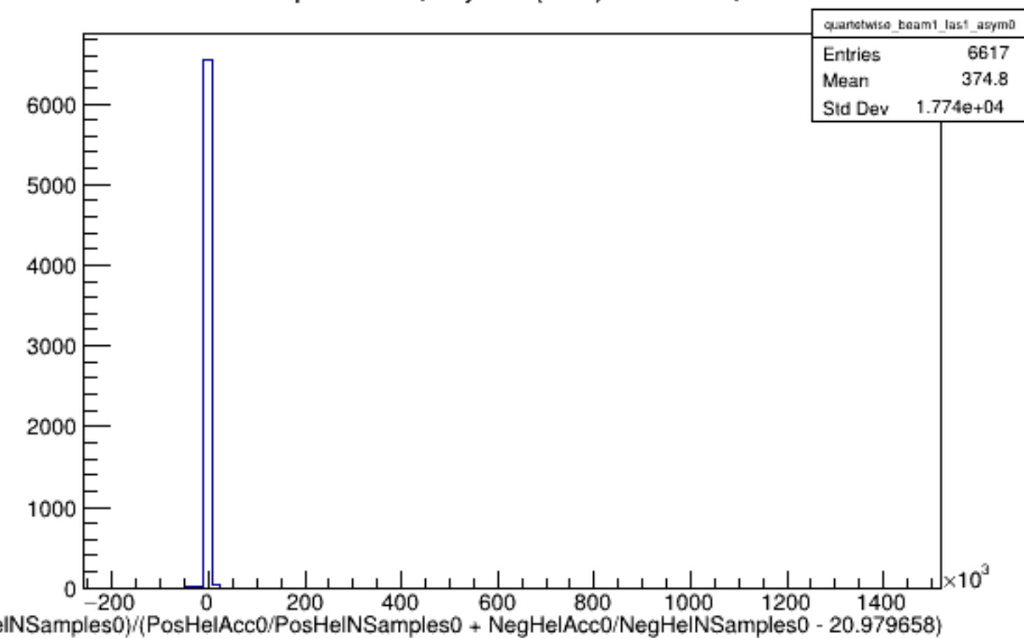
Run 5656 quartetwise, Asyms0 (Raw): Beam ON, Laser ON
