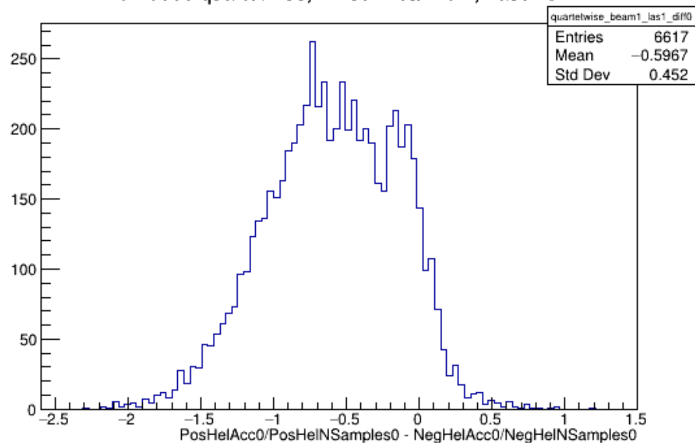
Run 5656 quartetwise, Diffs0: Beam ON, Laser ON
