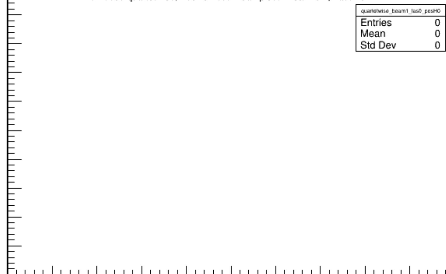
Run 5656 quartetwise, PosHelAcc0/NSamples0: Beam ON, Laser OFF
