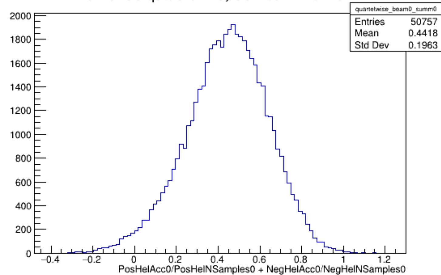
Run 5656 quartetwise, Sums0: Beam OFF
