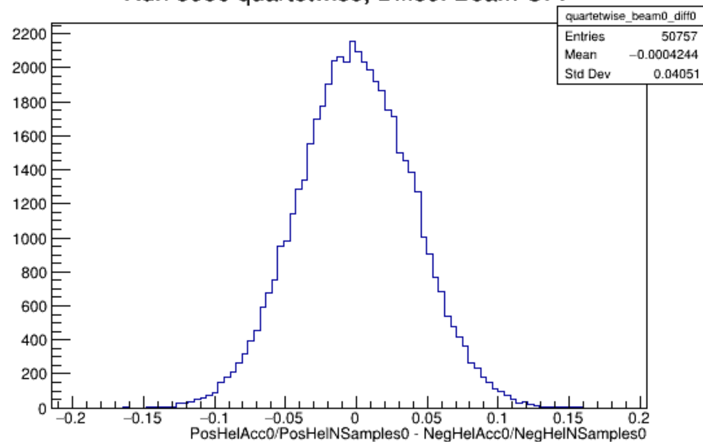
Run 5656 quartetwise, Diffs0: Beam OFF
