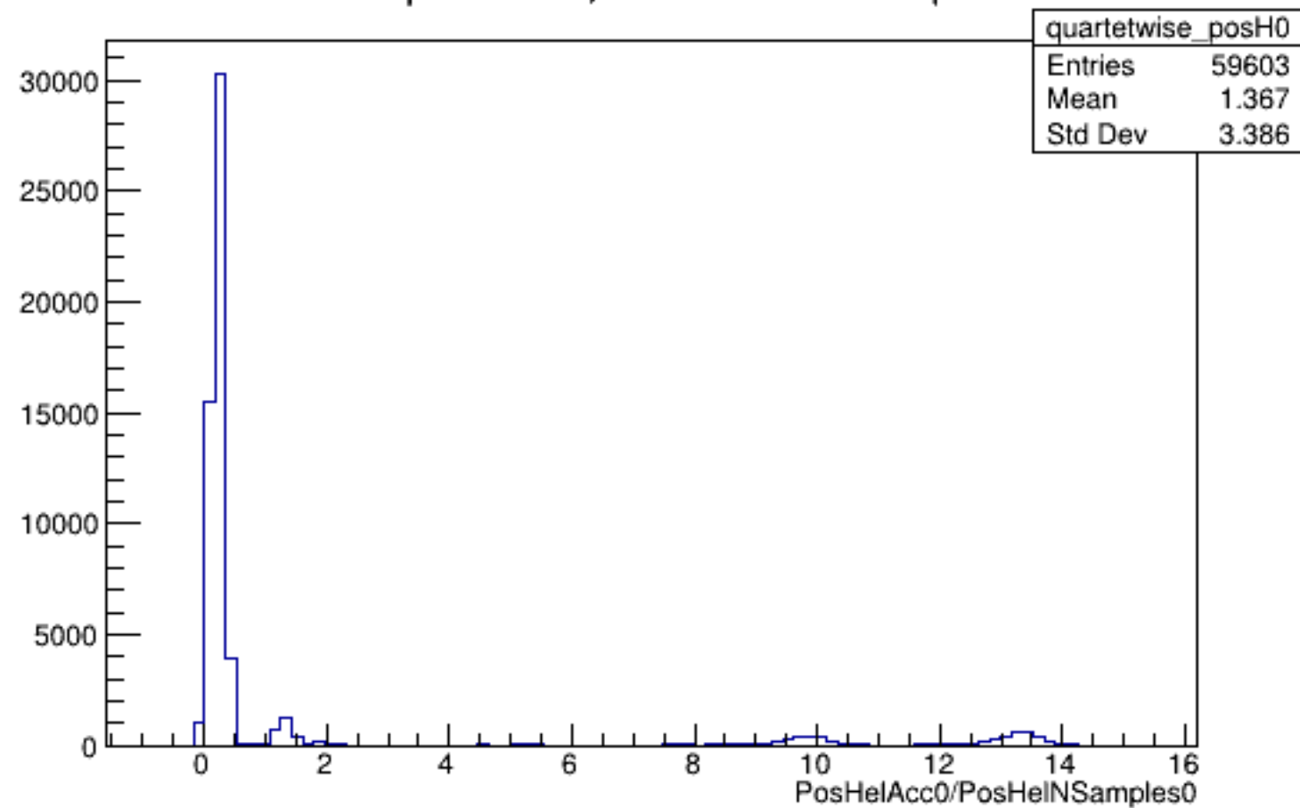
Run 5656 quartetwise, PosHelAcc0/NSamples0: All
