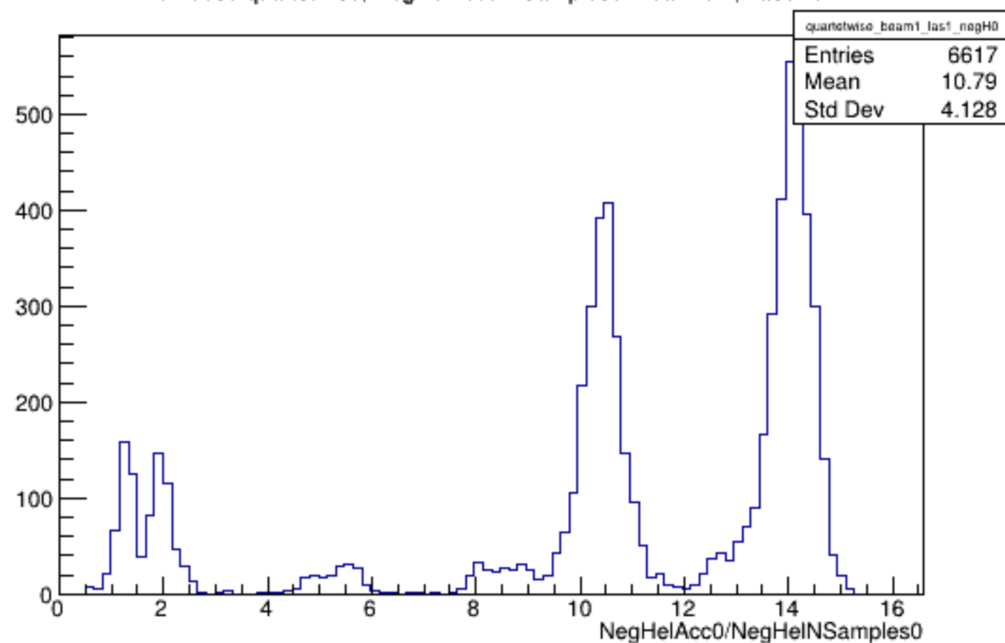
Run 5656 quartetwise, NegHelAcc0/NSamples0: Beam ON, Laser ON
