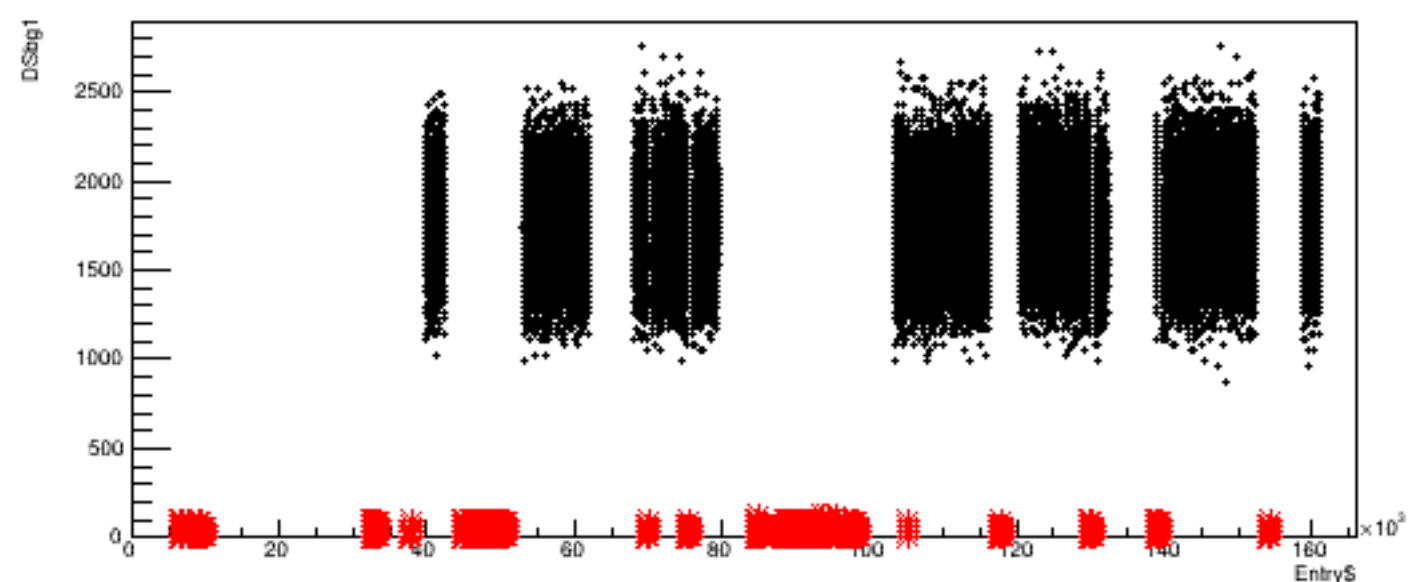
Run 5662, quartetwise: DSbg1 vs time
