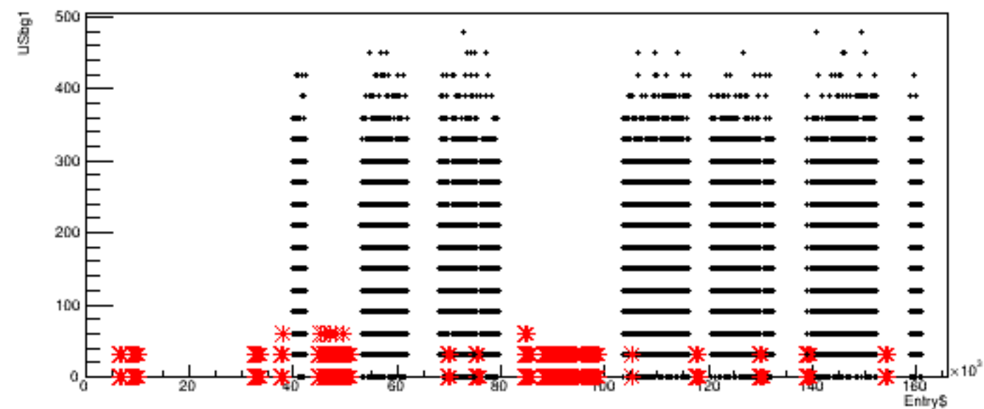
Run 5662, quartetwise: USbg1 vs time
