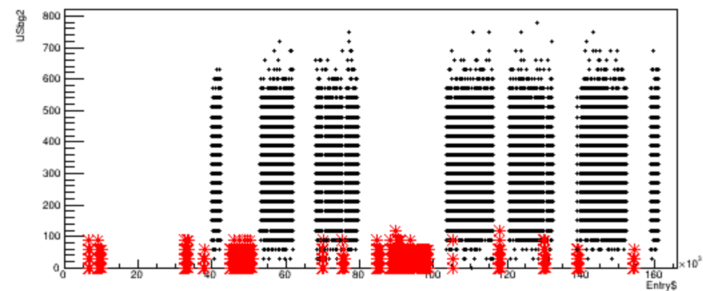
Run 5662, quartetwise: USbg2 vs time
