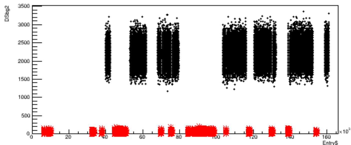
Run 5662, quartetwise: DSbg2 vs time
