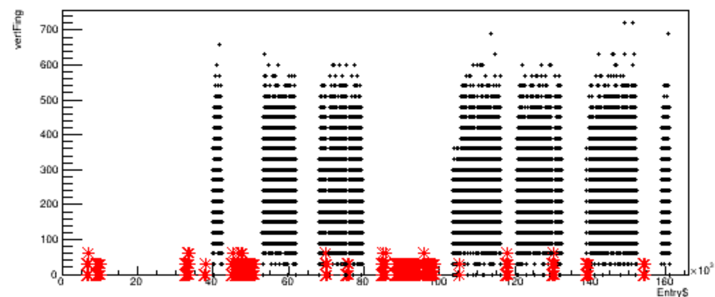
Run 5662, quartetwise: vertFing vs time
