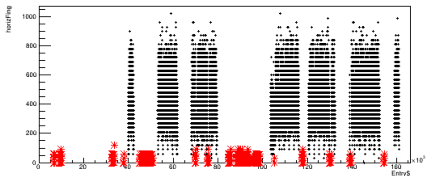
Run 5662, quartetwise: horizFing vs time
