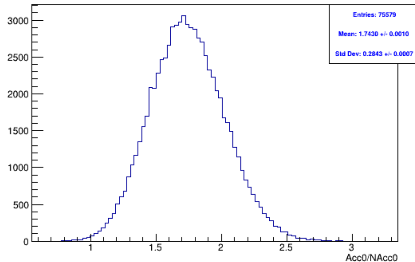
Run 5664, mpwise, acc0: Beam ON, Laser OFF
