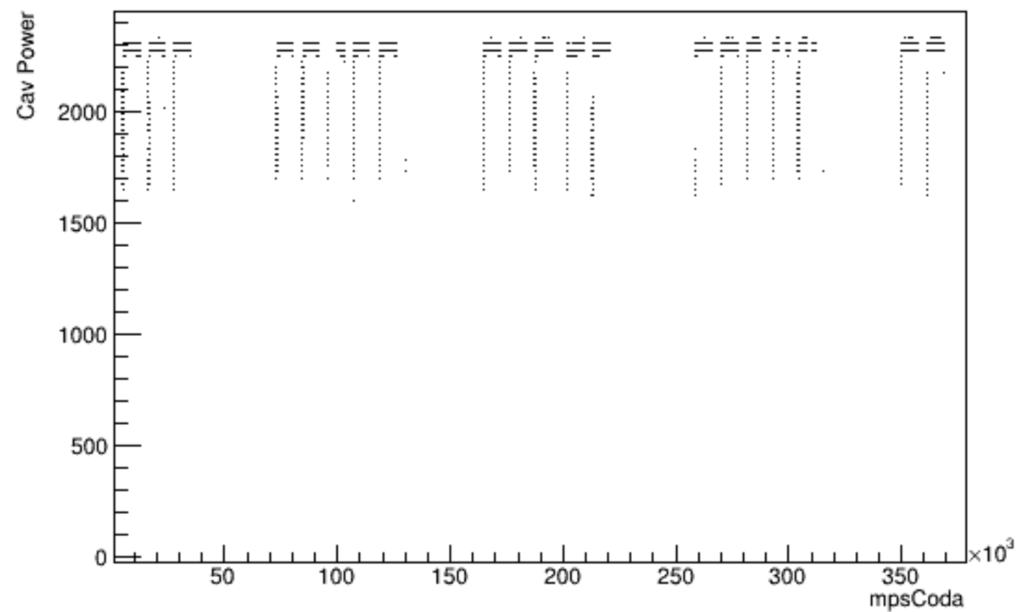
Run 5664 mpwise, beam ON, laser ON
