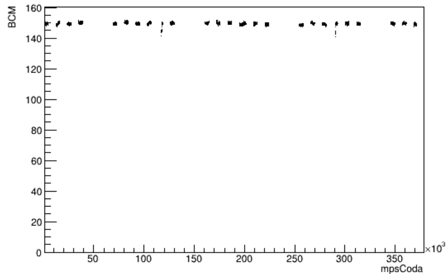
Run 5664 mpwise, beam ON, laser OFF
