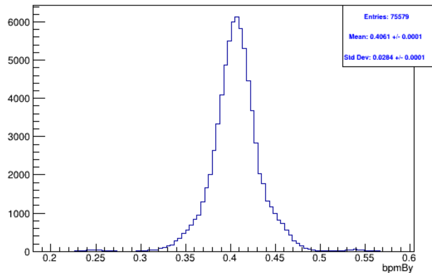
Run 5664, mpswise, bpmBy: Beam ON, Laser OFF
