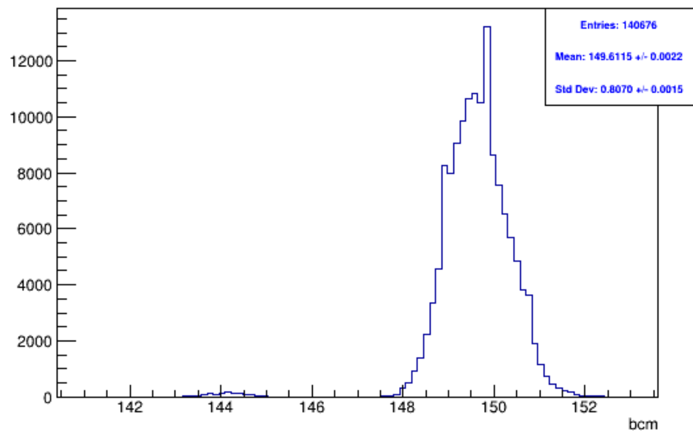
Run 5664, mpwise, BCM: Beam ON, Laser ON
