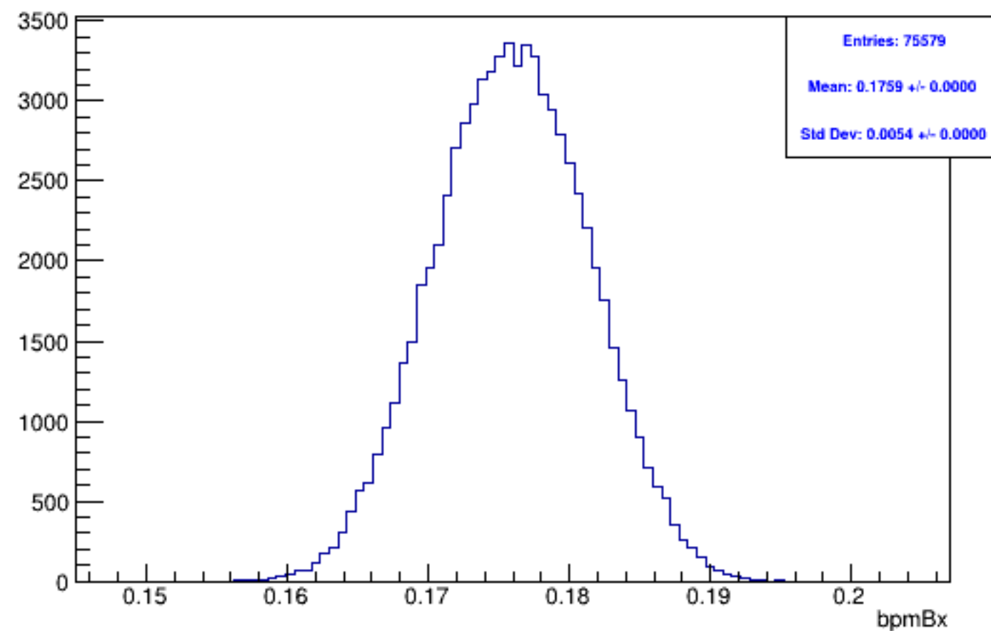
Run 5664, mpswise, bpmBx: Beam ON, Laser OFF
