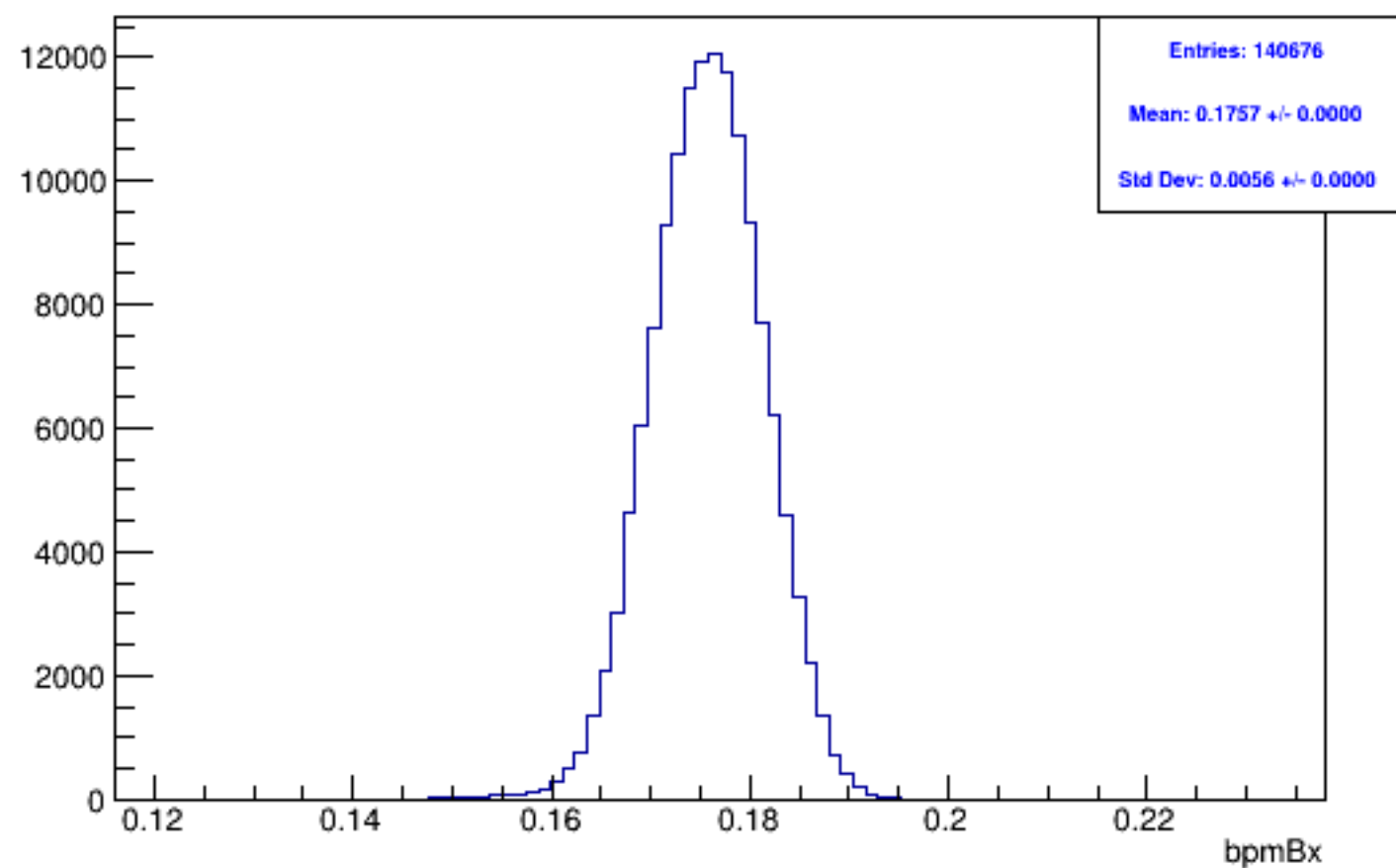
Run 5664, mpswise, bpmBx: Beam ON, Laser ON
