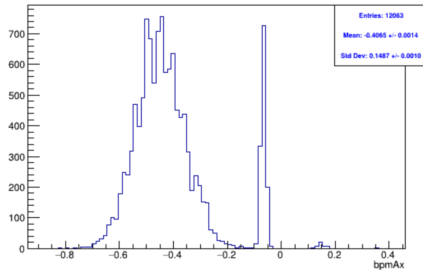
Run 5664 mpwise, bpmAx: Beam OFF
