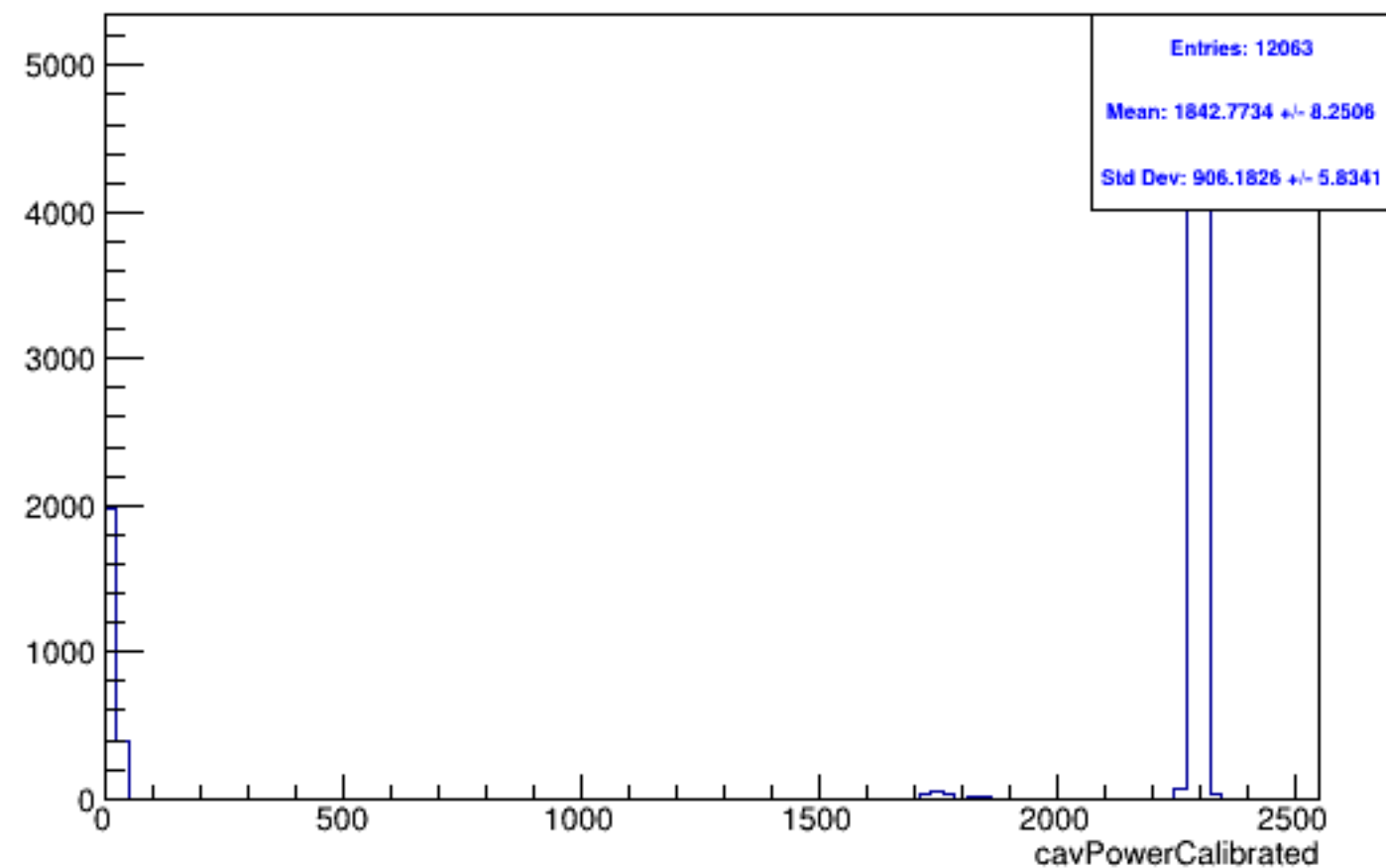
Run 5664 mpwise, lasPow: Beam OFF
