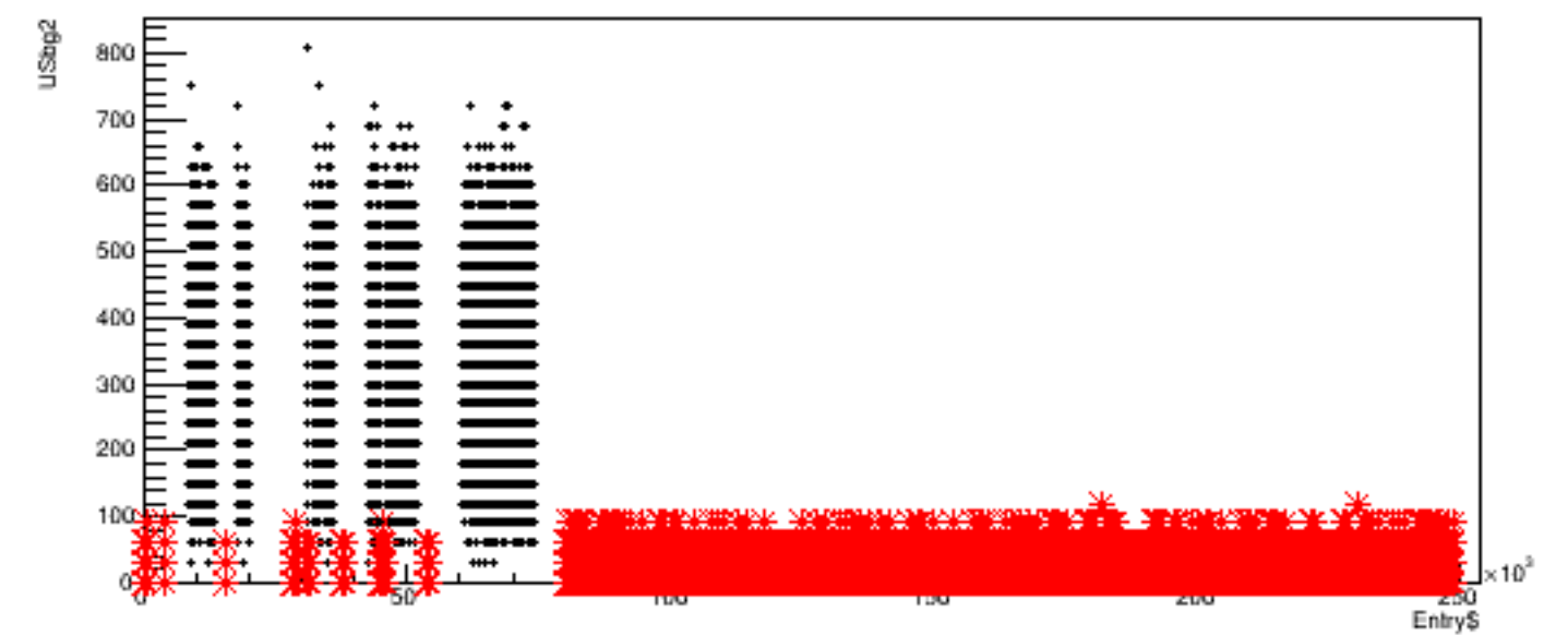
Run 5665, quartetwise: USbg2 vs time
