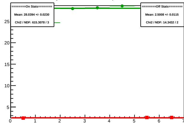
Cycle 5665.7: Multiplet Sums
