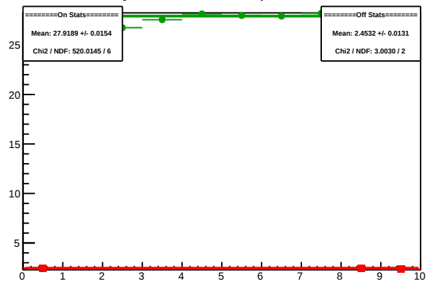
Cycle 5665.10: Multiplet Sums
