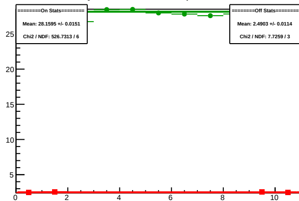
Cycle 5665.14: Multiplet Sums
