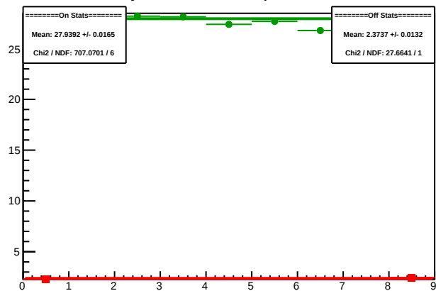
Cycle 5665.6: Multiplet Sums
