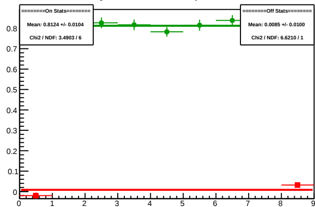
Cycle 5665.3: Multiplet Diffs
