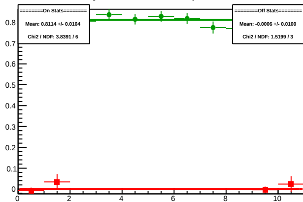
Cycle 5665.14: Multiplet Diffs
