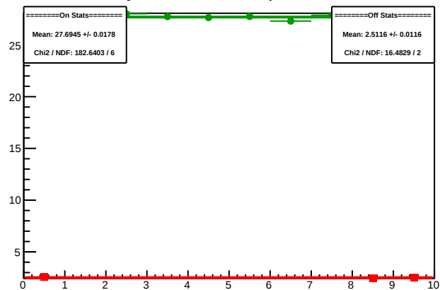
Cycle 5665.13: Multiplet Sums
