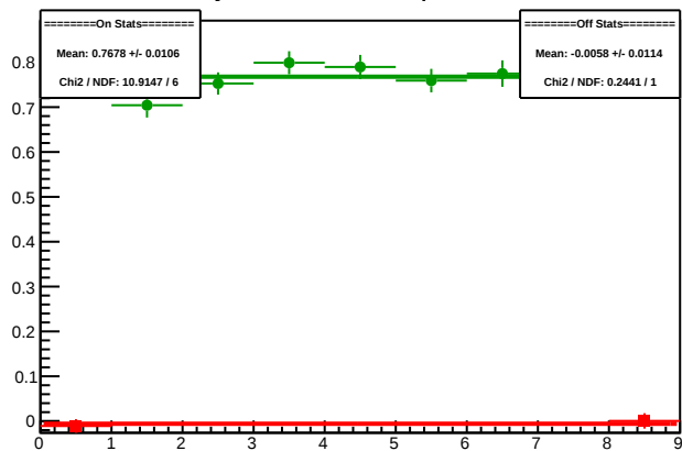
Cycle 5665.6: Multiplet Diffs
