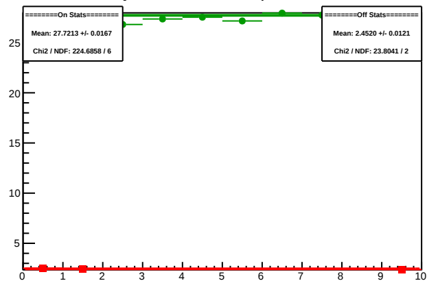
Cycle 5665.15: Multiplet Sums
