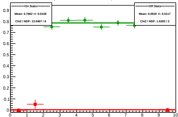
Cycle 5665.15: Multiplet Diffs
