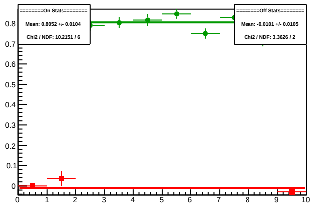
Cycle 5665.11: Multiplet Diffs
