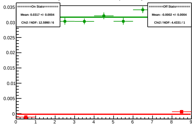
Cycle 5665.12: Multiplet Asyms
