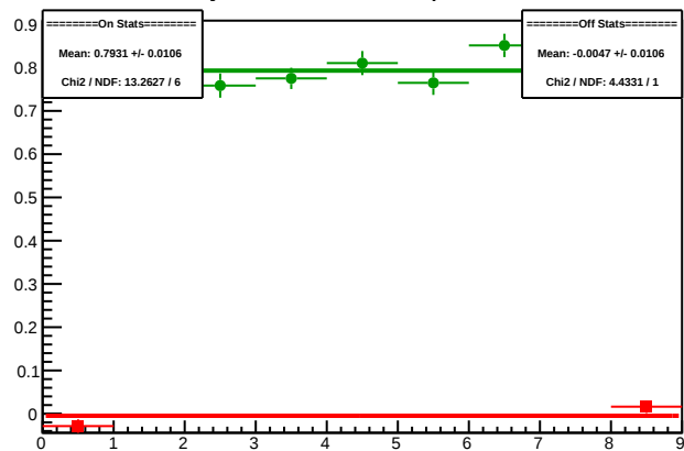
Cycle 5665.12: Multiplet Diffs
