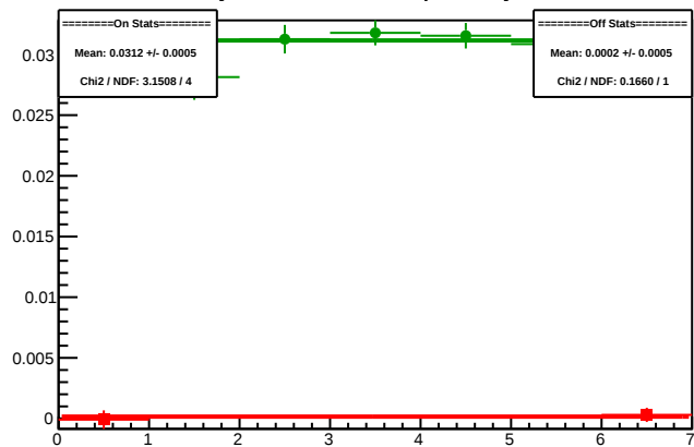
Cycle 5665.4: Multiplet Asyms
