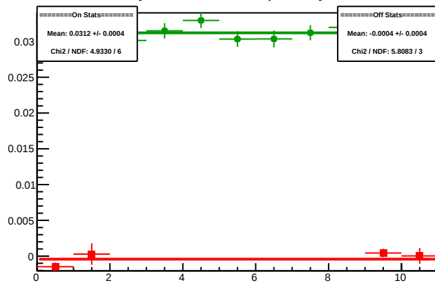
Cycle 5665.9: Multiplet Asyms
