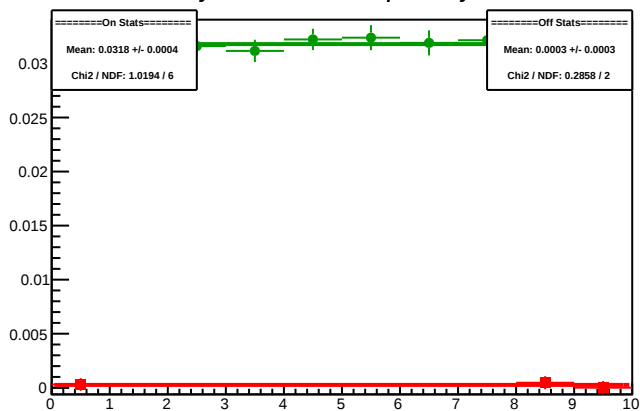
Cycle 5665.5: Multiplet Asyms
