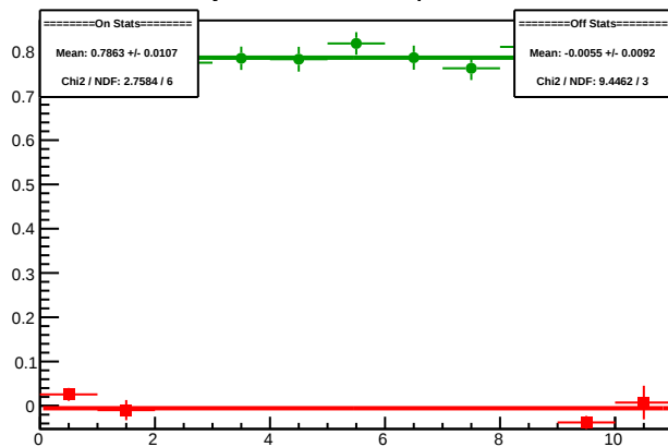
Cycle 5665.8: Multiplet Diffs
