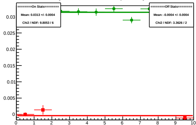
Cycle 5665.11: Multiplet Asyms
