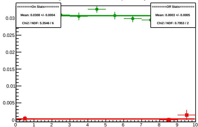
Cycle 5665.10: Multiplet Asyms
