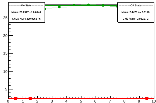
Cycle 5665.11: Multiplet Sums
