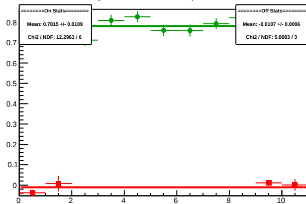
Cycle 5665.9: Multiplet Diffs
