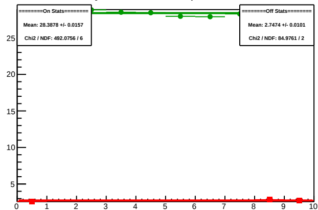
Cycle 5665.5: Multiplet Sums
