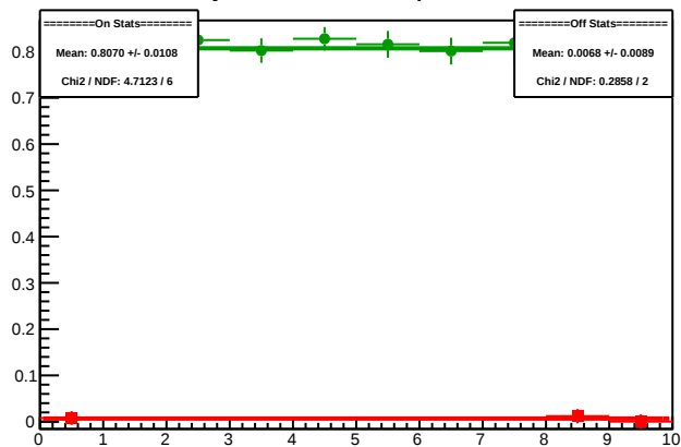
Cycle 5665.5: Multiplet Diffs
