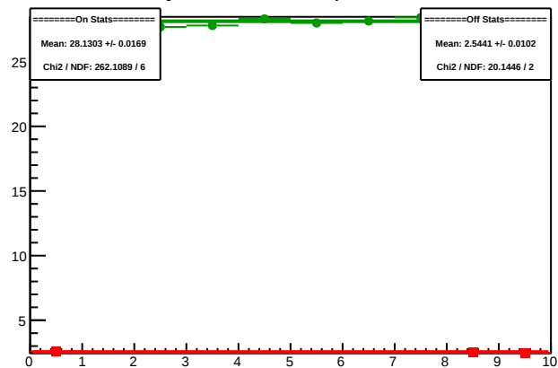
Cycle 5665.2: Multiplet Sums
