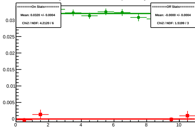
Cycle 5665.14: Multiplet Asyms
