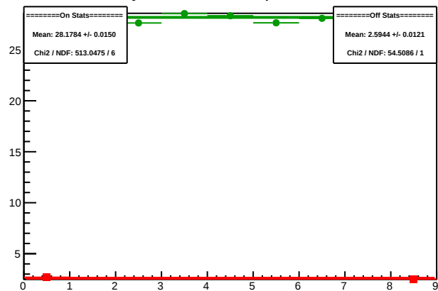
Cycle 5665.3: Multiplet Sums
