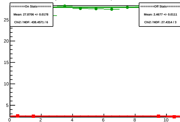
Cycle 5665.9: Multiplet Sums
