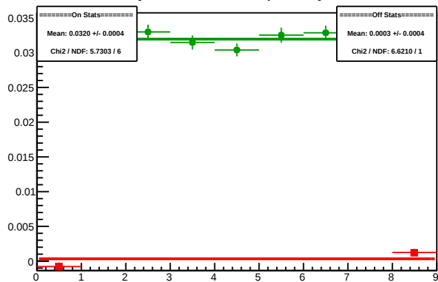
Cycle 5665.3: Multiplet Asyms
