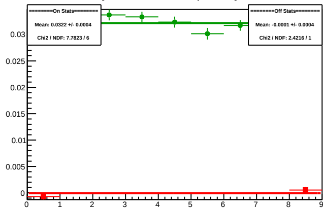
Cycle 5665.1: Multiplet Asyms
