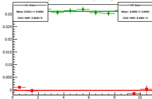
Cycle 5665.8: Multiplet Asyms
