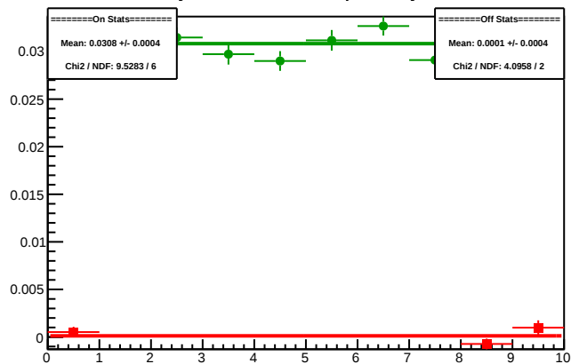
Cycle 5665.2: Multiplet Asyms
