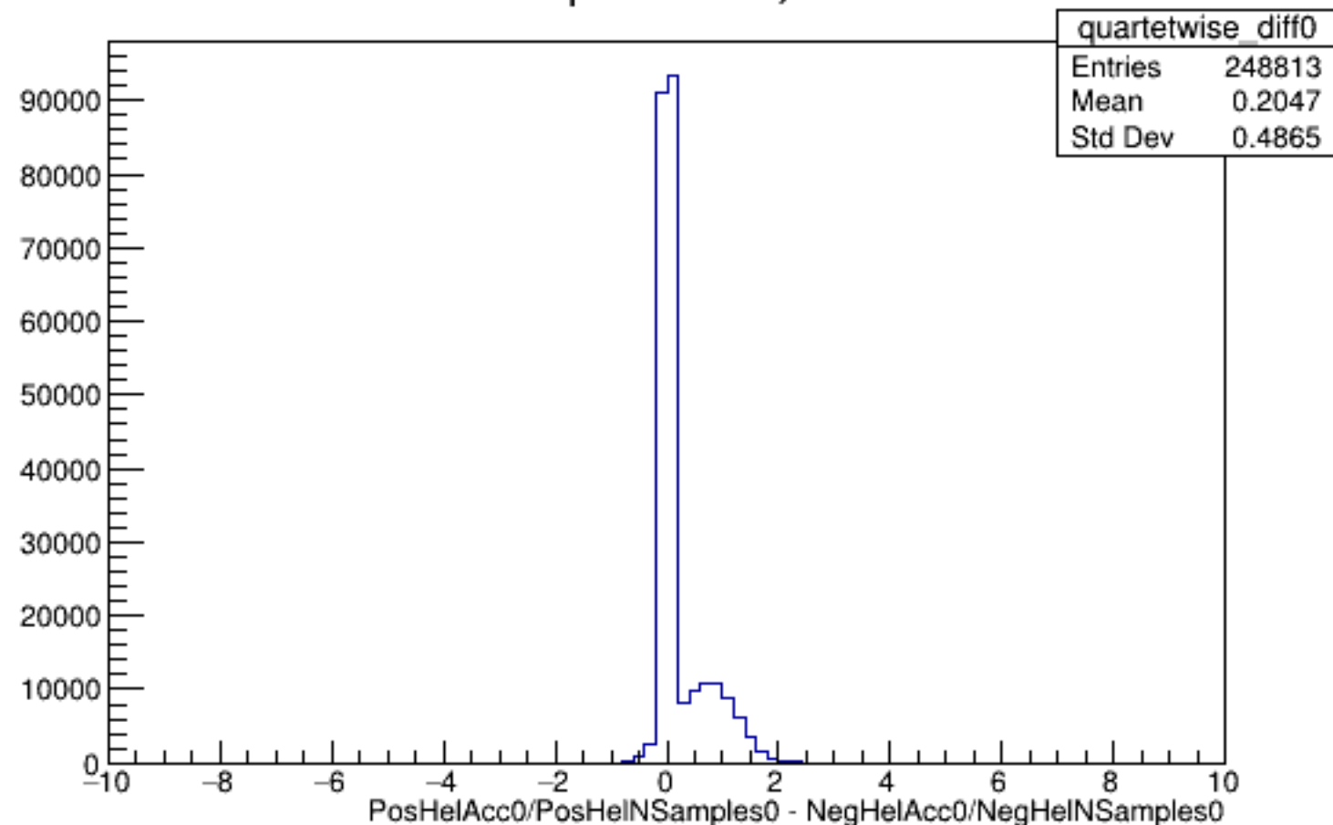
Run 5665 quartetwise, Diffs0: All
