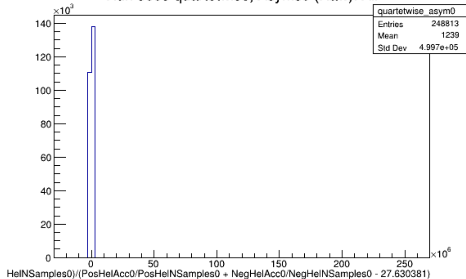
Run 5665 quartetwise, Asyms0 (Raw): All
