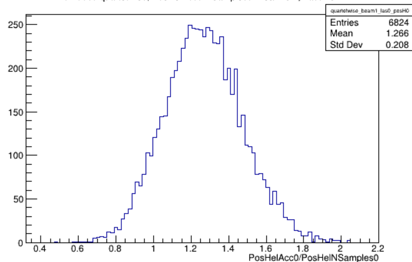
Run 5665 quartetwise, PosHelAcc0/NSamples0: Beam ON, Laser OFF
