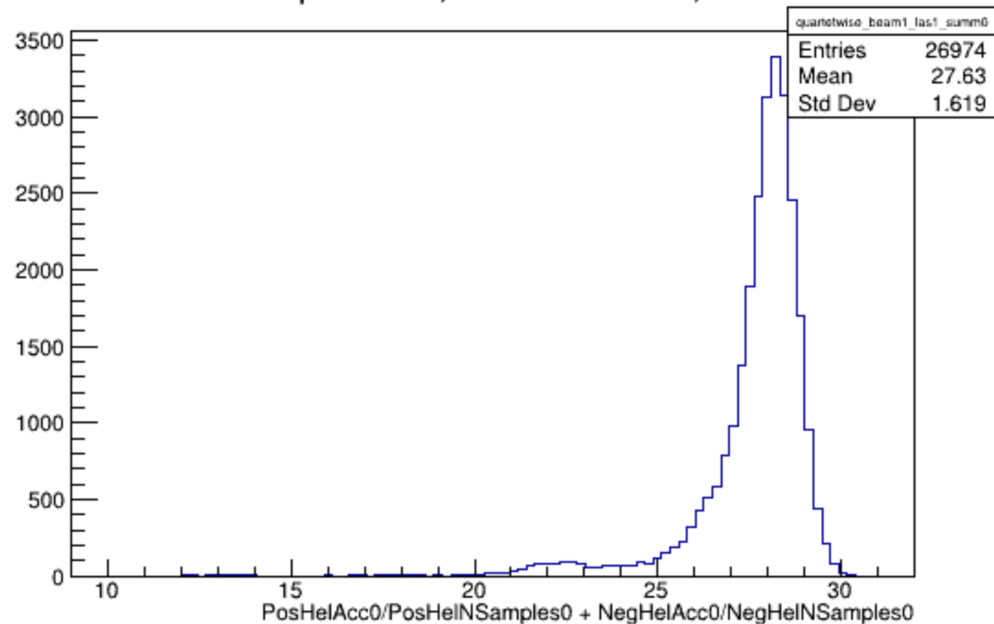
Run 5665 quartetwise, Sums0: Beam ON, Laser ON
