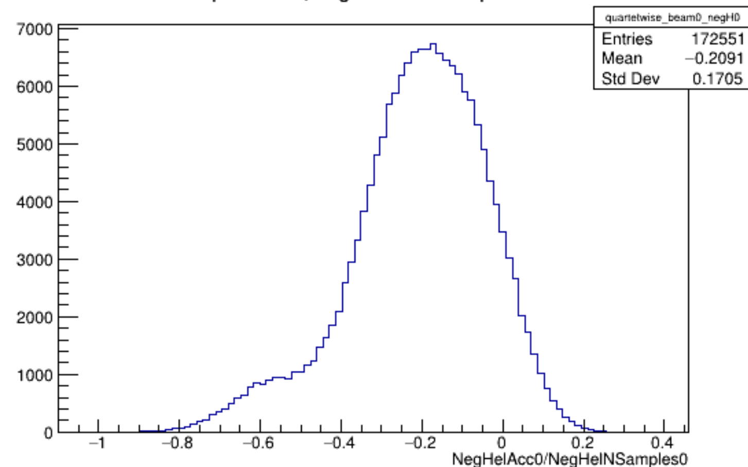
Run 5665 quartetwise, NegHelAcc0/NSamples0: Beam OFF
