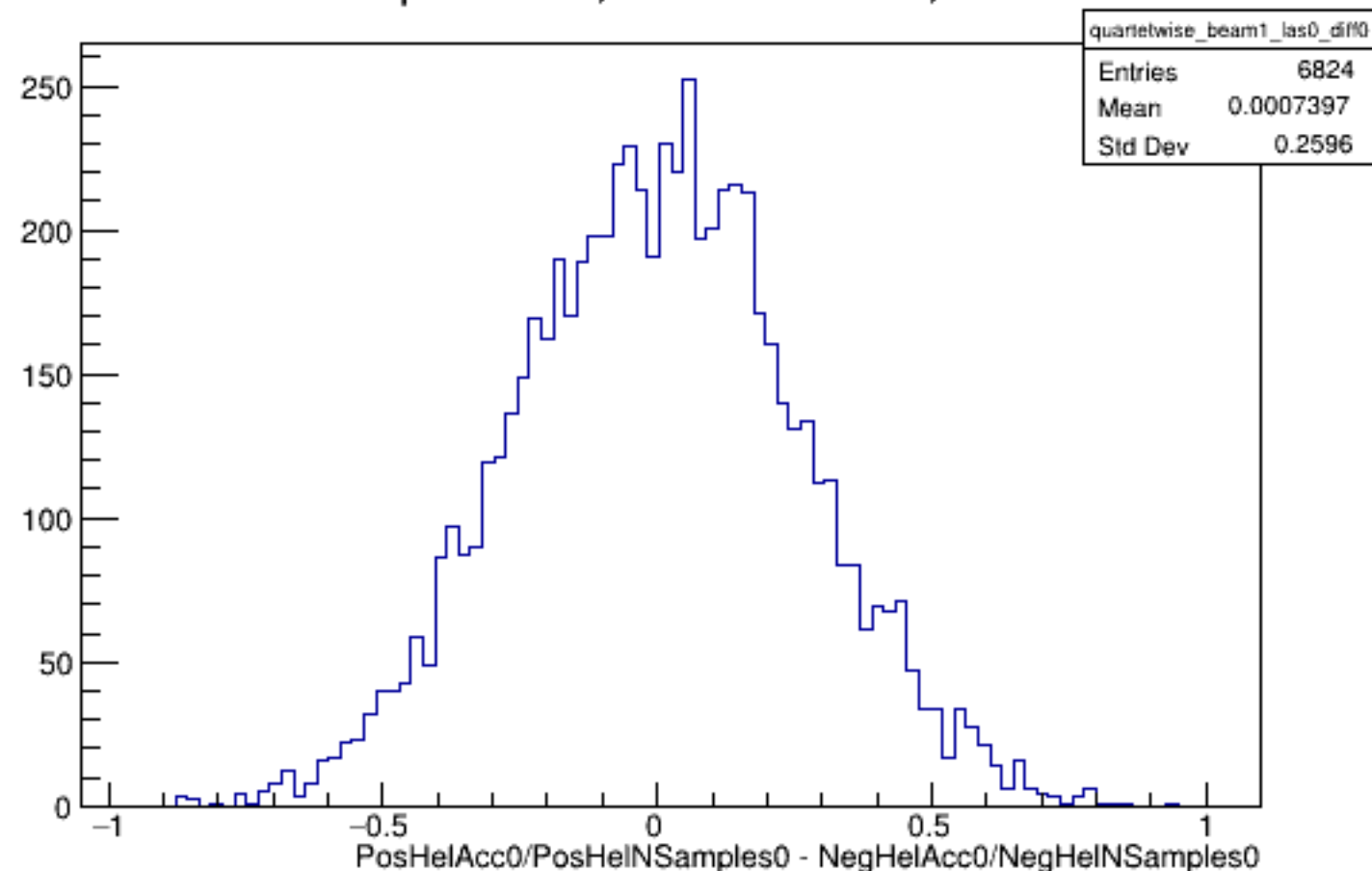
Run 5665 quartetwise, Diffs0: Beam ON, Laser OFF
