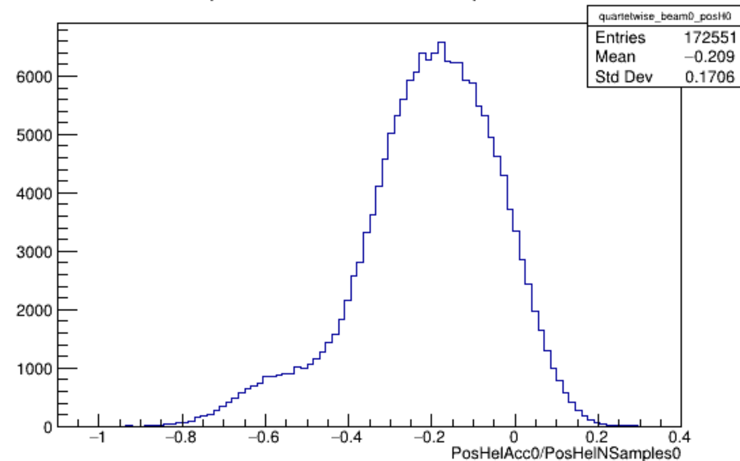
Run 5665 quartetwise, PosHelAcc0/NSamples0: Beam OFF
