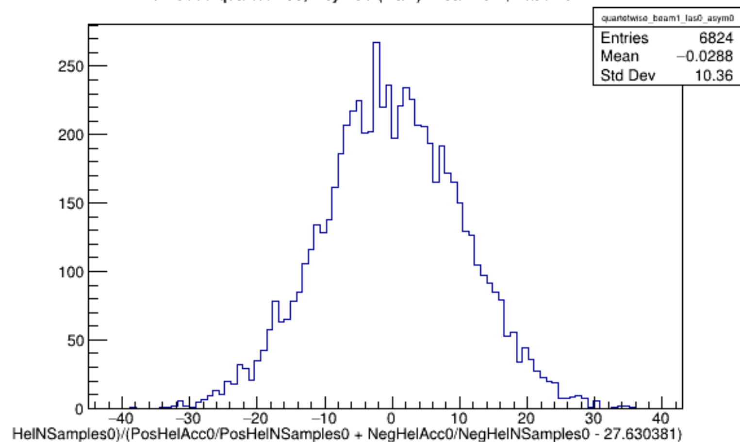
Run 5665 quartetwise, Asyms0 (Raw): Beam ON, Laser OFF
