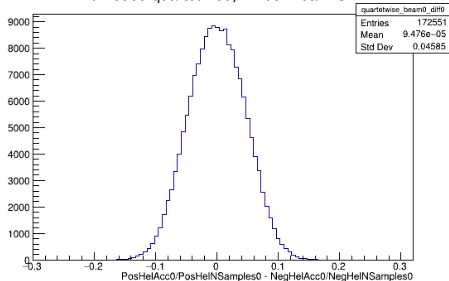
Run 5665 quartetwise, Diffs0: Beam OFF
