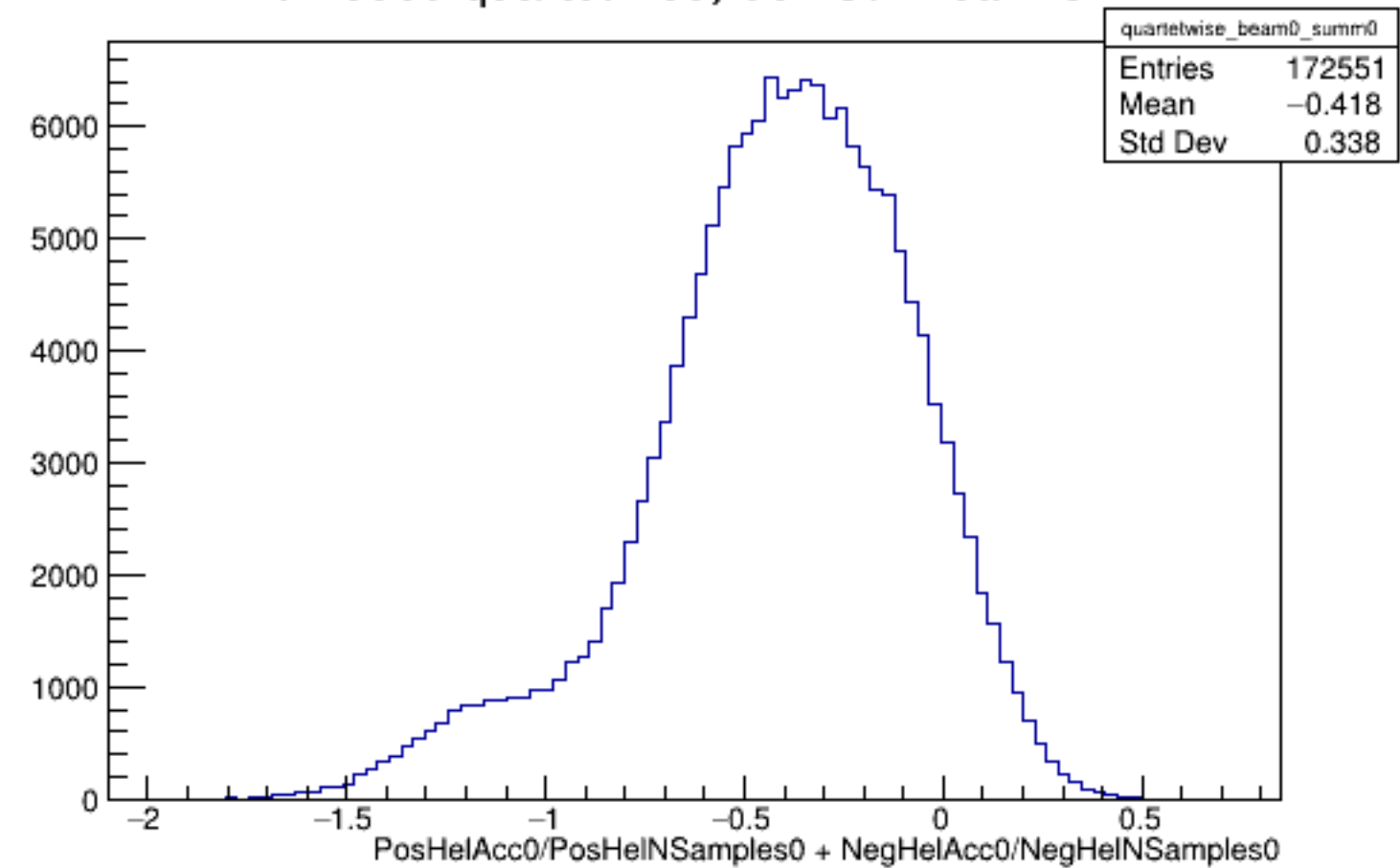
Run 5665 quartetwise, Sums0: Beam OFF
