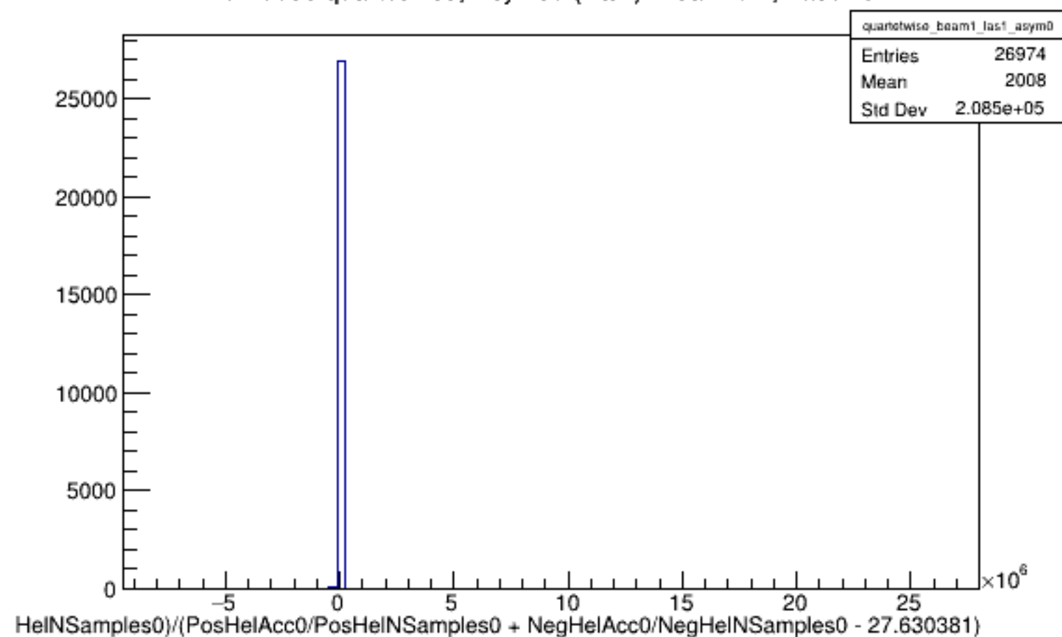
Run 5665 quartetwise, Asyms0 (Raw): Beam ON, Laser ON
