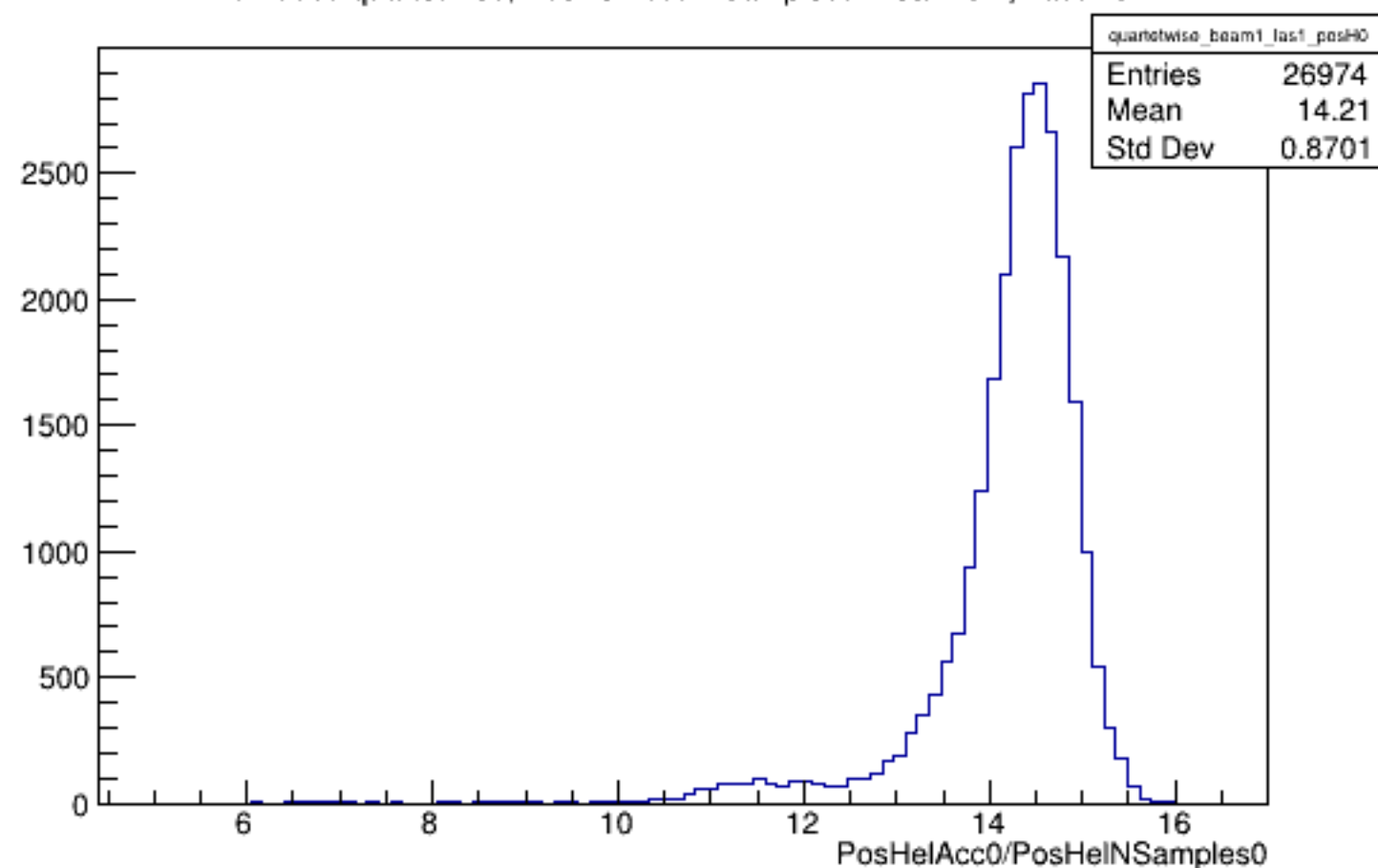
Run 5665 quartetwise, PosHelAcc0/NSamples0: Beam ON, Laser ON
