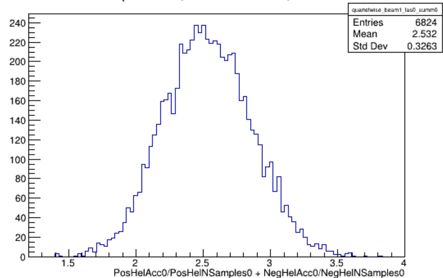
Run 5665 quartetwise, Sums0: Beam ON, Laser OFF
