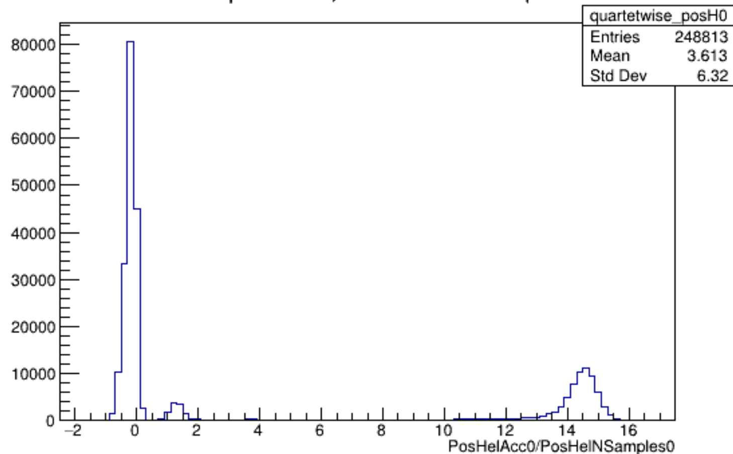
Run 5665 quartetwise, PosHelAcc0/NSamples0: All
