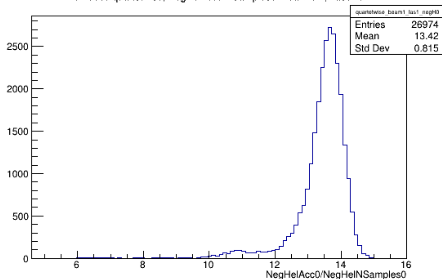
Run 5665 quartetwise, NegHelAcc0/NSamples0: Beam ON, Laser ON
