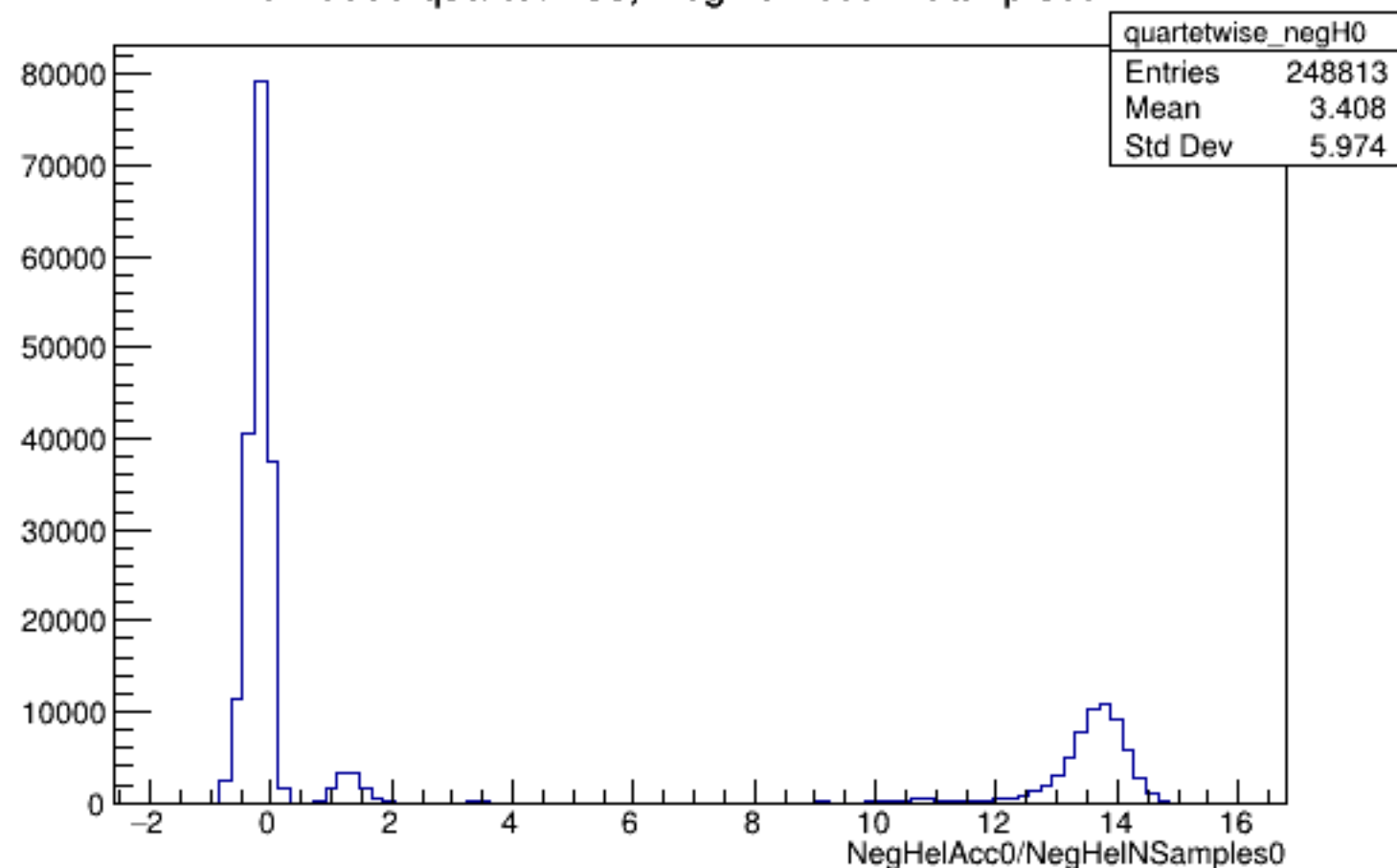
Run 5665 quartetwise, NegHelAcc0/NSamples0: All
