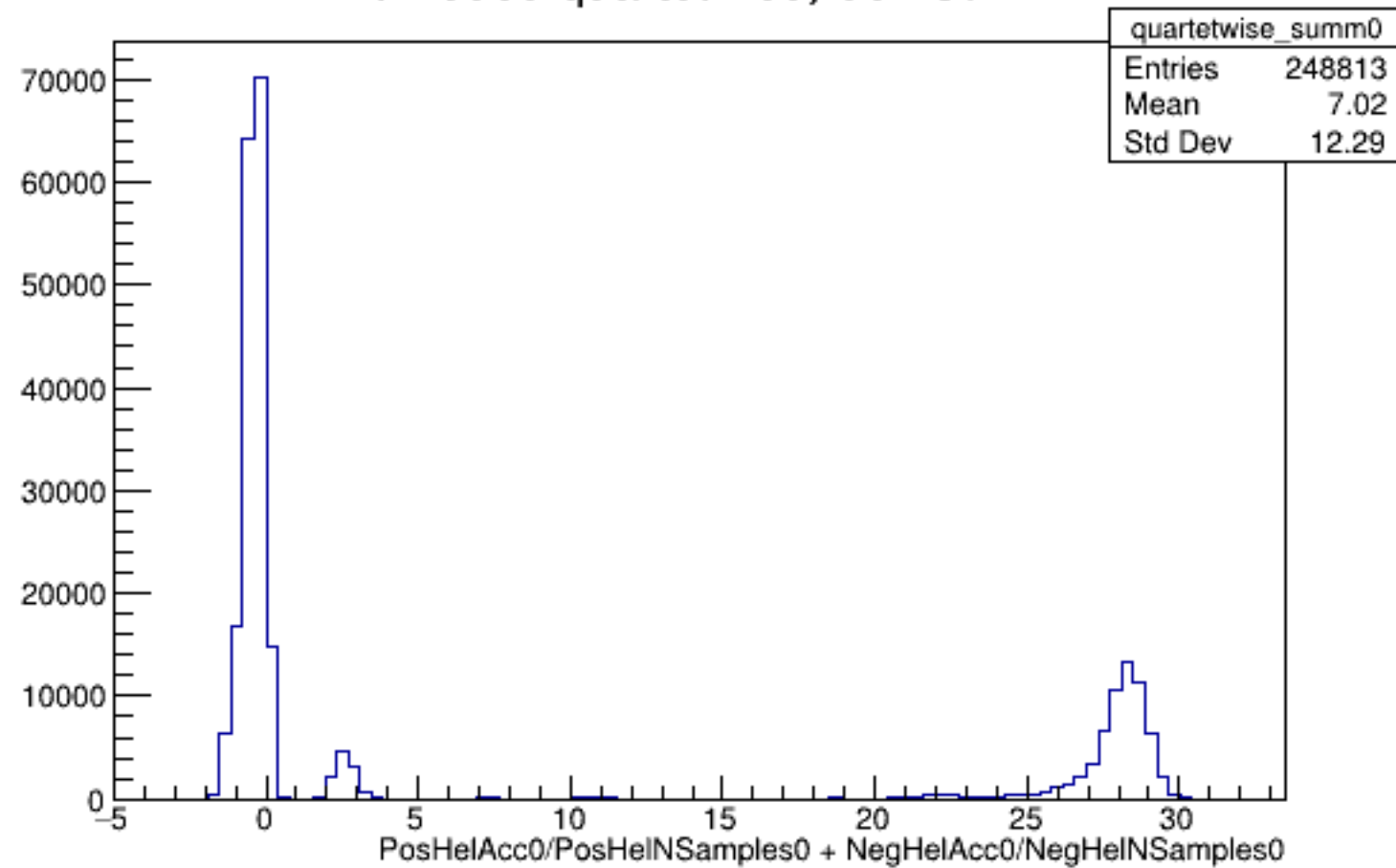
Run 5665 quartetwise, Sums0: All
