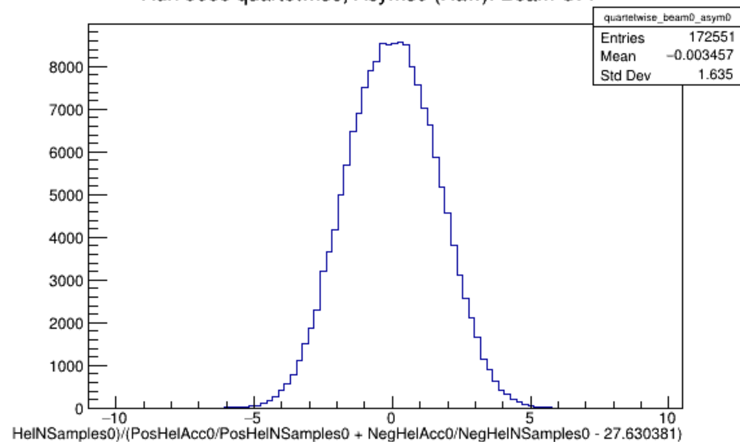
Run 5665 quartetwise, Asyms0 (Raw): Beam OFF
