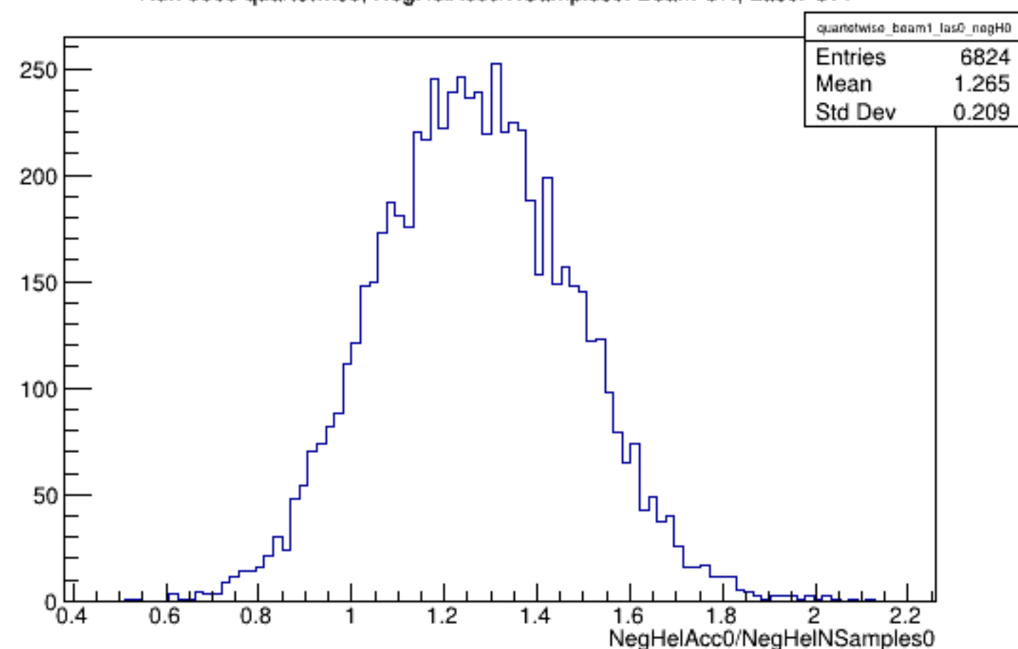
Run 5665 quartetwise, NegHelAcc0/NSamples0: Beam ON, Laser OFF
