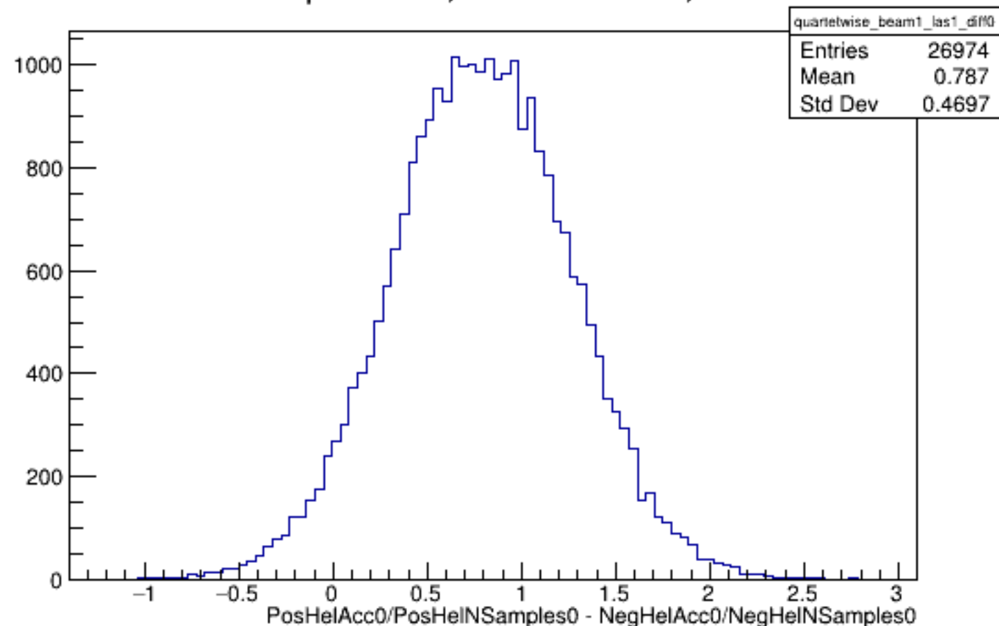
Run 5665 quartetwise, Diffs0: Beam ON, Laser ON
