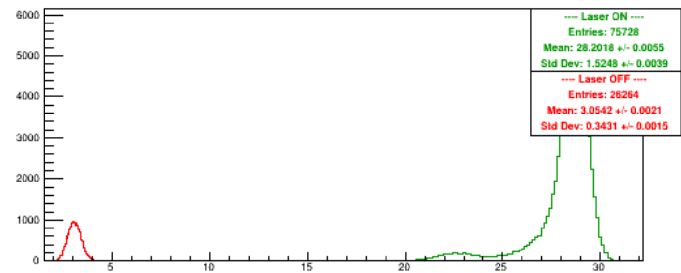
Run 5681 quartetwise, Sums0
