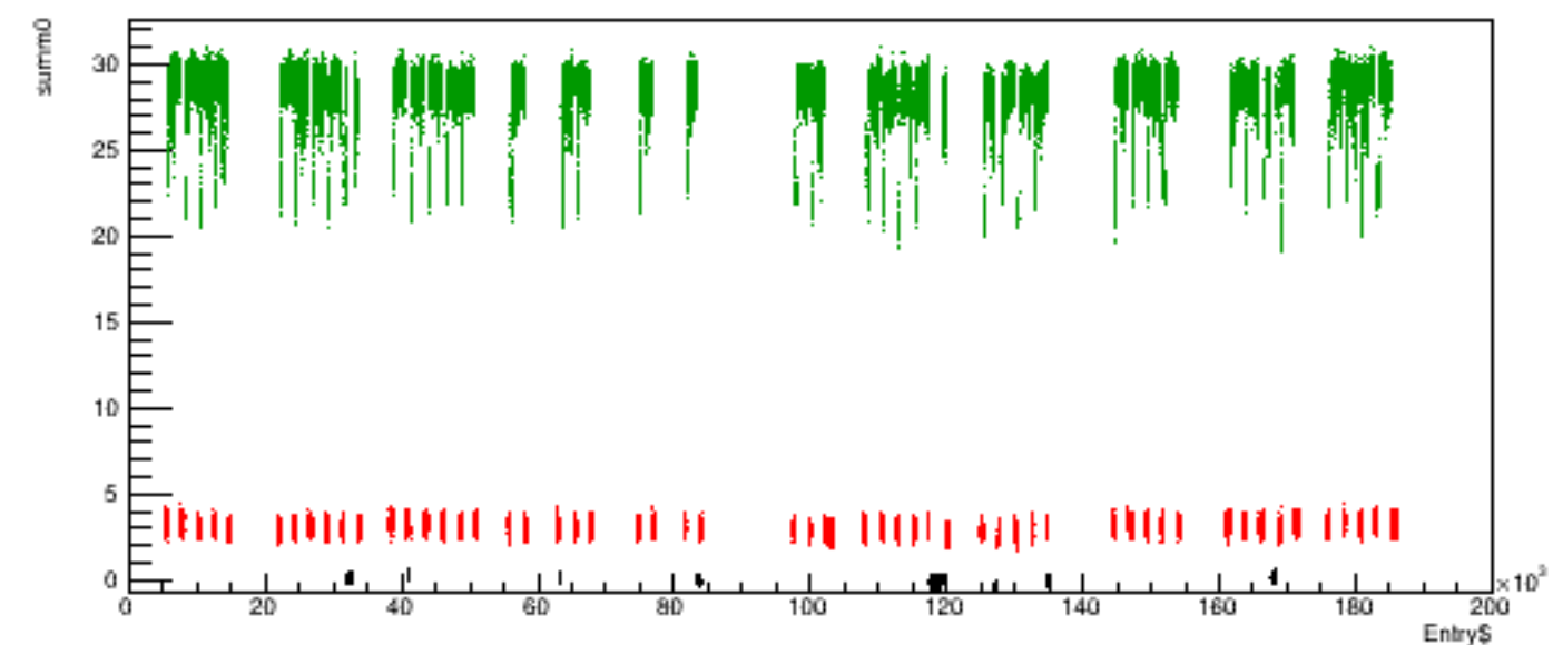
Run 5681 quartetwise, summ0 vs time
