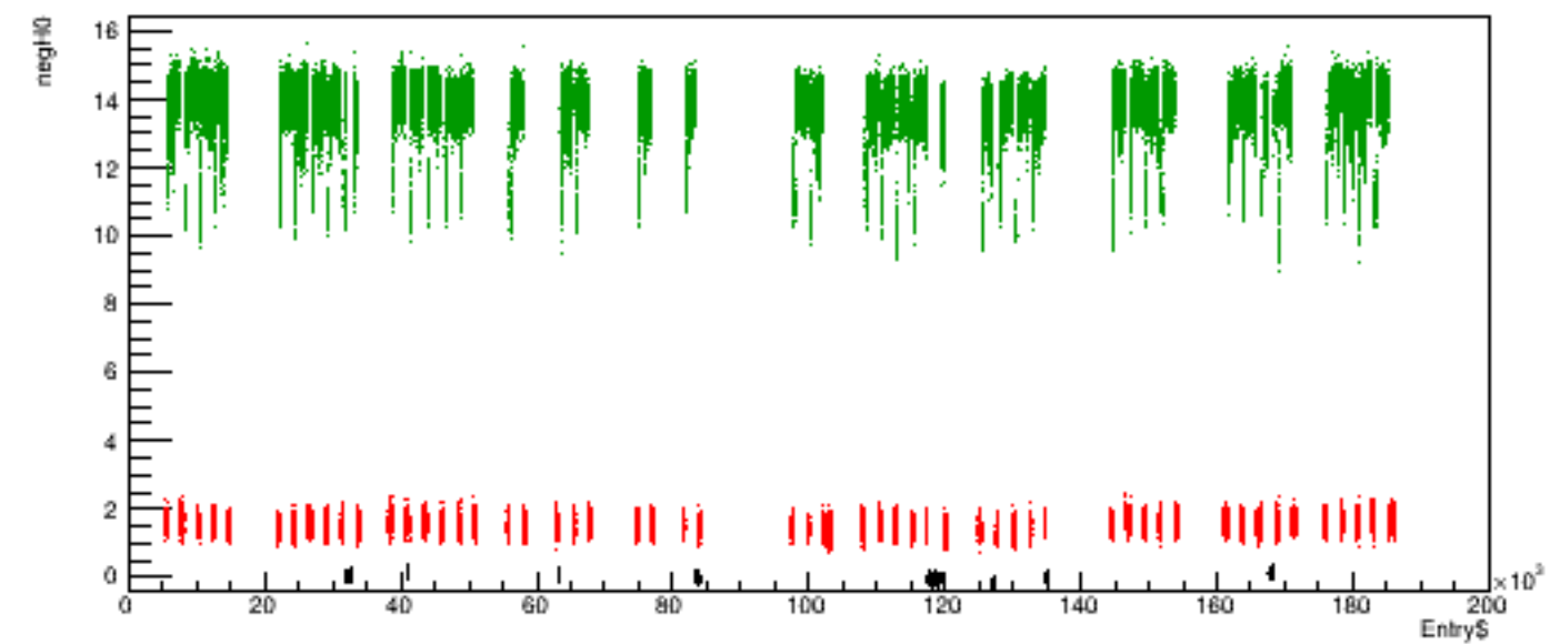
Run 5681 quartetwise, negH0 vs time
