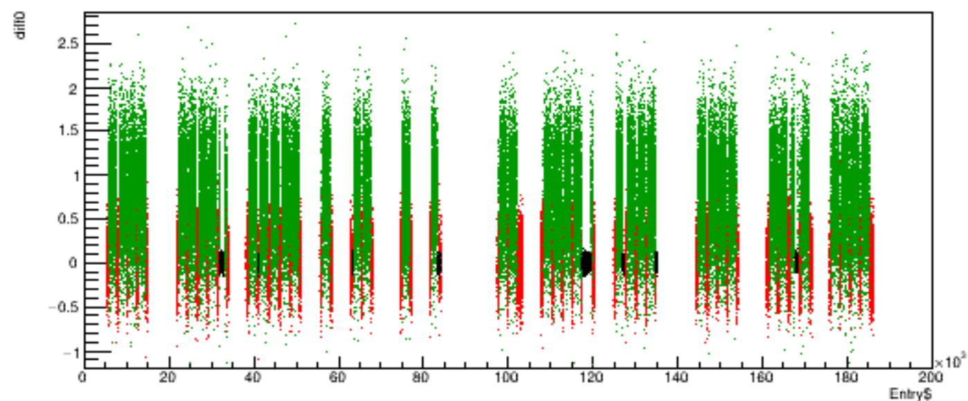
Run 5681 quartetwise, diff0 vs time
