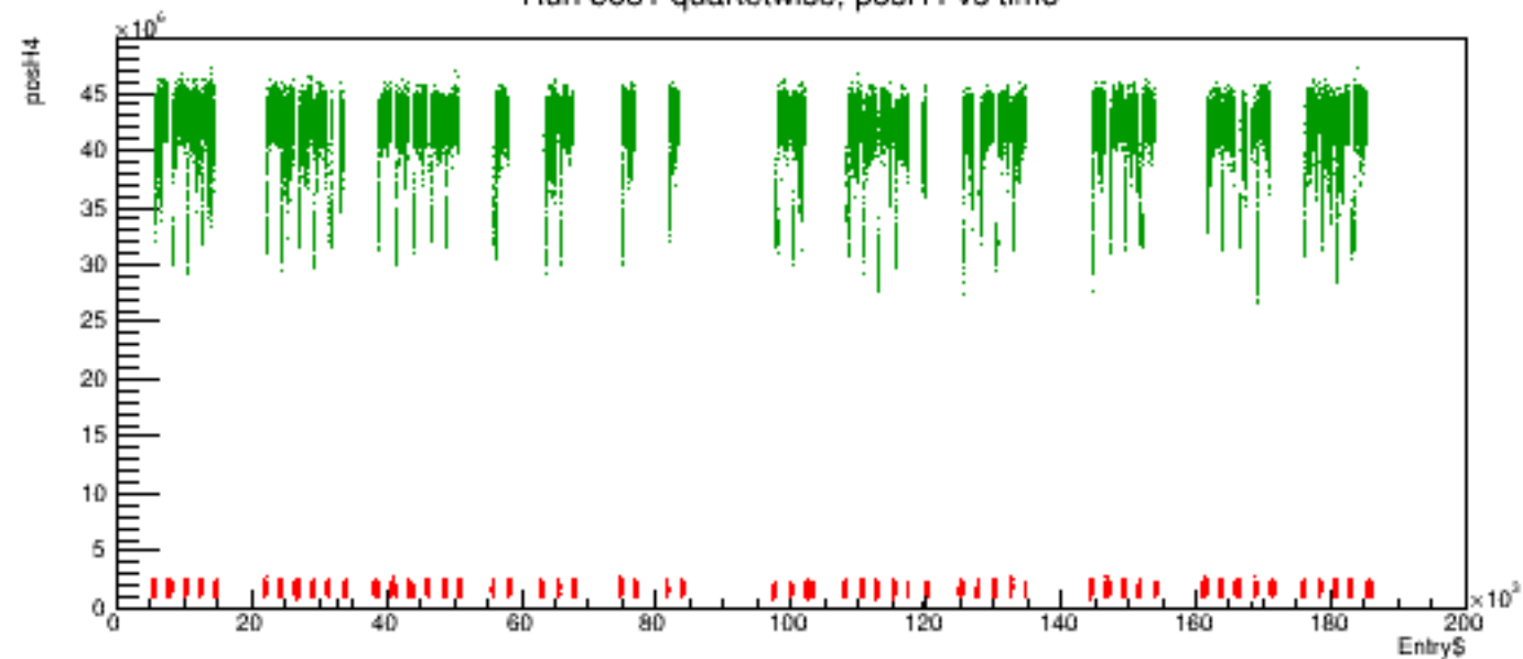
Run 5681 quartetwise, posH4 vs time
