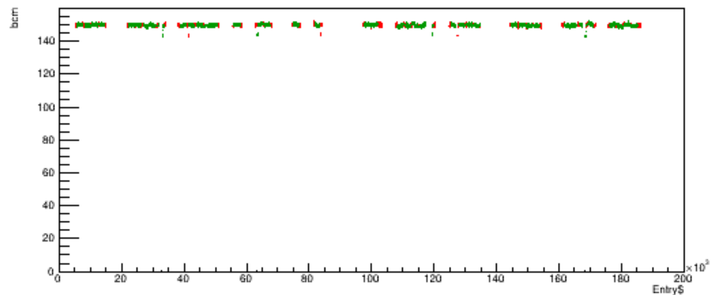
Run 5681 quartetwise, posH4 vs time
