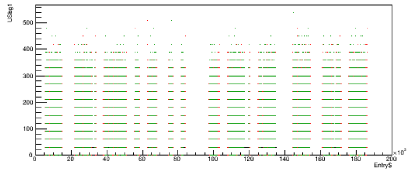
Run 5681 quartetwise, USbg1 vs time
