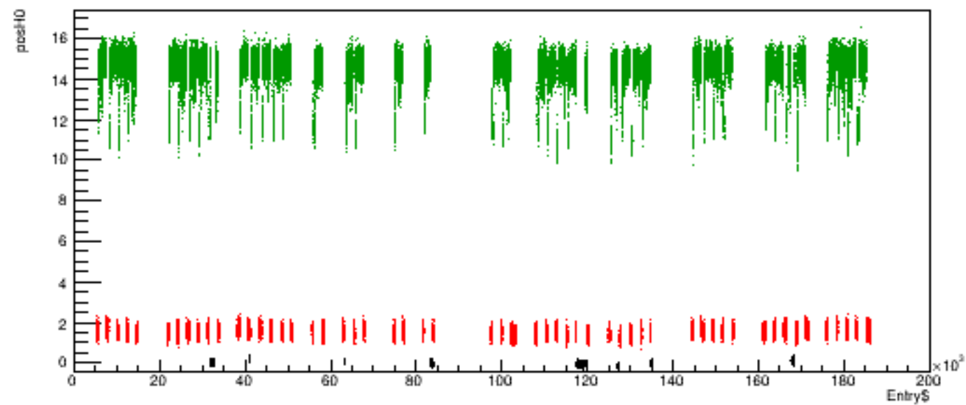
Run 5681 quartetwise, posH0 vs time
