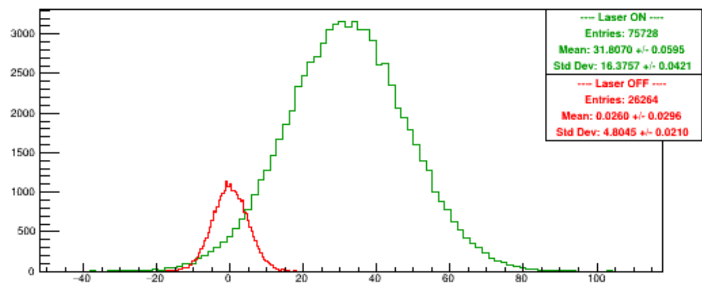
Run 5681 quartetwise, Asyms4
