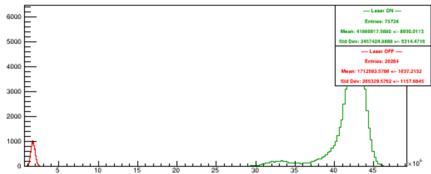
Run 5681 quartetwise, PosHelAcc4
