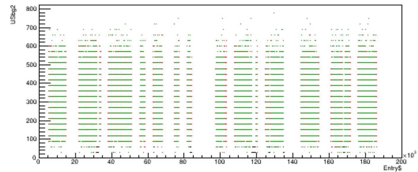
Run 5681 quartetwise, USbg2 vs time
