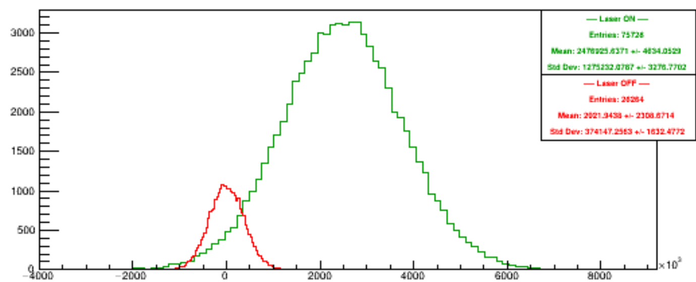
Run 5681 quartetwise, Diffs4
