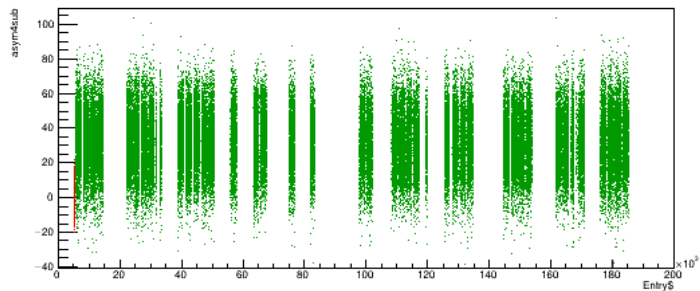
Run 5681 quartetwise, asym4sub vs time
