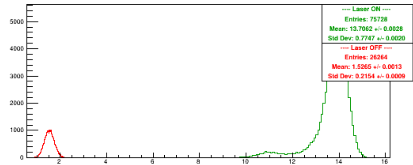
Run 5681 quartetwise, NegHelAcc0/NSamples0
