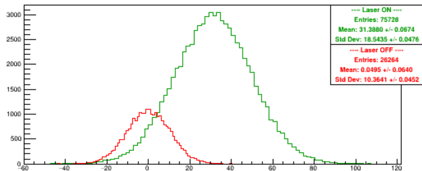
Run 5681 quartetwise, Asyms0
