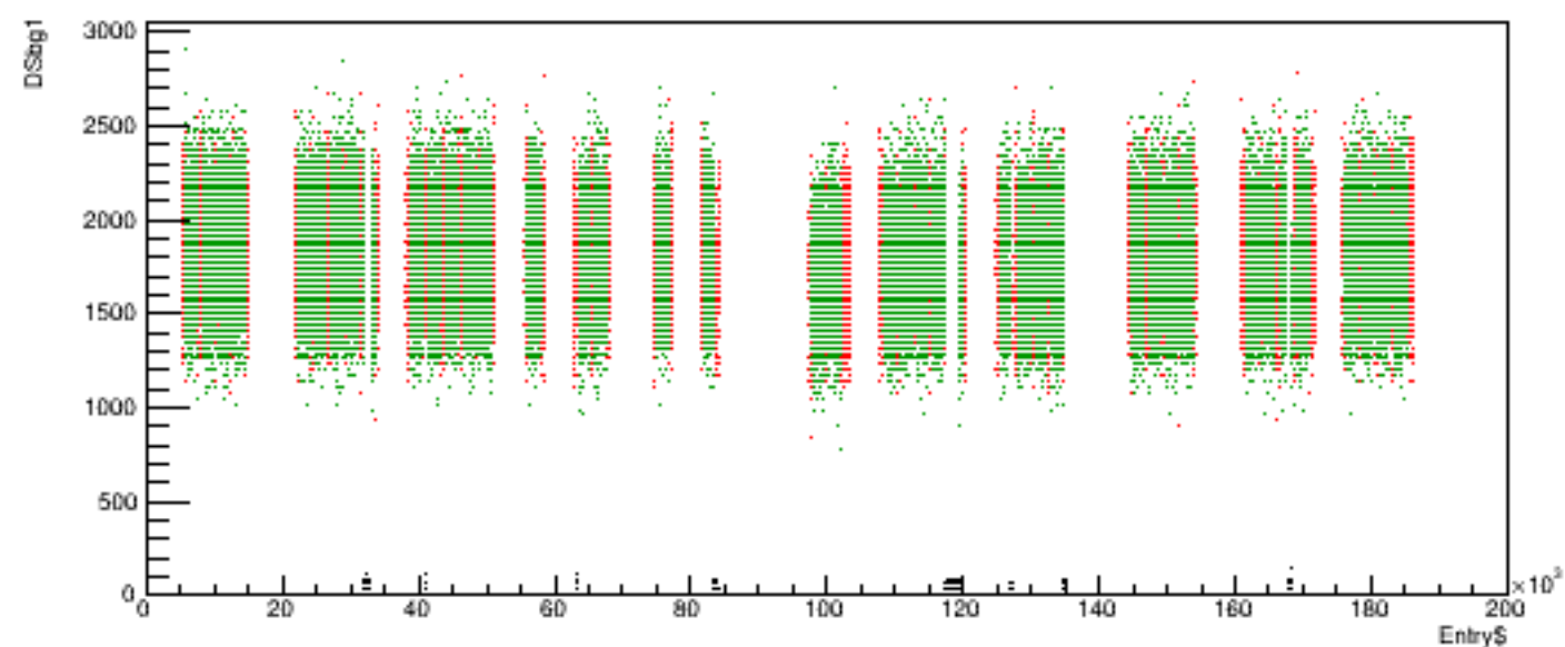
Run 5681 quartetwise, DSbg1 vs time
