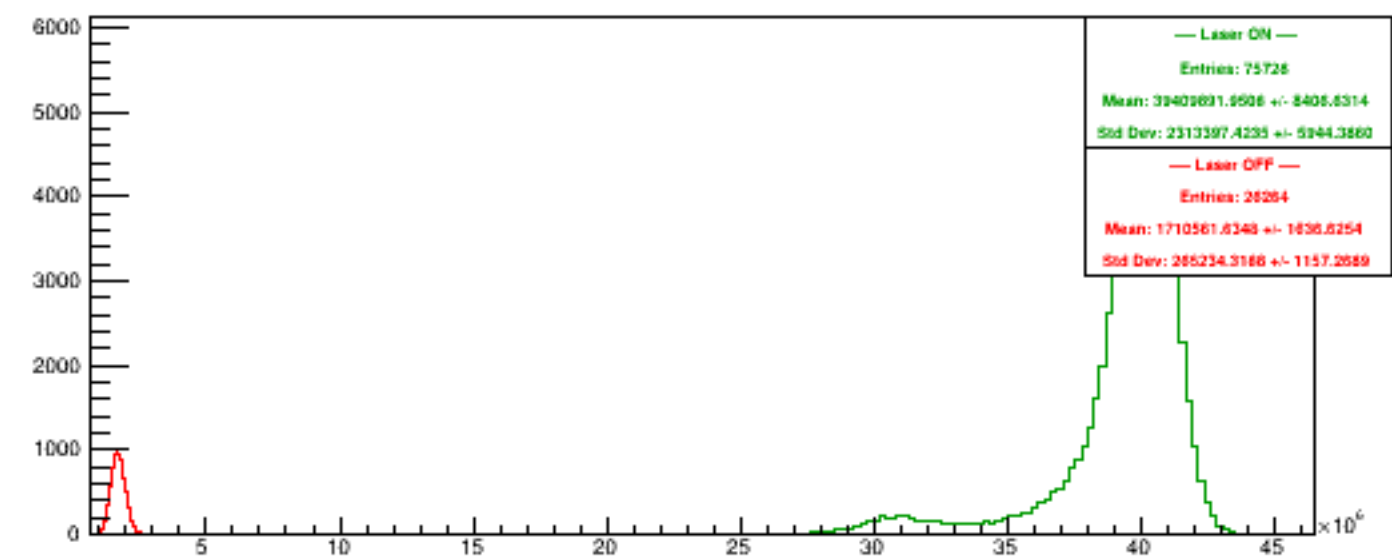
Run 5681 quartetwise, NegHelAcc4
