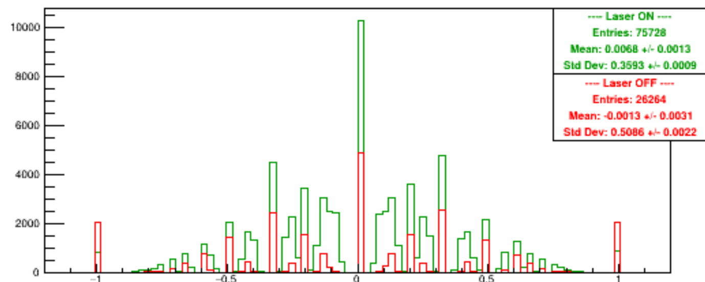
Run 5681 quartetwise, Asyms Horiz Finger
