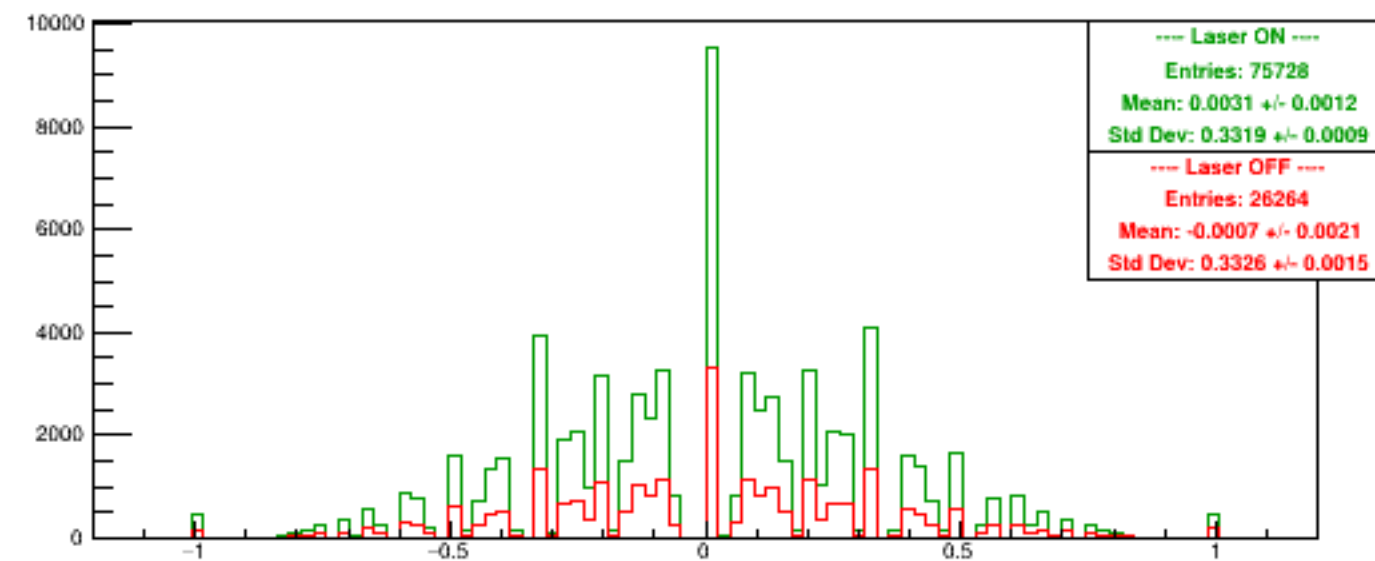
Run 5681 quartetwise, Asyms USbg2
