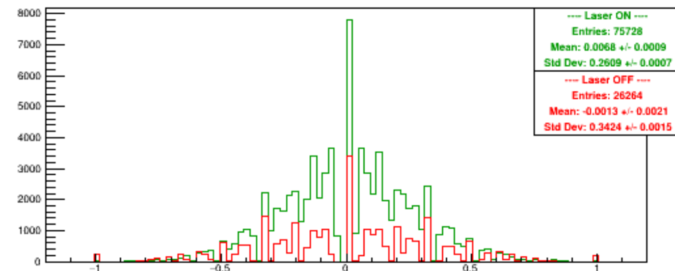
Run 5681 quartetwise, Asyms Vert Finger
