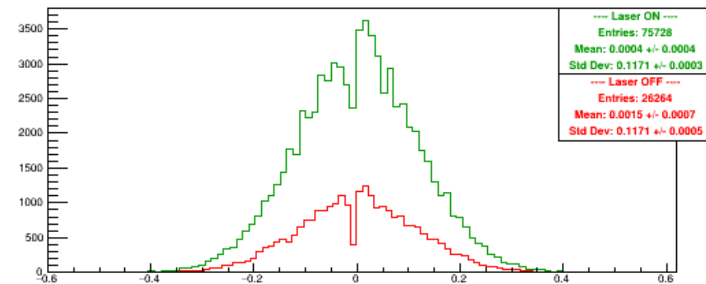
Run 5681 quartetwise, Asyms DSbg2
