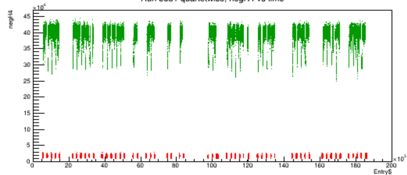
Run 5681 quartetwise, negH4 vs time
