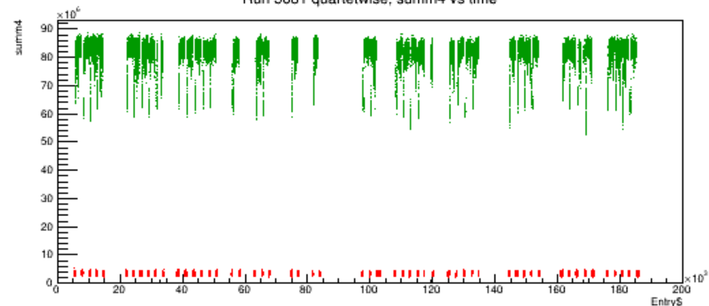
Run 5681 quartetwise, summ4 vs time
