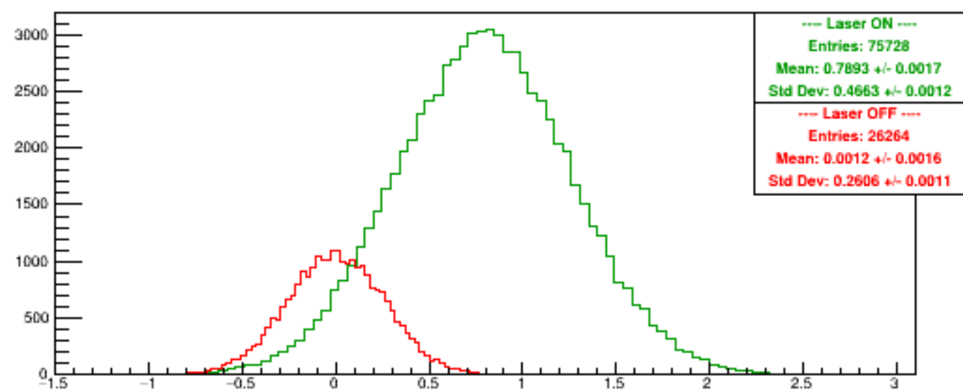
Run 5681 quartetwise, Diffs0
