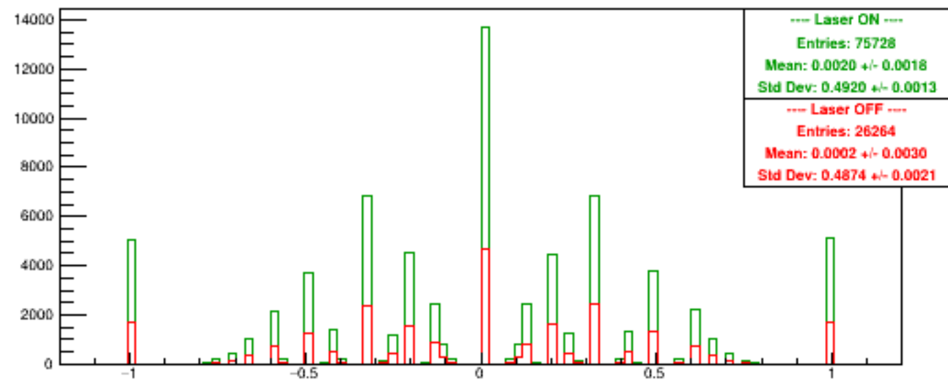
Run 5681 quartetwise, Asyms USbg1
