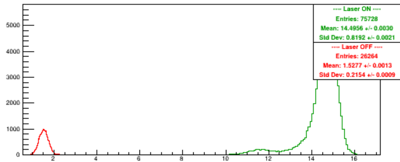
Run 5681 quartetwise, PosHelAcc0/NSamples0
