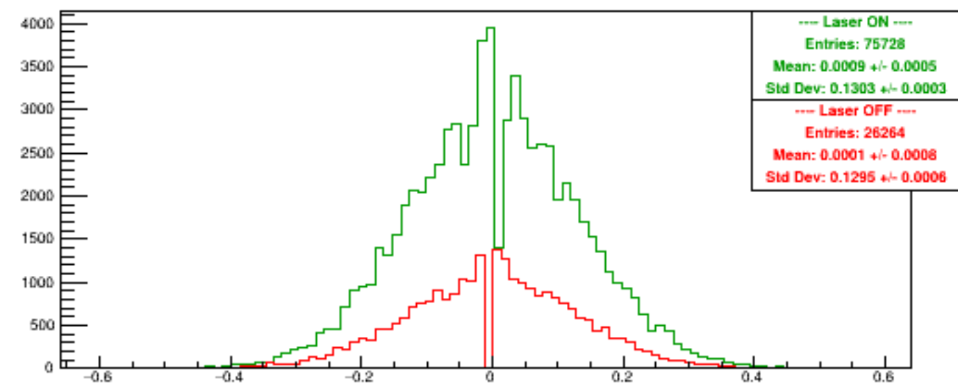
Run 5681 quartetwise, Asyms DSbg1
