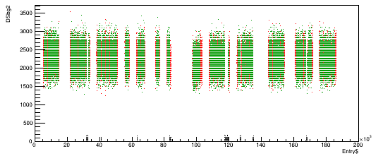
Run 5681 quartetwise, DSbg2 vs time
