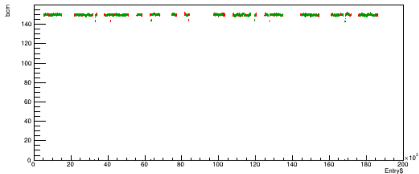
Run 5681 quartetwise, posH4 vs time
