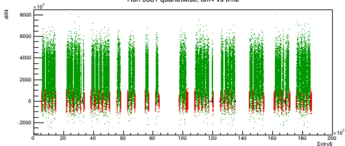
Run 5681 quartetwise, diff4 vs time
