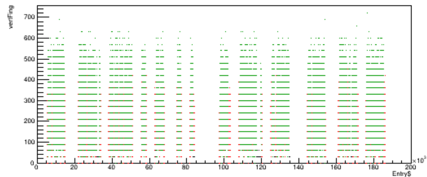
Run 5681 quartetwise, vertFing vs time
