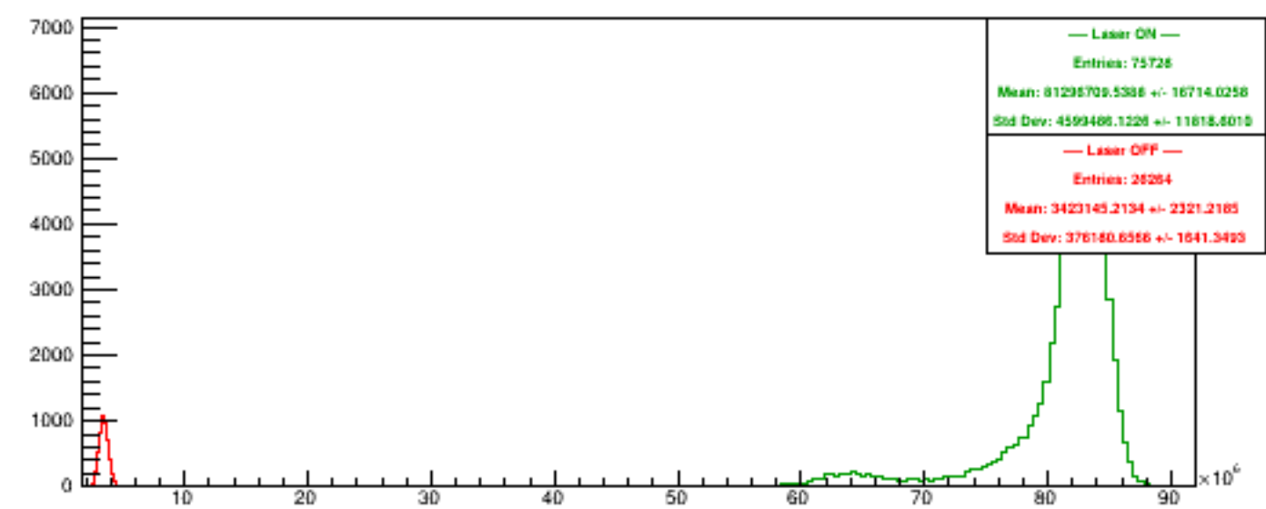
Run 5681 quartetwise, Sums4
