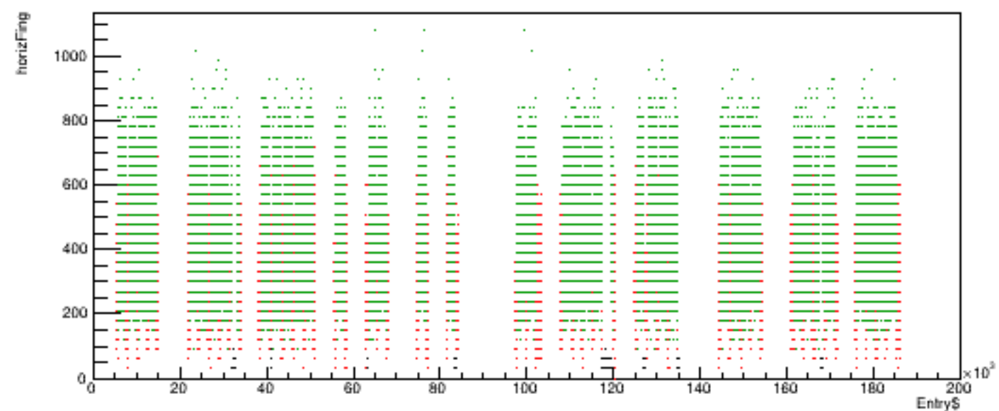
Run 5681 quartetwise, horizFing vs time
