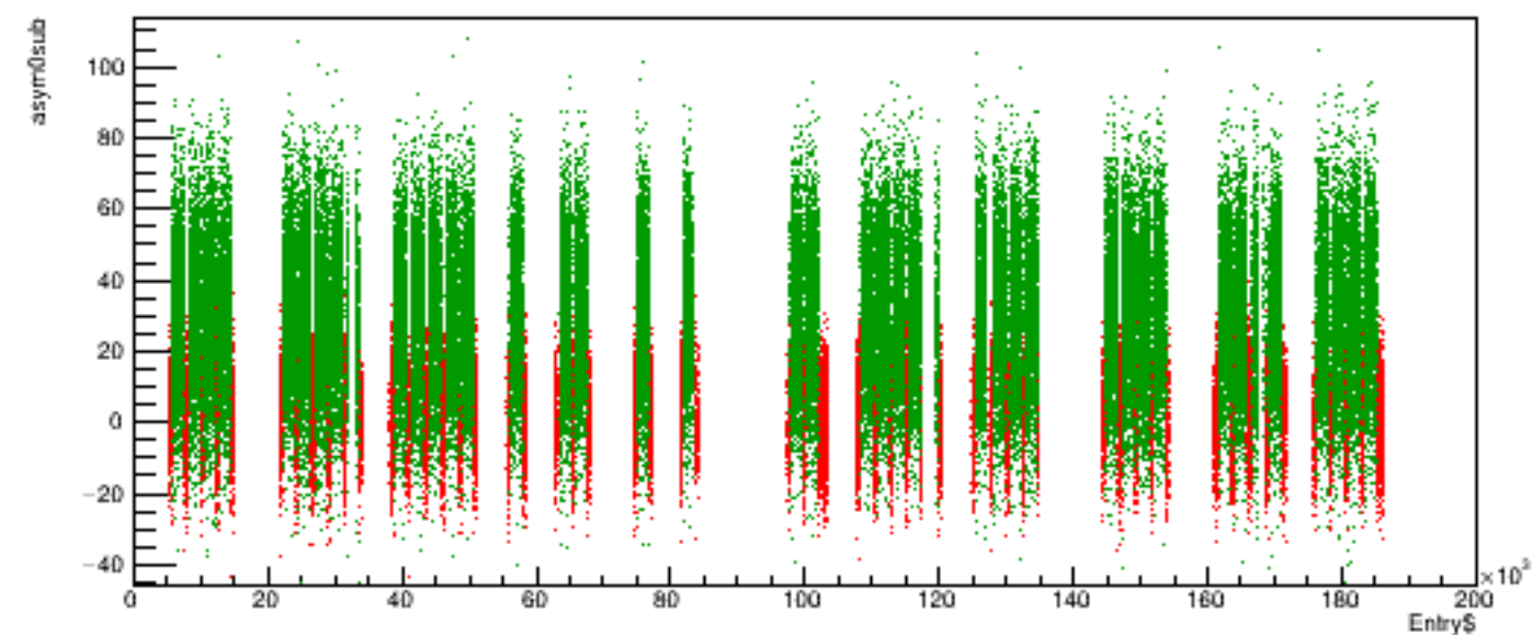
Run 5681 quartetwise, asym0sub vs time
