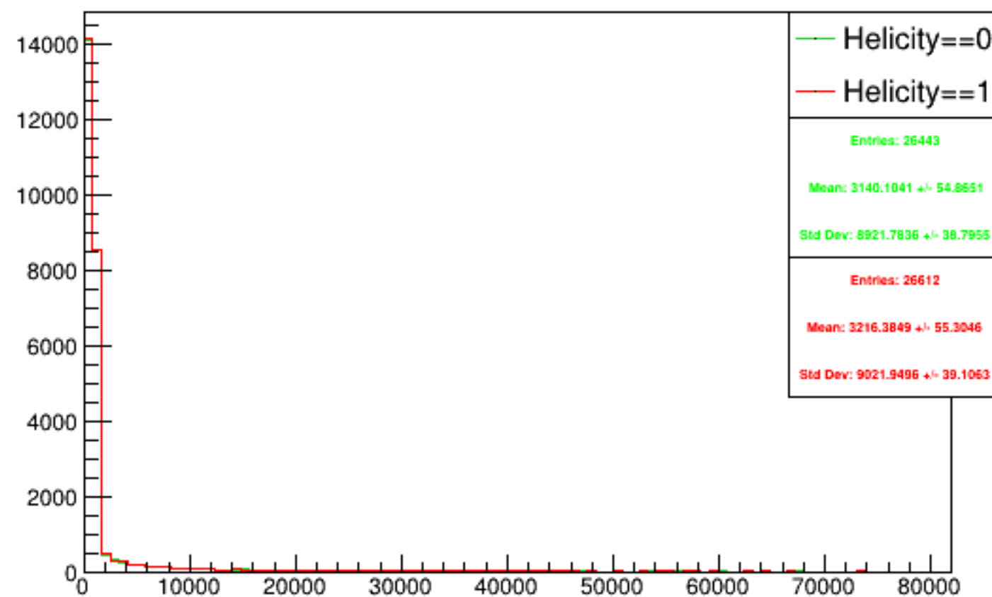
Run 5684 triggerwise, sums: Beam ON, Laser OFF
