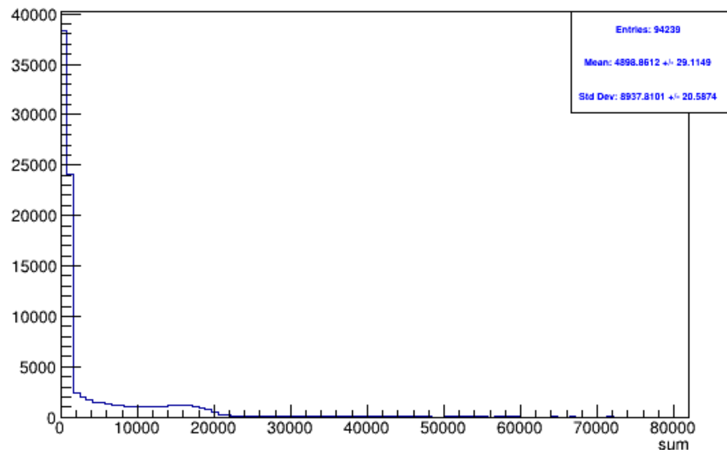
Run 5684 triggerwise, sums: All
