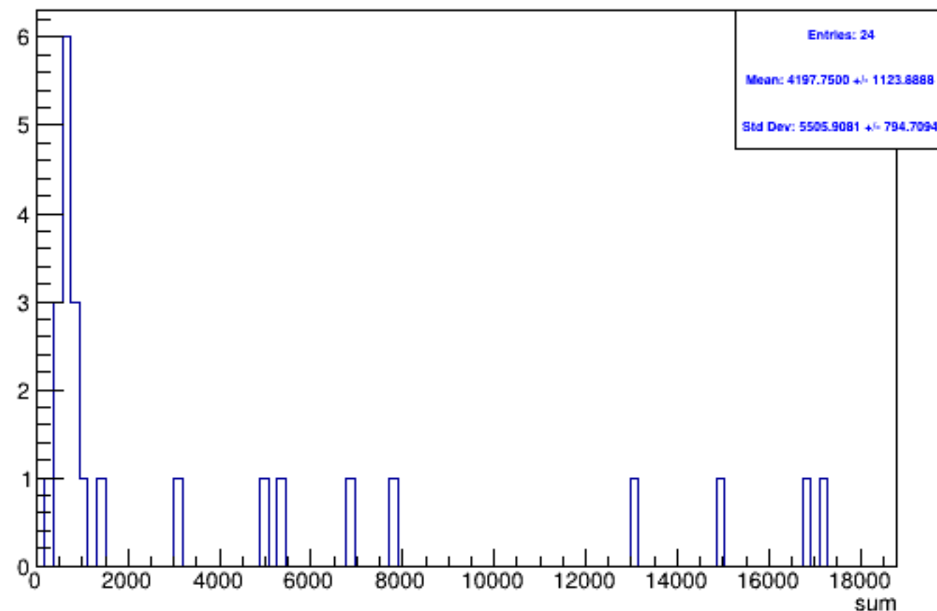
Run 5684 triggerwise, sums: Beam OFF
