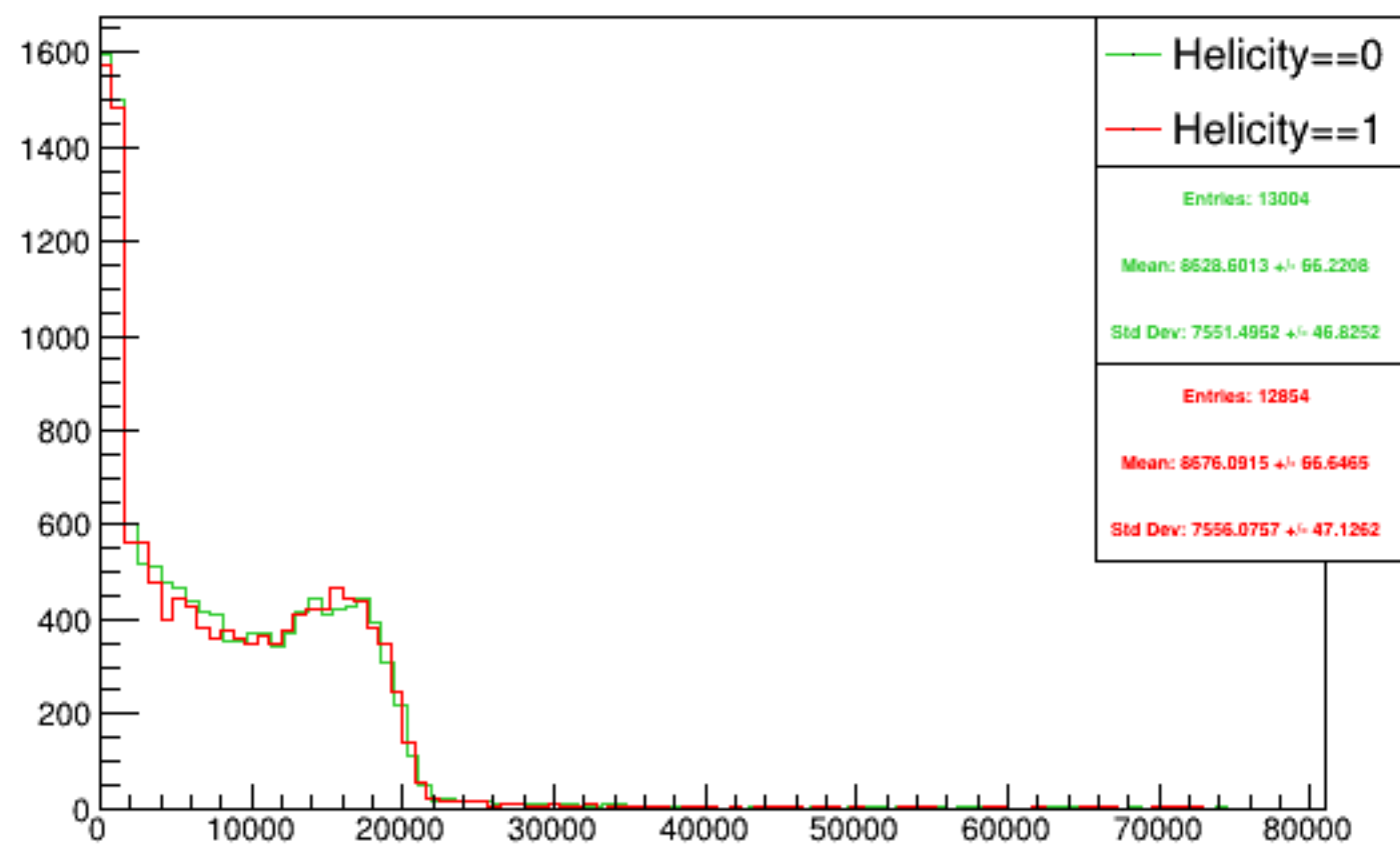
Run 5684 triggerwise, sums: Beam ON, Laser ON
