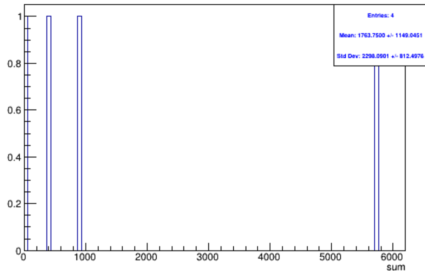
Run 5685 triggerwise, sums: Beam OFF
