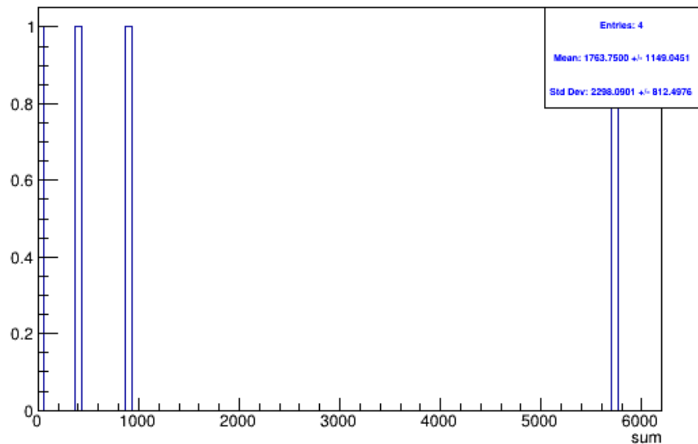
Run 5685 triggerwise, sums: All
