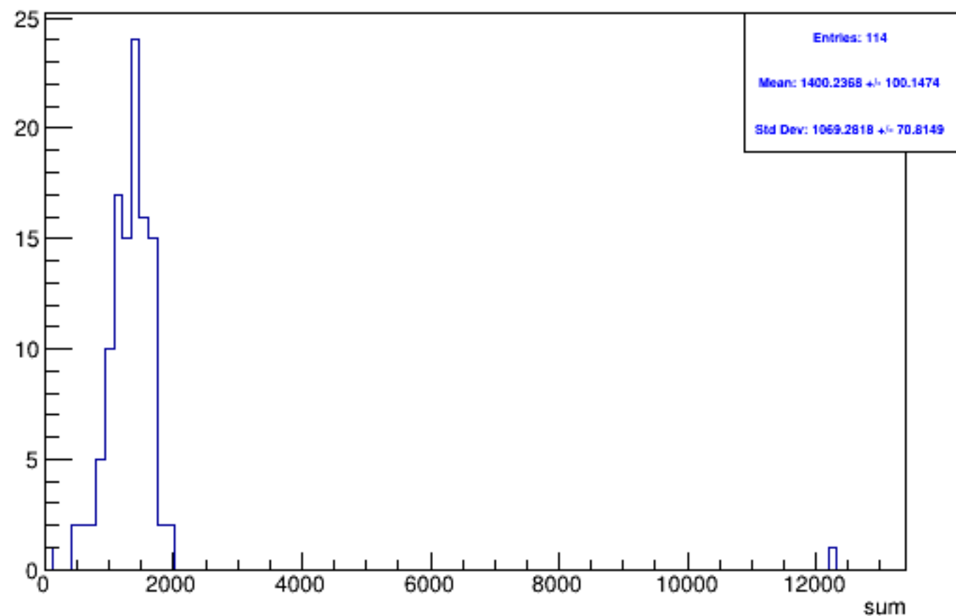
Run 5690 triggerwise, sums: All
