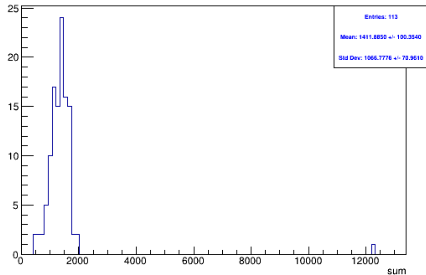
Run 5690 triggerwise, sums: Beam OFF
