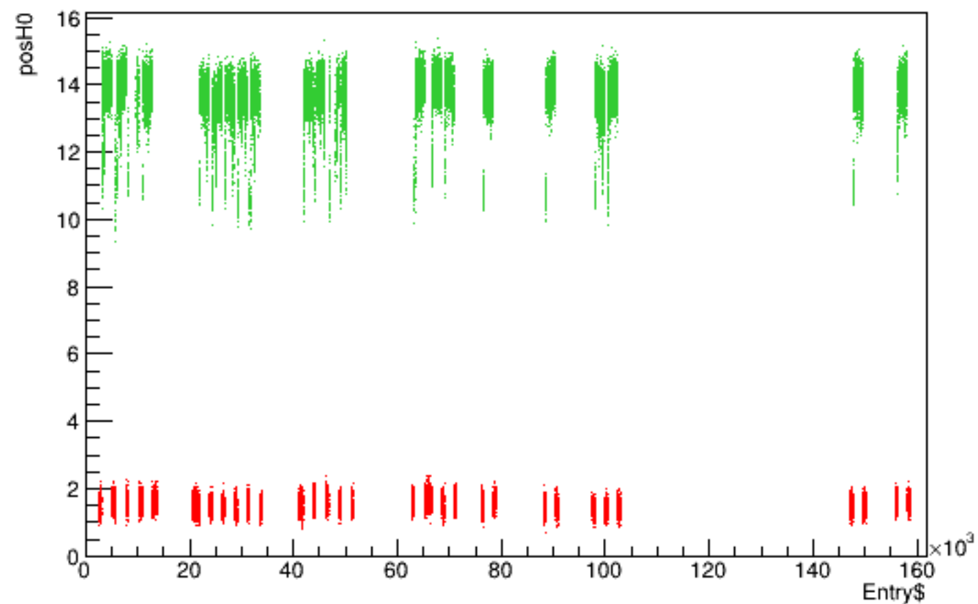
Run 5691 quartetwise, posH0 vs time
