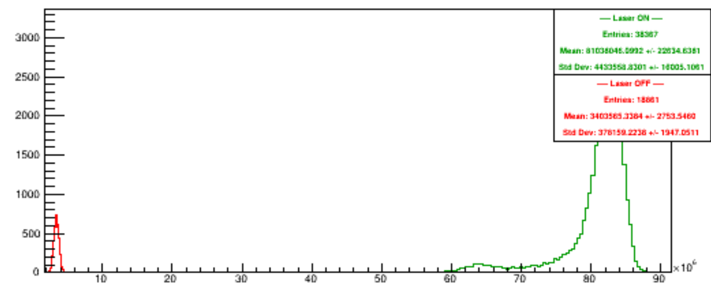
Run 5691 quartetwise, Sums4
