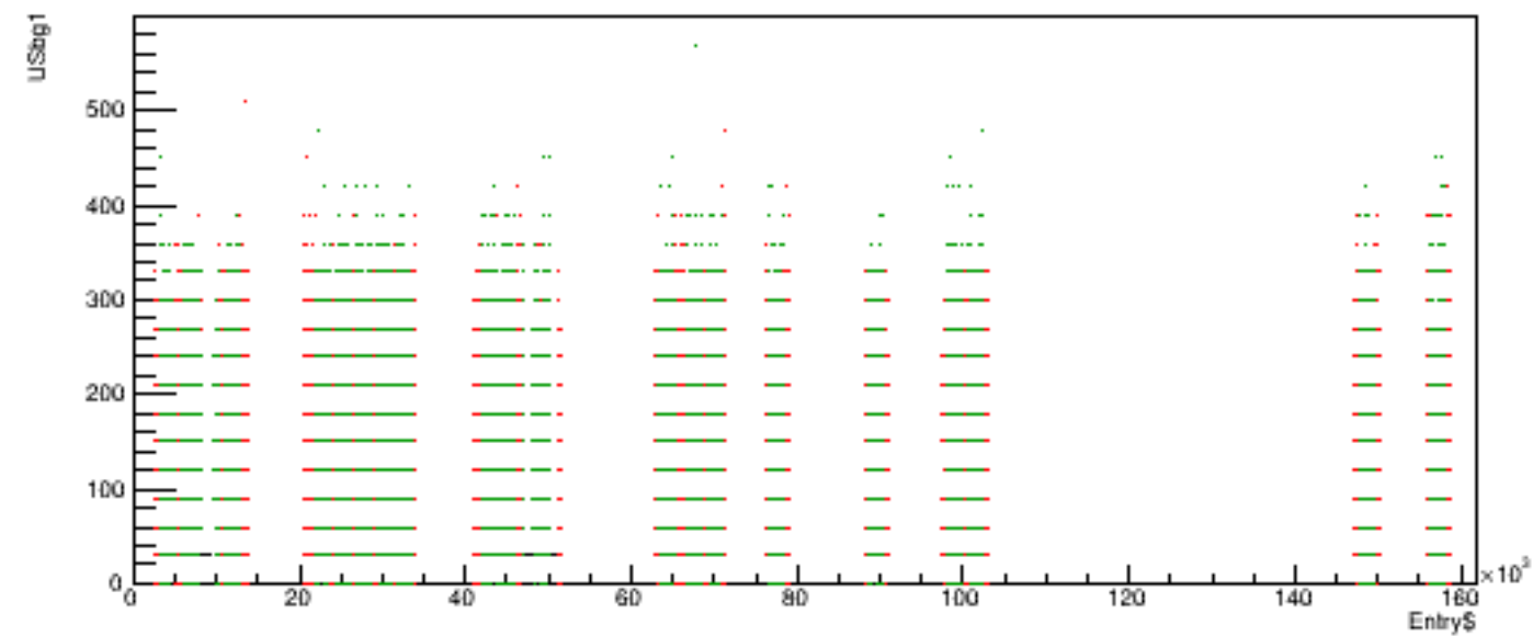
Run 5691 quartetwise, USbg1 vs time
