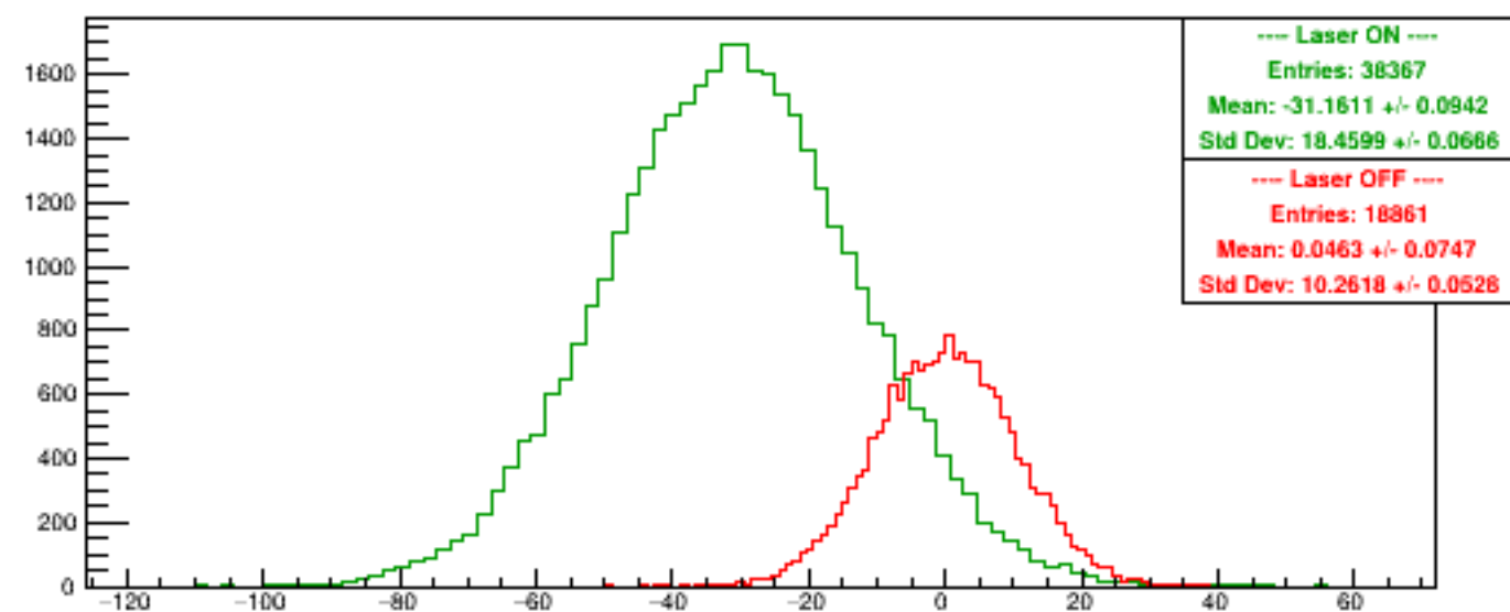
Run 5691 quartetwise, Asyms0
