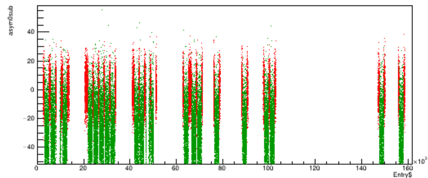
Run 5691 quartetwise, asym0sub vs time
