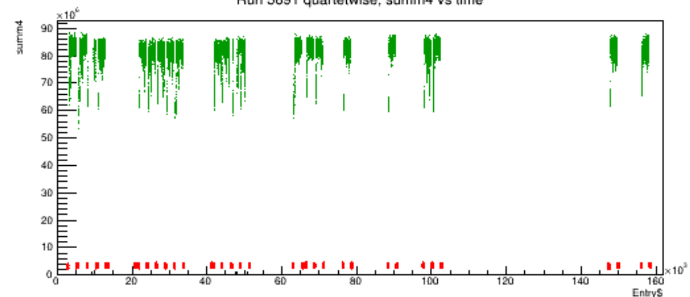
Run 5691 quartetwise, summ4 vs time
