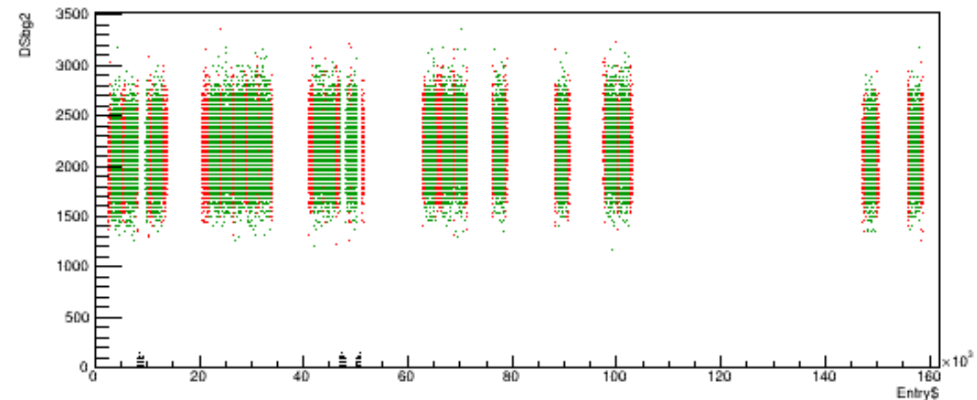
Run 5691 quartetwise, DSbg2 vs time
