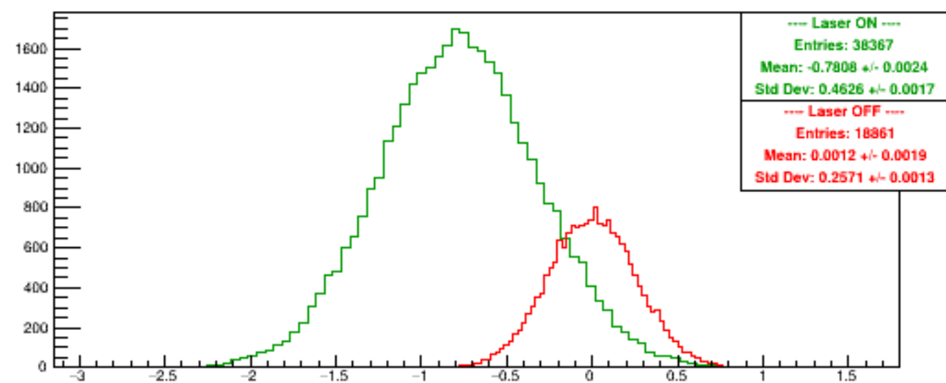
Run 5691 quartetwise, Diffs0
