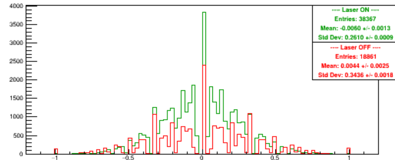
Run 5691 quartetwise, Asyms Vert Finger
