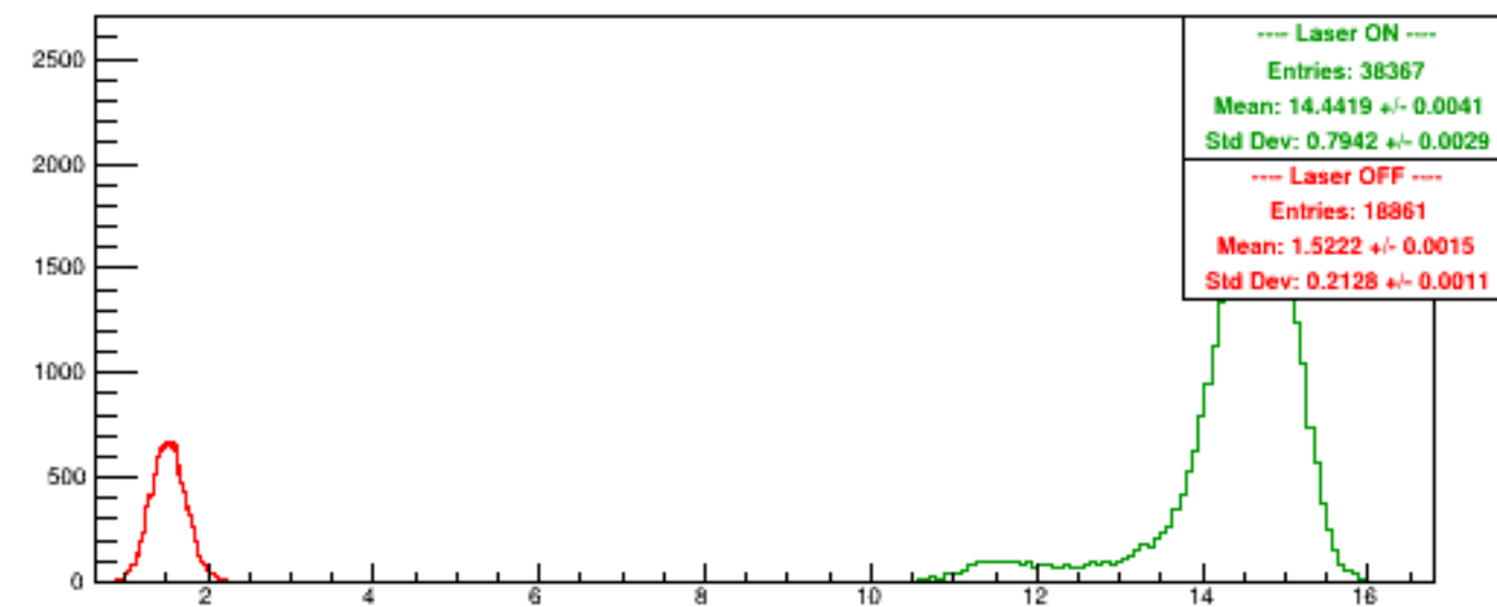
Run 5691 quartetwise, NegHelAcc0/NSamples0
