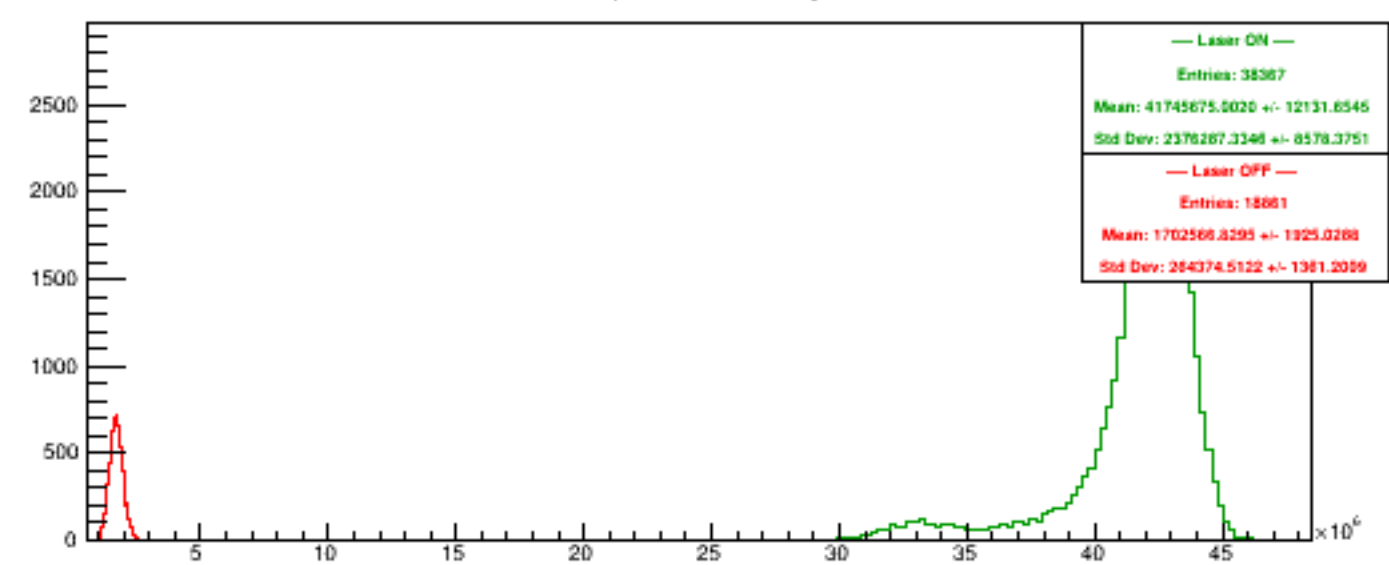
Run 5691 quartetwise, NegHelAcc4
