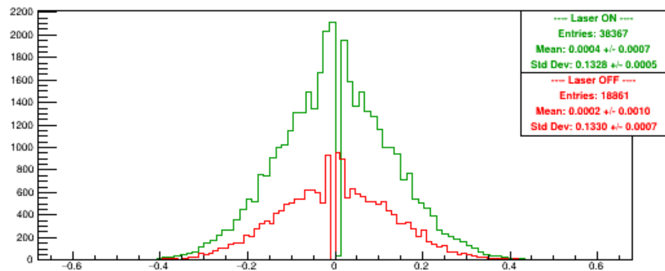
Run 5691 quartetwise, Asyms DSbg1
