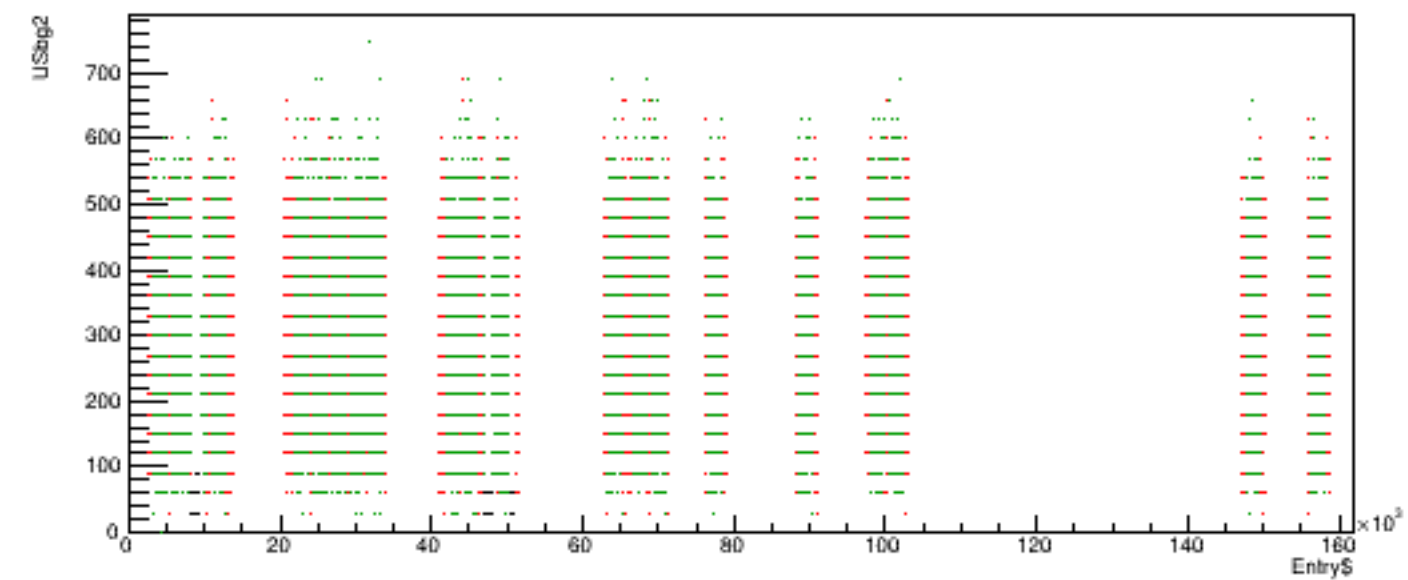
Run 5691 quartetwise, USbg2 vs time
