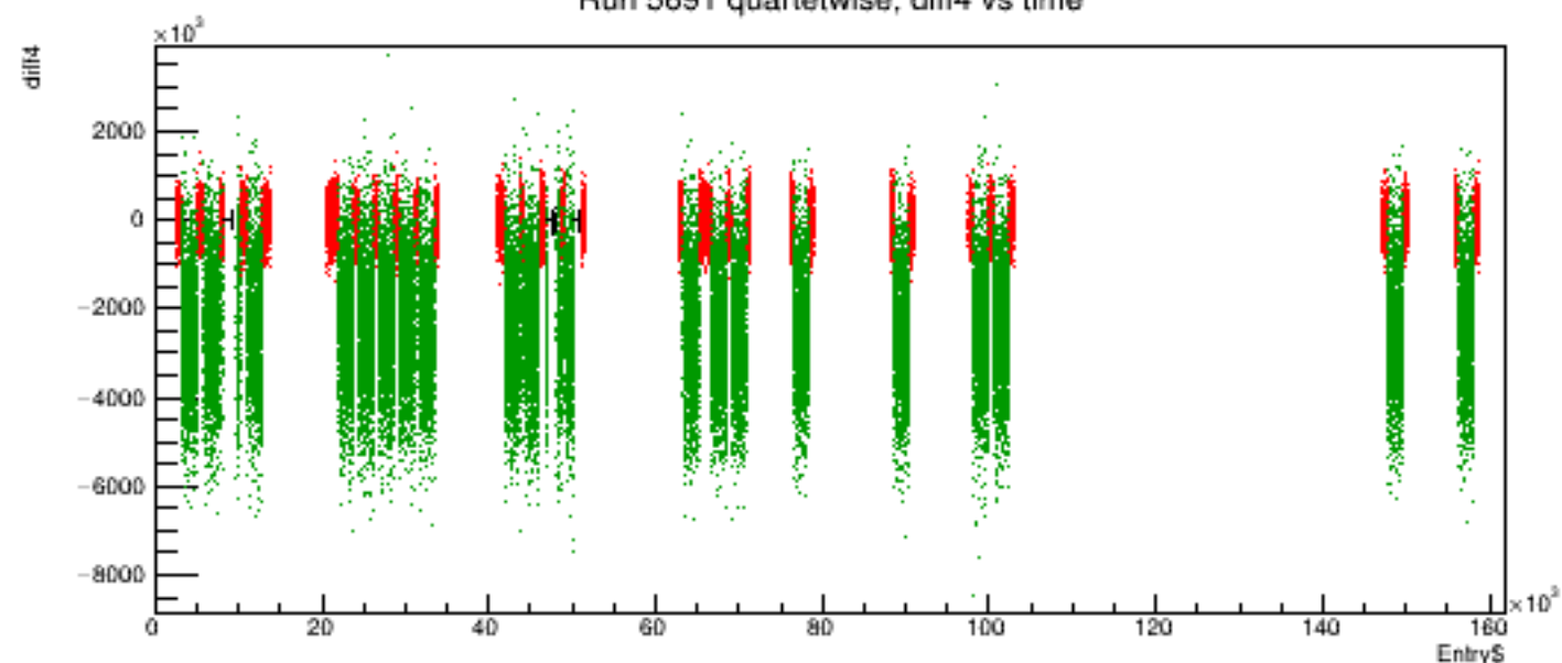
Run 5691 quartetwise, diff4 vs time
