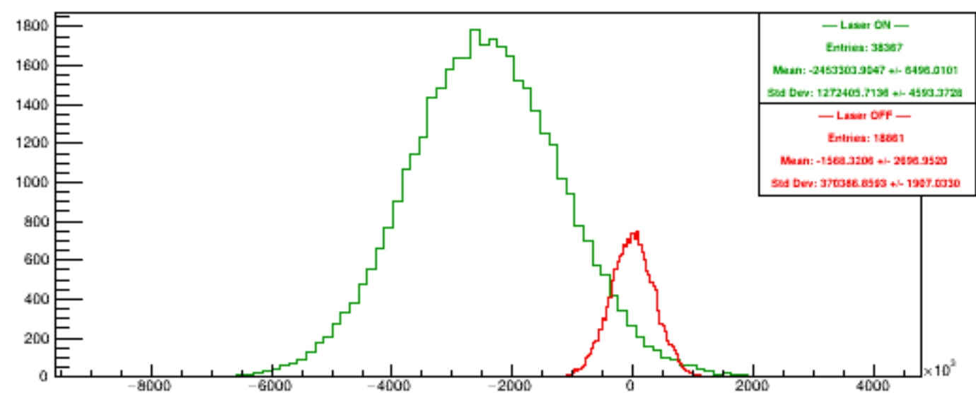
Run 5691 quartetwise, Diffs4
