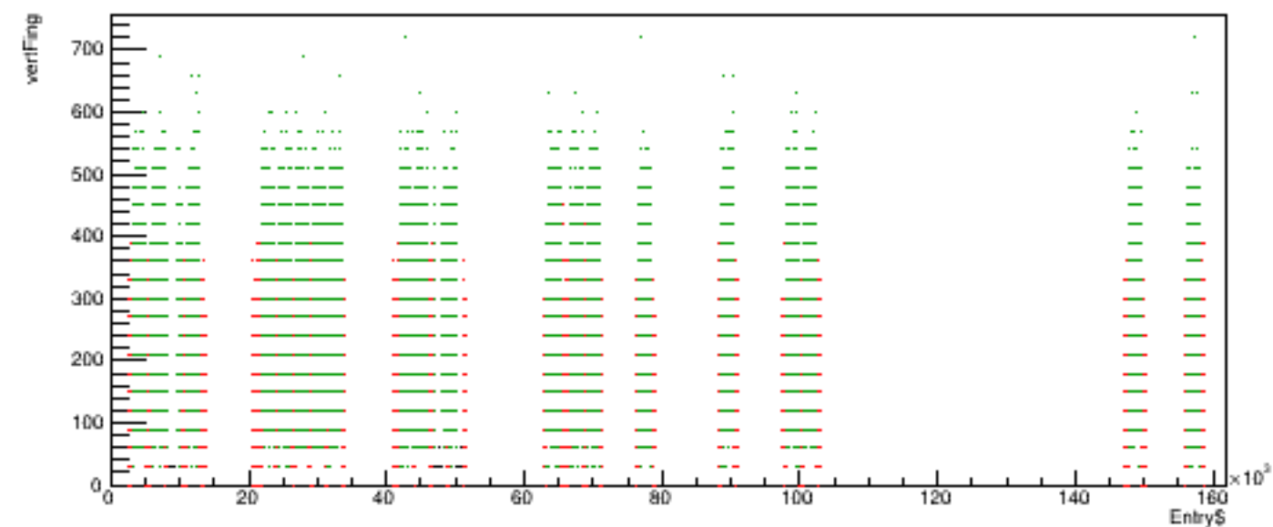
Run 5691 quartetwise, vertFing vs time
