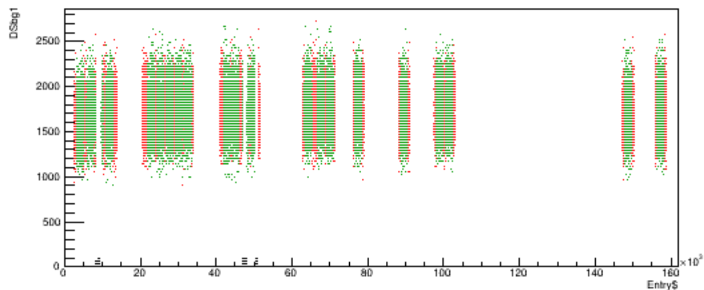
Run 5691 quartetwise, DSbg1 vs time
