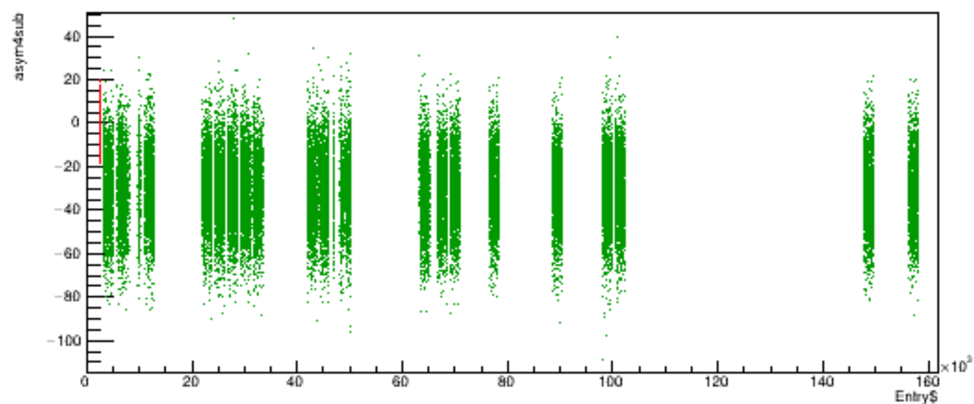
Run 5691 quartetwise, asym4sub vs time
