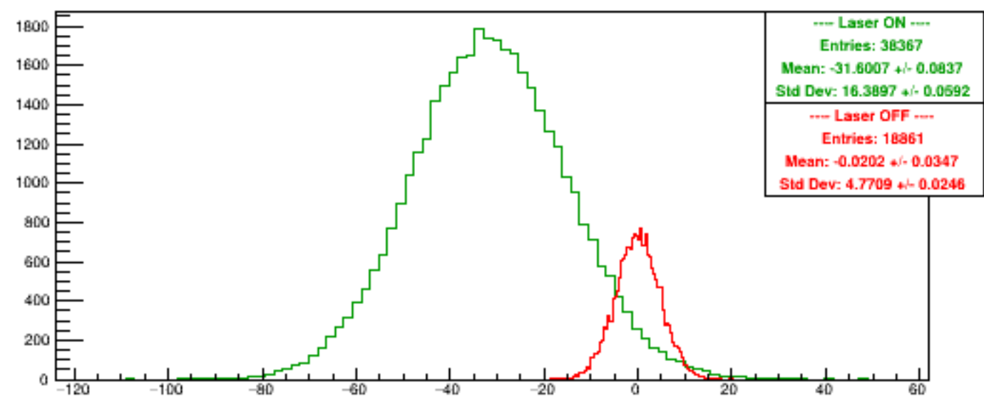
Run 5691 quartetwise, Asyms4
