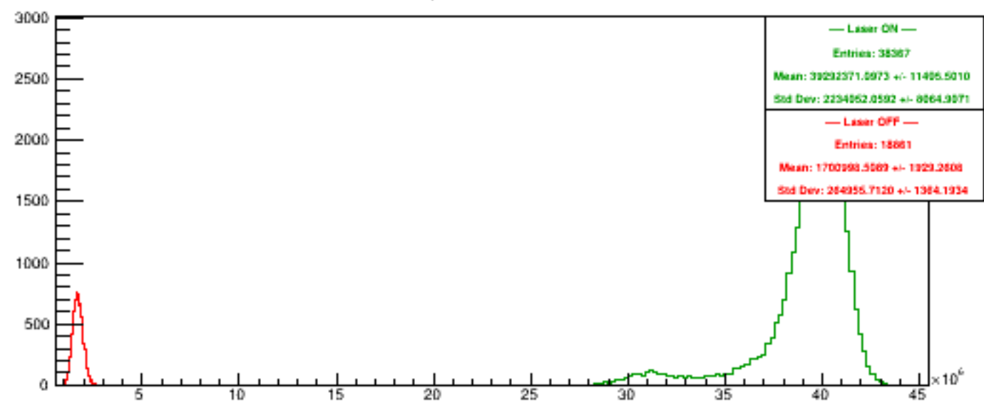
Run 5691 quartetwise, PosHelAcc4
