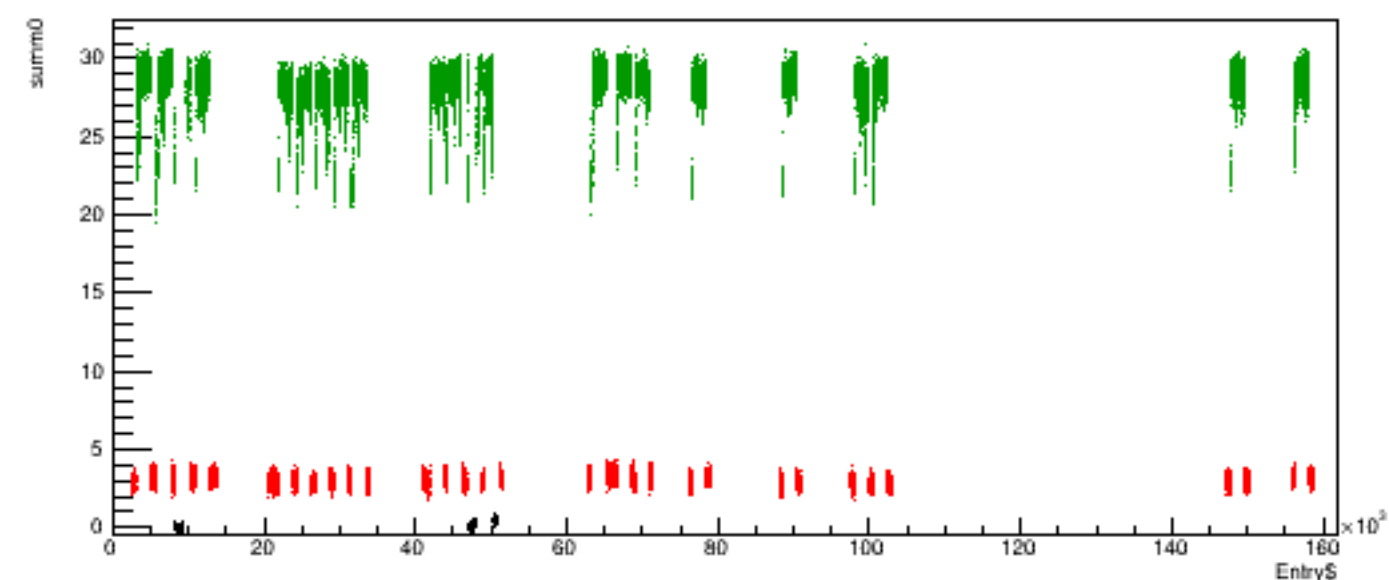
Run 5691 quartetwise, summ0 vs time
