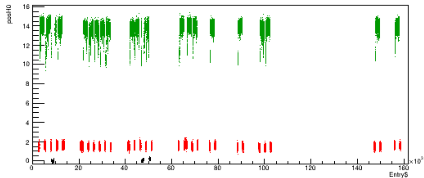
Run 5691 quartetwise, posH0 vs time
