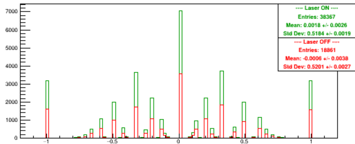
Run 5691 quartetwise, Asyms USbg1
