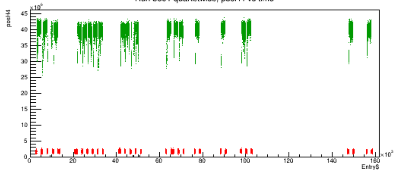
Run 5691 quartetwise, posH4 vs time
