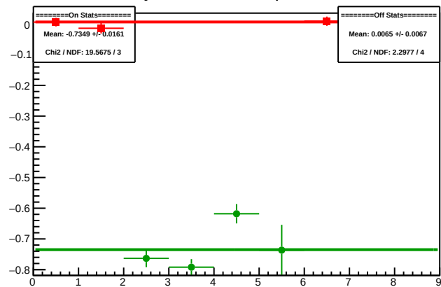
Cycle 5693.1: Multiplet Diffs
