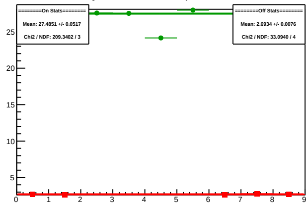
Cycle 5693.1: Multiplet Sums
