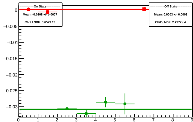
Cycle 5693.1: Multiplet Asyms
