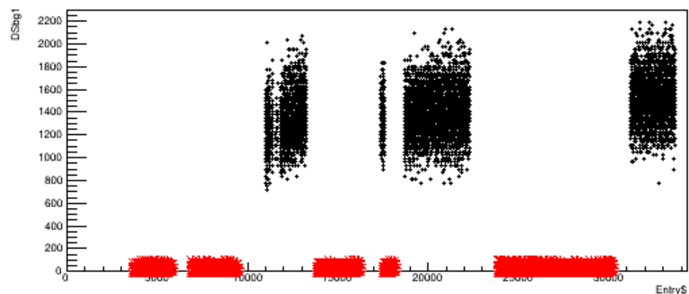
Run 5695, quartetwise: DSbg1 vs time
