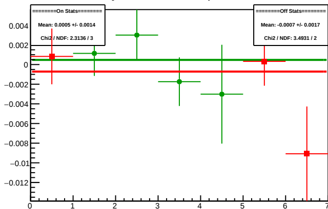
Cycle 5695.2: Multiplet Diffs
