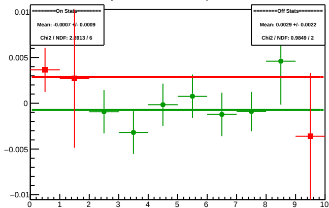
Cycle 5695.4: Multiplet Diffs
