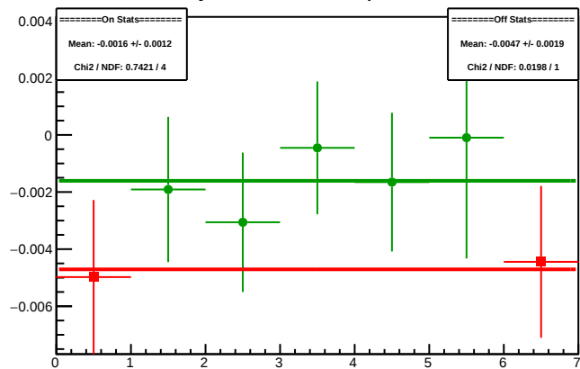
Cycle 5695.1: Multiplet Diffs
