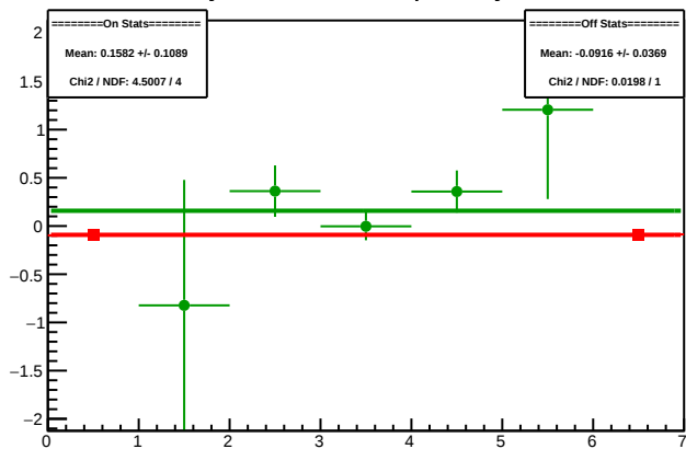
Cycle 5695.1: Multiplet Asyms
