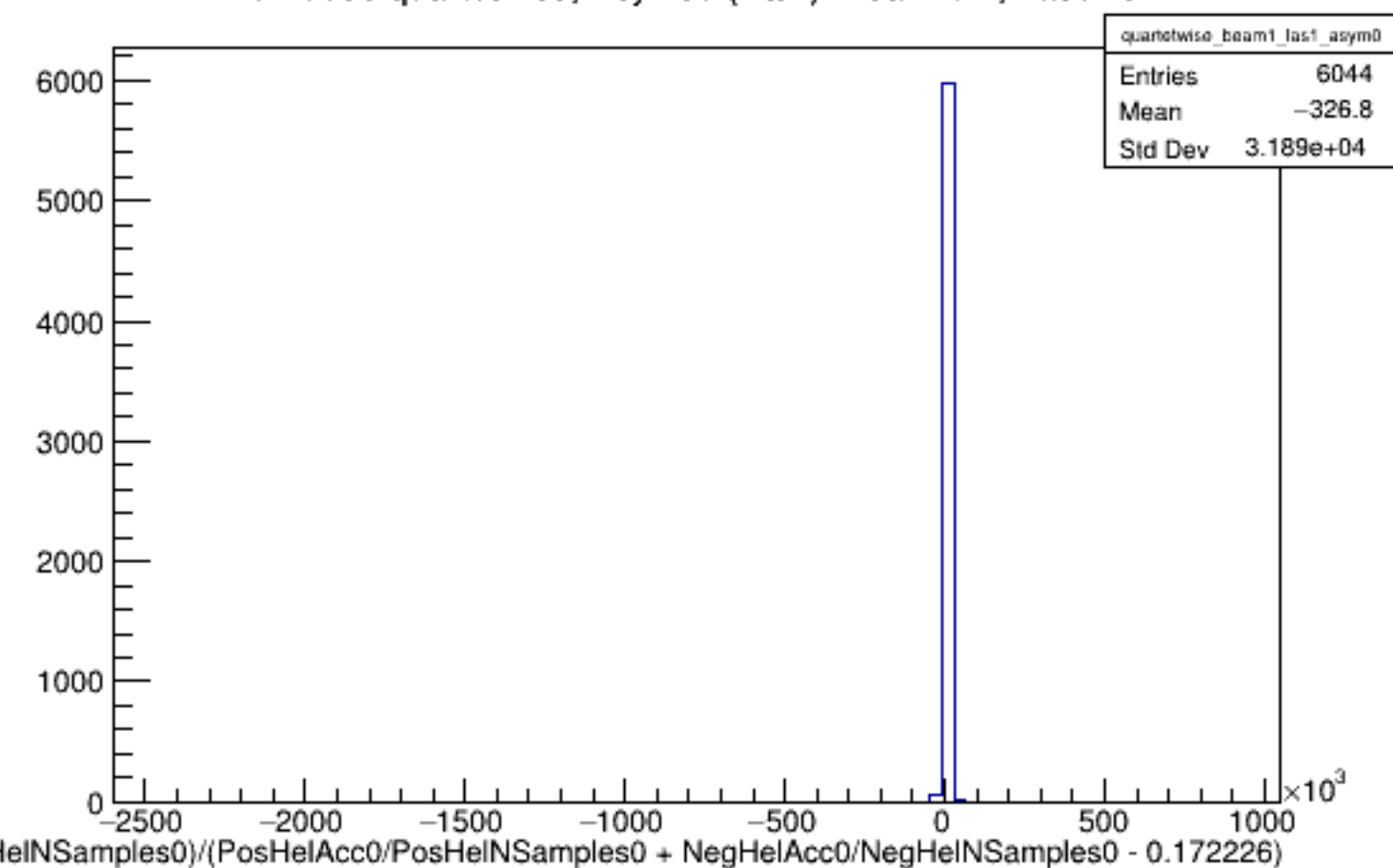
Run 5695 quartetwise, Asyms0 (Raw): Beam ON, Laser ON
