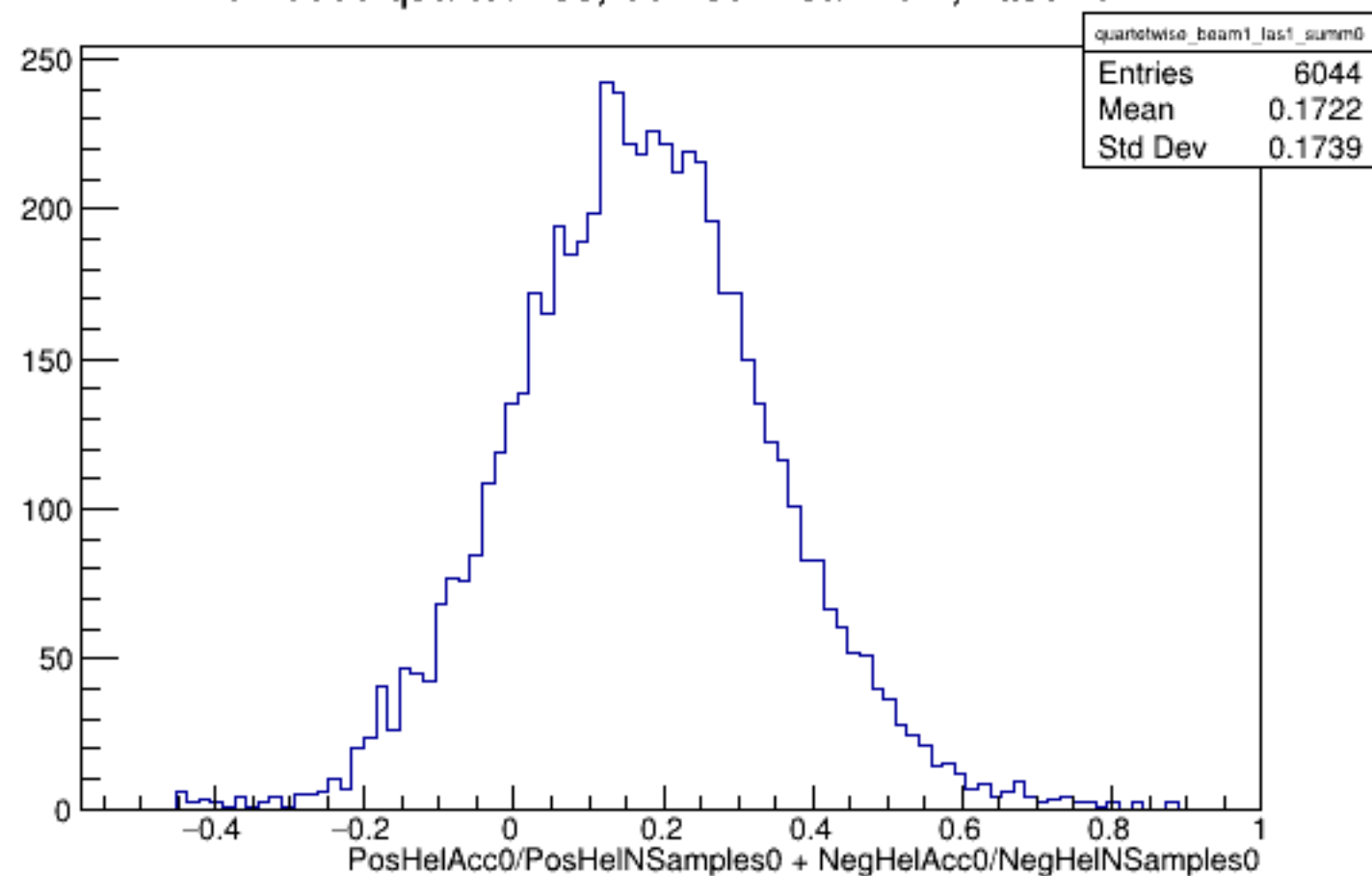
Run 5695 quartetwise, Sums0: Beam ON, Laser ON
