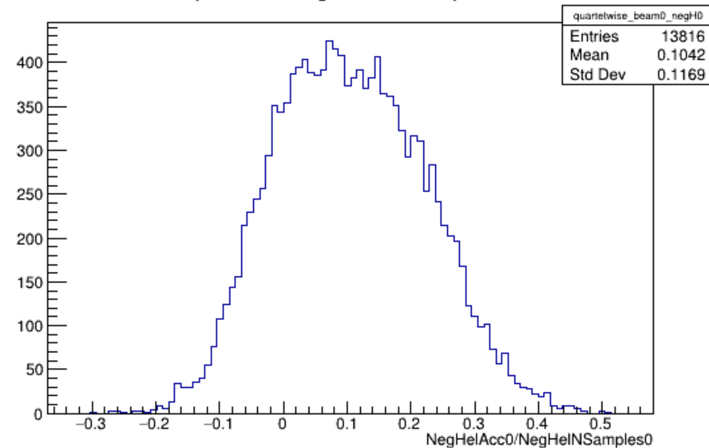
Run 5695 quartetwise, NegHelAcc0/NSamples0: Beam OFF
