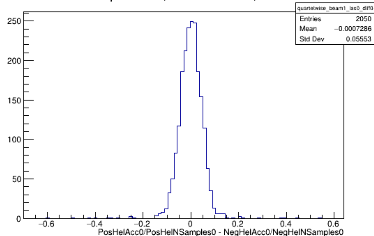
Run 5695 quartetwise, Diffs0: Beam ON, Laser OFF
