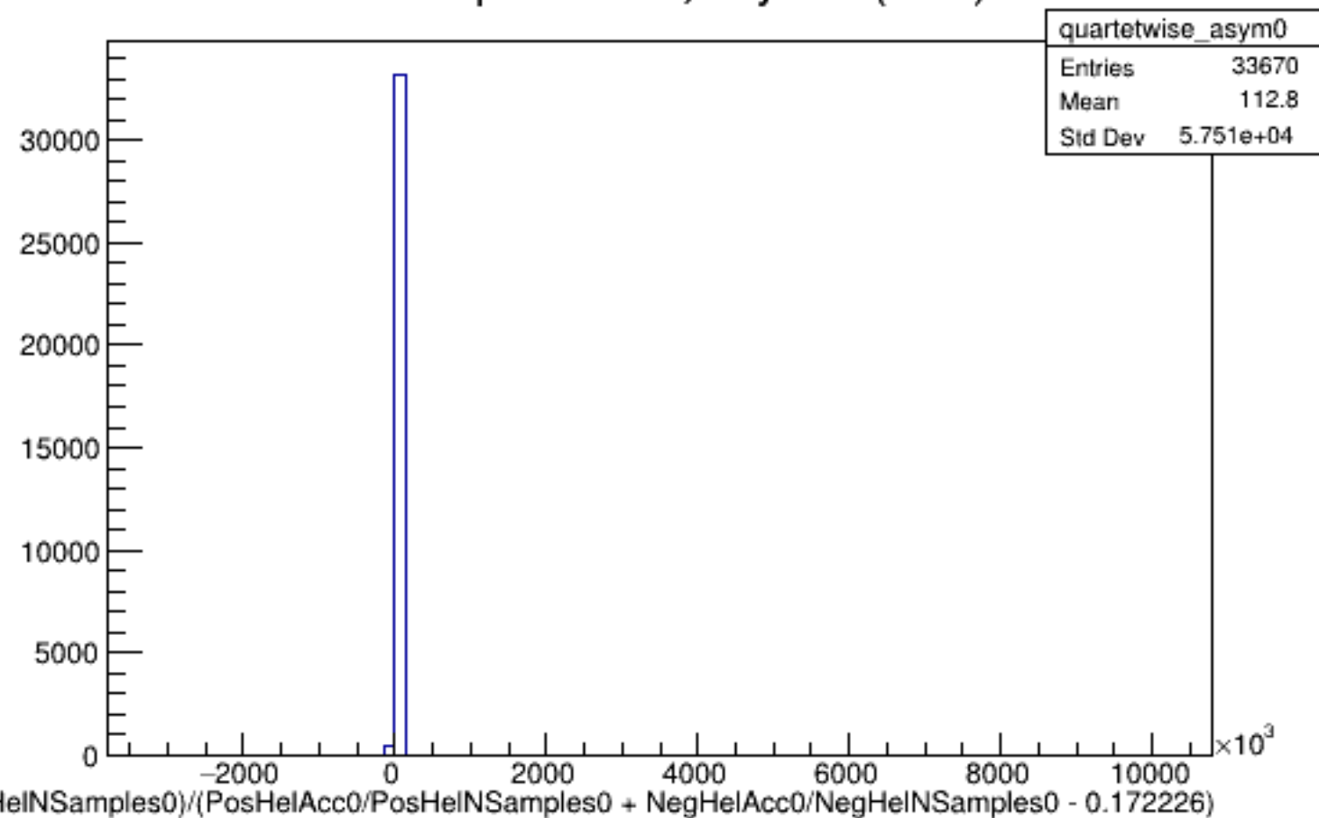
Run 5695 quartetwise, Asyms0 (Raw): All
