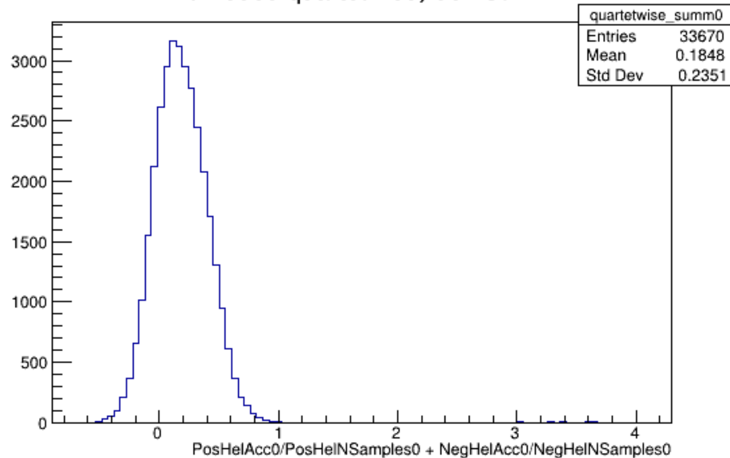
Run 5695 quartetwise, Sums0: All
