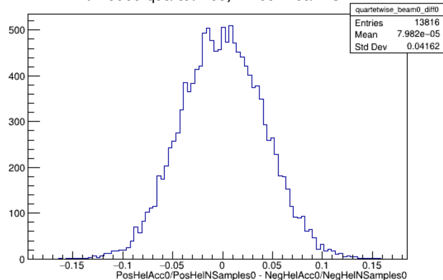
Run 5695 quartetwise, Diffs0: Beam OFF
