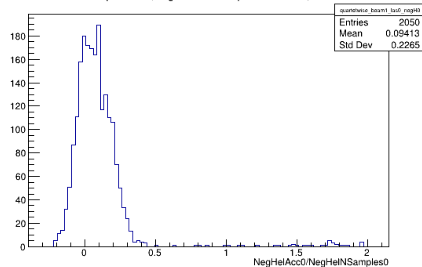
Run 5695 quartetwise, NegHelAcc0/NSamples0: Beam ON, Laser OFF
