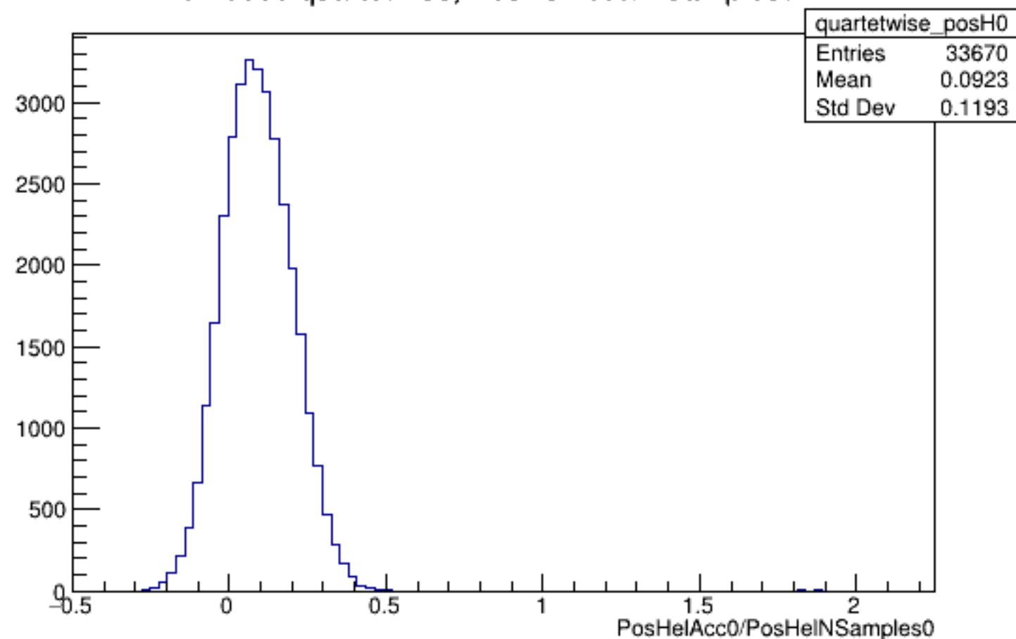
Run 5695 quartetwise, PosHelAcc0/NSamples0: All
