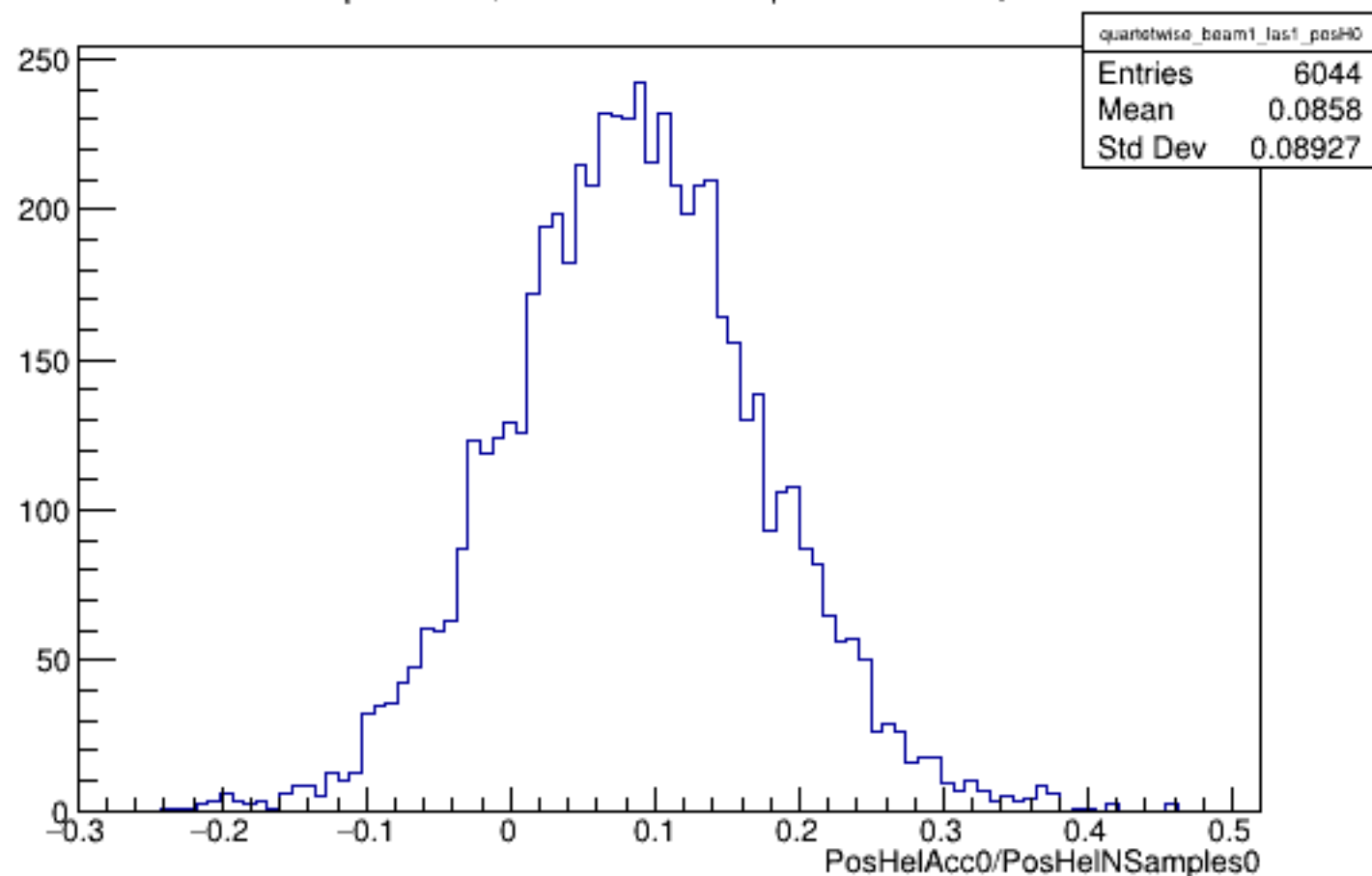
Run 5695 quartetwise, PosHelAcc0/NSamples0: Beam ON, Laser ON
