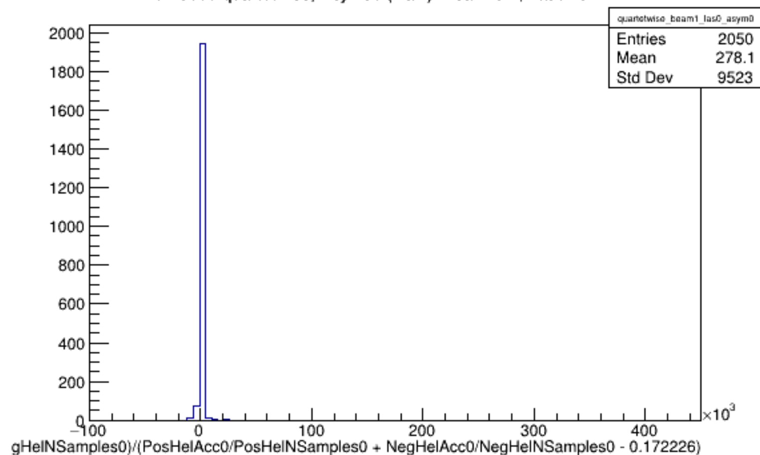
Run 5695 quartetwise, Asyms0 (Raw): Beam ON, Laser OFF
