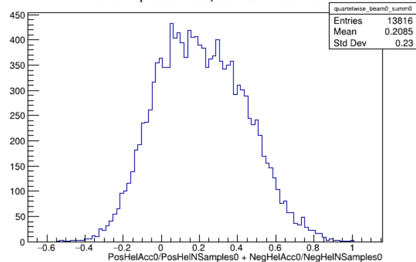
Run 5695 quartetwise, Sums0: Beam OFF
