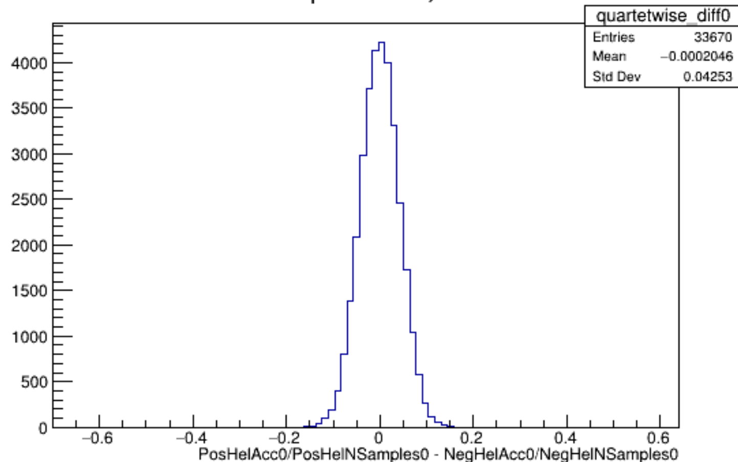
Run 5695 quartetwise, Diffs0: All
