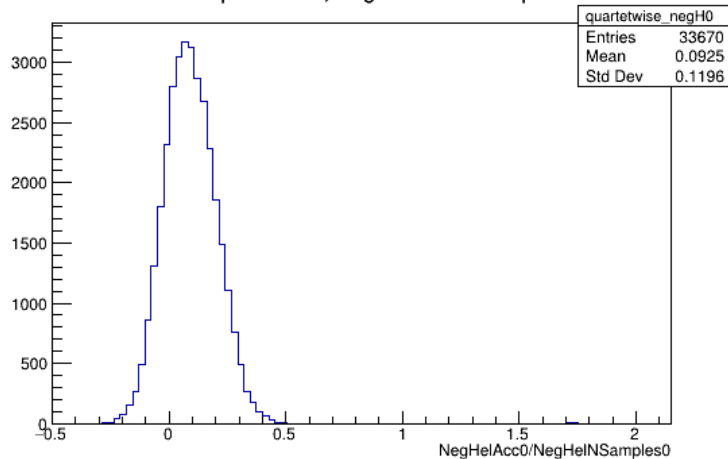
Run 5695 quartetwise, NegHelAcc0/NSamples0: All
