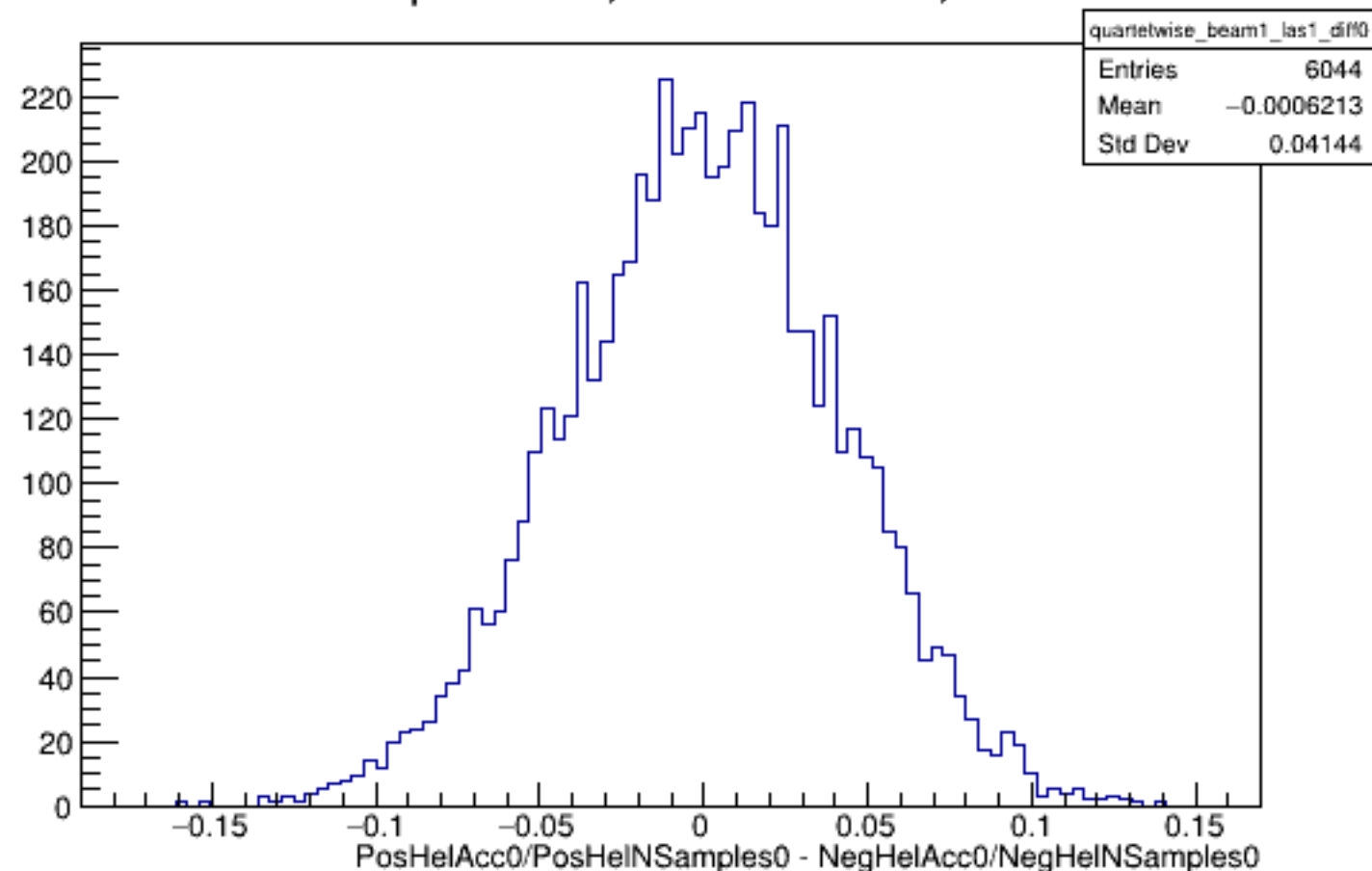
Run 5695 quartetwise, Diffs0: Beam ON, Laser ON
