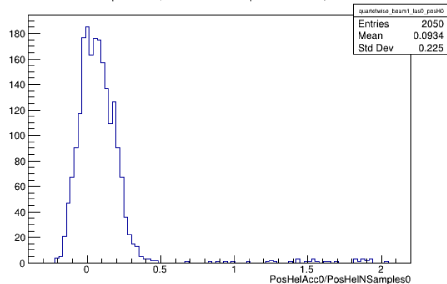
Run 5695 quartetwise, PosHelAcc0/NSamples0: Beam ON, Laser OFF
