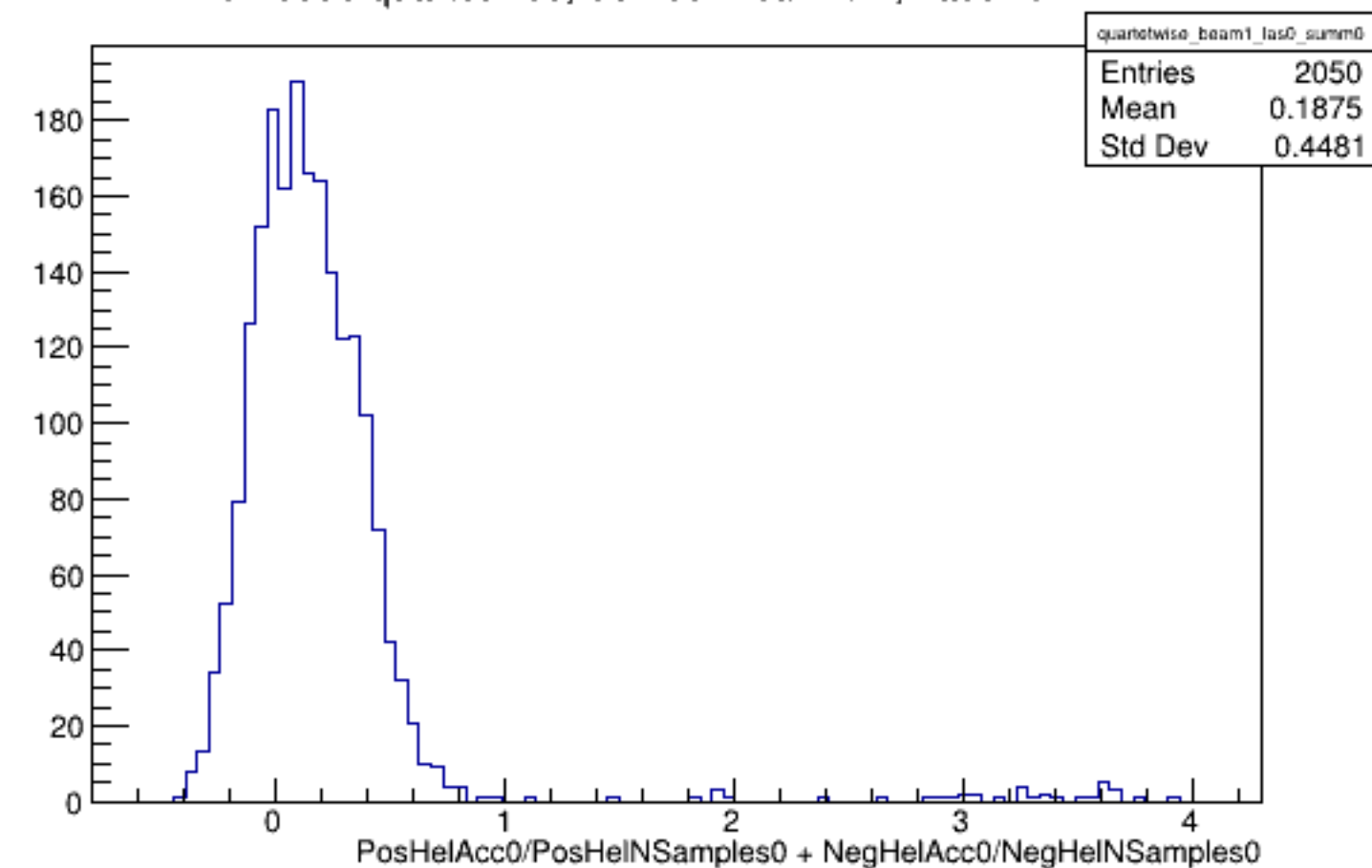
Run 5695 quartetwise, Sums0: Beam ON, Laser OFF
