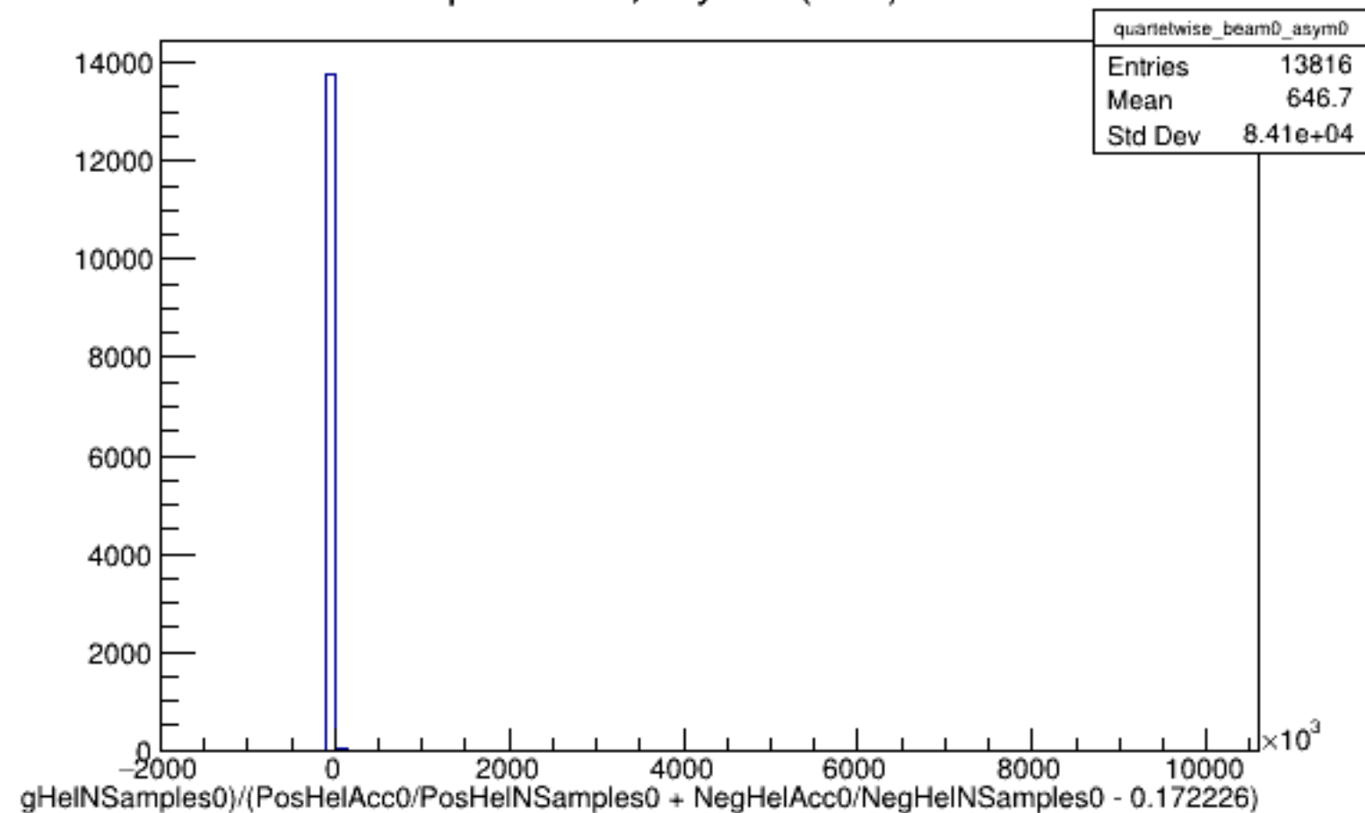
Run 5695 quartetwise, Asyms0 (Raw): Beam OFF
