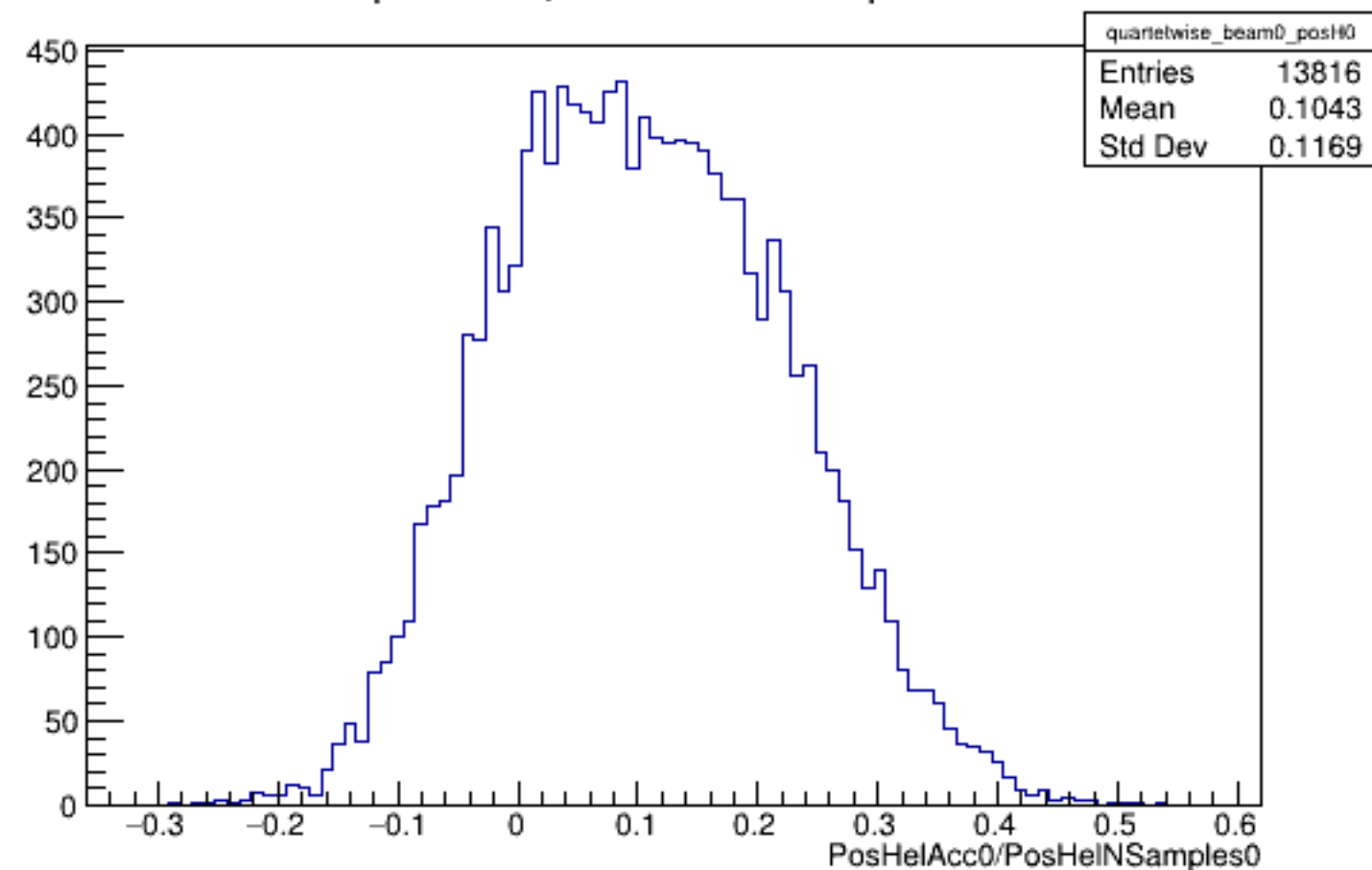
Run 5695 quartetwise, PosHelAcc0/NSamples0: Beam OFF
