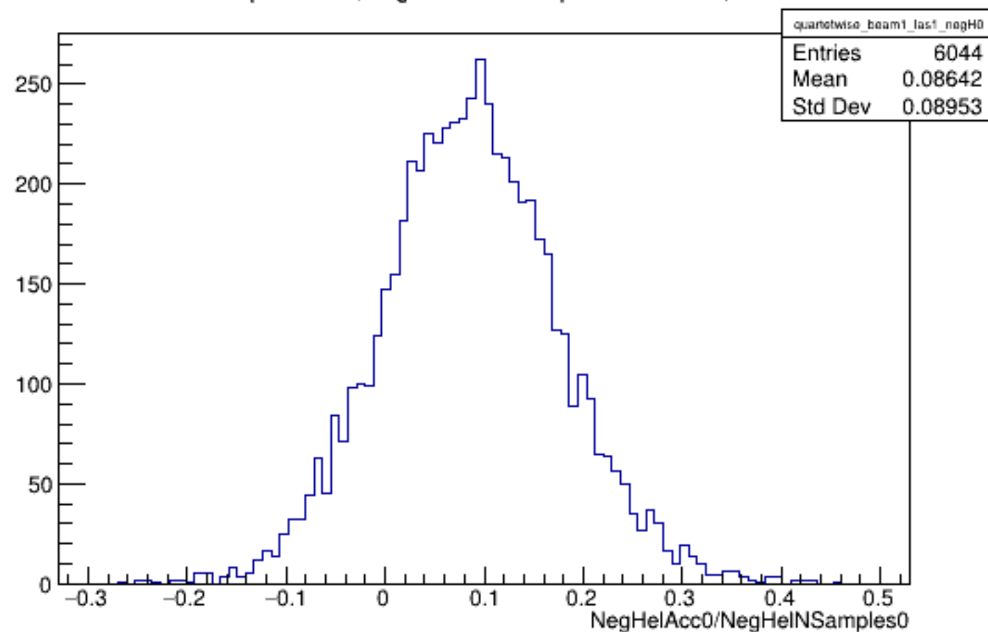
Run 5695 quartetwise, NegHelAcc0/NSamples0: Beam ON, Laser ON
