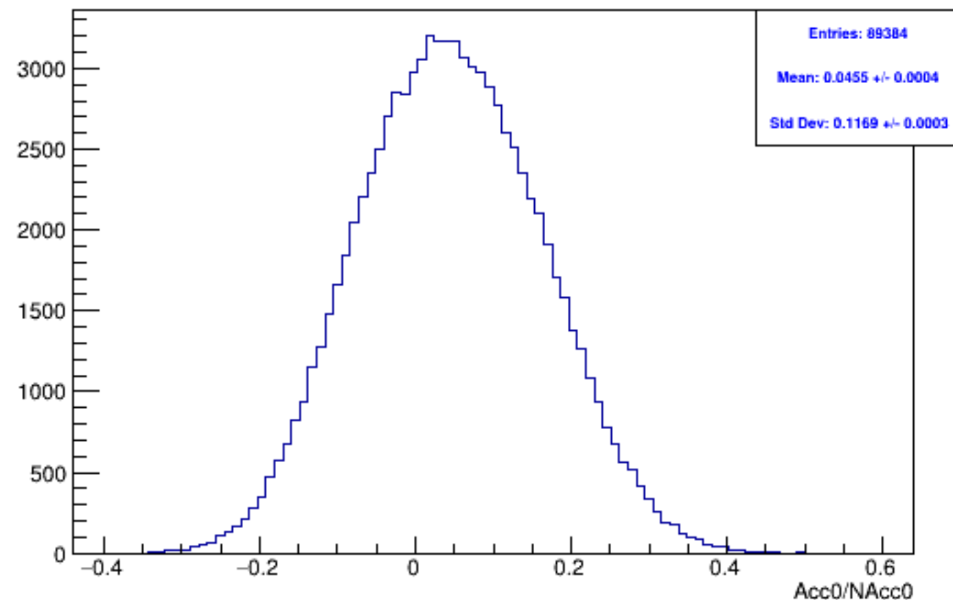
Run 5700 mpwise, acc0: Beam OFF
