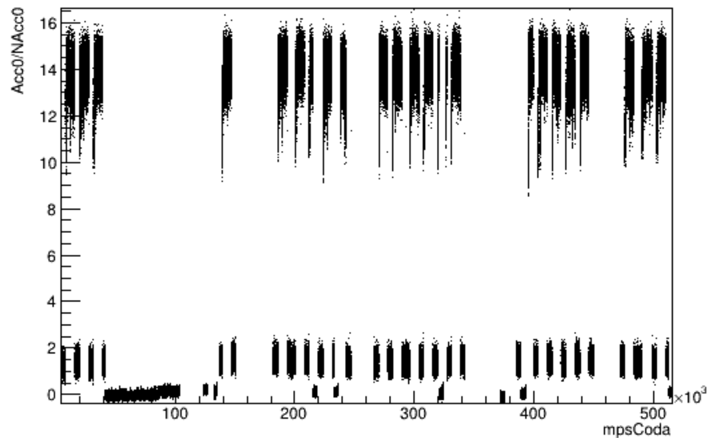
Run 5700 mpwise, Acc0 vs Time: All
