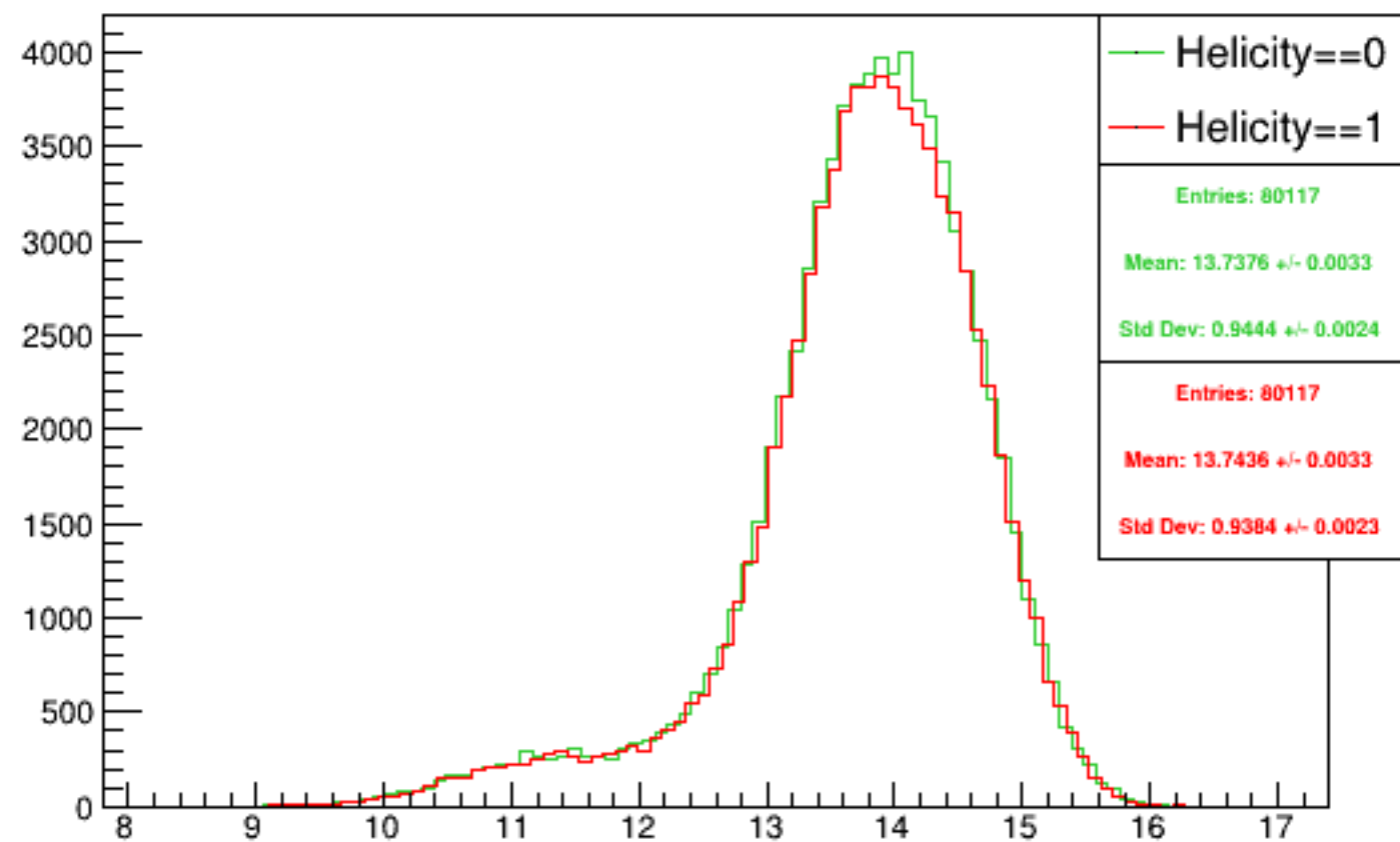
Run 5700 mpwise, acc0: Beam ON, Laser ON
