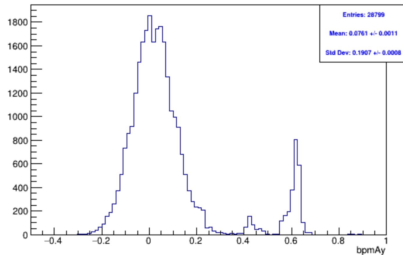
Run 5701 mpwise, bpmAy: Beam OFF
