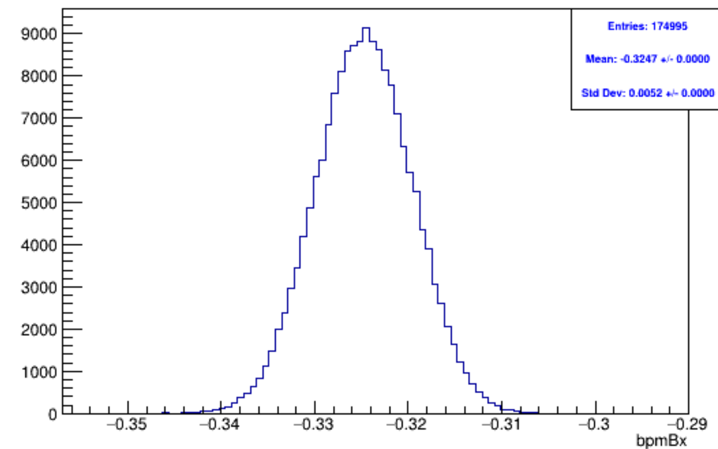
Run 5701, mpswise, bpmBx: Beam ON, Laser OFF
