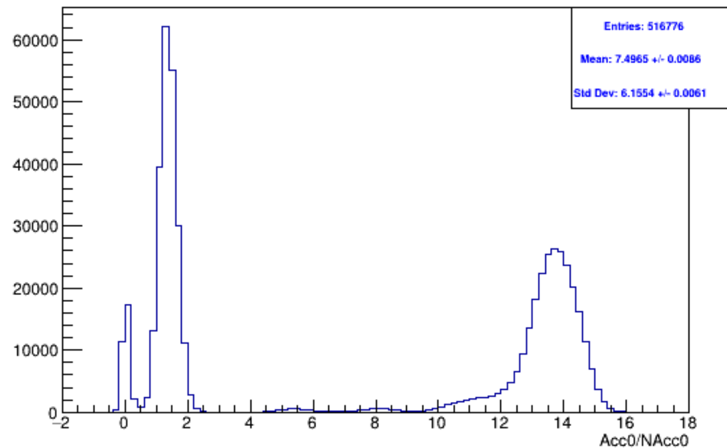
Run 5701 mpwise, acc0: All
