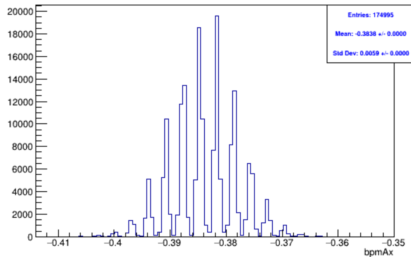
Run 5701, mpwise, bpmAx: Beam ON, Laser OFF
