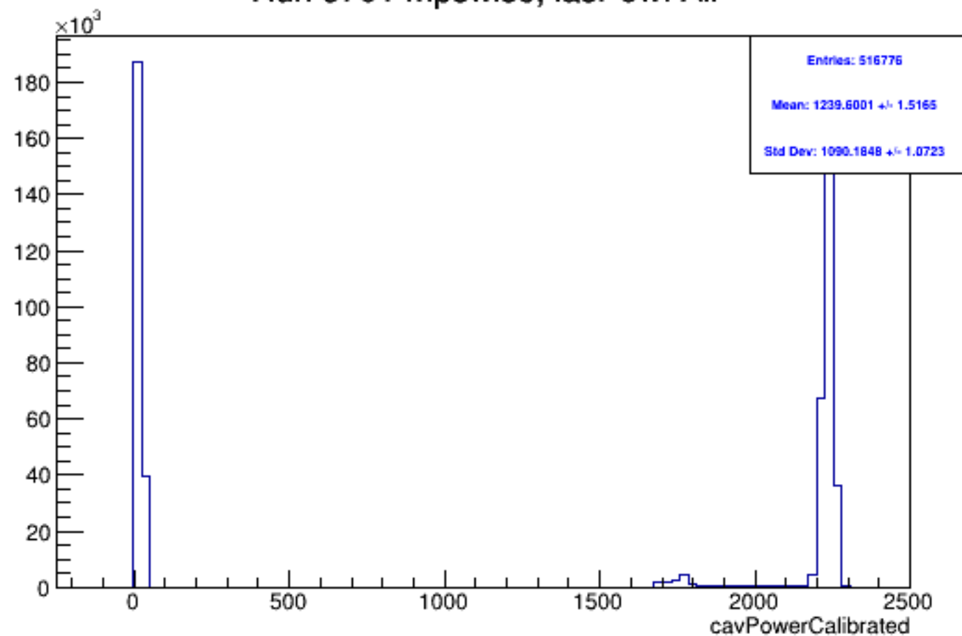
Run 5701 mpwise, lasPow: All
