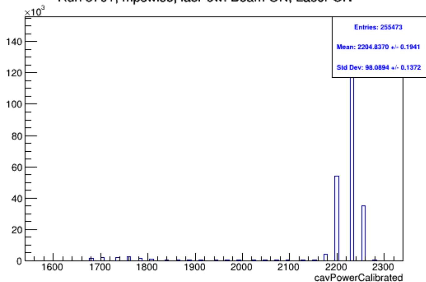
Run 5701, mpwise, lasPow: Beam ON, Laser ON
