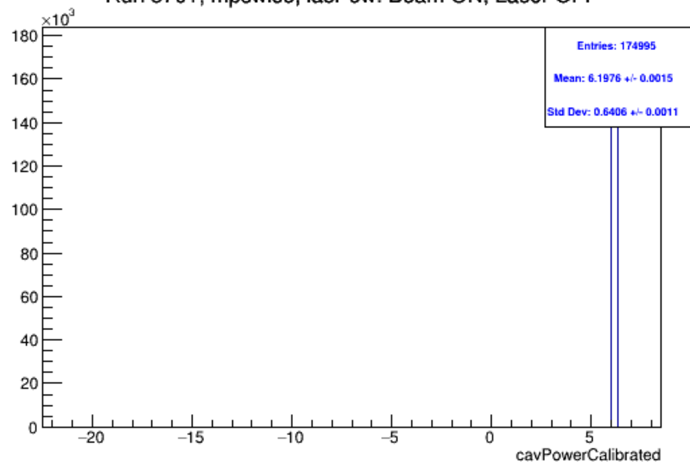
Run 5701, mpwise, lasPow: Beam ON, Laser OFF
