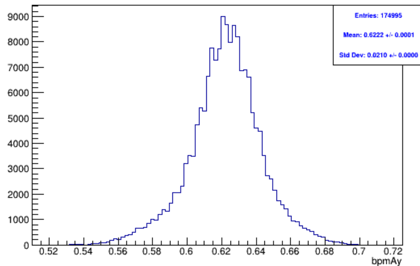
Run 5701, mpwise, bpmAy: Beam ON, Laser OFF
