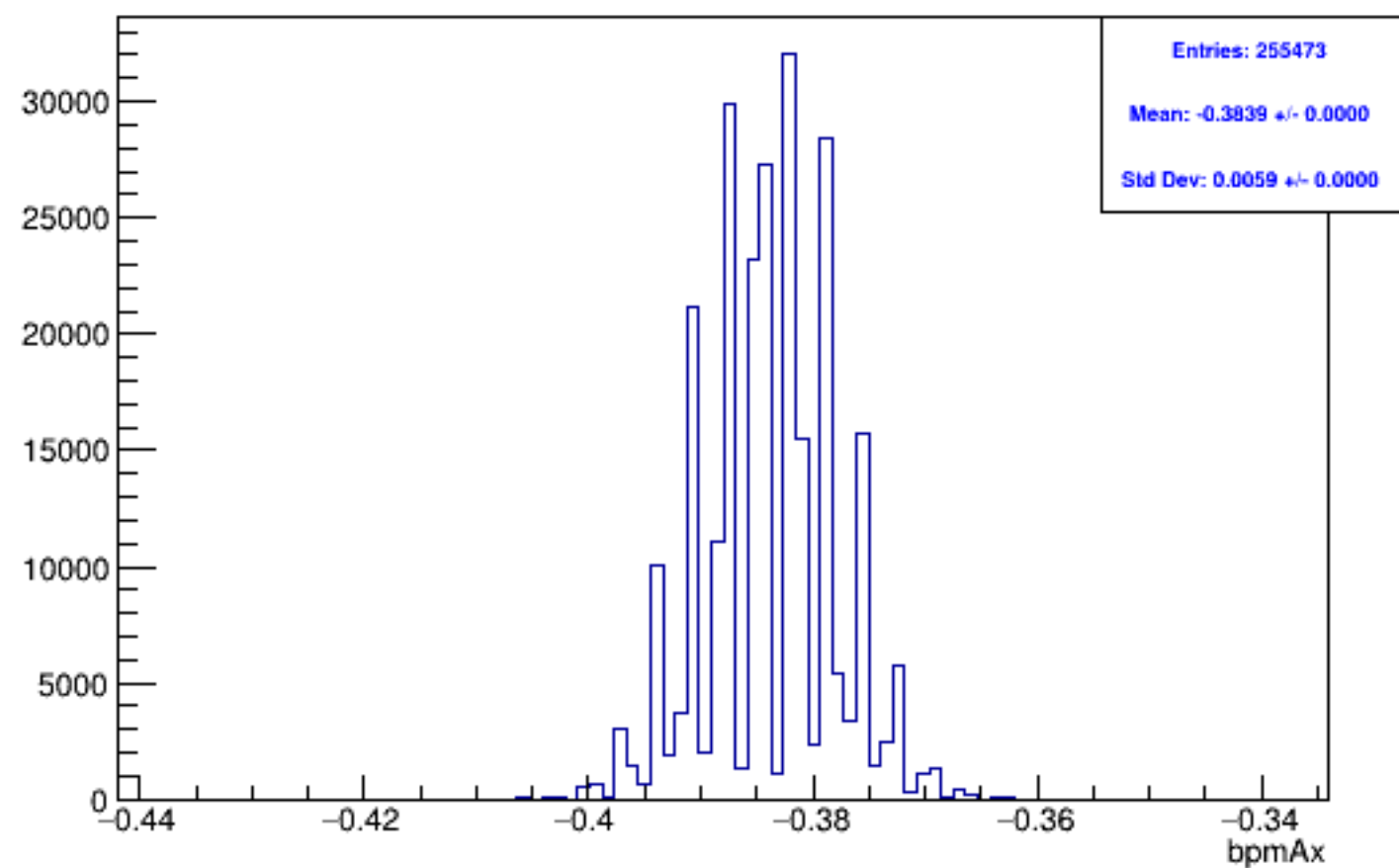
Run 5701, mpwise, bpmAx: Beam ON, Laser ON
