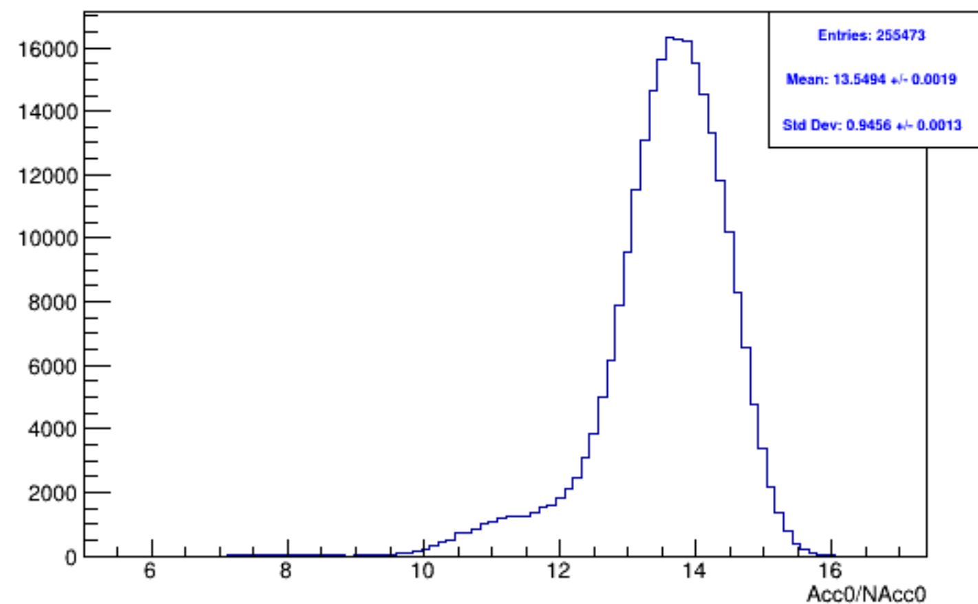
Run 5701, mpwise, acc0: Beam ON, Laser ON
