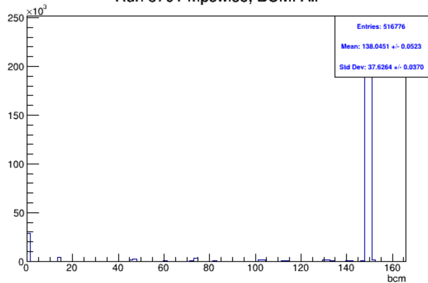
Run 5701 mpwise, BCM: All
