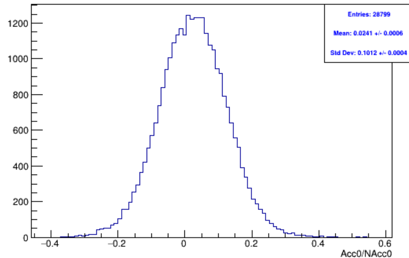
Run 5701 mpwise, acc0: Beam OFF
