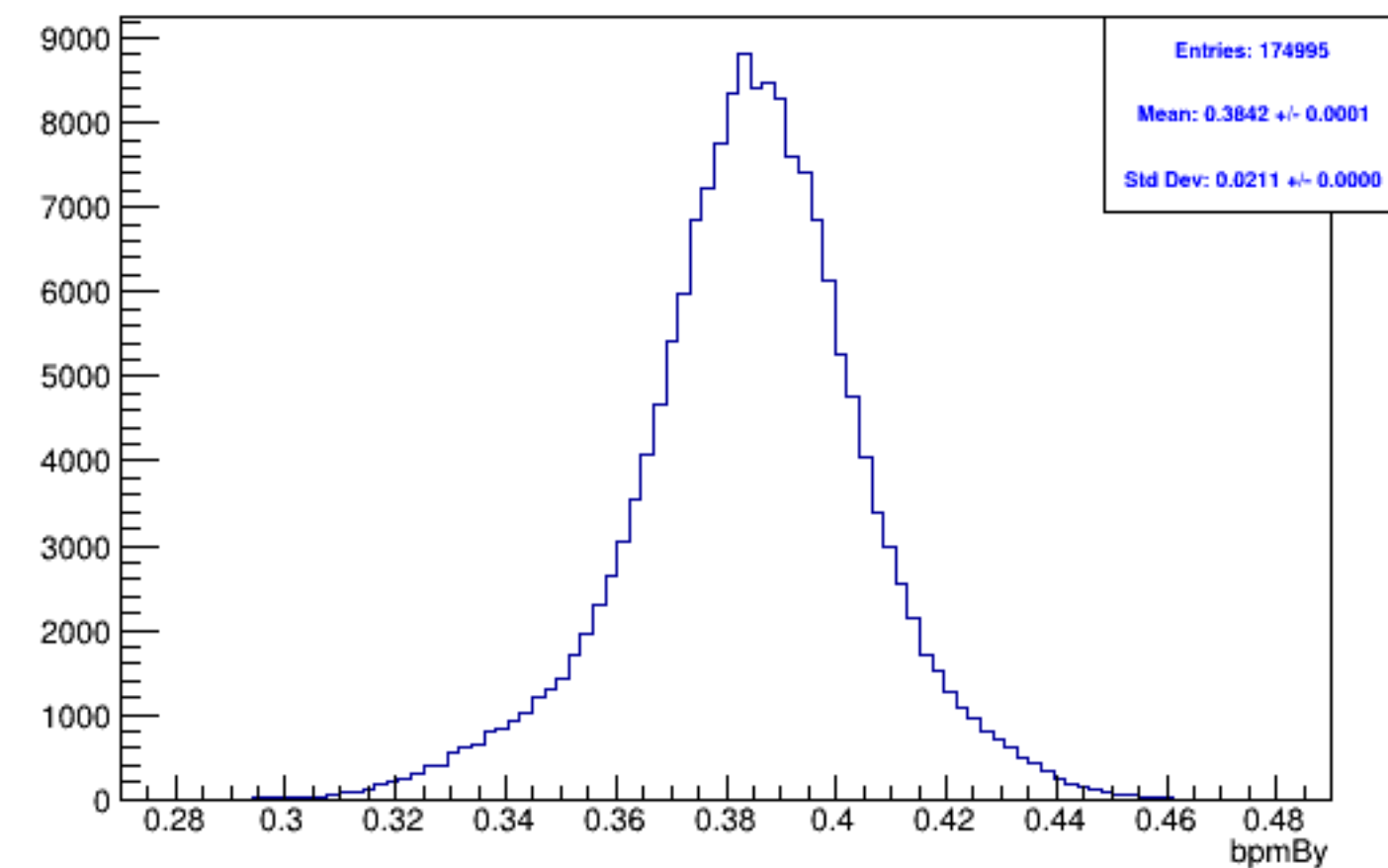
Run 5701, mpswise, bpmBy: Beam ON, Laser OFF
