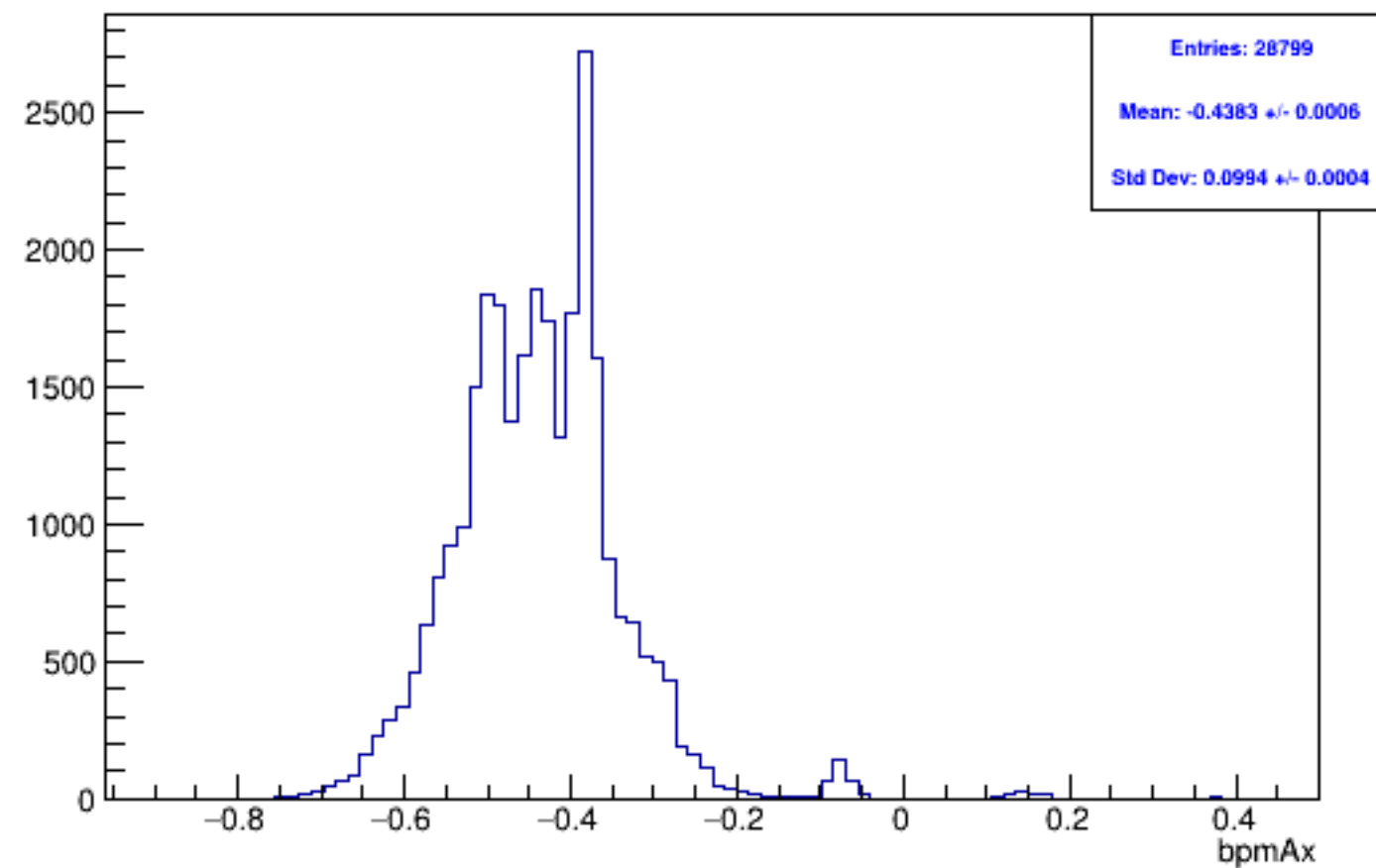
Run 5701 mpwise, bpmAx: Beam OFF
