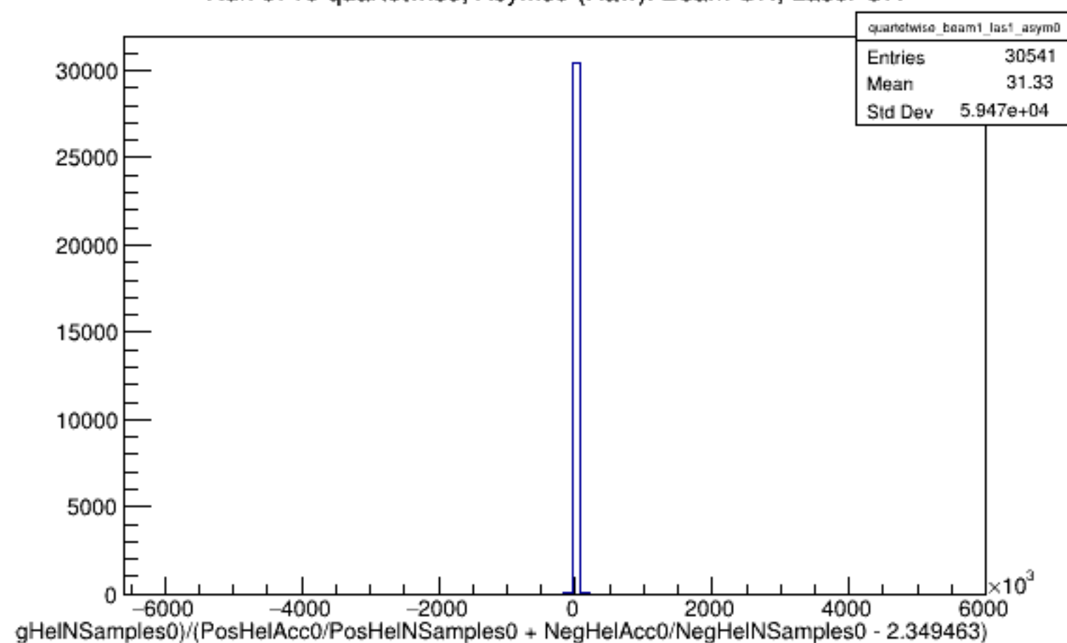
Run 5719 quartetwise, Asyms0 (Raw): Beam ON, Laser ON
