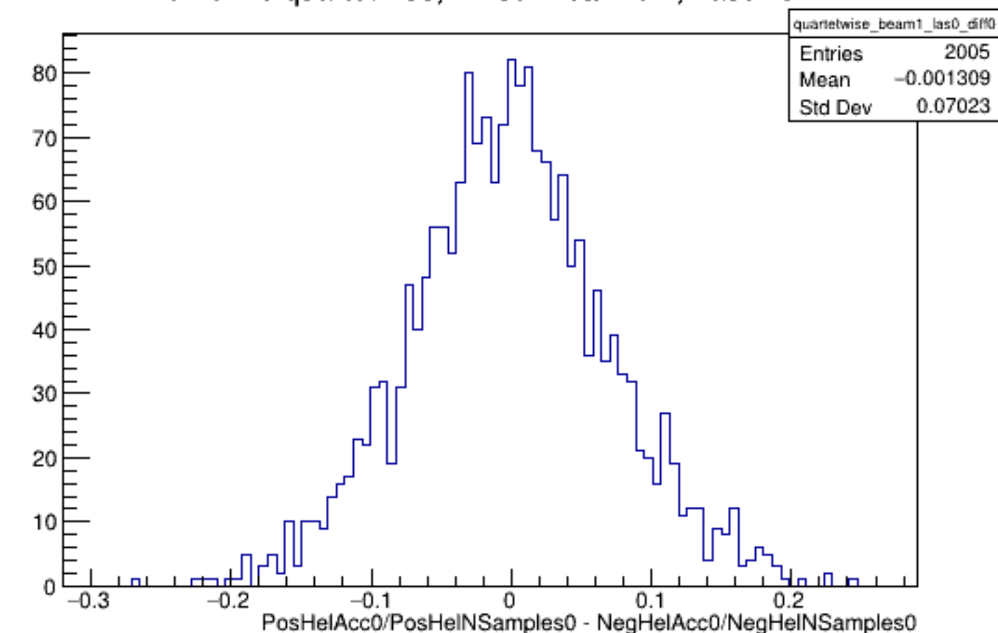
Run 5719 quartetwise, Diffs0: Beam ON, Laser OFF
