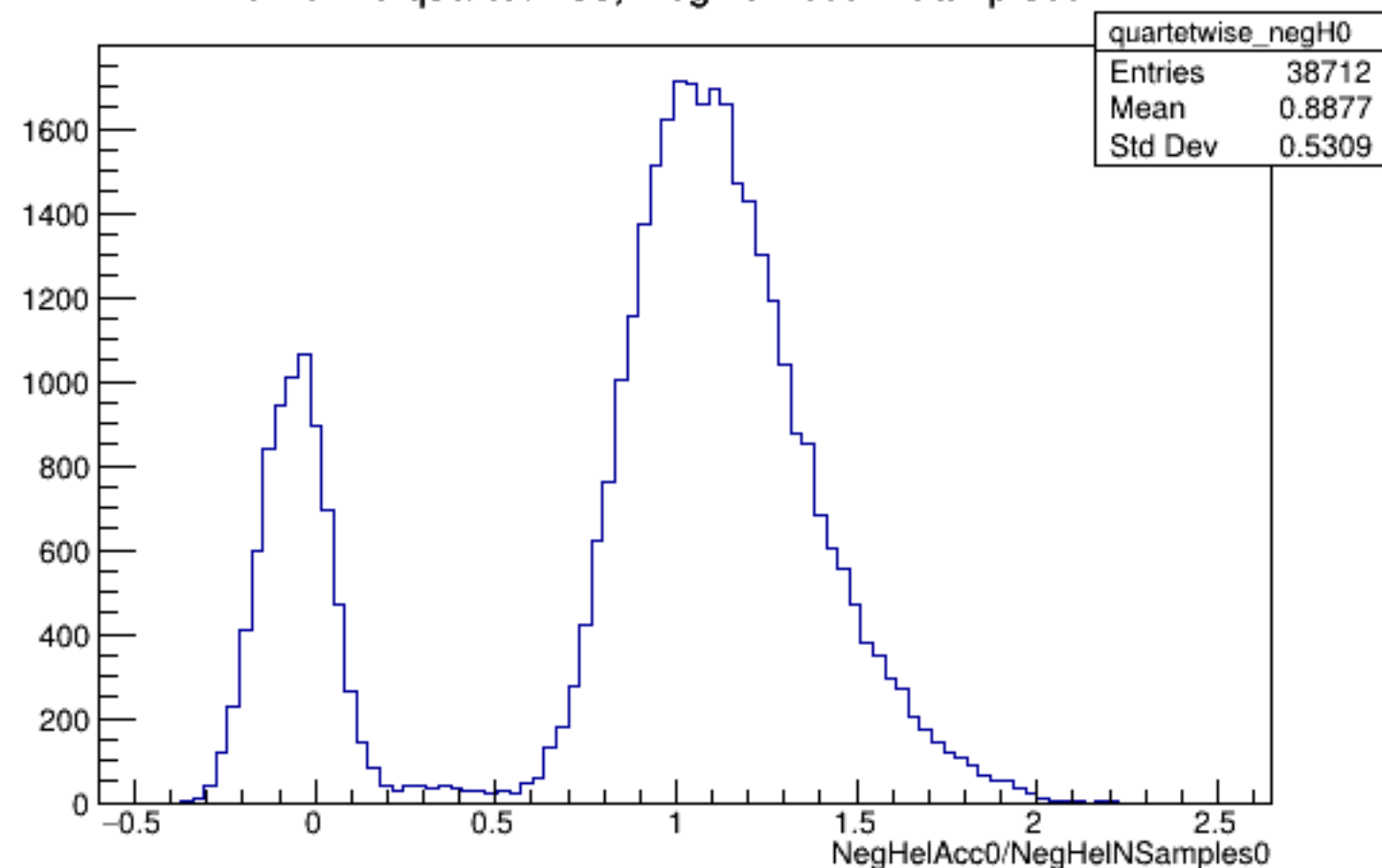
Run 5719 quartetwise, NegHelAcc0/NSamples0: All
