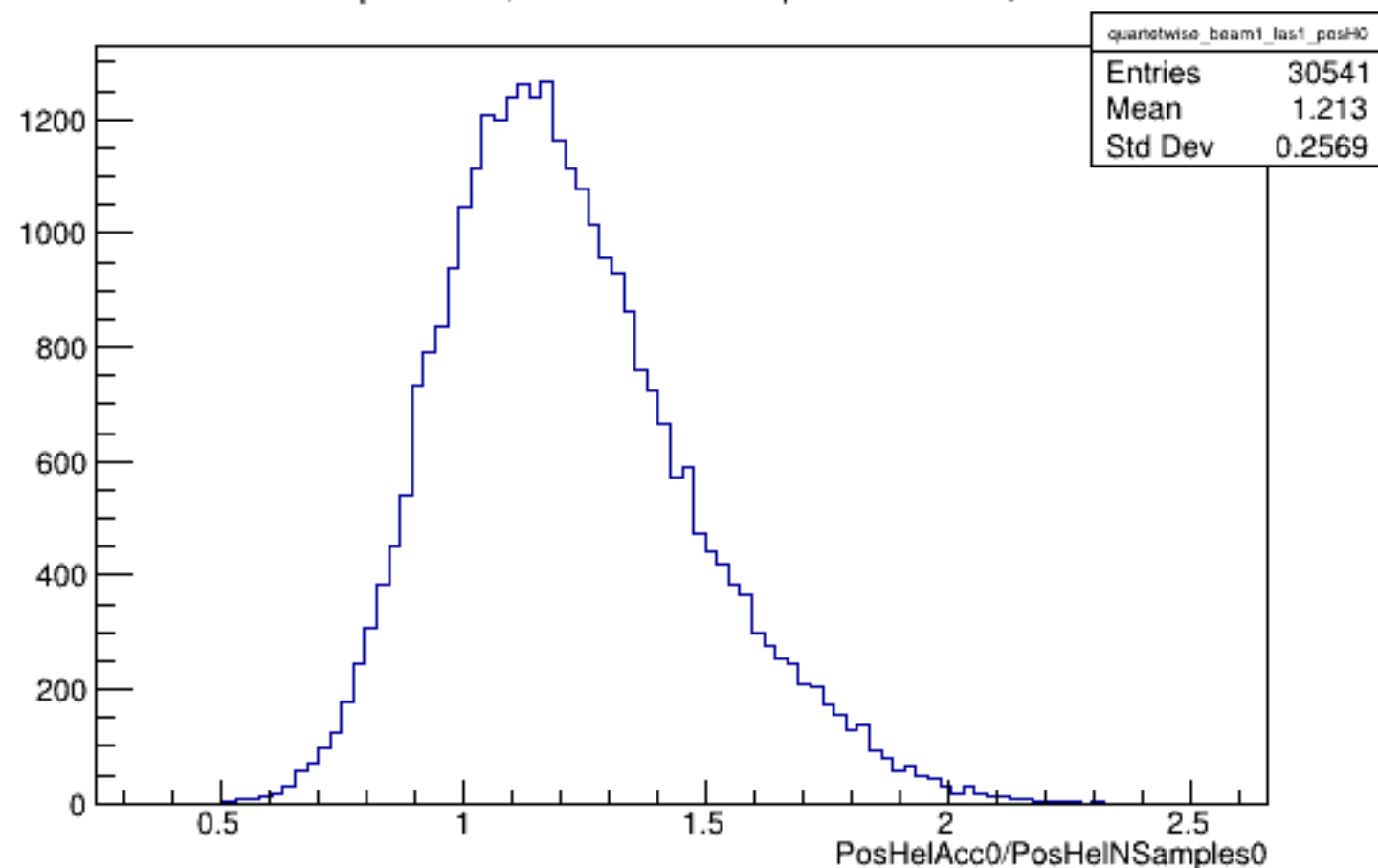
Run 5719 quartetwise, PosHelAcc0/NSamples0: Beam ON, Laser ON
