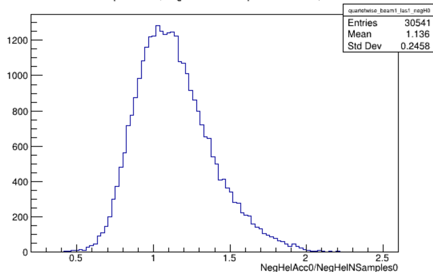
Run 5719 quartetwise, NegHelAcc0/NSamples0: Beam ON, Laser ON
