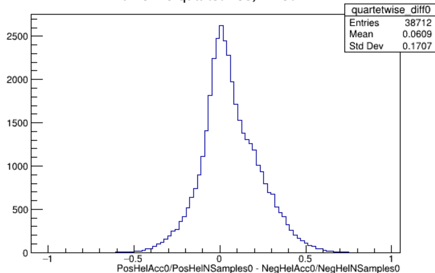
Run 5719 quartetwise, Diffs0: All
