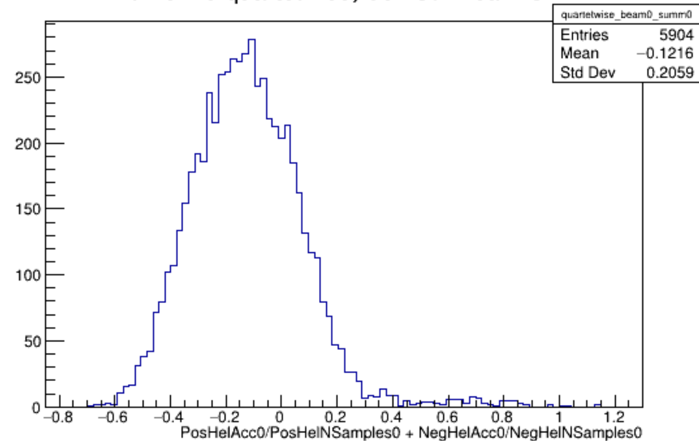
Run 5719 quartetwise, Sums0: Beam OFF
