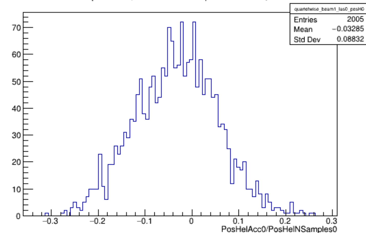
Run 5719 quartetwise, PosHelAcc0/NSamples0: Beam ON, Laser OFF
