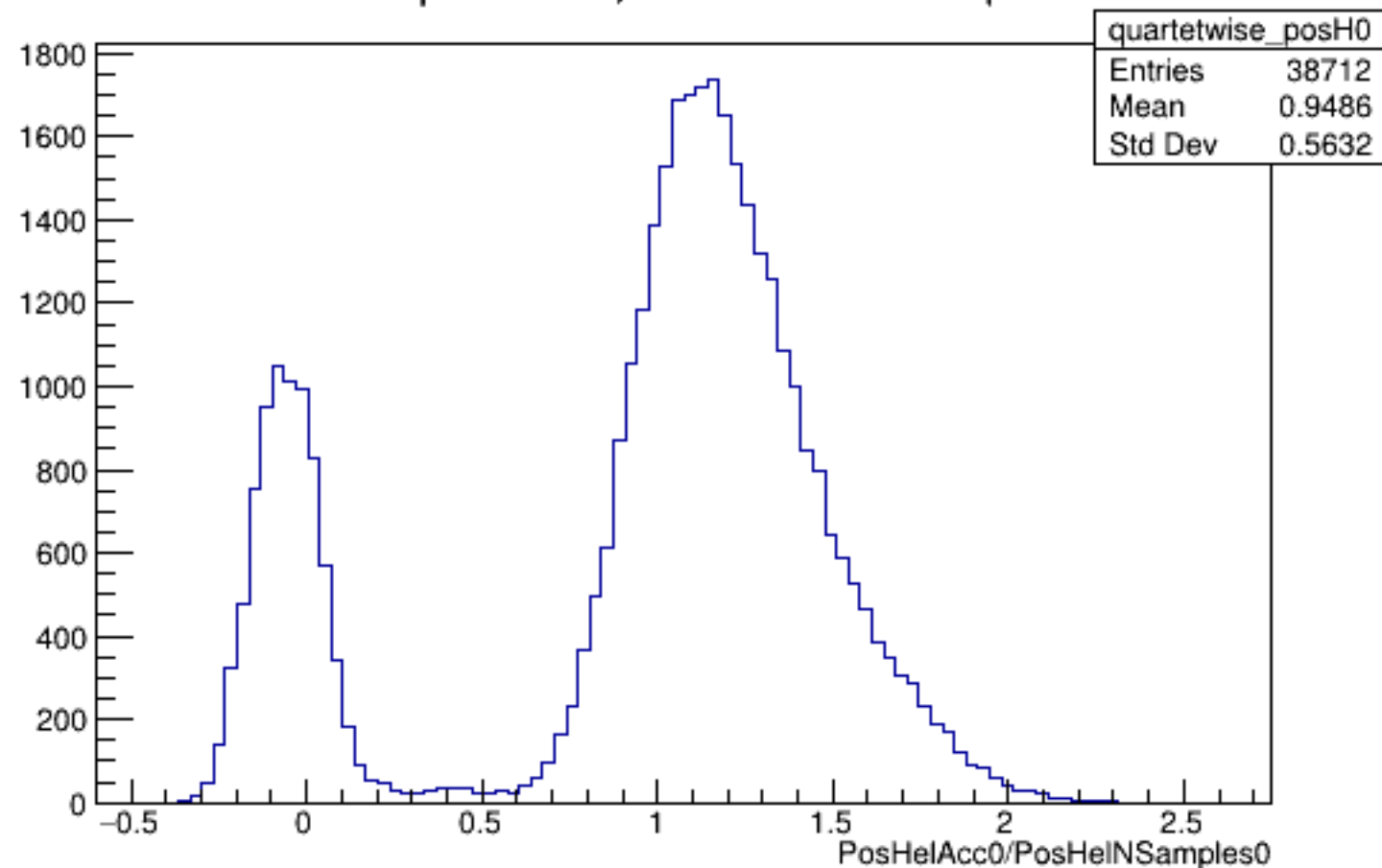
Run 5719 quartetwise, PosHelAcc0/NSamples0: All
