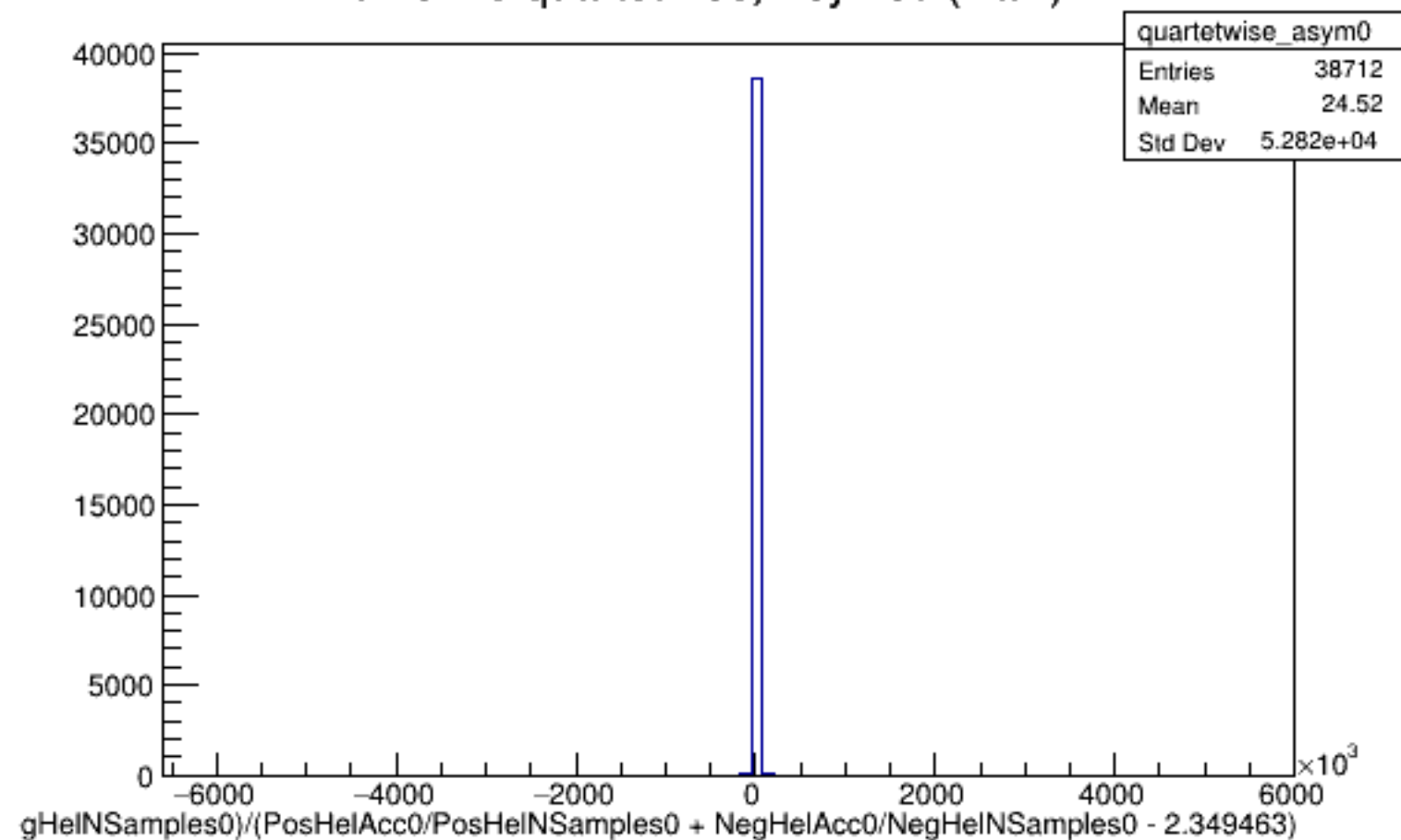
Run 5719 quartetwise, Asyms0 (Raw): All
