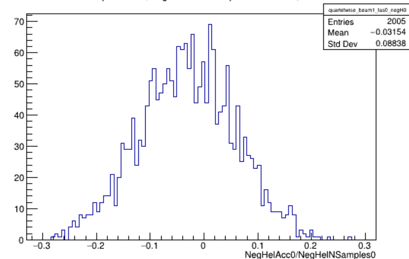
Run 5719 quartetwise, NegHelAcc0/NSamples0: Beam ON, Laser OFF
