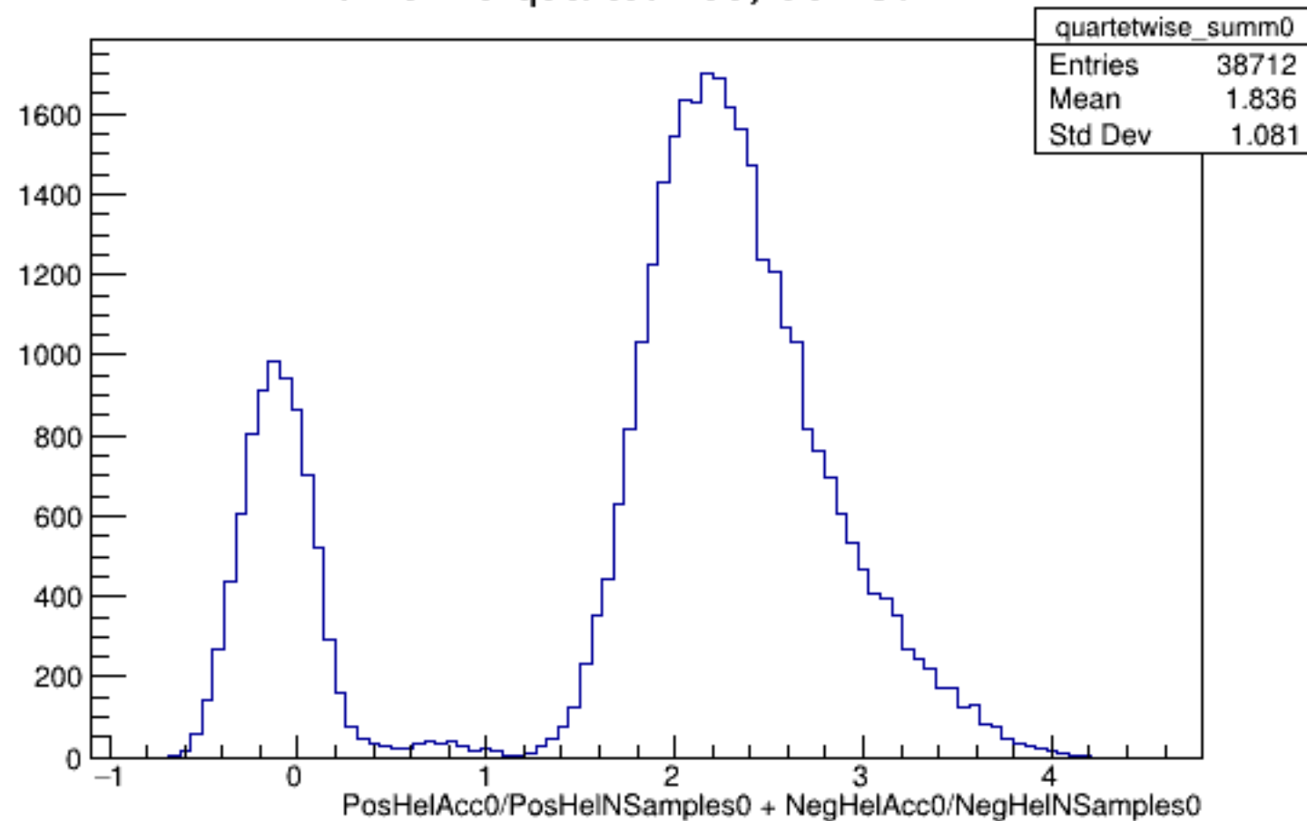
Run 5719 quartetwise, Sums0: All
