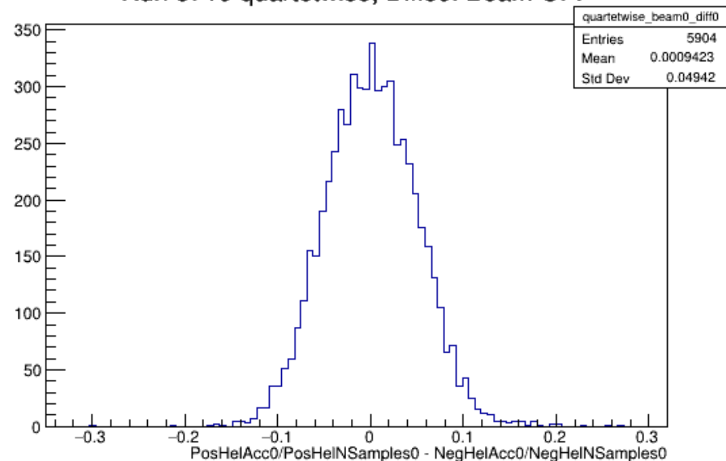
Run 5719 quartetwise, Diffs0: Beam OFF
