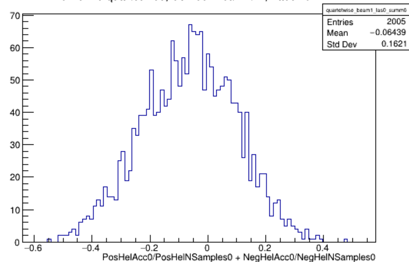
Run 5719 quartetwise, Sums0: Beam ON, Laser OFF
