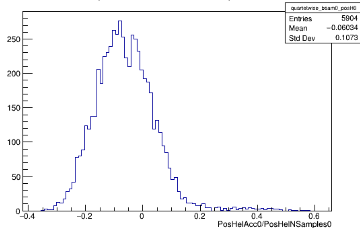
Run 5719 quartetwise, PosHelAcc0/NSamples0: Beam OFF
