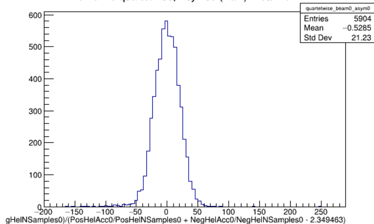
Run 5719 quartetwise, Asyms0 (Raw): Beam OFF
