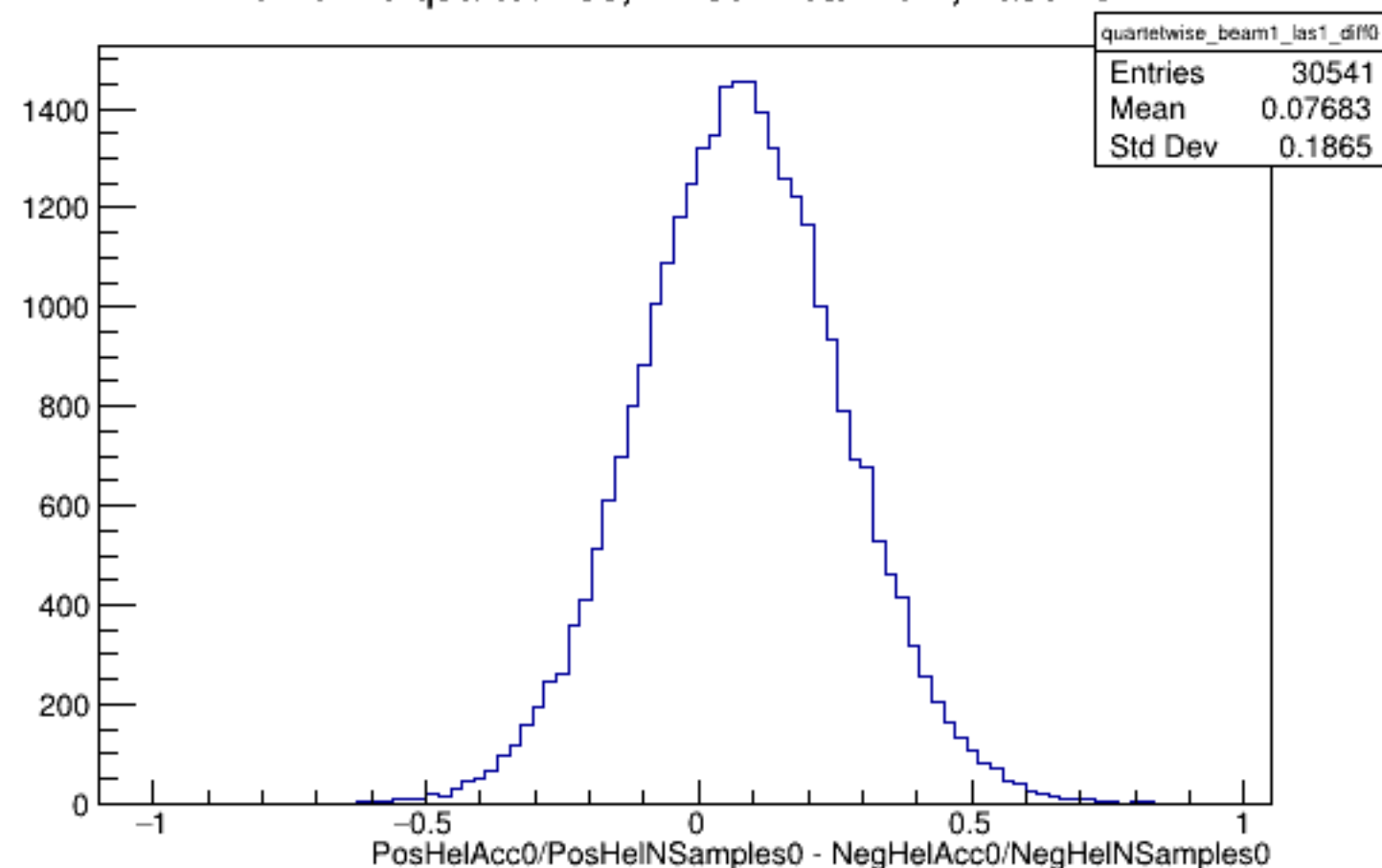
Run 5719 quartetwise, Diffs0: Beam ON, Laser ON
