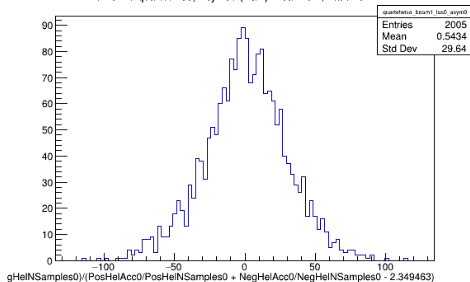
Run 5719 quartetwise, Asyms0 (Raw): Beam ON, Laser OFF
