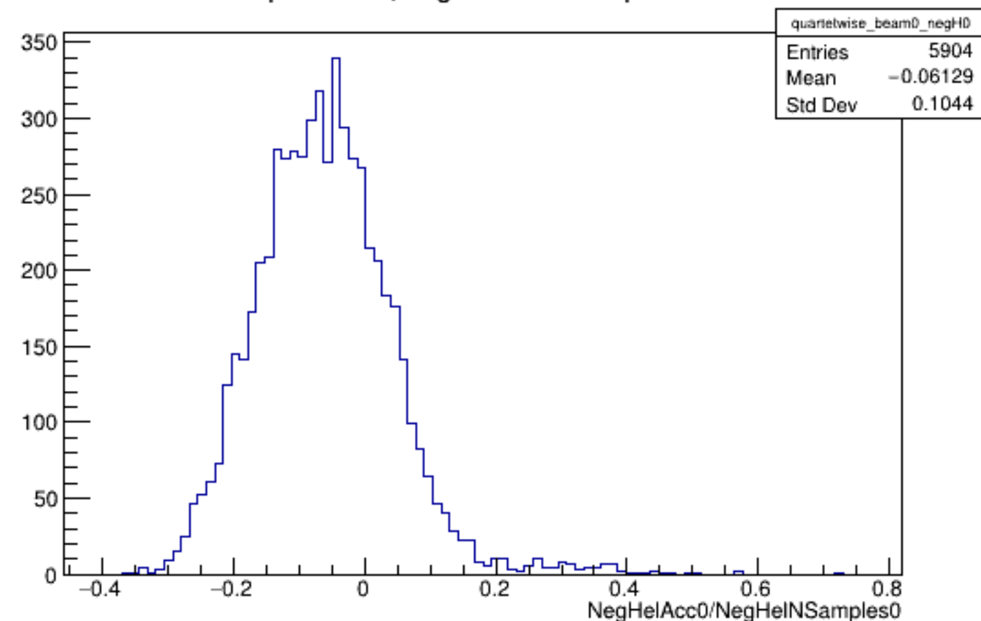
Run 5719 quartetwise, NegHelAcc0/NSamples0: Beam OFF
