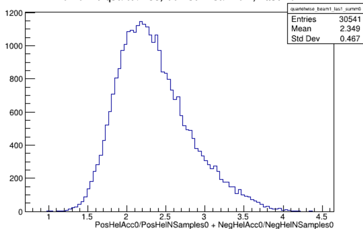
Run 5719 quartetwise, Sums0: Beam ON, Laser ON
