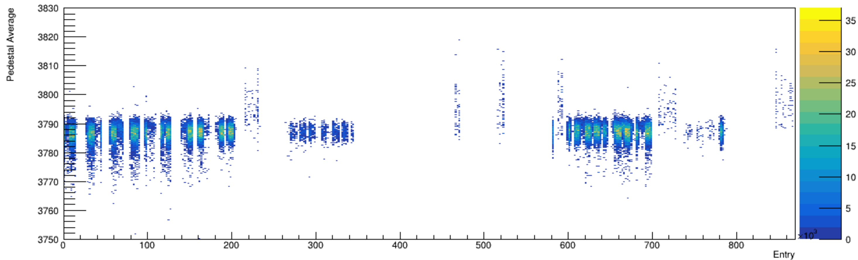
Run 5721, snapshots: Pedestal vs. Time
