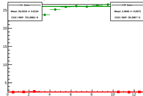
Cycle 5725.9: Multiplet Sums
