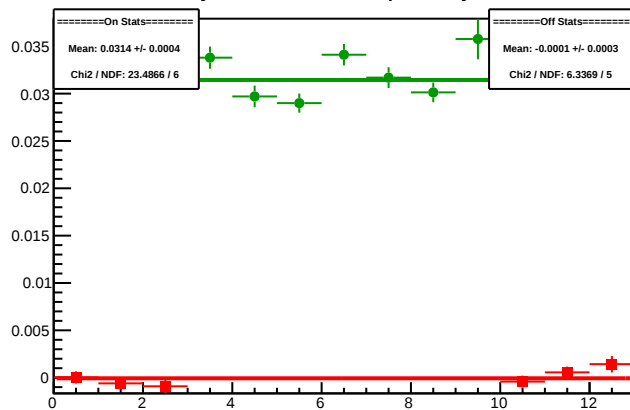
Cycle 5725.9: Multiplet Asyms
