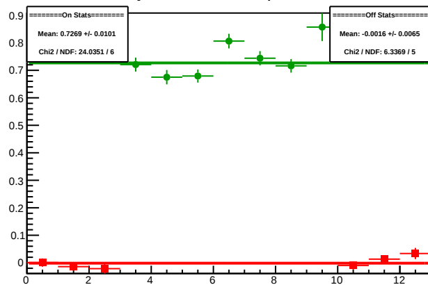
Cycle 5725.9: Multiplet Diffs
