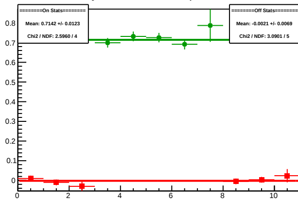
Cycle 5725.14: Multiplet Diffs
