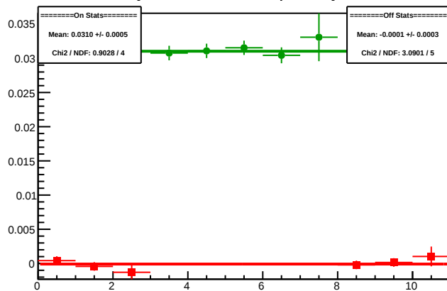
Cycle 5725.14: Multiplet Asyms
