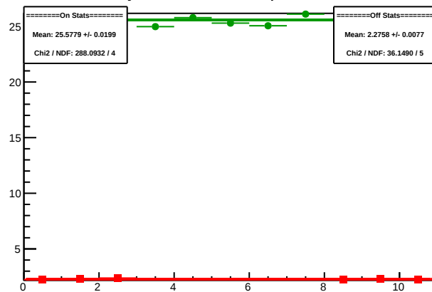
Cycle 5725.14: Multiplet Sums
