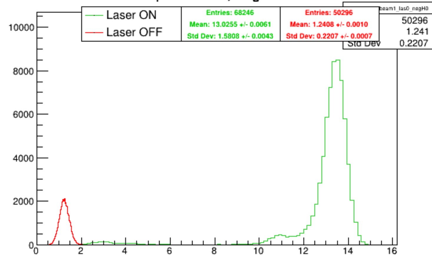
Run 5727 quartetwise, negH0: Beam ON
