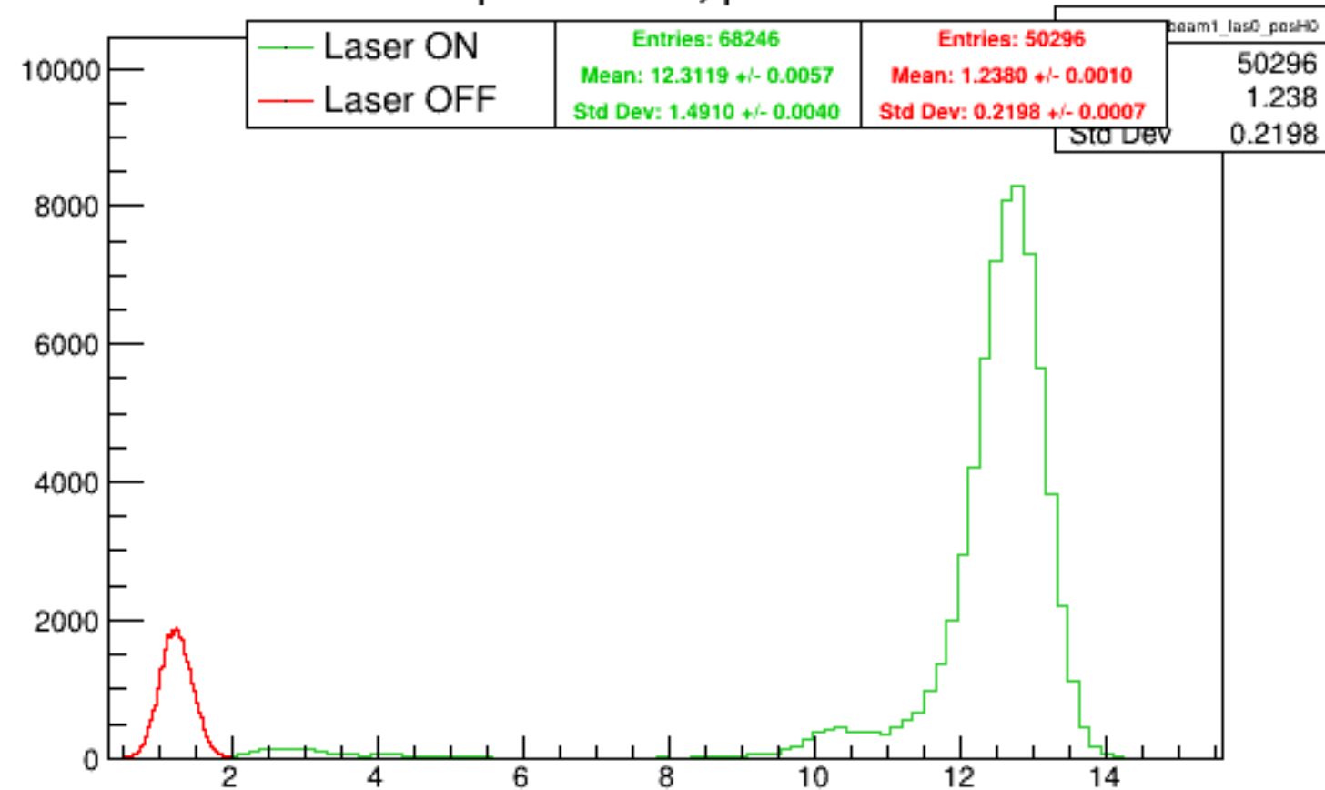
Run 5727 quartetwise, posH0: Beam ON
