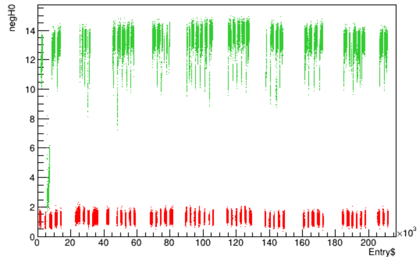
Run 5727 quartetwise, negH0 vs time
