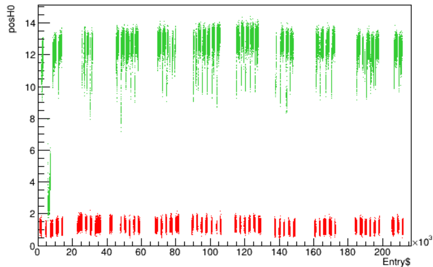
Run 5727 quartetwise, posH0 vs time
