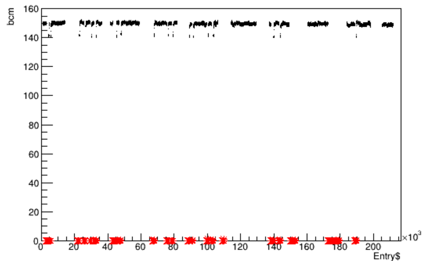
Run 5727 quartetwise, bcm vs time
