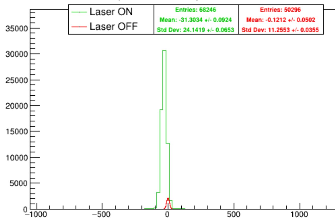
Run 5727 quartetwise, asym0sub: Beam ON
