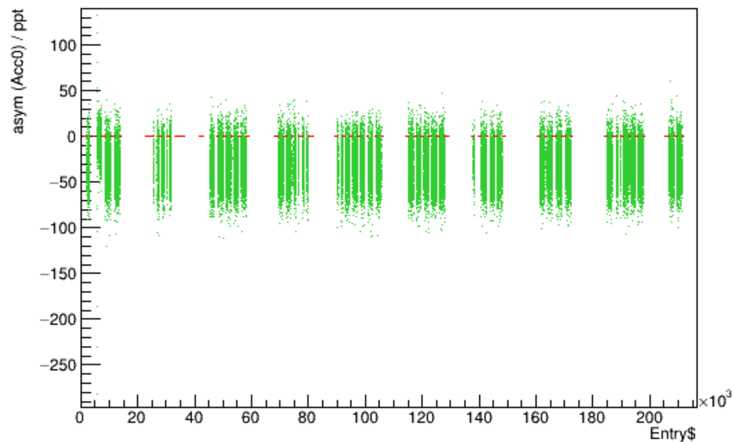
Run 5727 quartetwise, asym0sub vs time
