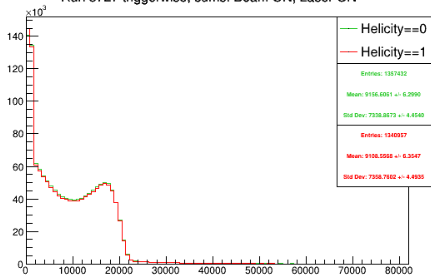
Run 5727 triggerwise, sums: Beam ON, Laser ON
