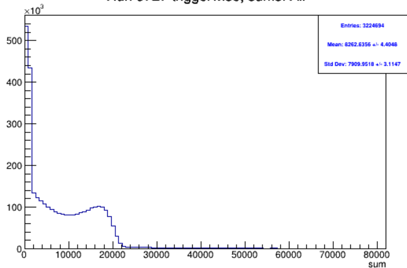
Run 5727 triggerwise, sums: All
