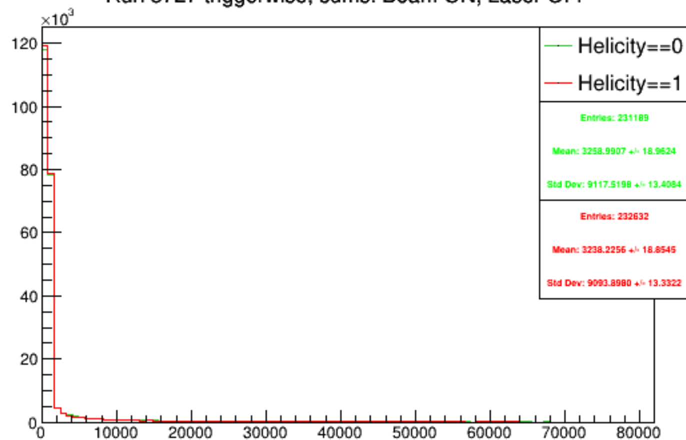
Run 5727 triggerwise, sums: Beam ON, Laser OFF
