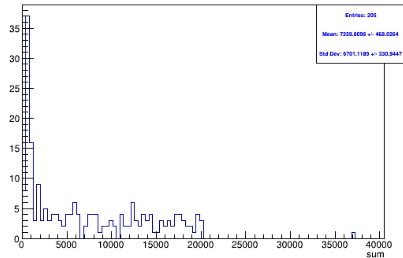
Run 5727 triggerwise, sums: Beam OFF
